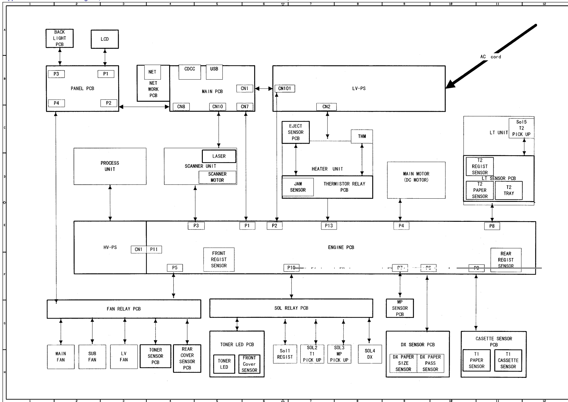
Appendix 1. Connection Diagram, HL-1650/1670N
