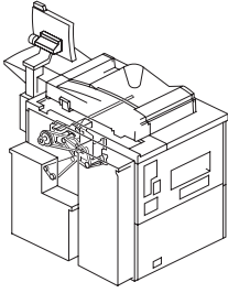
65. DRIVE SECTION 7
