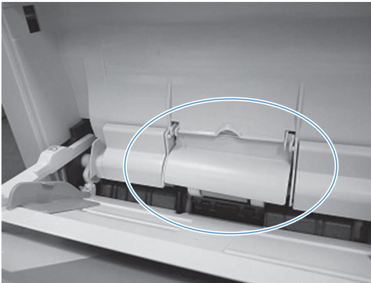
Figure 3-86 Examine the roller cover
