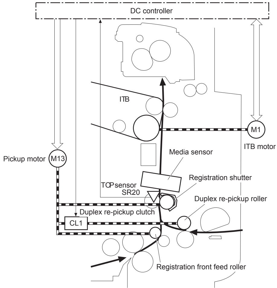
Figure 1-39 Paper-feed mechanism
