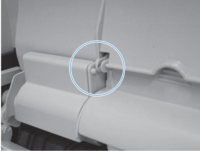
Figure 3-87 Roller out of position
