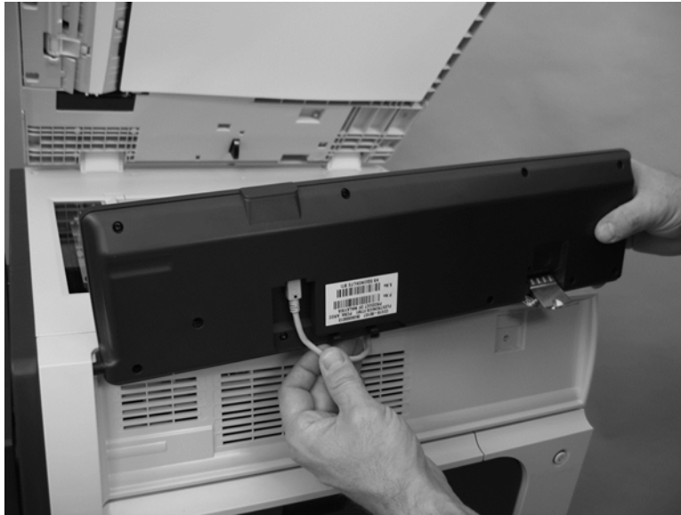
Figure 2-6 Remove the control panel (3 of 3)
