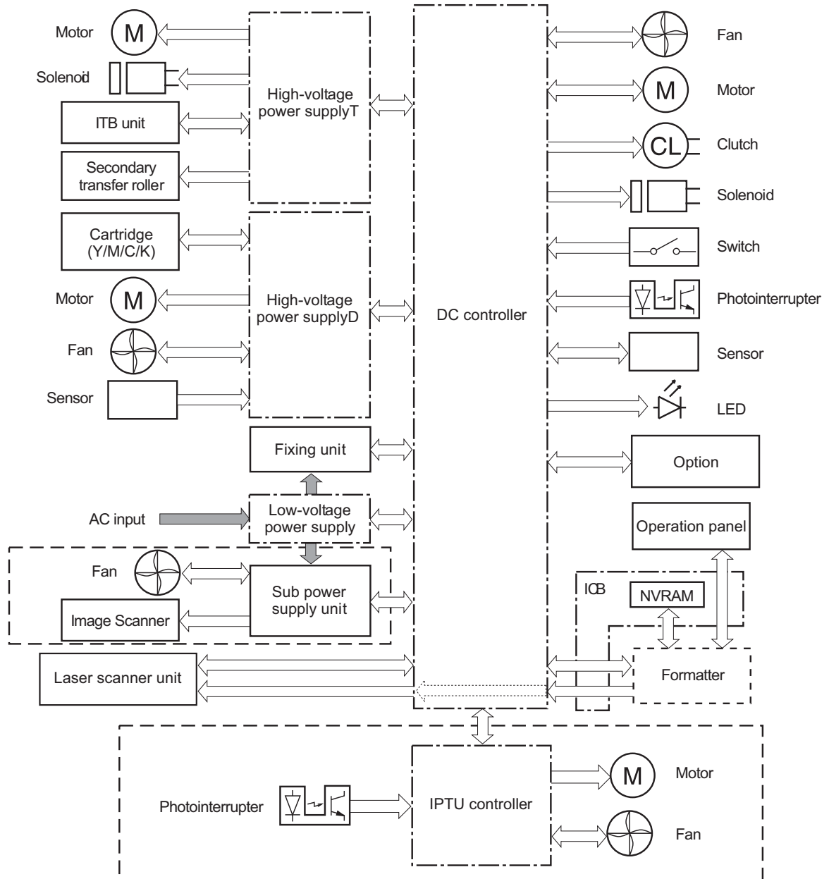
Figure 1-4 DC controller block diagram
