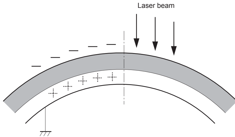
Figure 1-16 Laser-beam exposure
