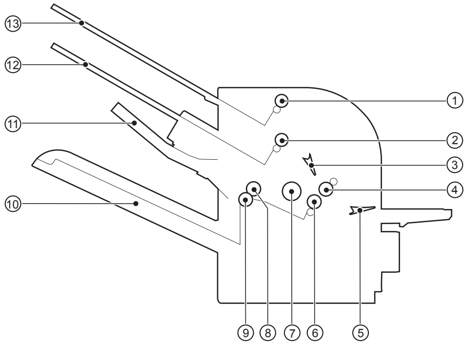
Figure 3-53 Stapler/stacker
