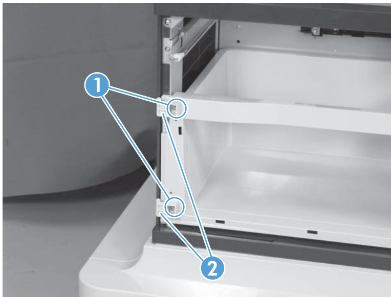
Figure 2-298 Remove the left cover (optional paper feeder) (1 of 3)
