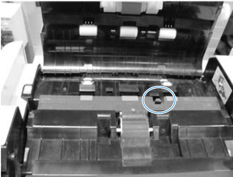
Figure 3-97 Registration sensor flag location
