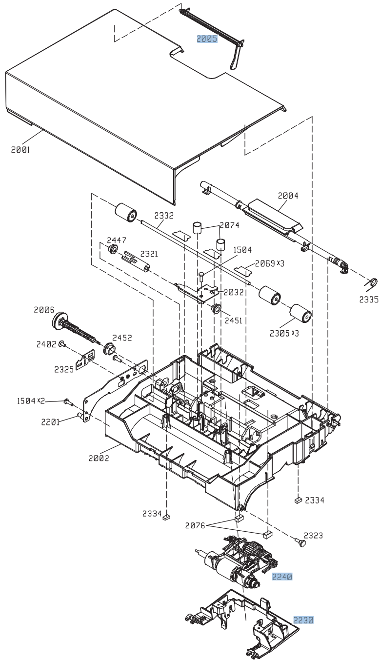
Figure 4-45 Document feeder assembly (5 of 5)
