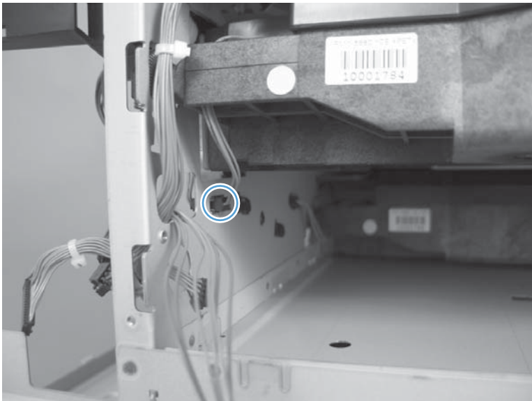
Figure 2-257 Remove the laser/scanner assembly (Y/M) (2 of 5)
