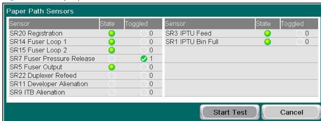
Figure 3-46 Paper path sensors
