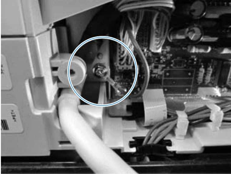
Figure 3-100 Ground wire for ADF cable not touching the test point
