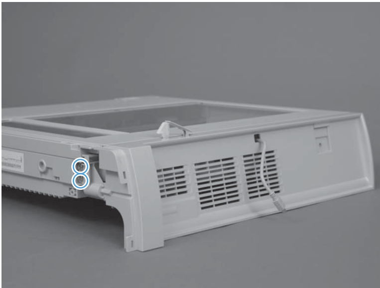
Figure 2-118 Remove the S-ASSY-CP-ADAPTER (CP adapter assembly) (1 of 4)
