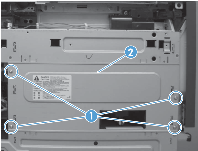
Figure 2-184 Remove the cartridge fan and environmental sensor (1 of 7)
