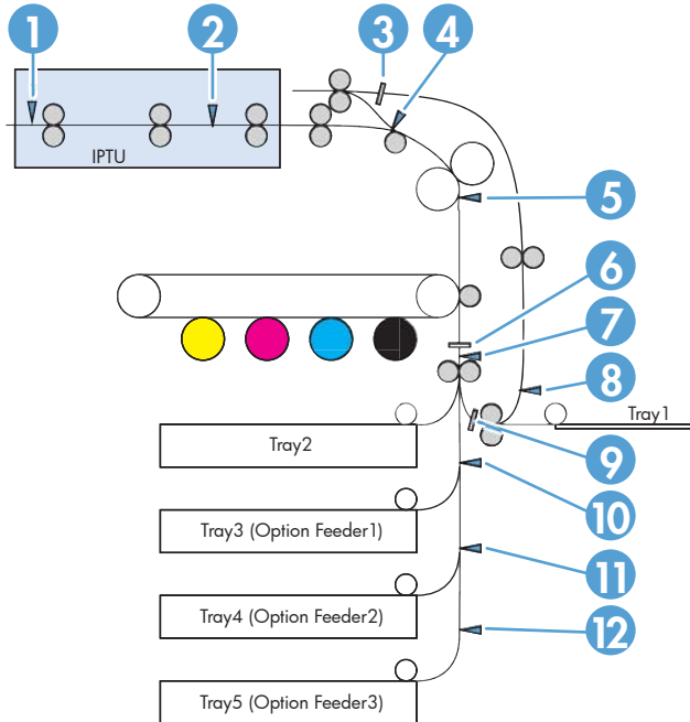
Figure 3-103 Paper path sensor locations
