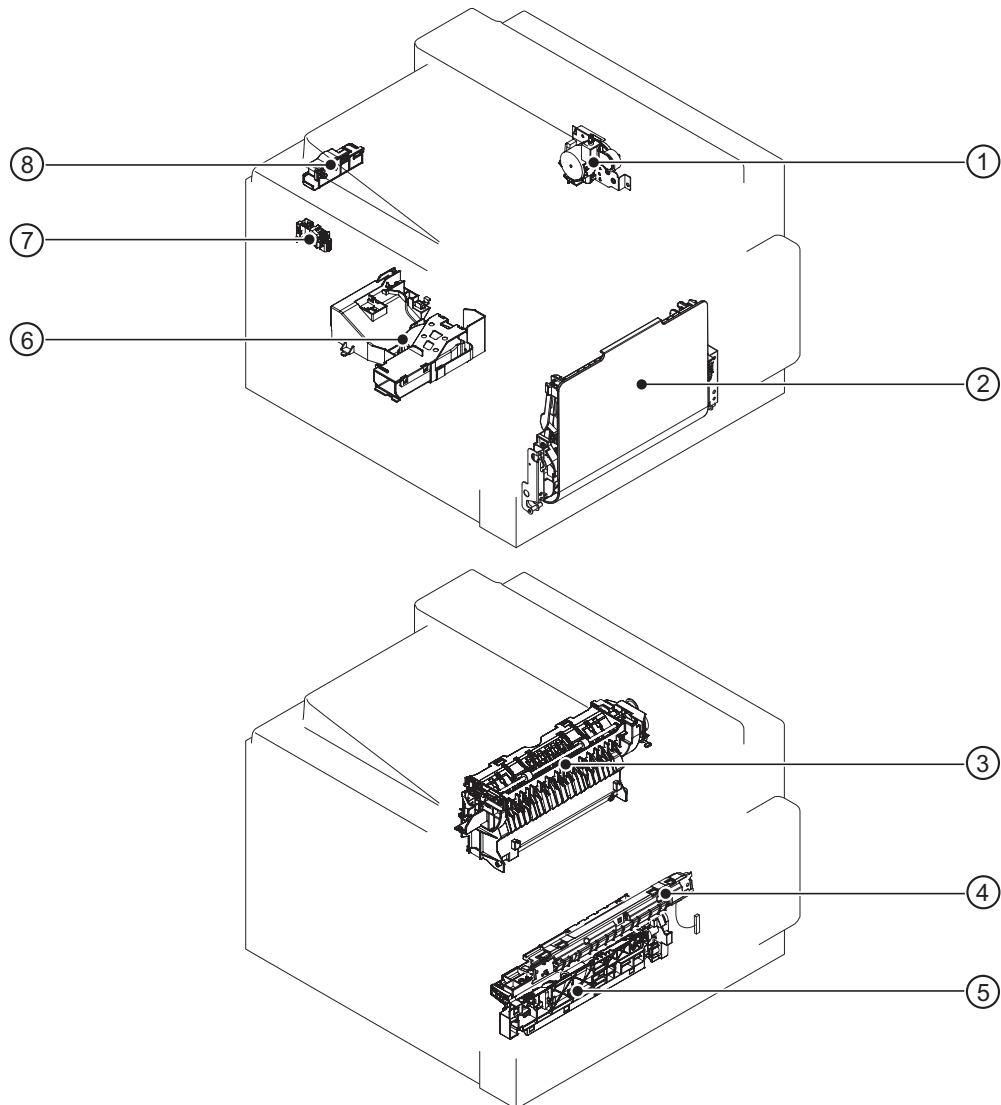
Figure 3-59 Major component locations (2 of 4)
