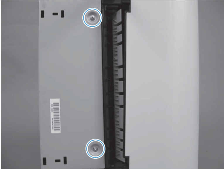
Figure 2-343 Remove the stapling mailbox PCA (1 of 5)
