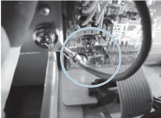
Figure 3-99 Ground wire for ADF cable touching the test point
