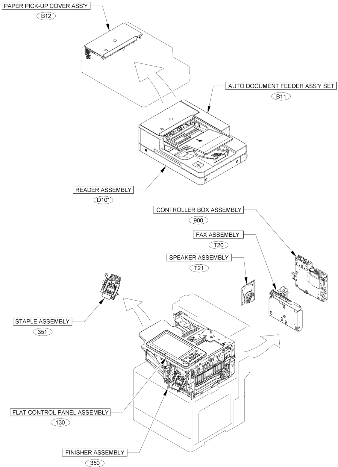
Figure A1A ASSEMBLY LOCATION DIAGRAM (IR-ADV DX C477iFZ)
