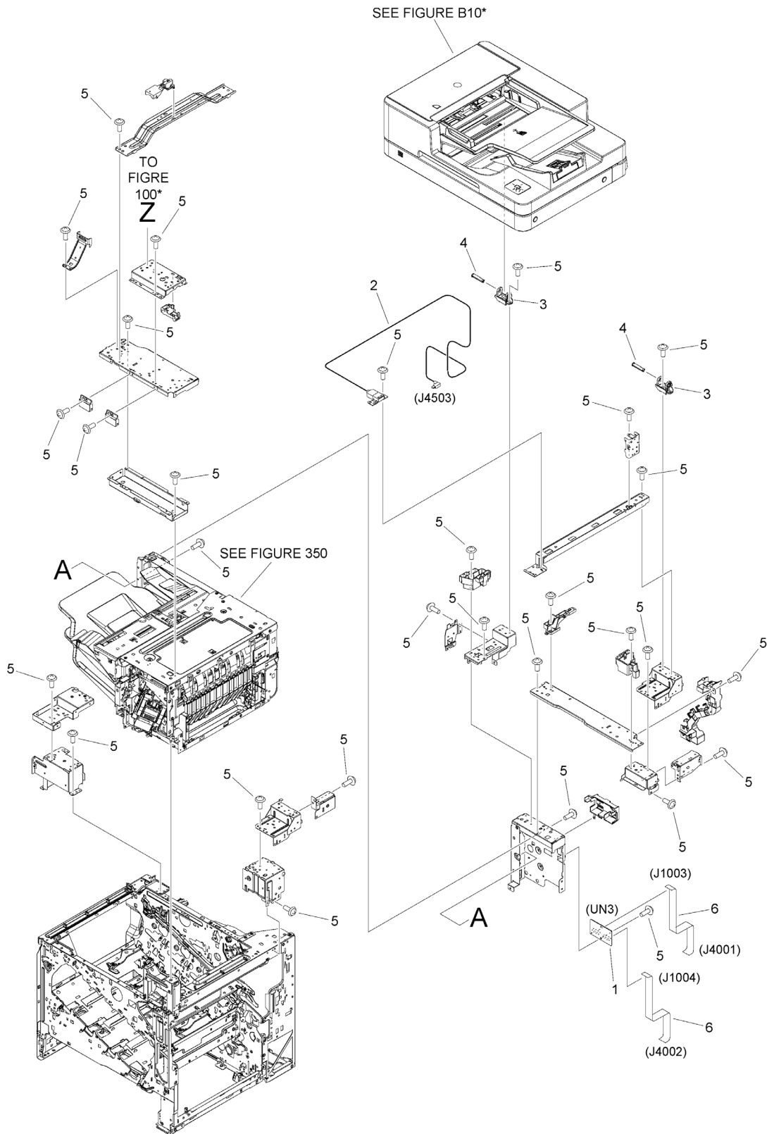
Figure 107A INTERNAL COMPONENTS 7 (FINISHER model)
