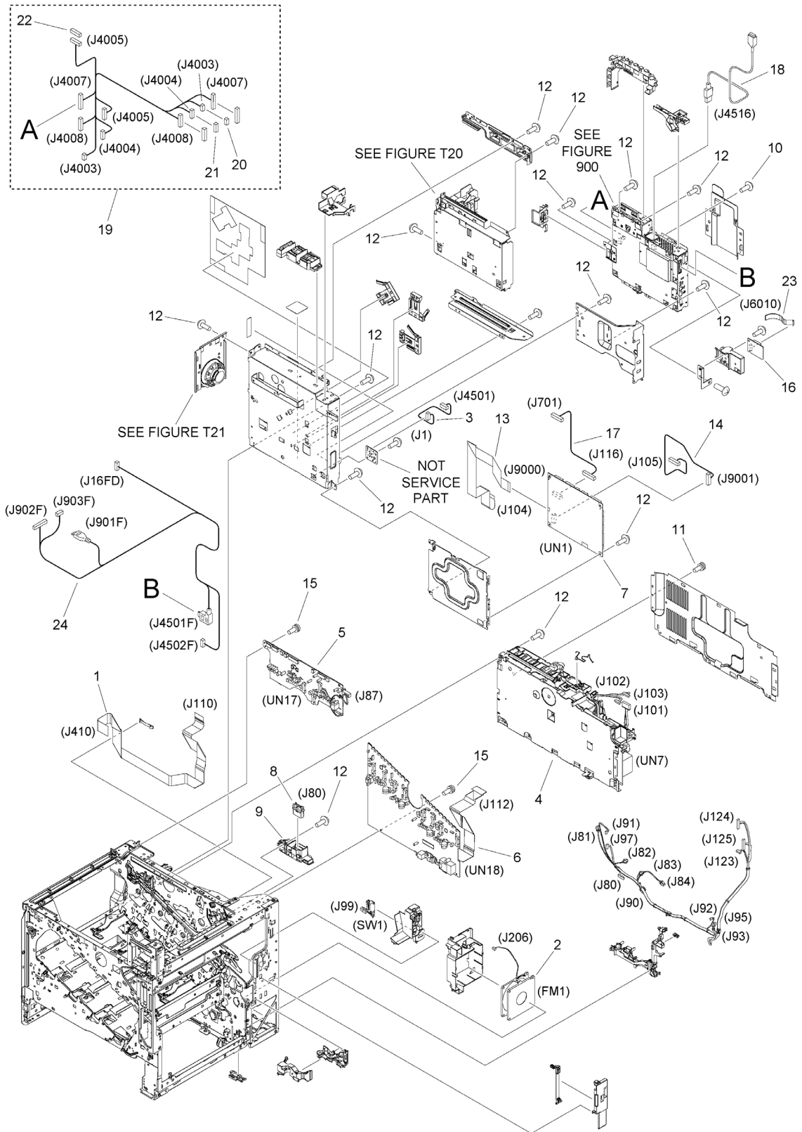
Figure 106A INTERNAL COMPONENTS 6 (IR-ADV DX C477iFZ)
