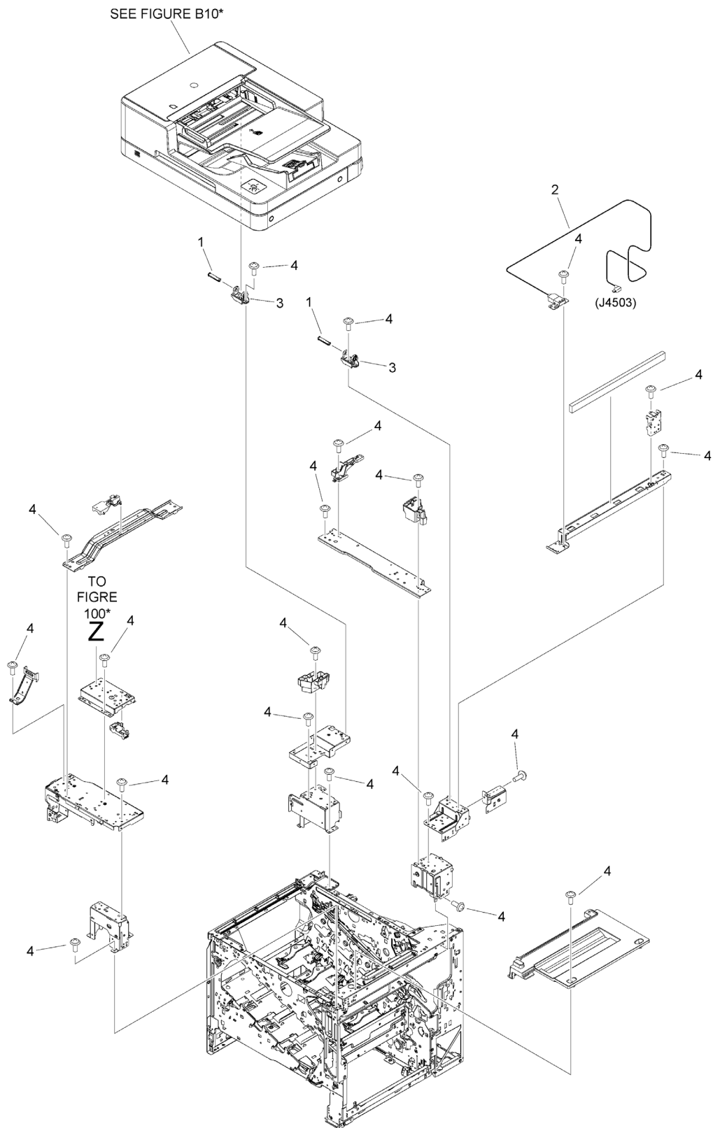
Figure 107B INTERNAL COMPONENTS 7 (MODEL WITHOUT FINISHER)
