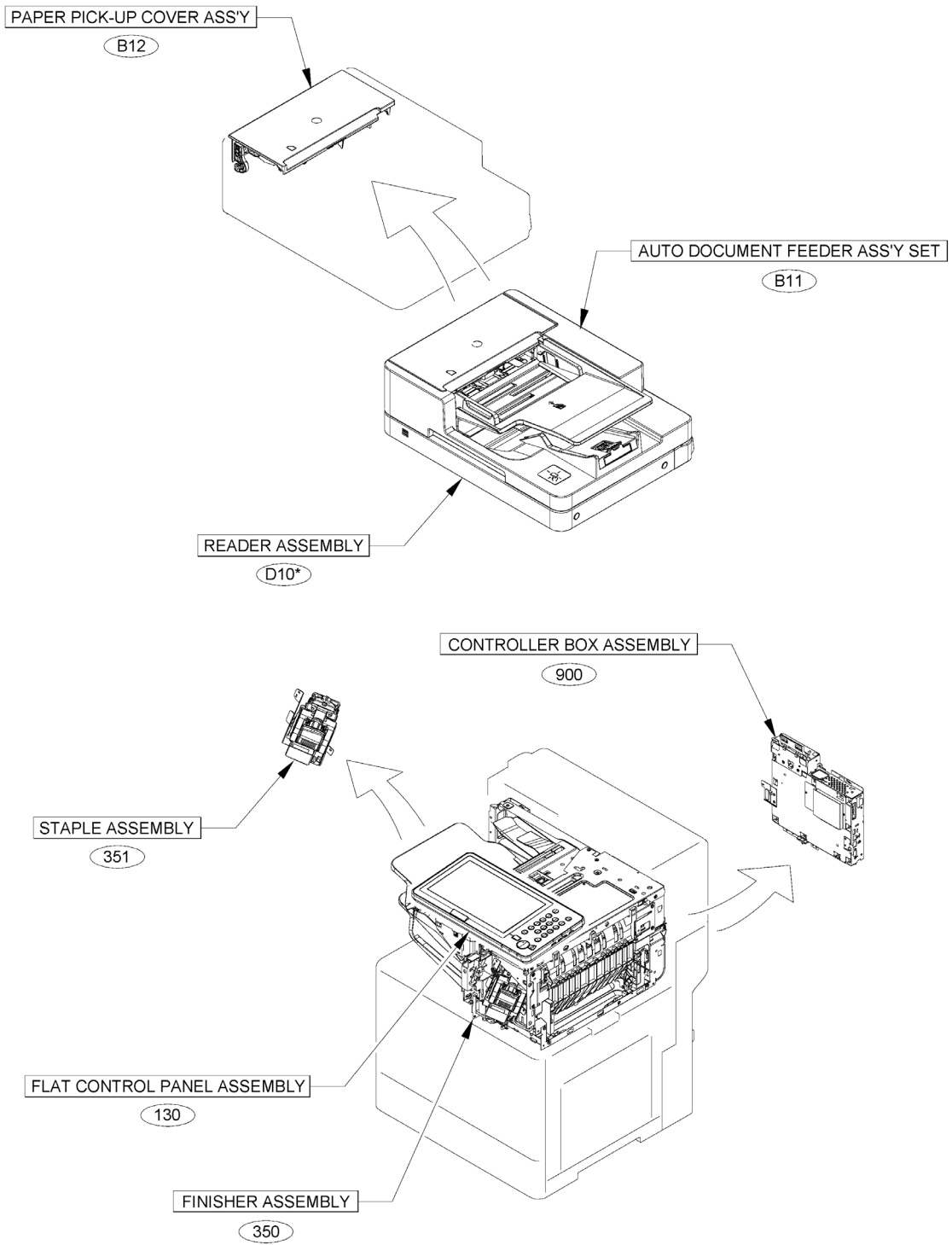
Figure A1F ASSEMBLY LOCATION DIAGRAM (IR-ADV DX C477i)
