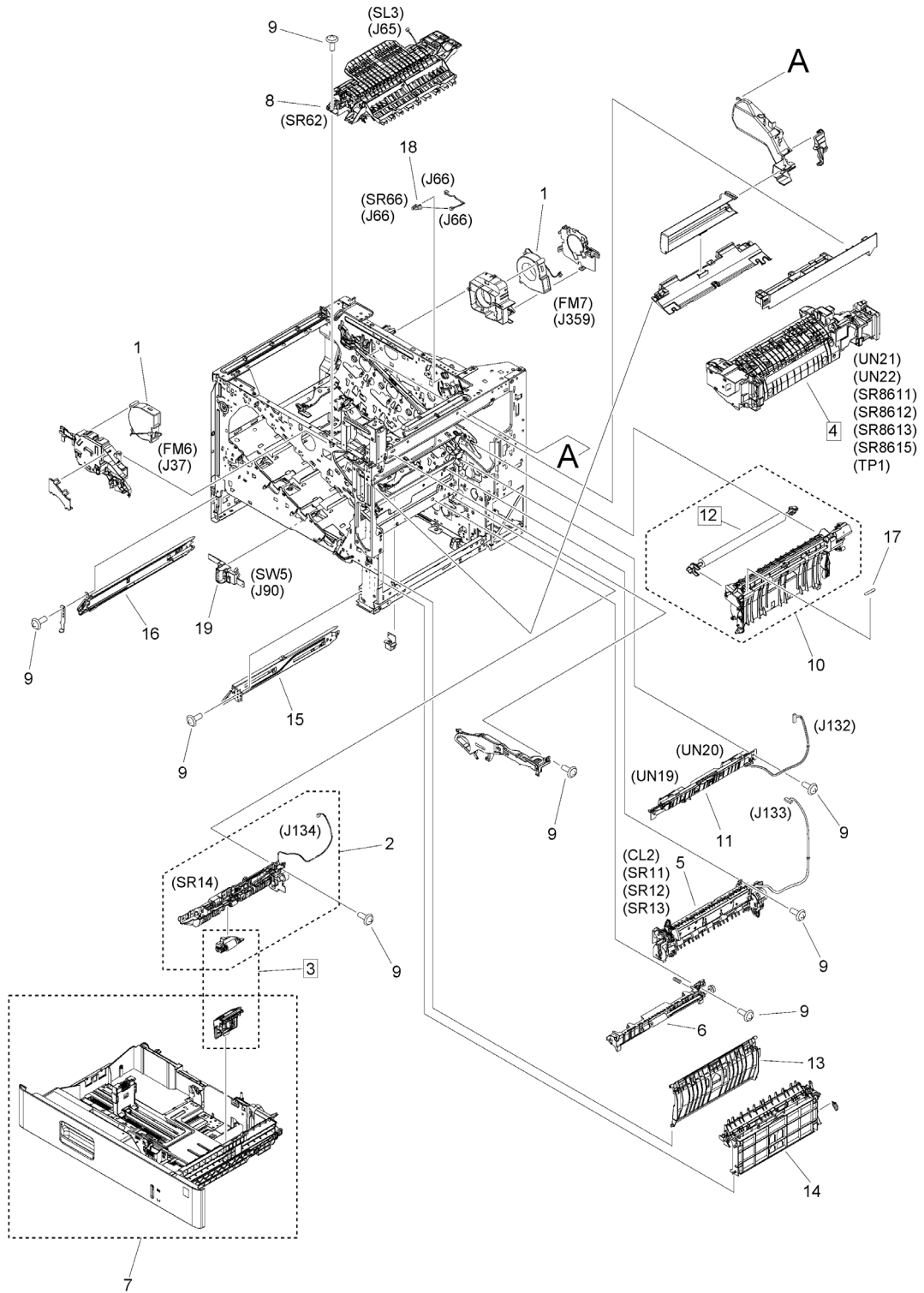
Figure 104A INTERNAL COMPONENTS 4
