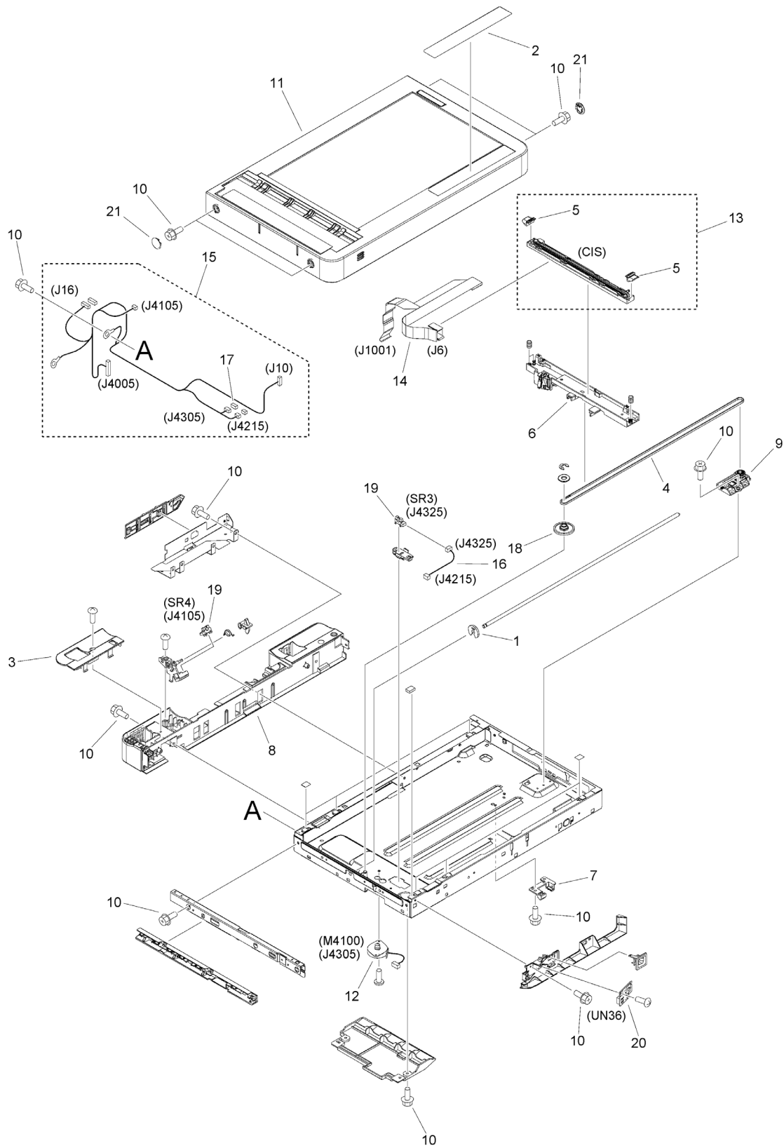
Figure D10 READER ASSEMBLY
