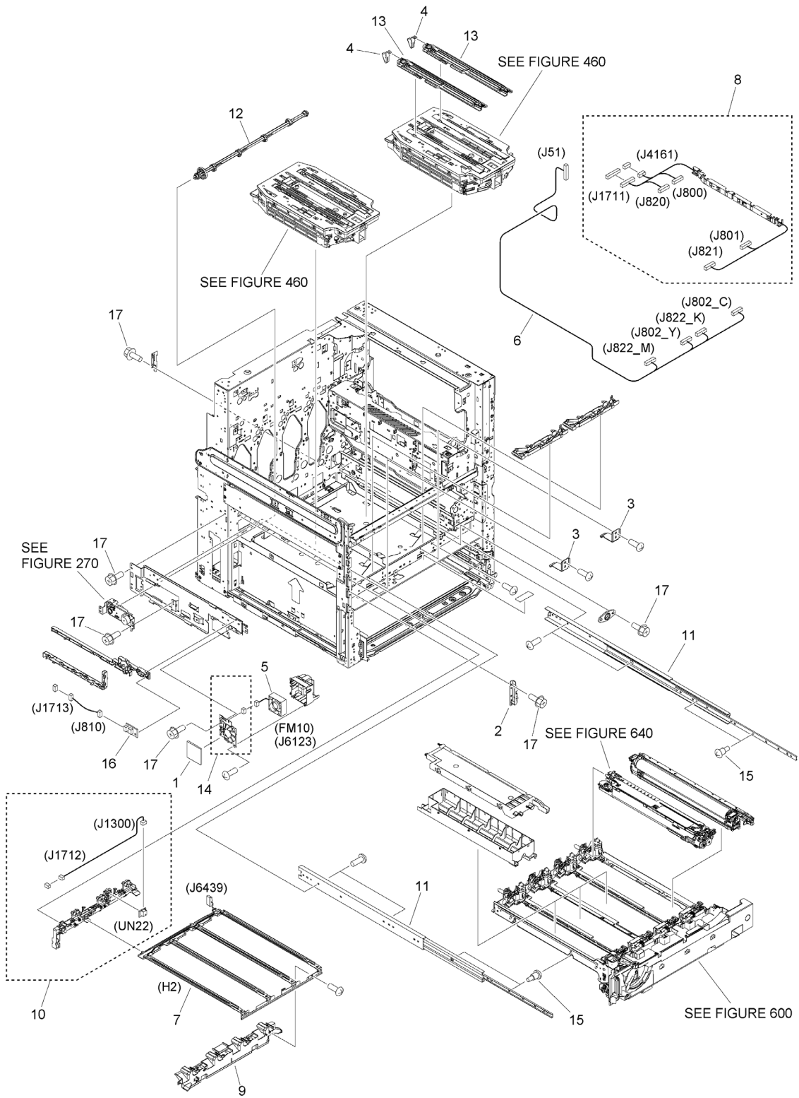
Figure 104 INTERNAL COMPONENTS 4
