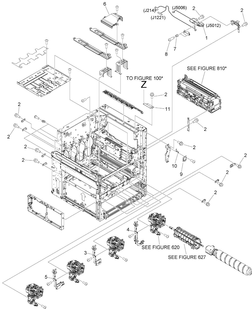
Figure 105 INTERNAL COMPONENTS 5
