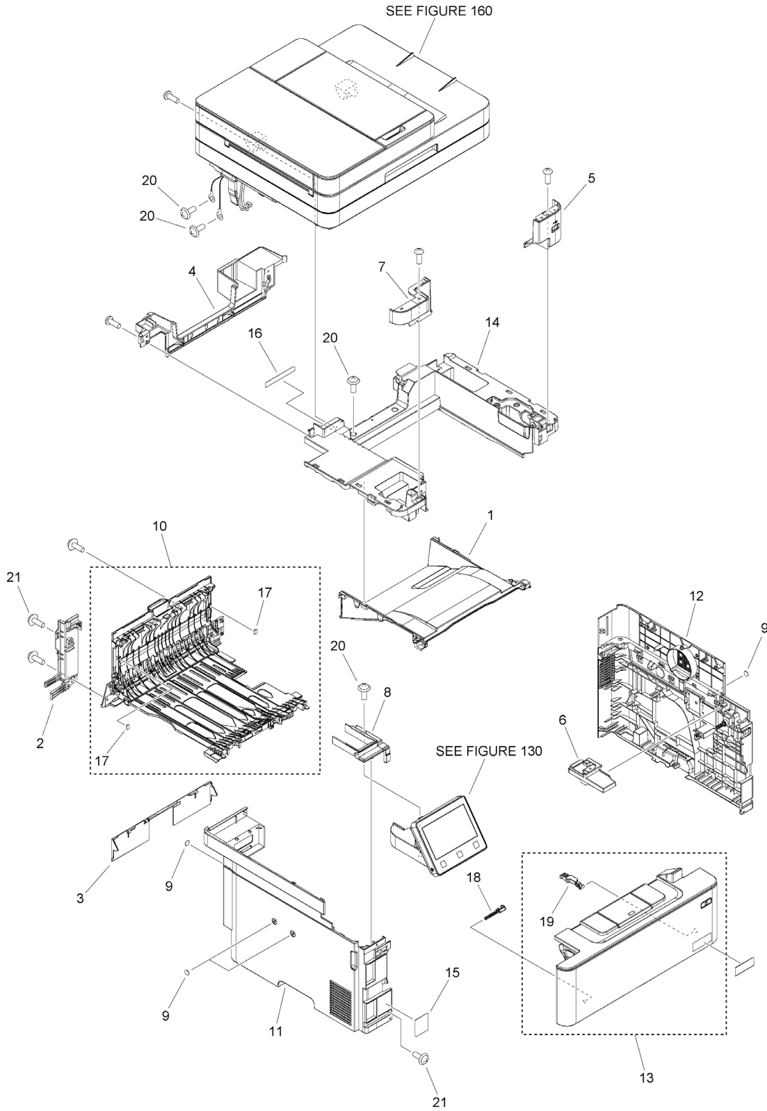
Figure 100A EXTERNAL COVERS, PANELS, ETC. (MF429dw)
