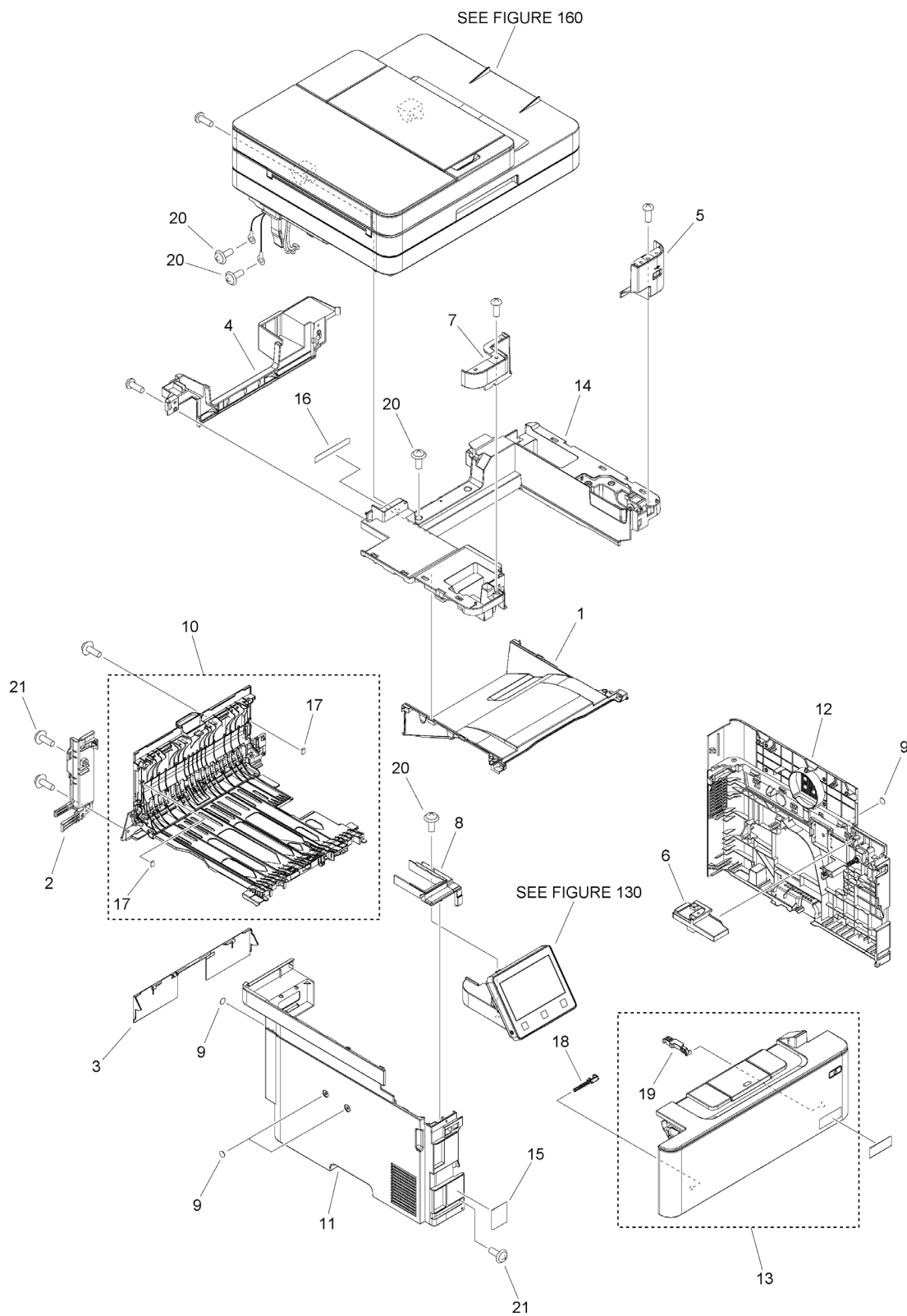
Figure 100B EXTERNAL COVERS, PANELS, ETC. (MF429x)
