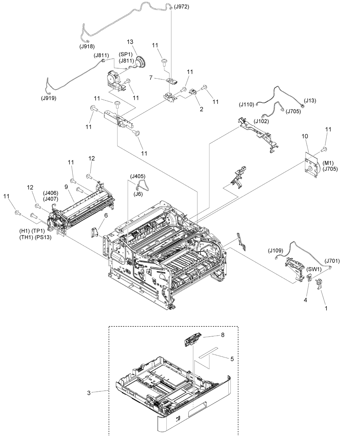
Figure 102A INTERNAL COMPONENTS 2 (120V)
