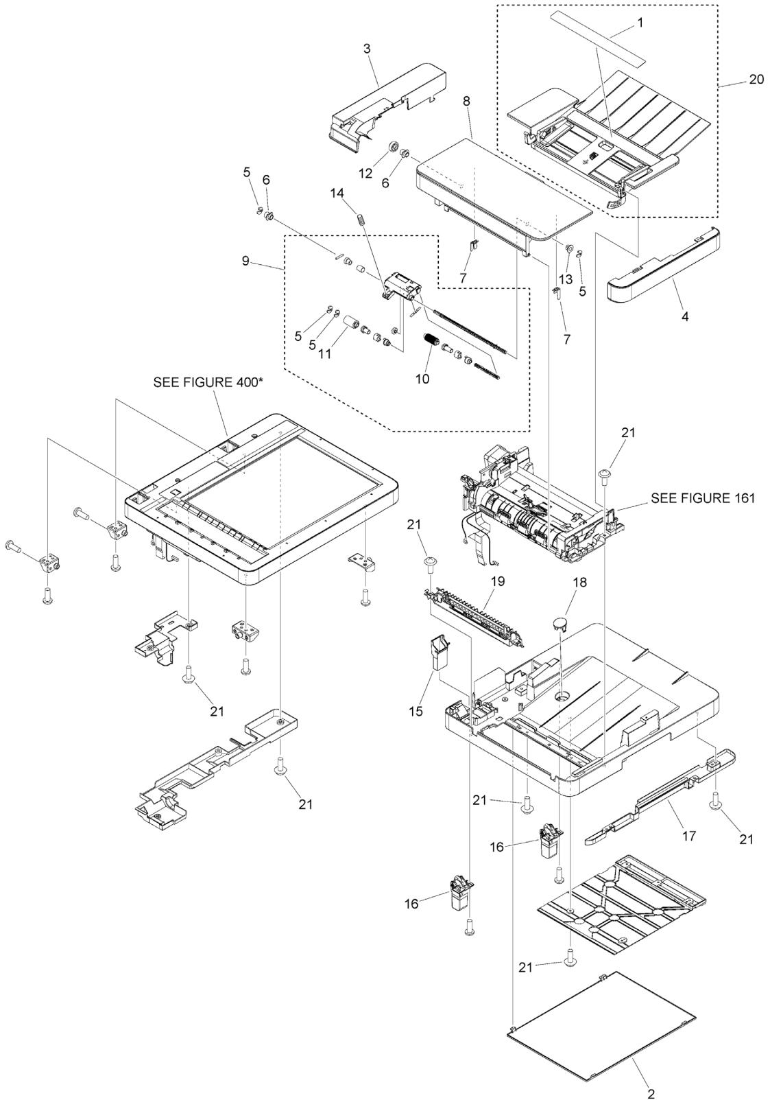
Figure 160 READER/ADF ASSEMBLY
