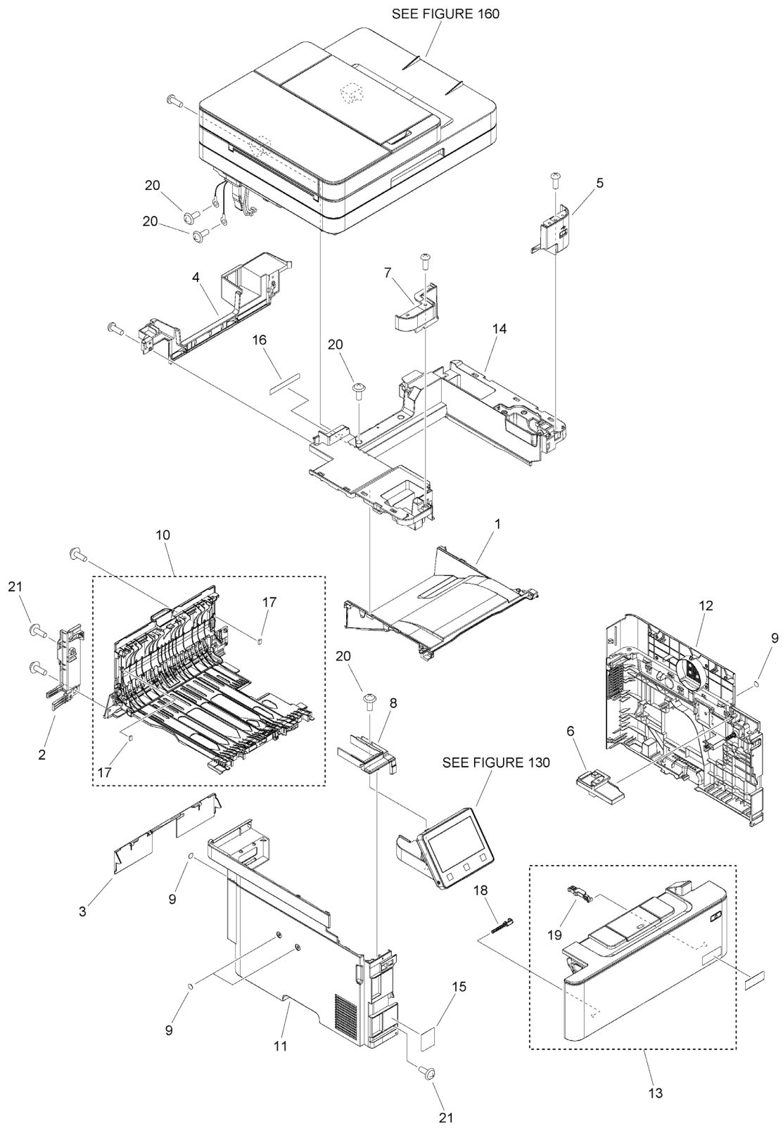
Figure 100D EXTERNAL COVERS, PANELS, ETC. (MF424dw)
