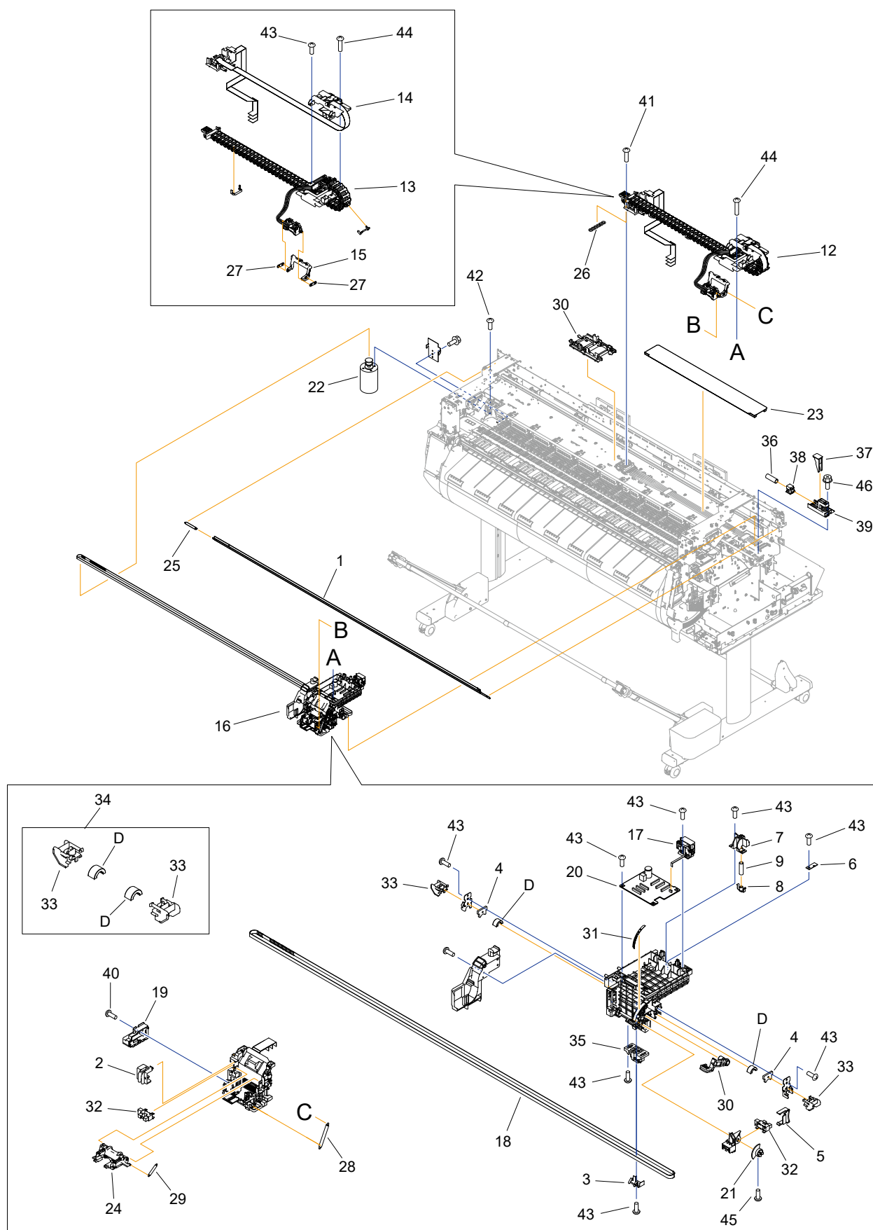
FIGURE 6 Carriage, Tube Unit & Film Strip
