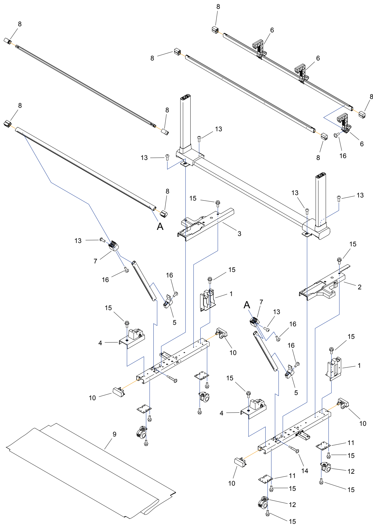
FIGURE R5 Stacker
