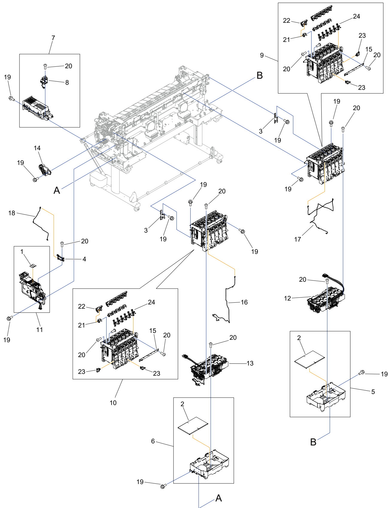
FIGURE 5 Ink Tank Unit & Purge Unit
