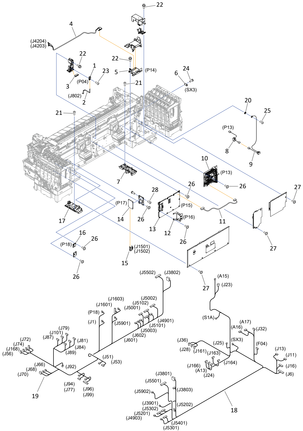
FIGURE 3 Electrical Parts
