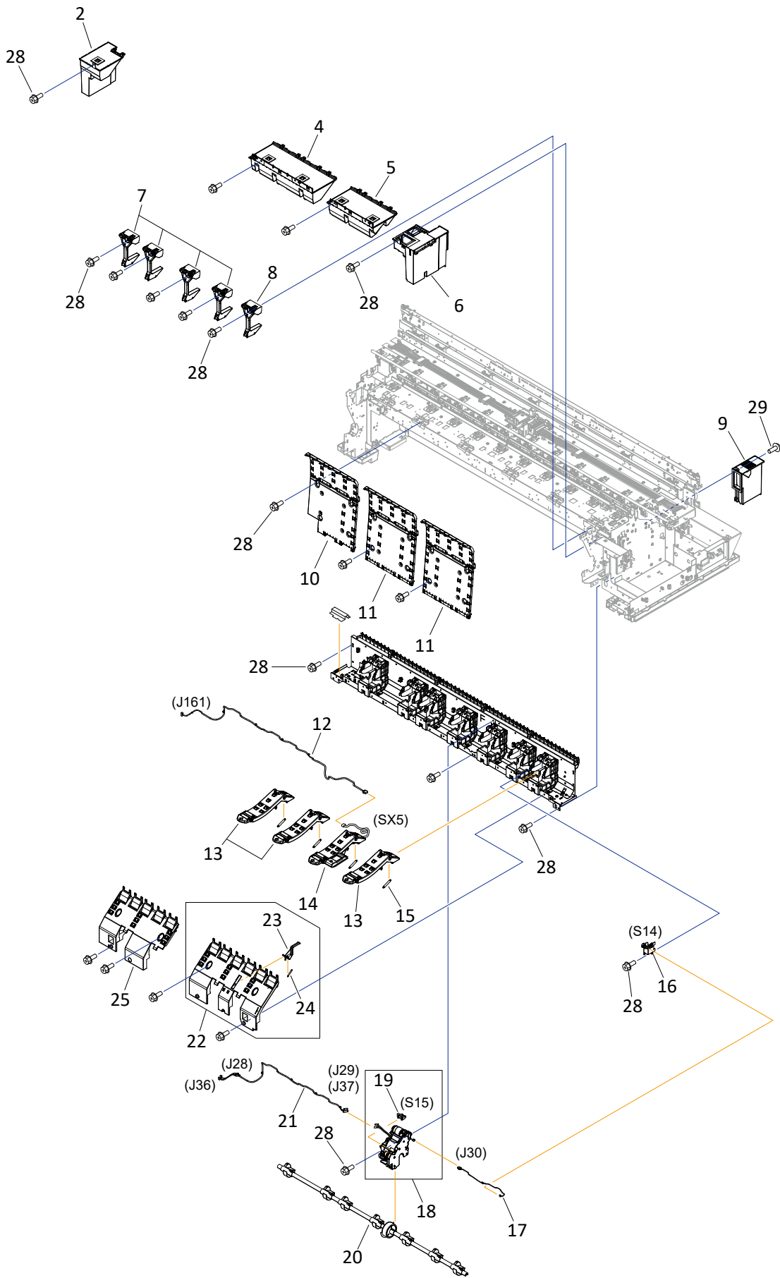
FIGURE 10 Upper Roll Unit, Suction Fan & Waste Ink Unit
