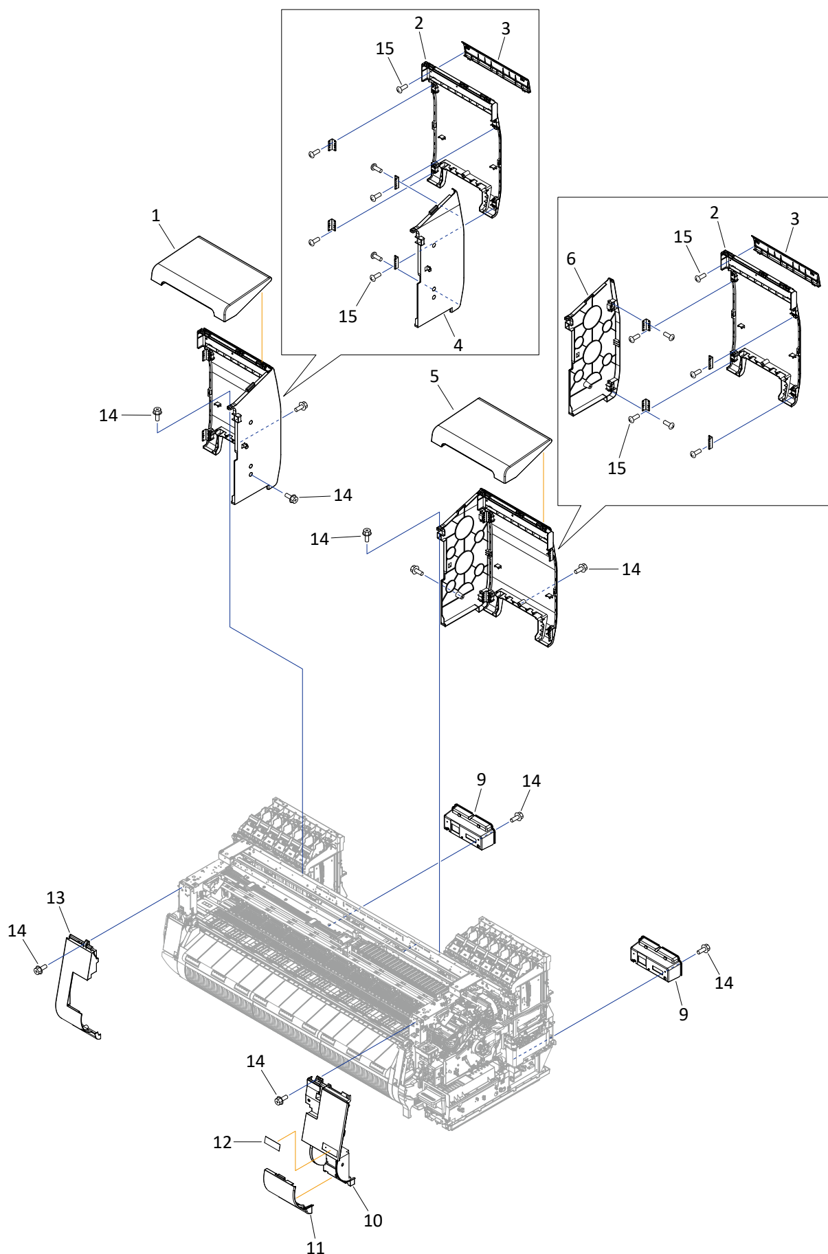
FIGURE 2 Front Covers & Rear Covers
