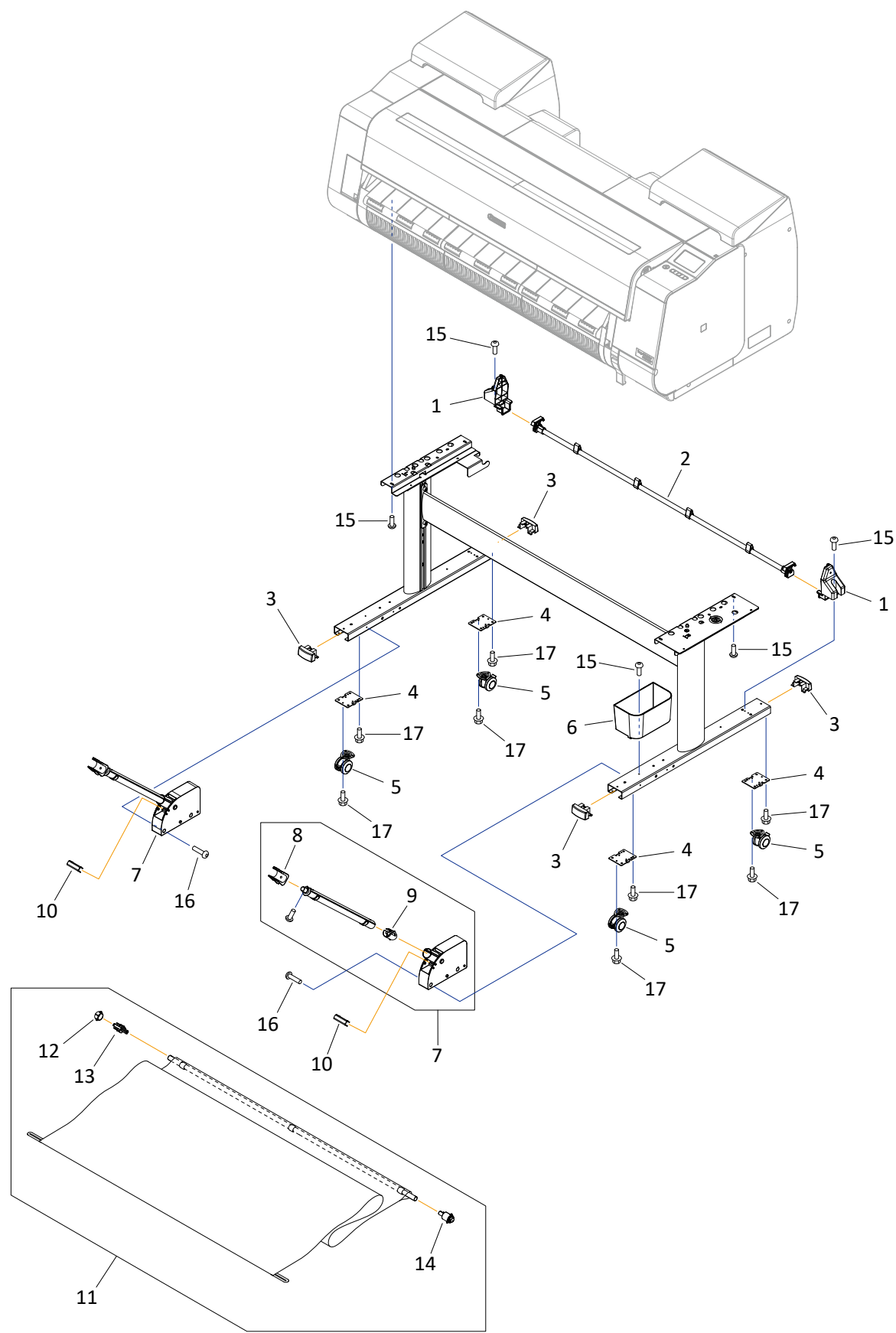
FIGURE 12 Stand Unit SD-21
