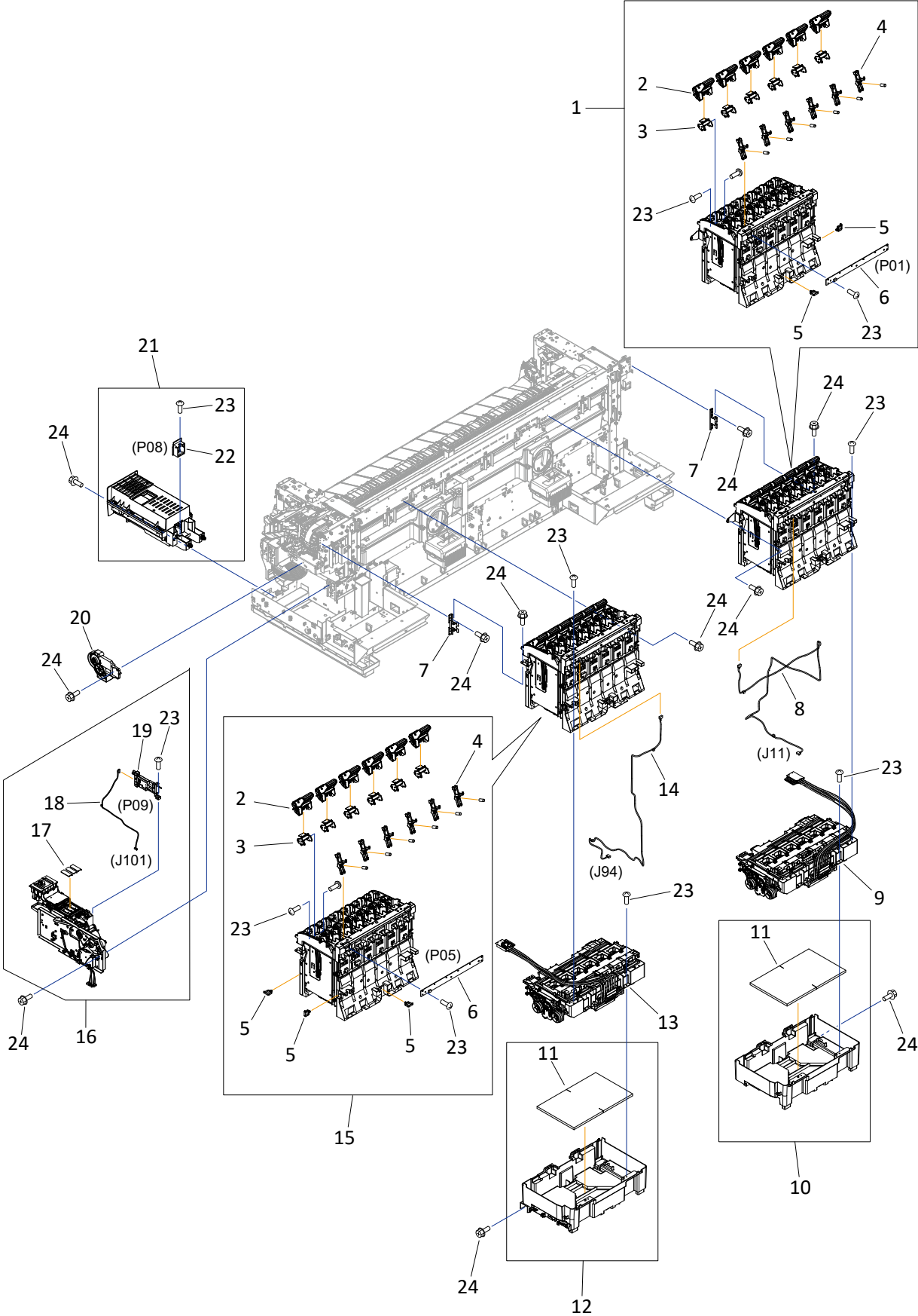
FIGURE 4 Ink Tank Unit & Purge Unit
