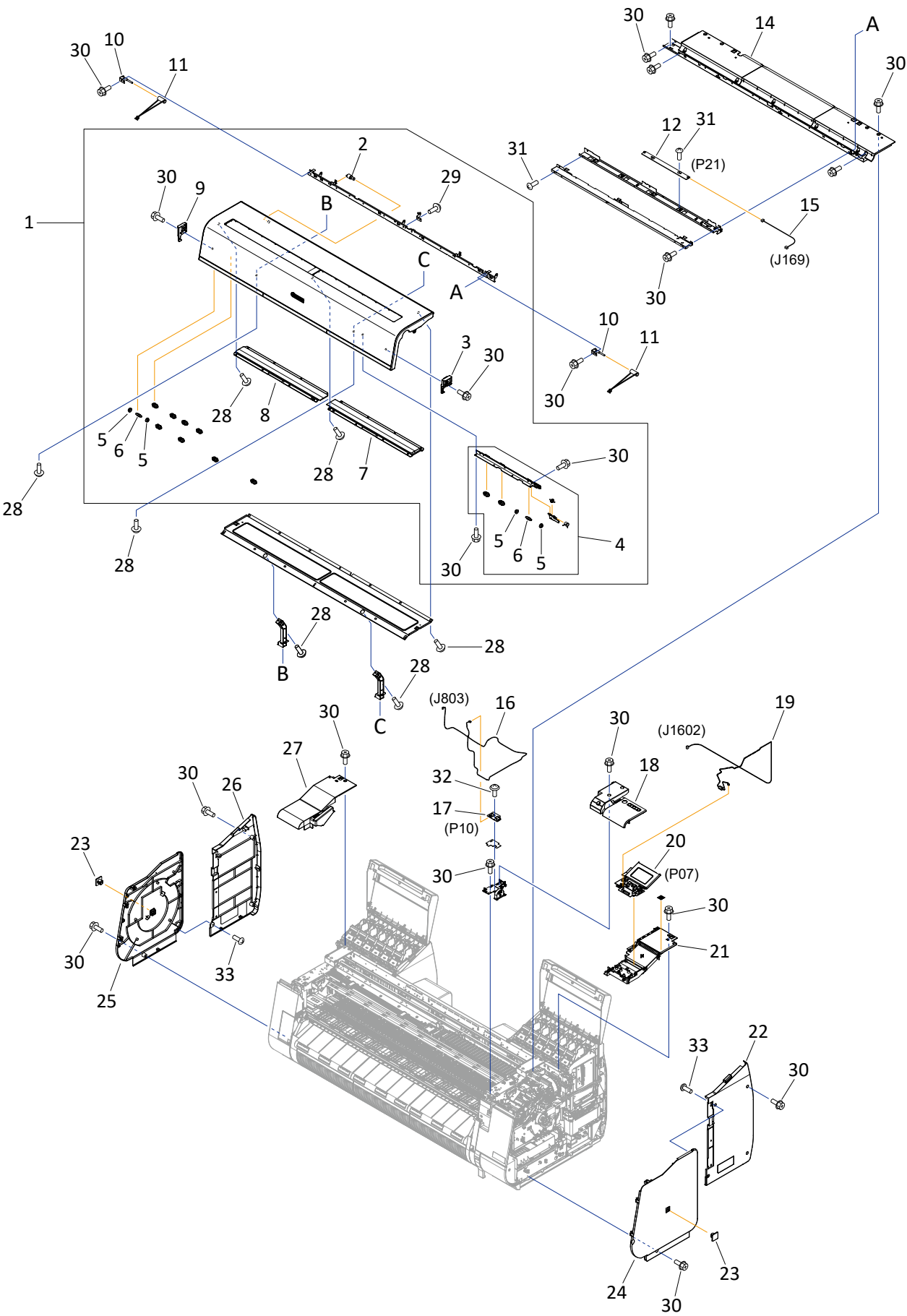
FIGURE 1 Top Covers & Side Covers
