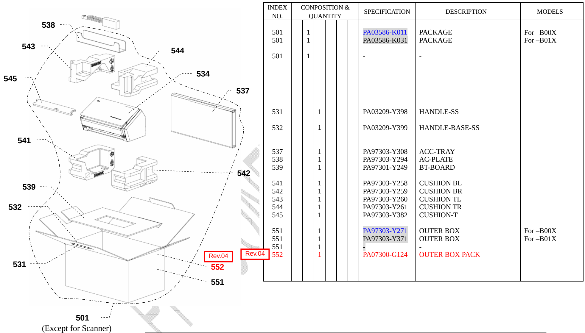
FIGURE 5-1. S1500 PACKAGING BOX for Scanner
