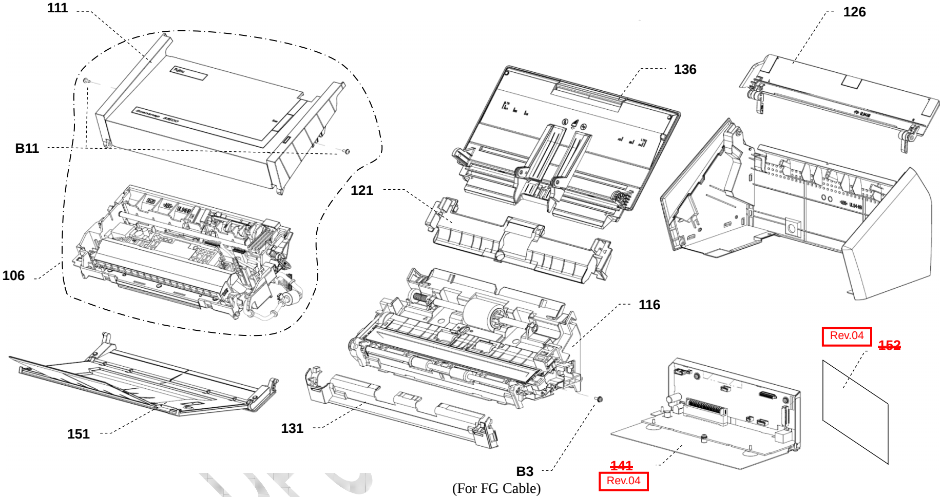
FIGURE 1. FINAL ASSEMBLY
