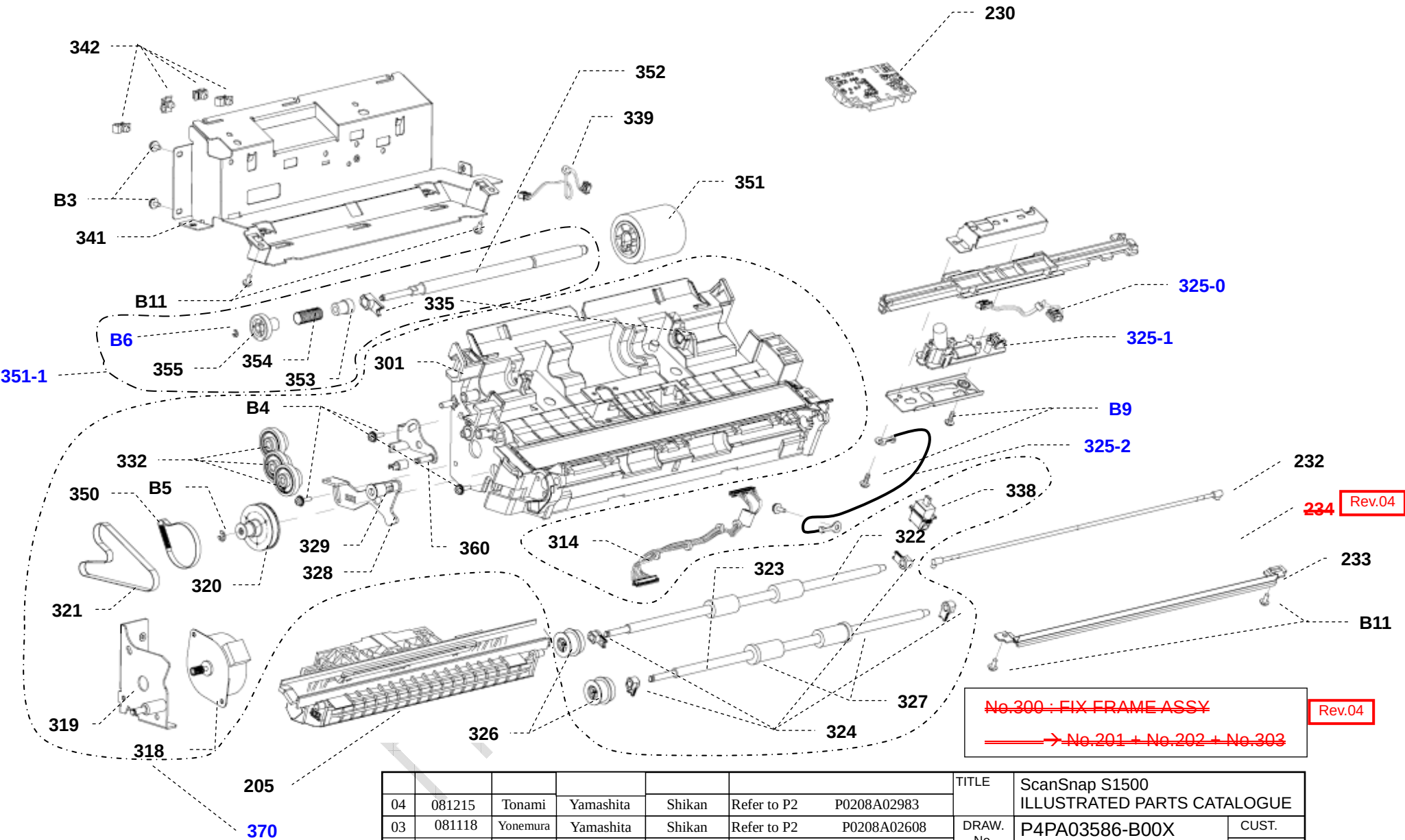
FIGURE 3. FIXED UNIT
