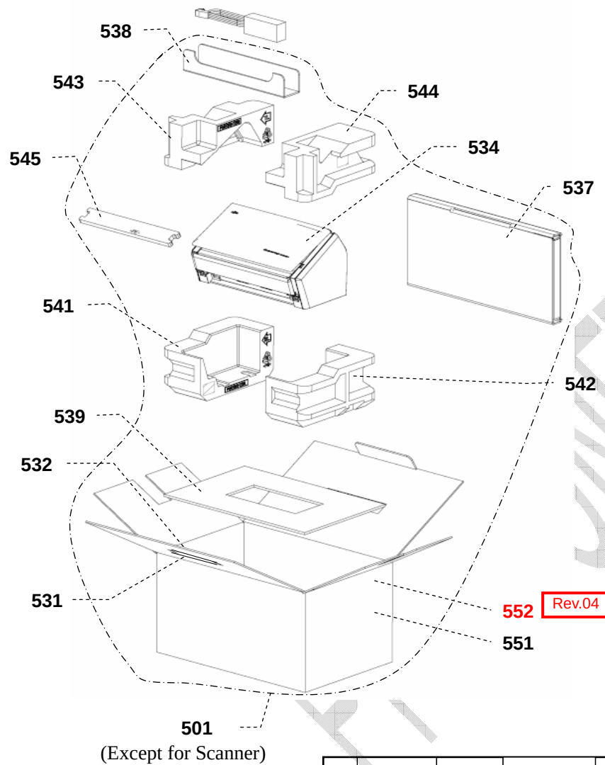
FIGURE 5-2. S1500M PACKAGING BOX for Scanner
