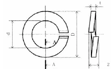
FIGURE B.6 WASHER
