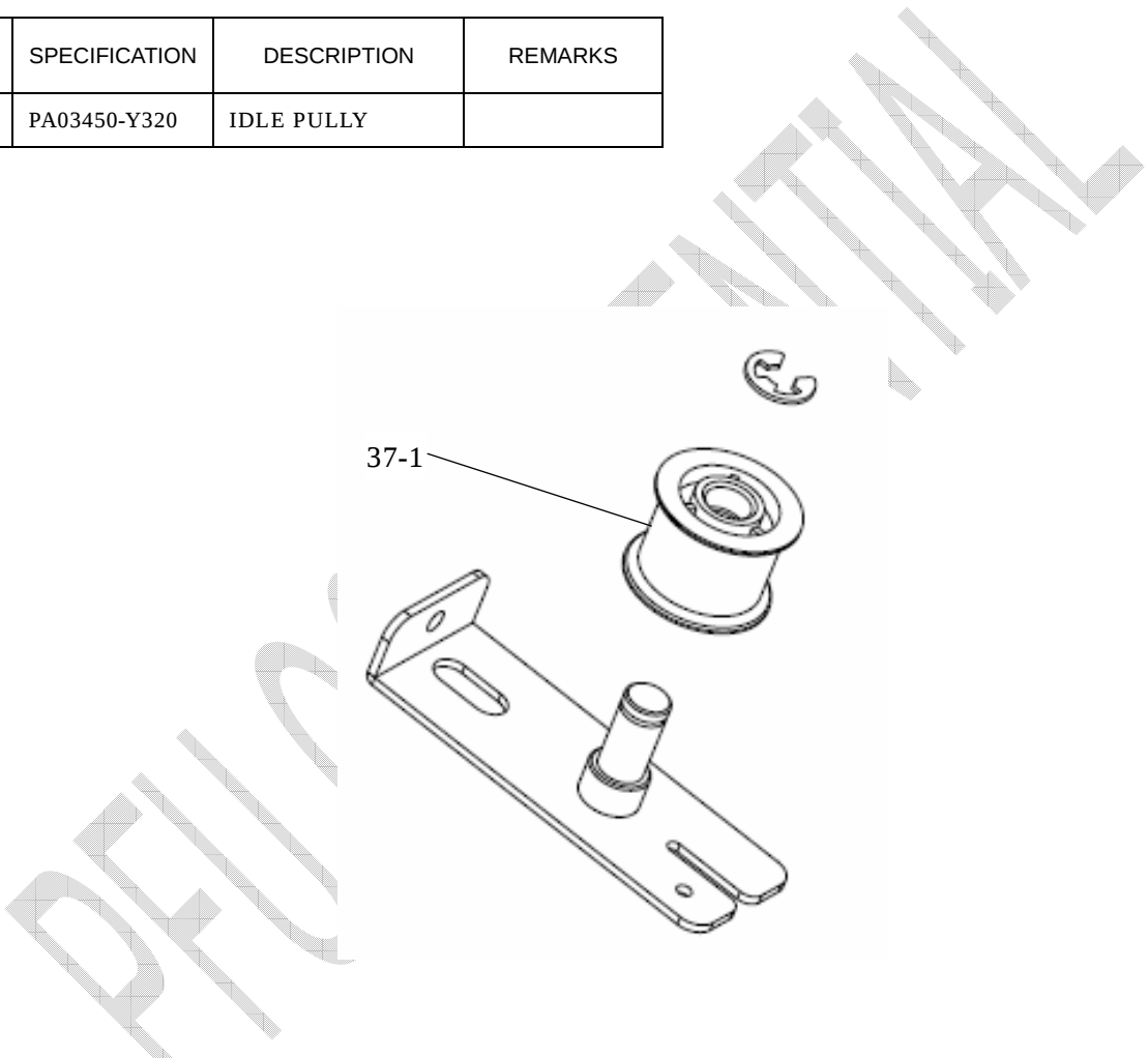
FIGURE 37. TENSIONASSY ( -F030 )
