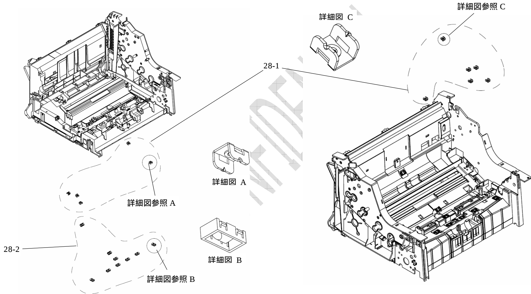
FIGURE 28. FIX-ASM ( -F001 )
