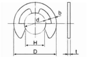
FIGURE B2 E-RING
