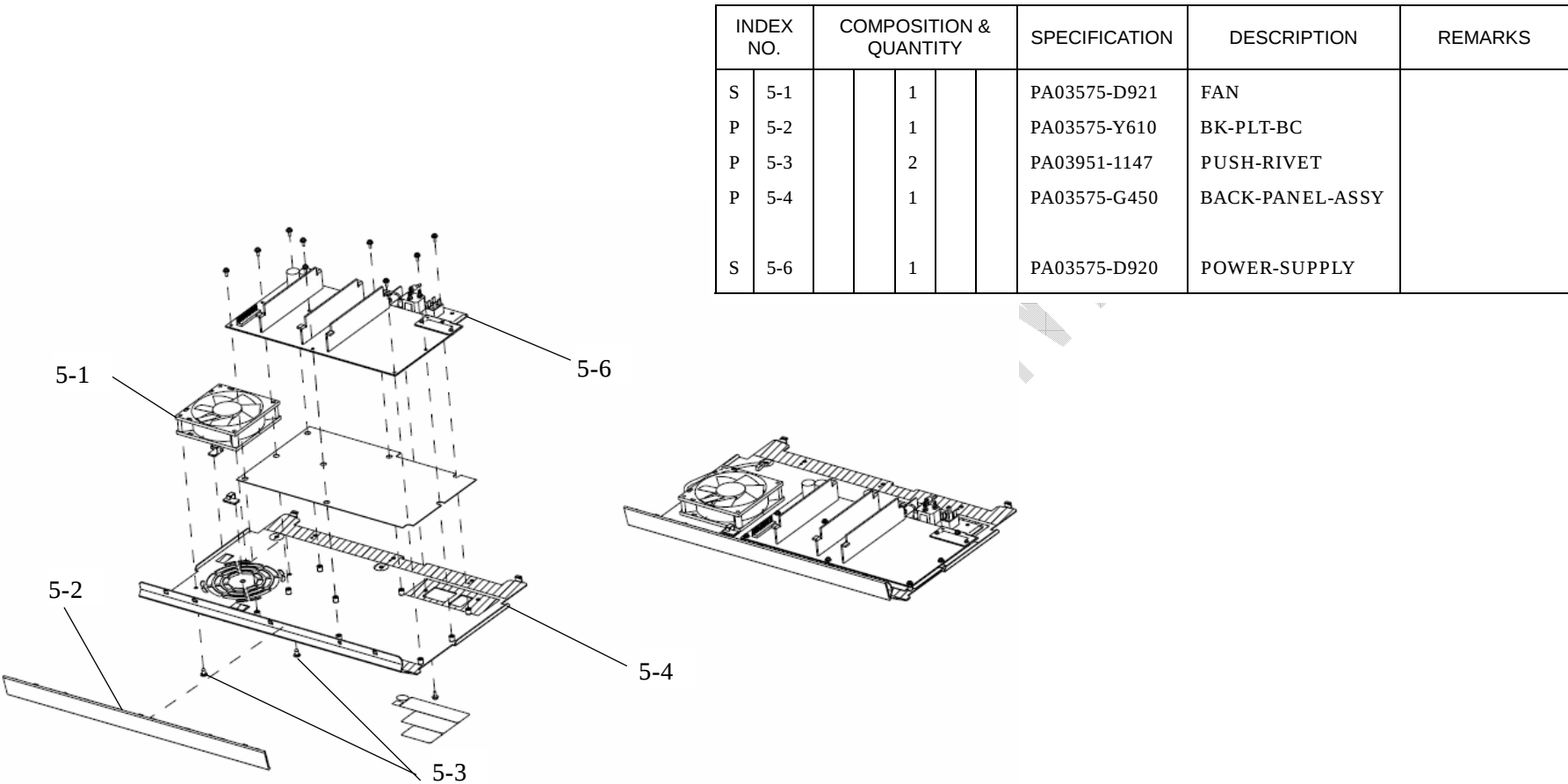
FIGURE 5. PWR-UNIT (-D450)
