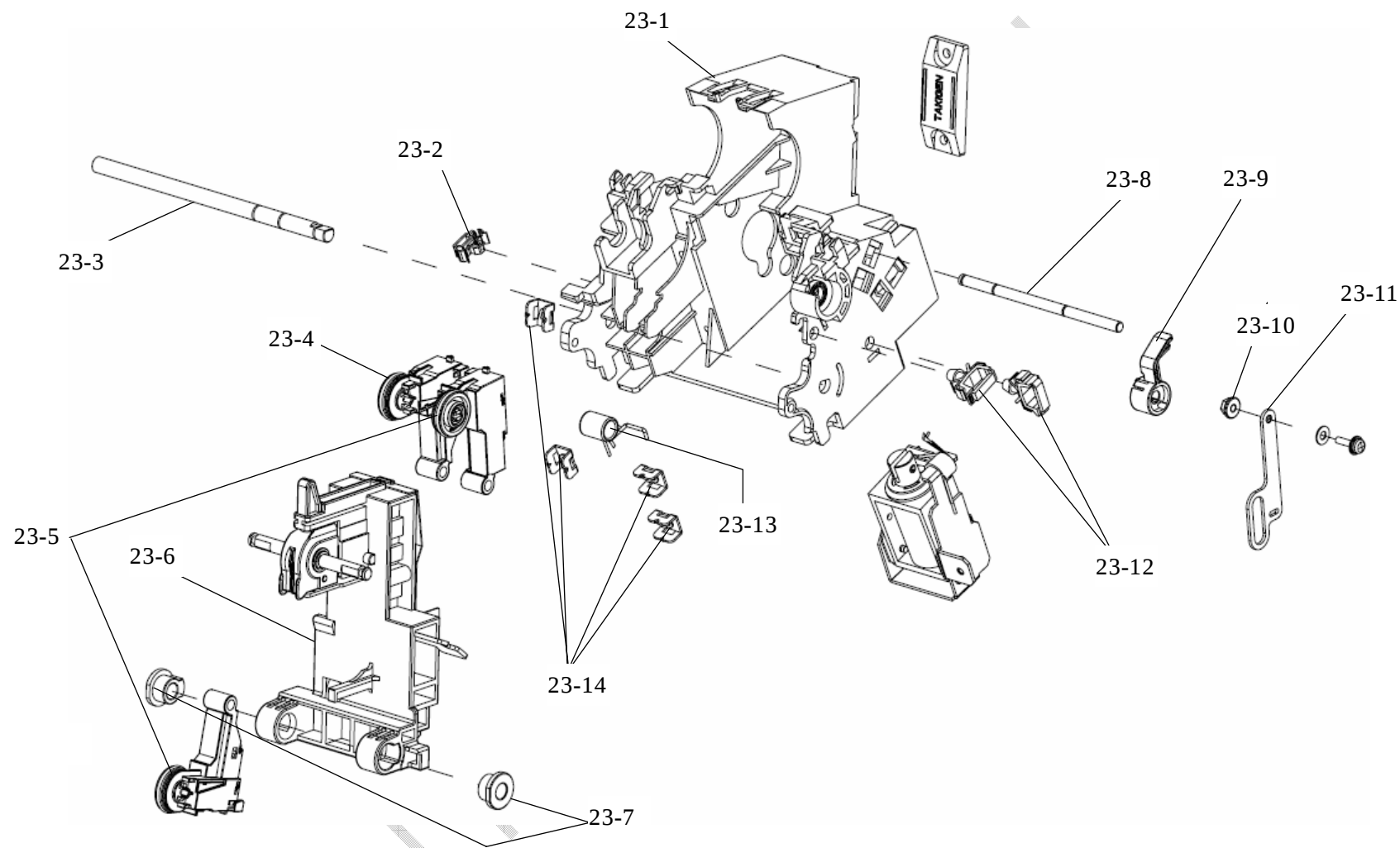
FIGURE 23. PIC-POLLER-ASSY (-E355)
