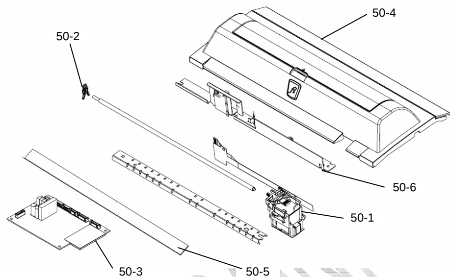
FIGURE 50 IMPRINTER (Option), fi-680PRB (-D203,-D204)
