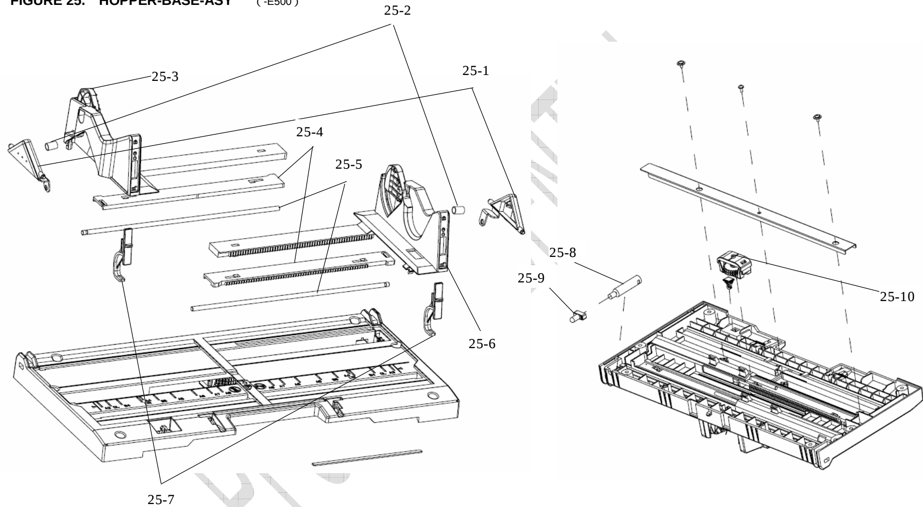
FIGURE 25. HOPPER-BASE-ASY (-E500)
