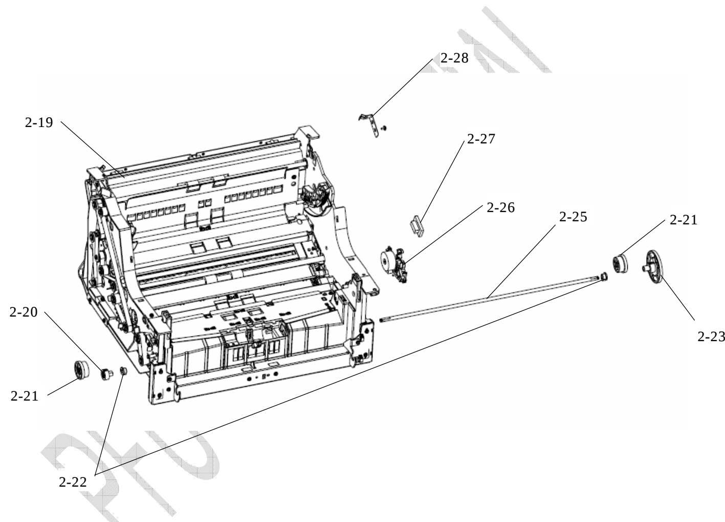
FIGURE 2. FIXED-UNIT 2/3 (-D00X)
