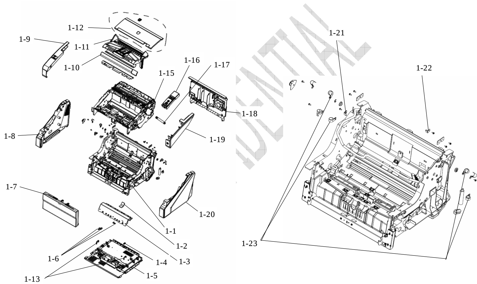
FIGURE 1. SCANNER-UNIT (-C00X)
