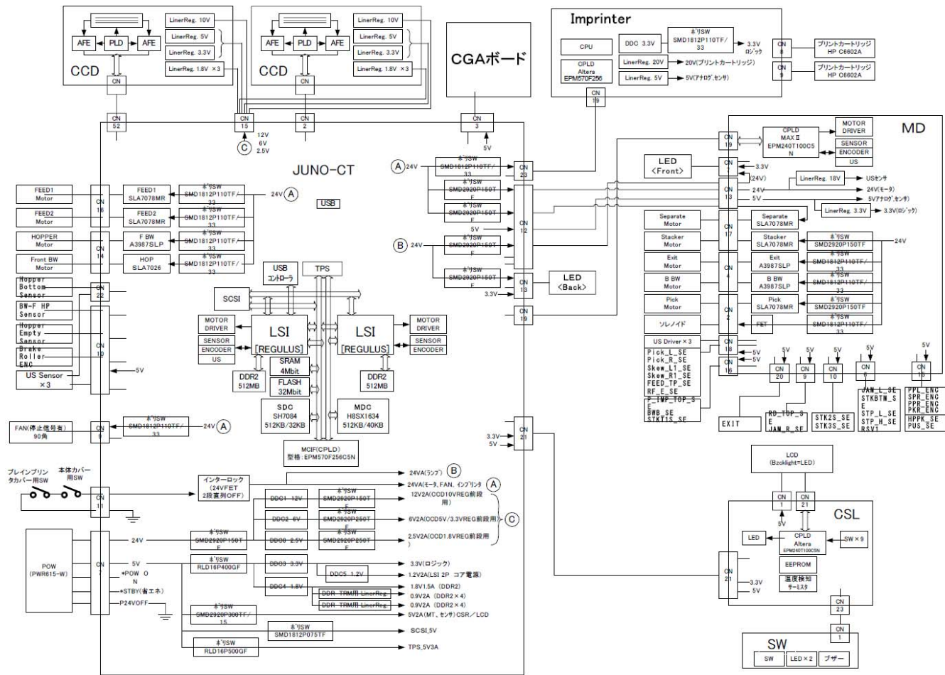
FIGURE 45. CIRCUIT BLOCK DIAGRAM
