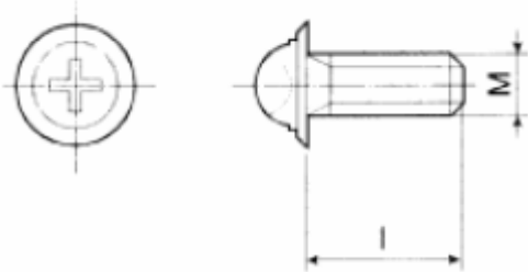
FIGURE B3 SCREW
