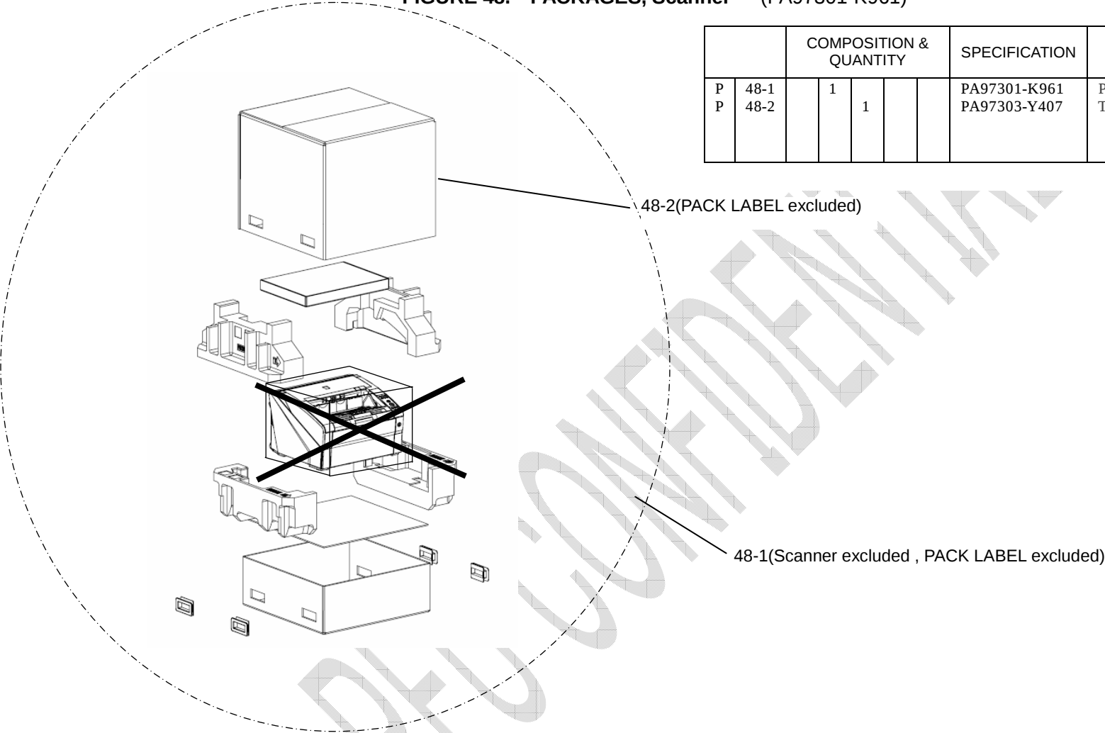
FIGURE 48. PACKAGES, Scanner (PA97301-K961)
