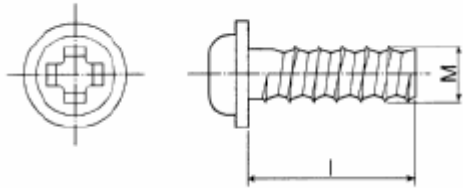
FIGURE B1 PT SCREW
