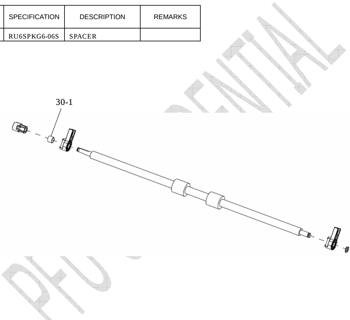
FIGURE 30. ASSIST-ROLLER (-D951)
