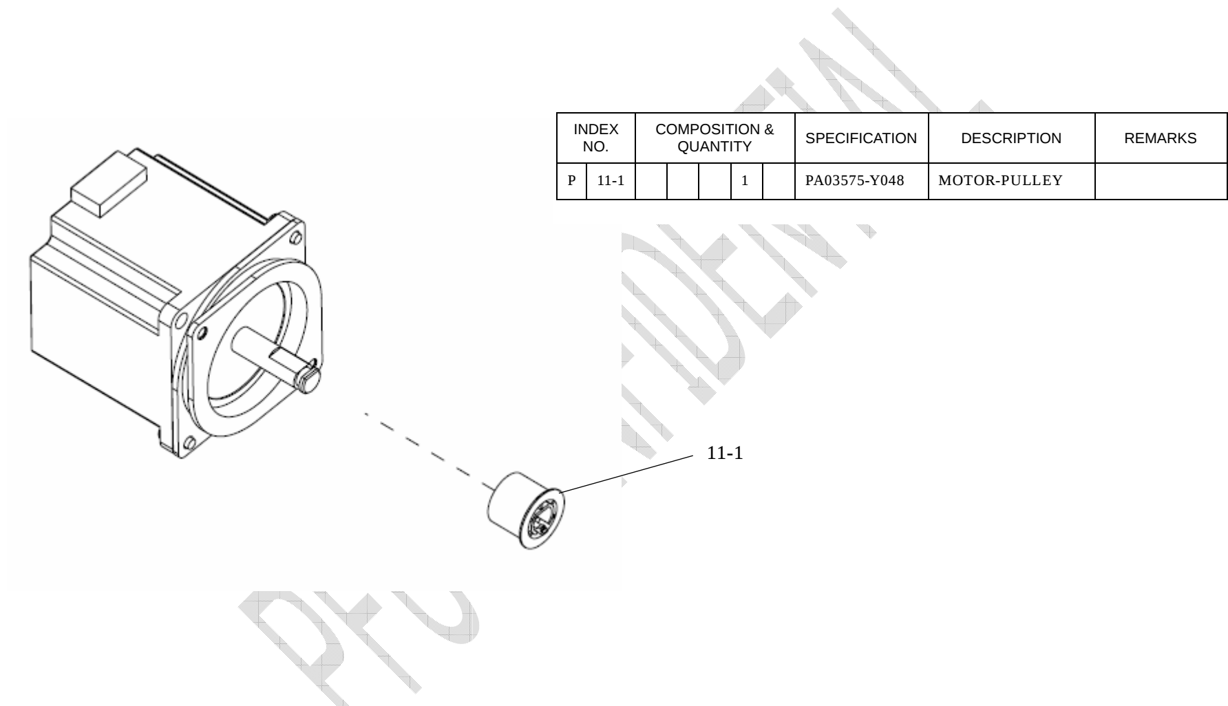
FIGURE 11. FEED-MOT-UNIT2 (-D961)
