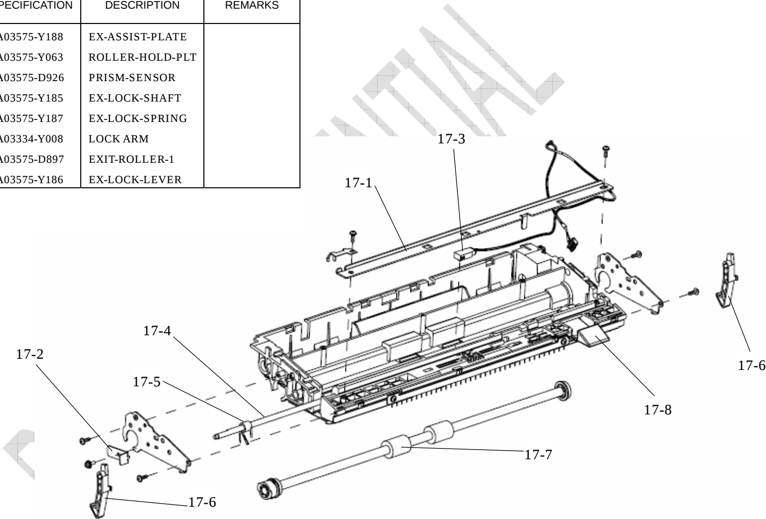
FIGURE 17. EXIT-TOP-UNIT 1/2 (-E180)
