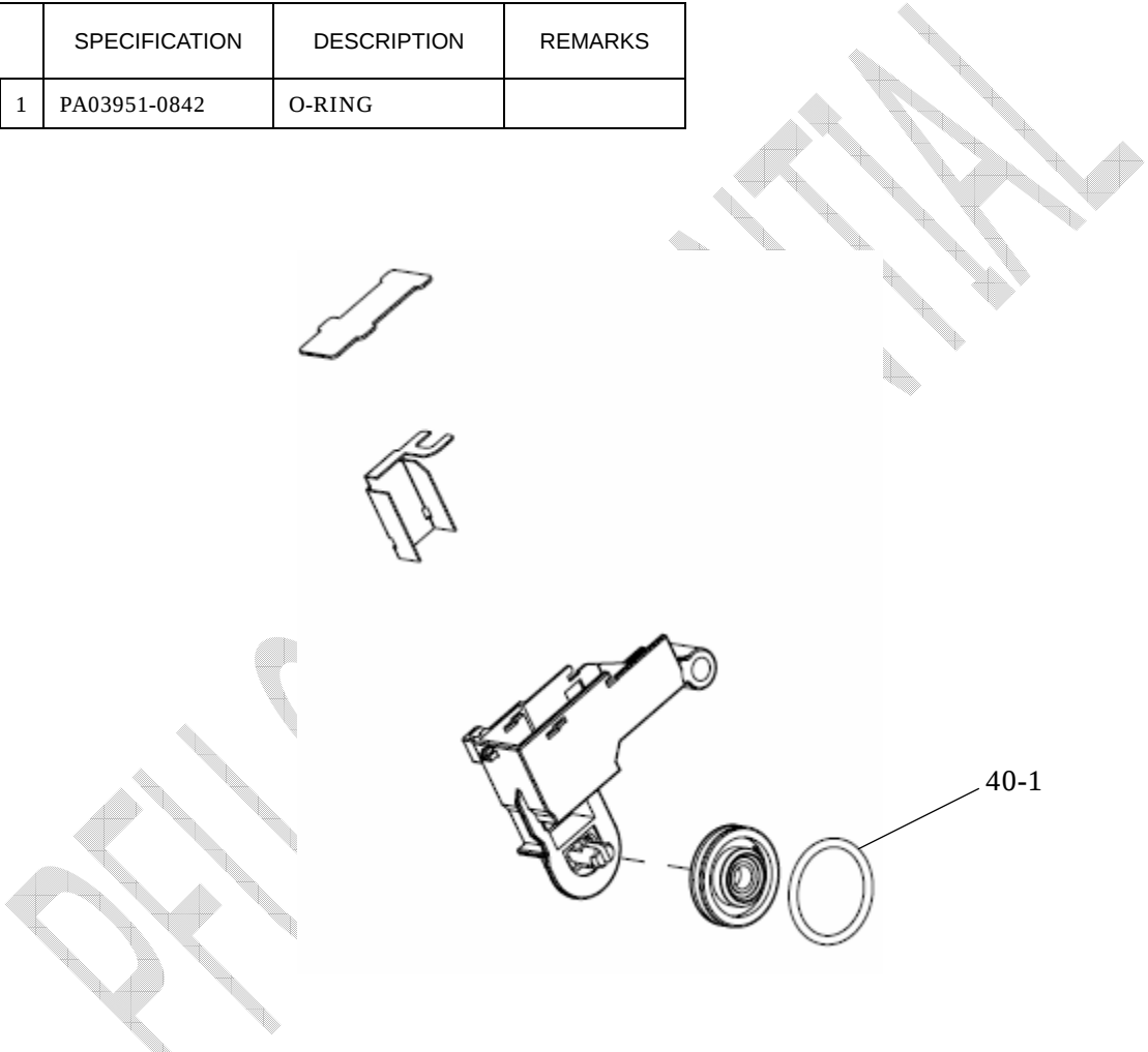
FIGURE 40. PIC-ENC-ARM-R (-F354)
