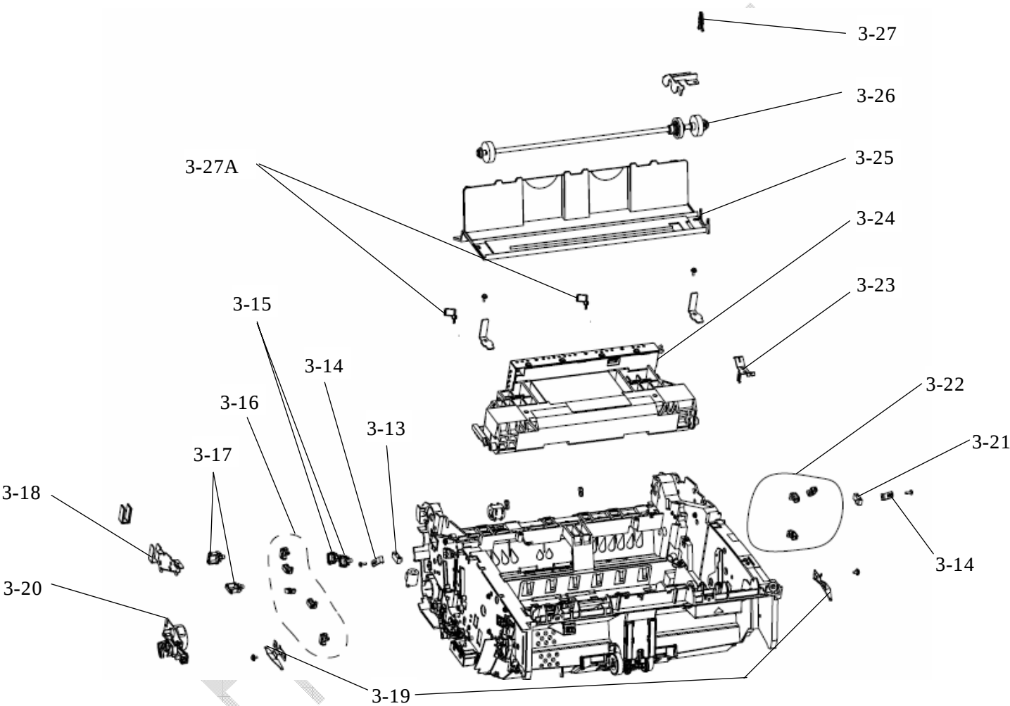
FIGURE 3. RV-UNIT 2/5 (-D10 x)
