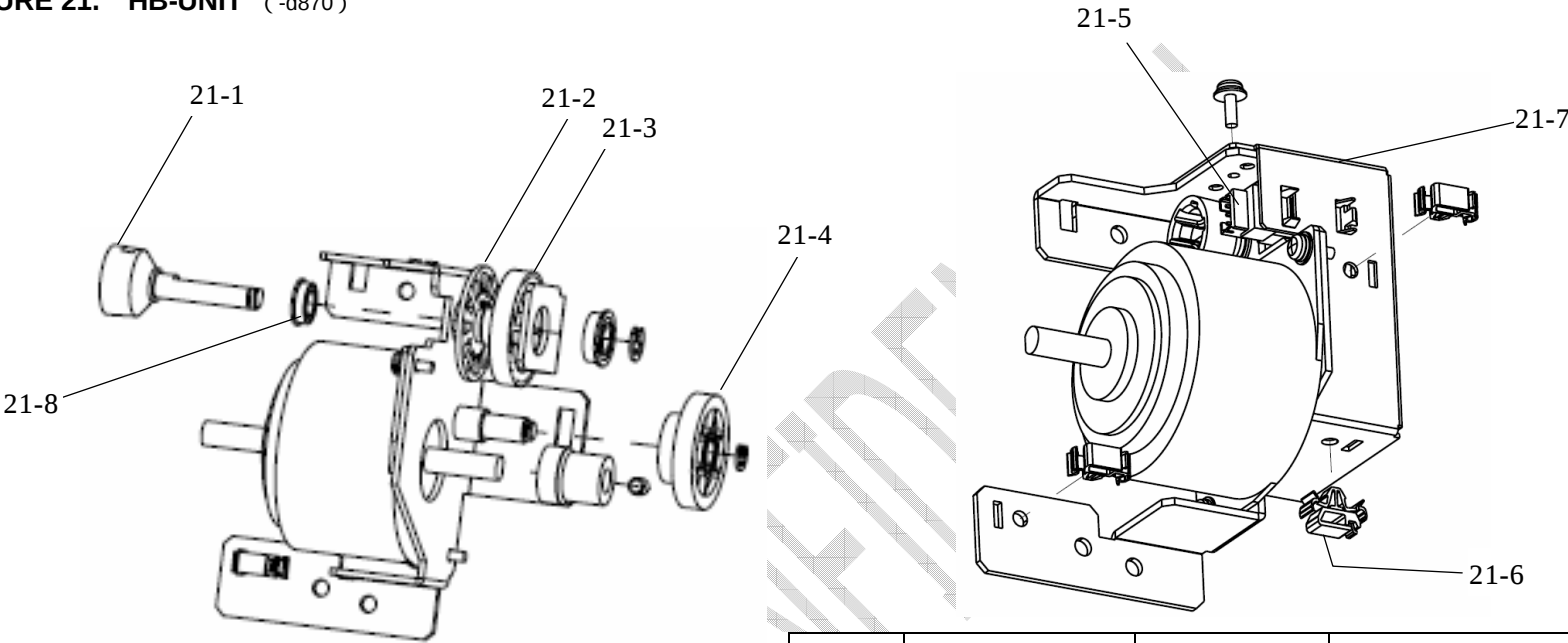
FIGURE 21. HB-UNIT (-d870)
