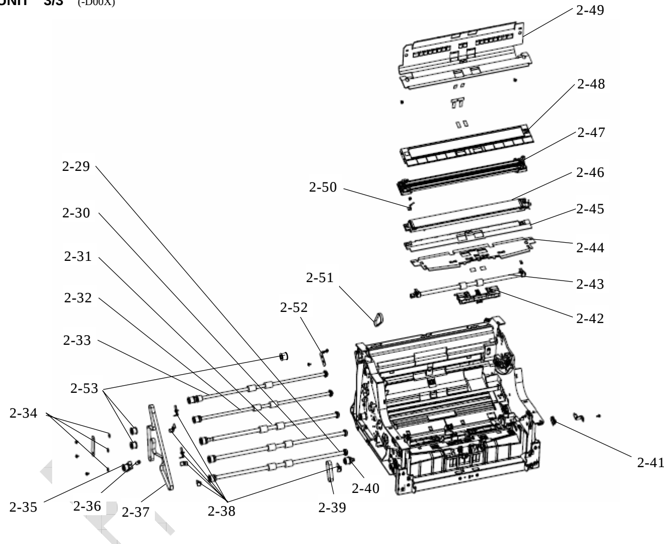
FIGURE 2. FIXED-UNIT 3/3 (-D00X)
