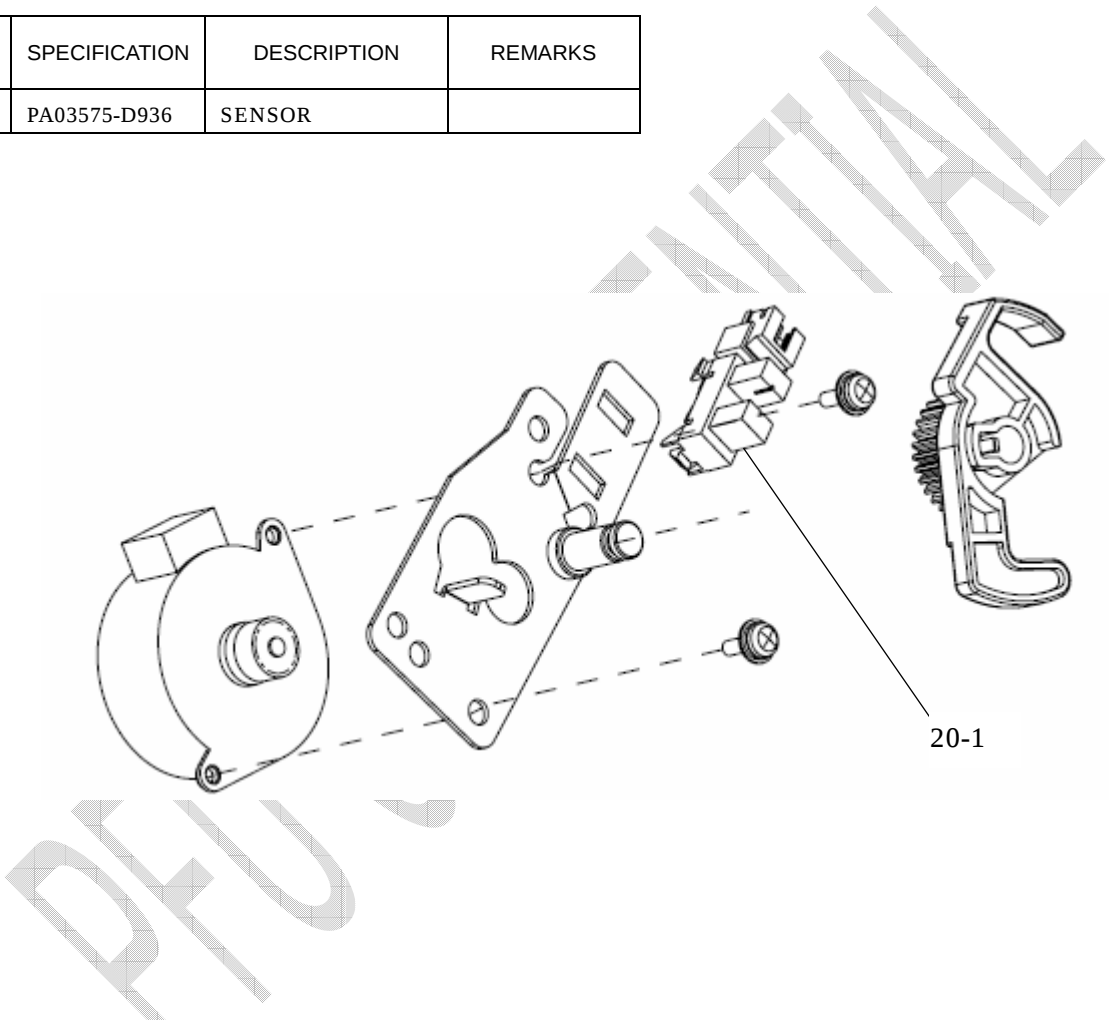
FIGURE 20. BW-MOTER-UNIT (-D962)
