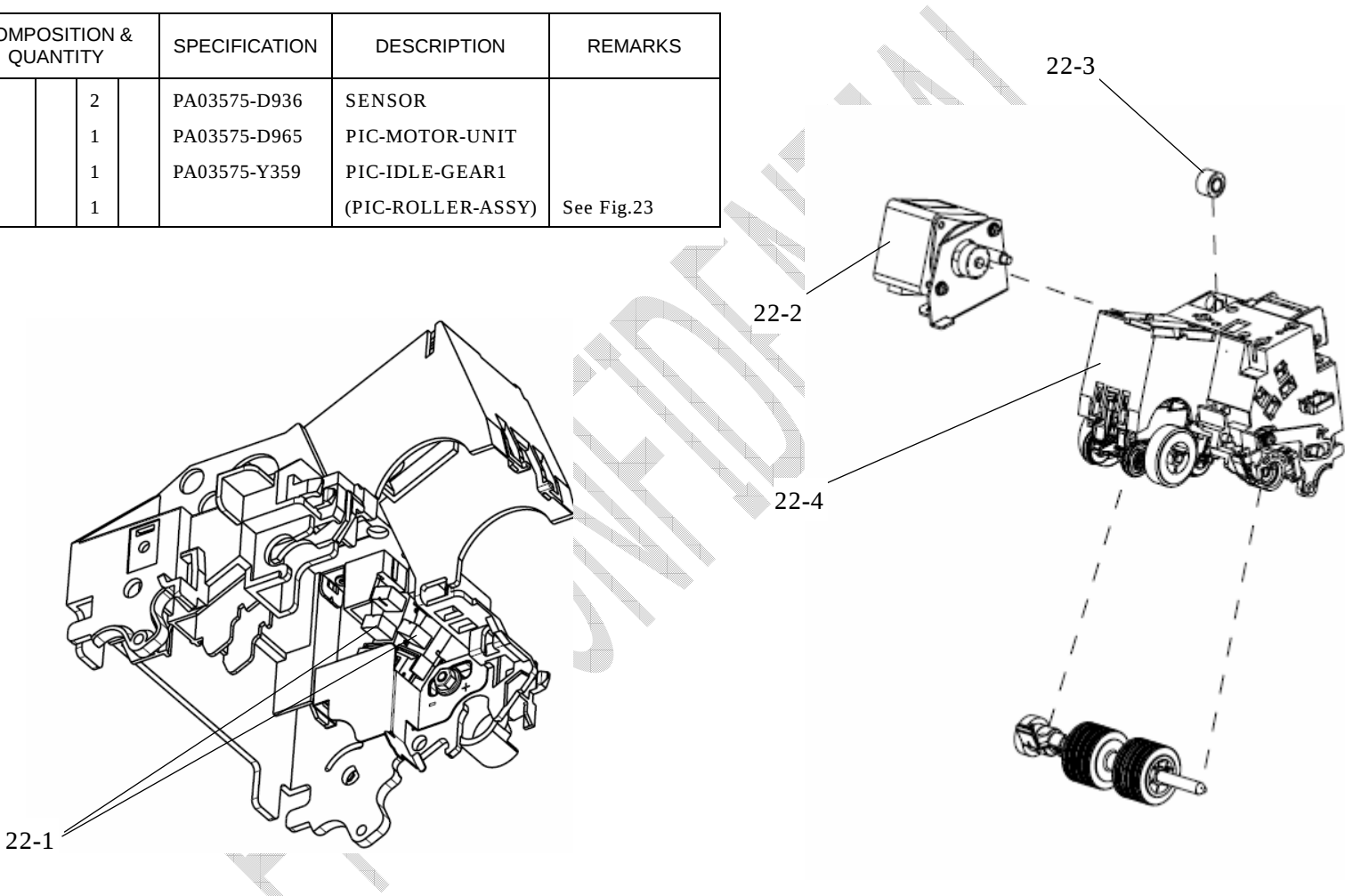
FIGURE 22. PIC-POLLER-UNIT 1/2 (-E350)
