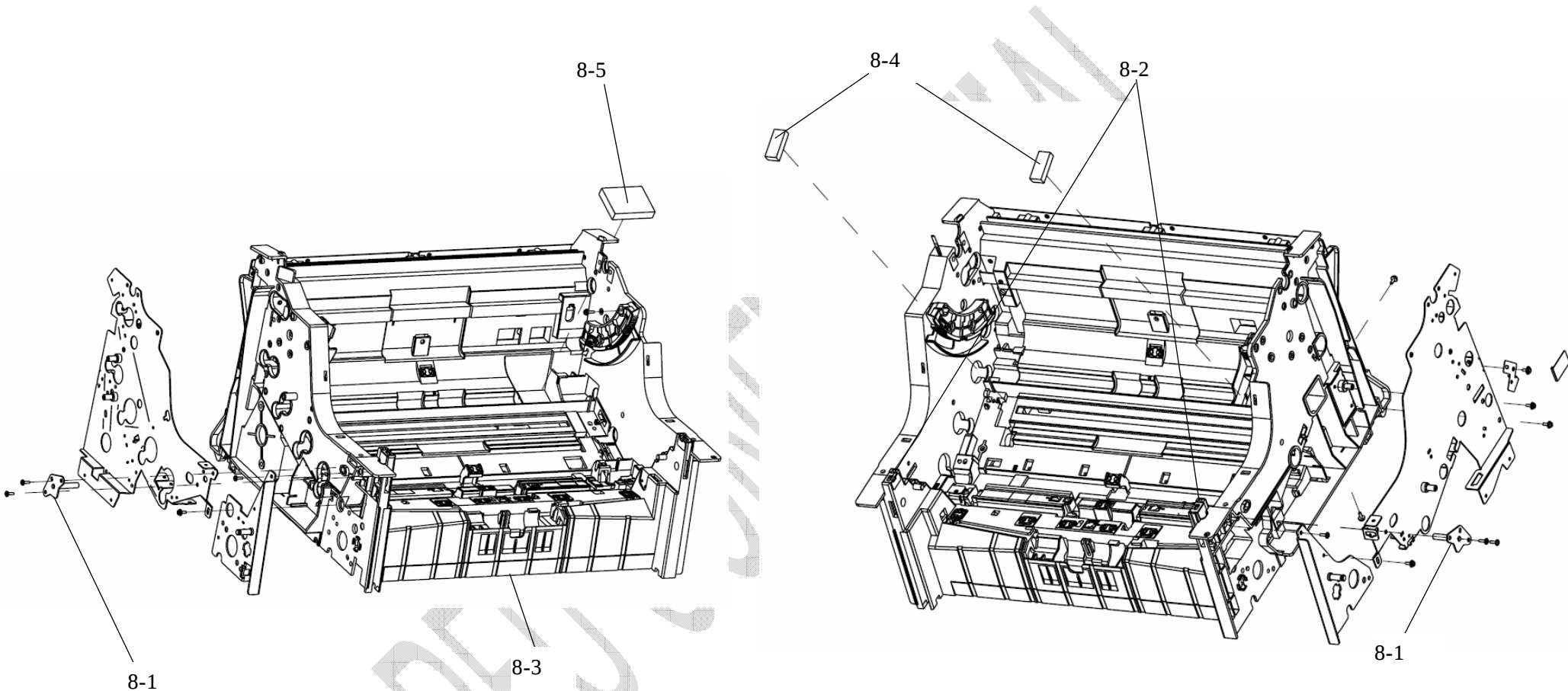
FIGURE 8. FIX-ASSY 1/2 (-E001)
