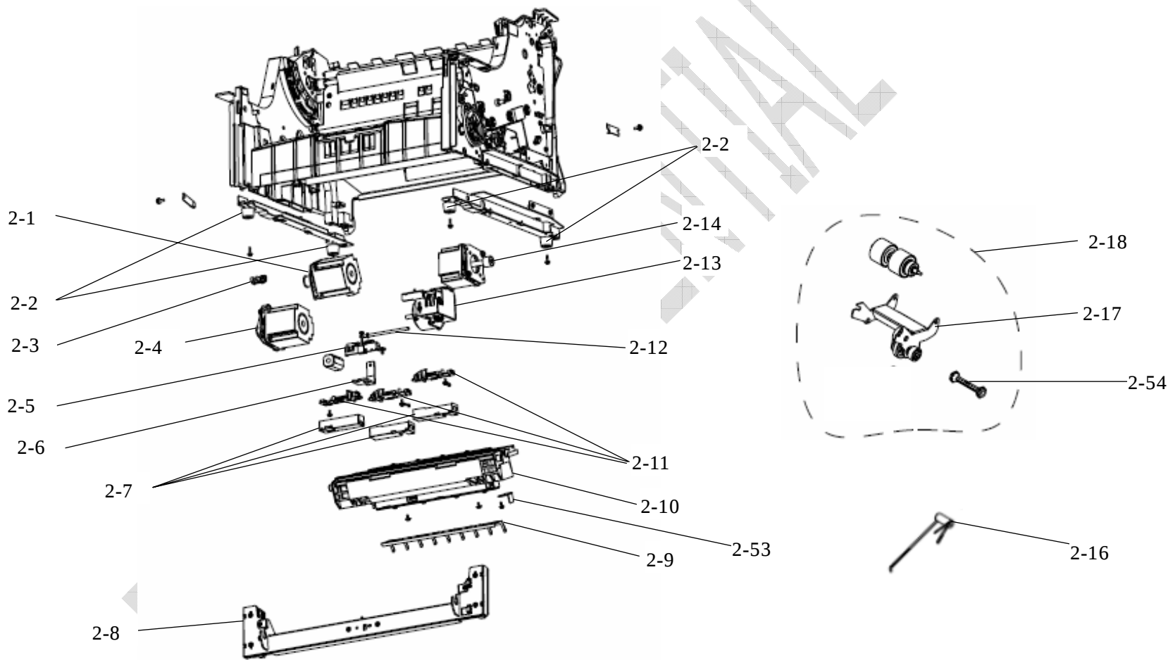
FIGURE 2. FIXED-UNIT 1/3 (-D00X)
