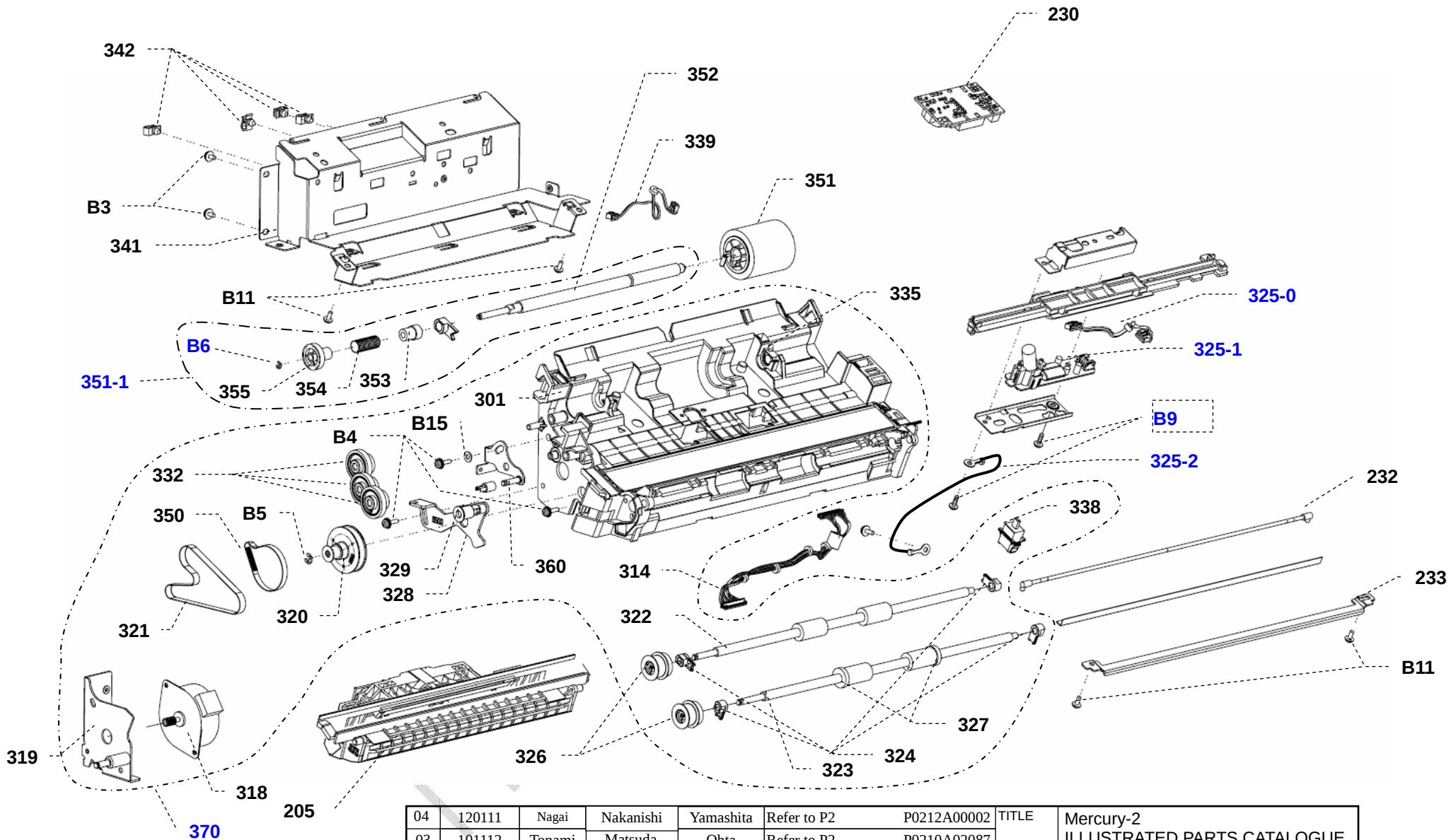
FIGURE 3. FIXED UNIT
