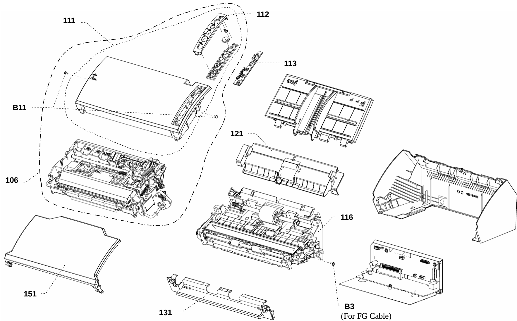
FIGURE 1. FINAL ASSEMBLY
