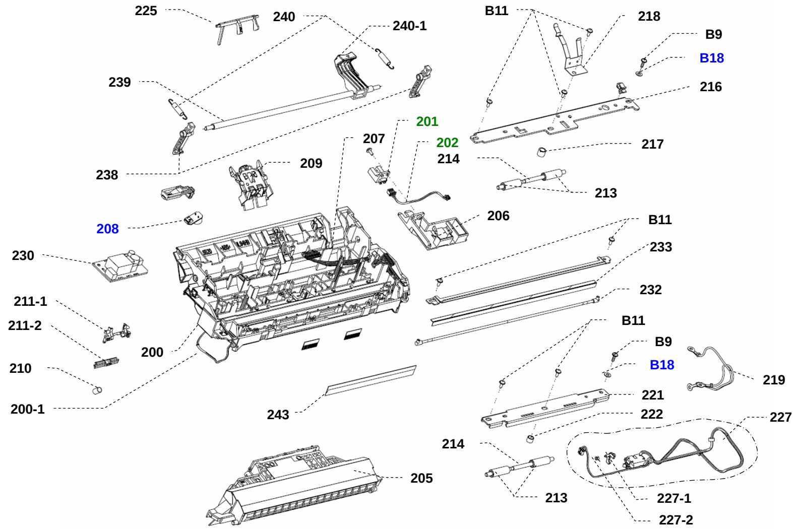
FIGURE 2. REVOLVE UNIT
