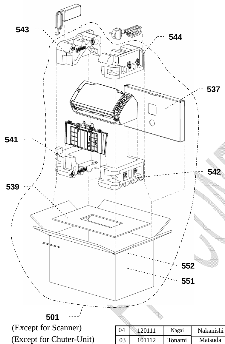
FIGURE 5-1. PACKAGING BOX for Scanner
