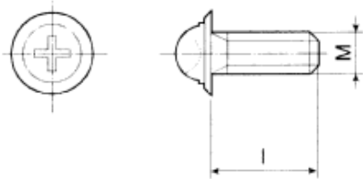
FIGURE B.1 SCREW
