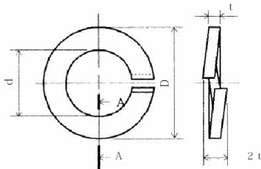
FIGURE B.6 WASHER
