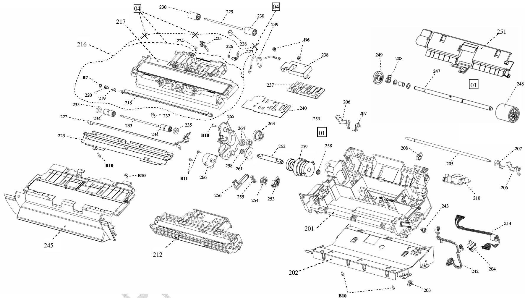
FIGURE 10. BASE UNIT
