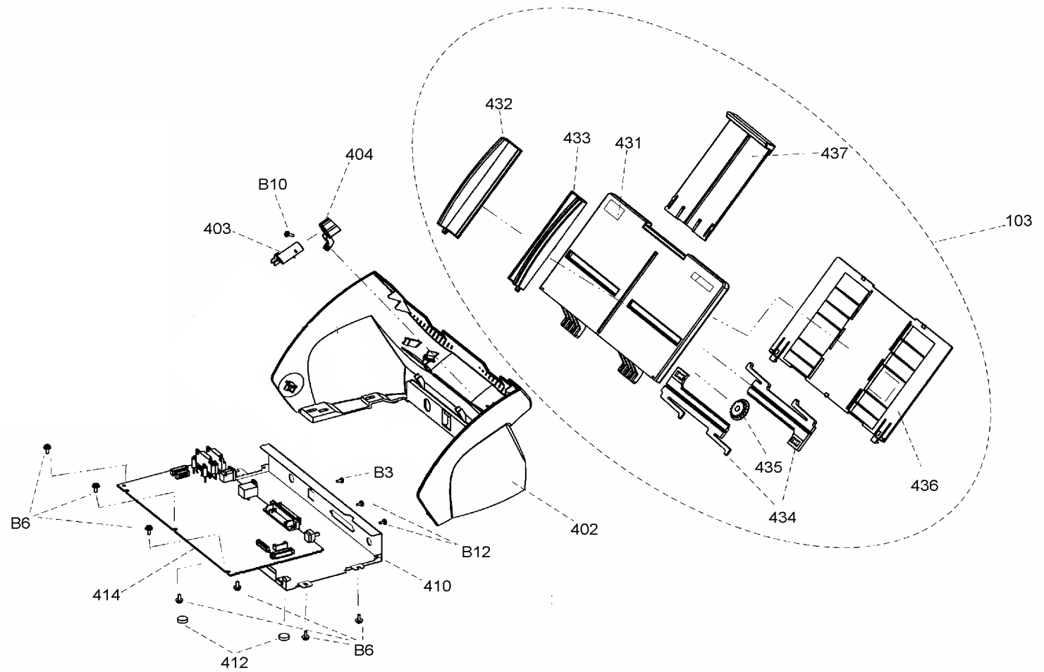
FIGURE 12. PCB UNIT, RER COVER and CHUTE UNIT
