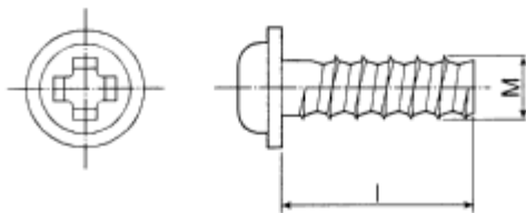
FIGURE B4 PT SCREW
