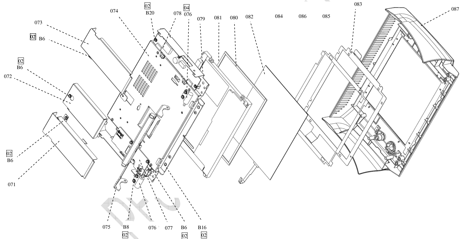
FIGURE 7. LCD UNIT
