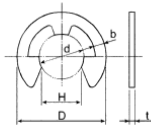
FIGURE B3 RETAINING RING (E-RING)
