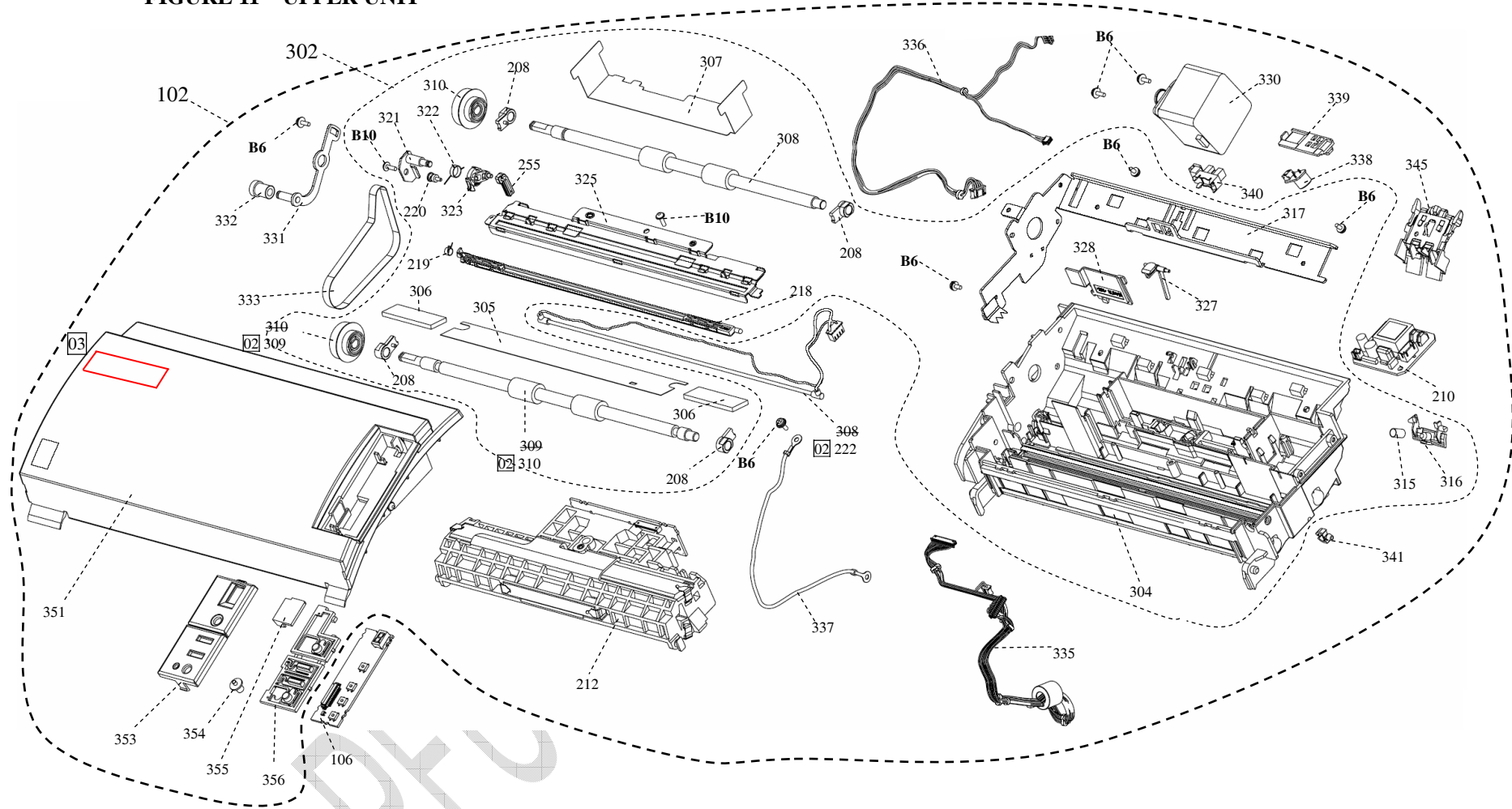
FIGURE 11 UPPER UNIT
