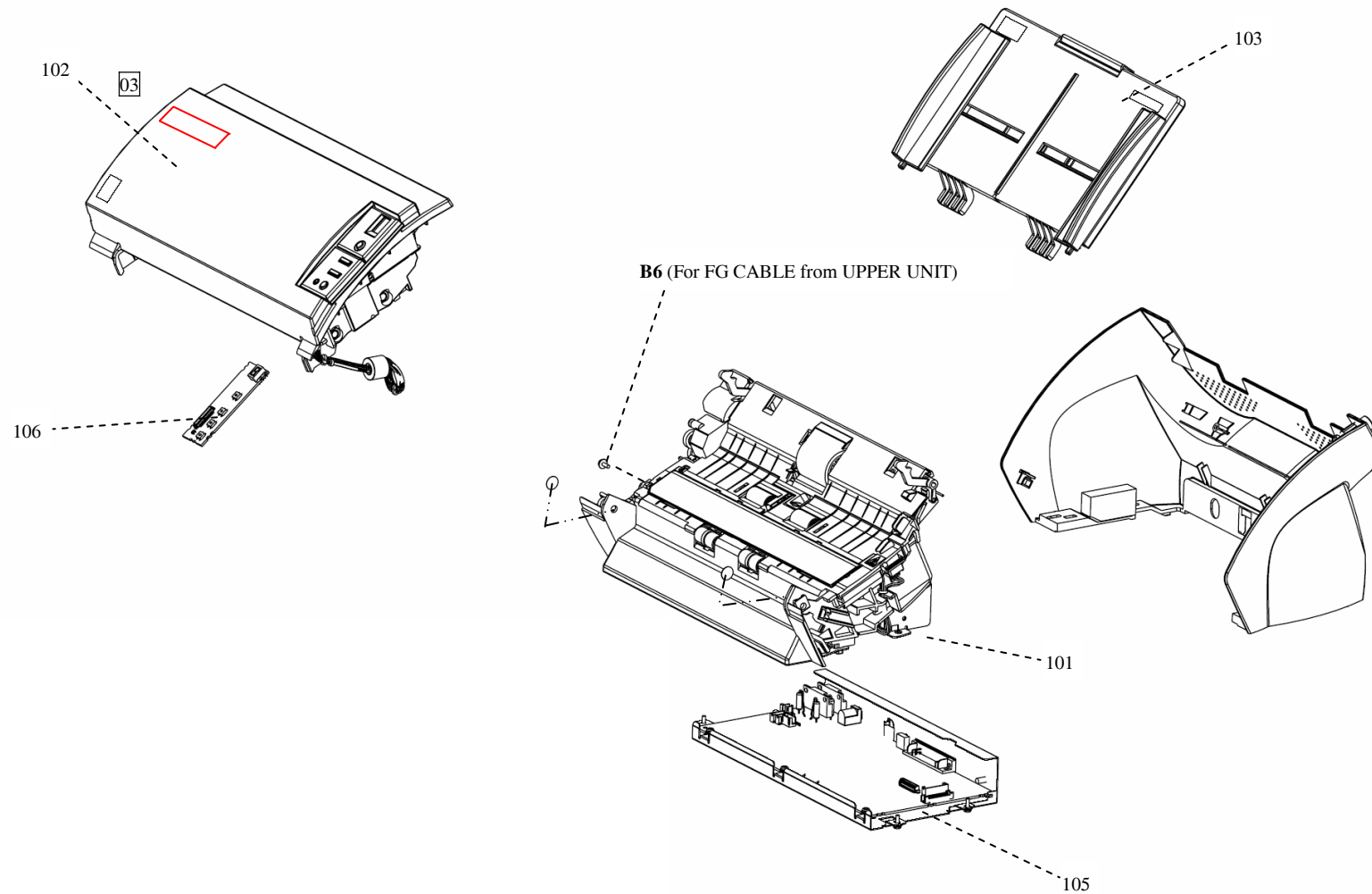
FIGURE 9. SCANNER UNIT
