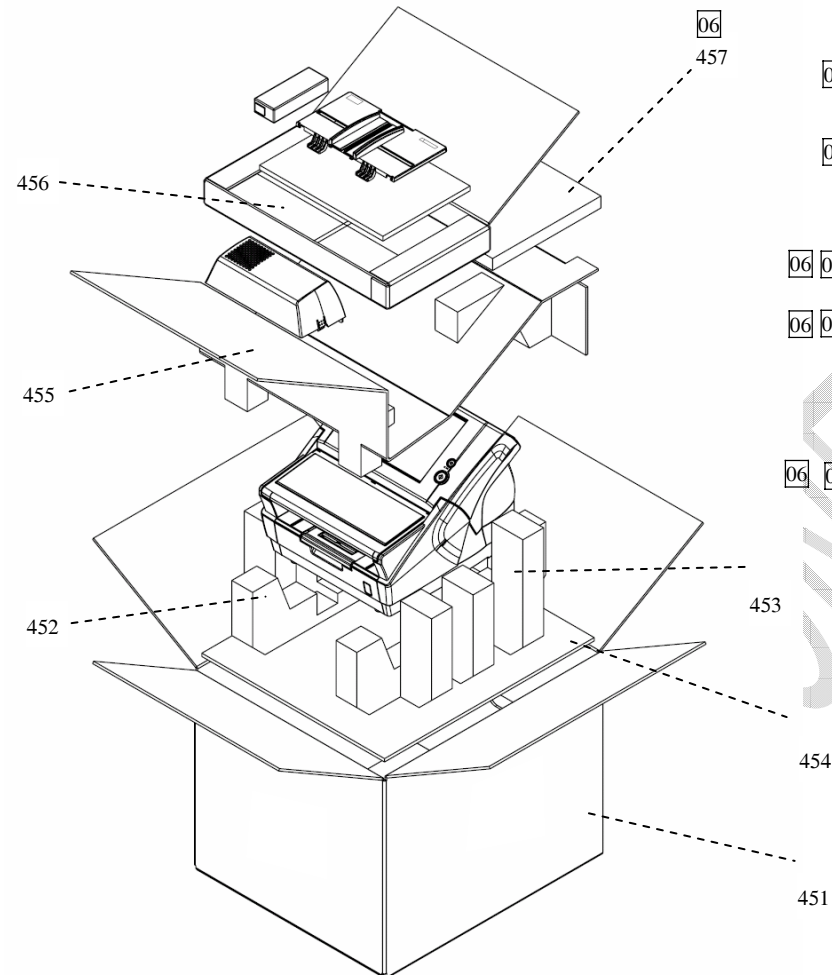
FIGURE 13. PACKAGE
