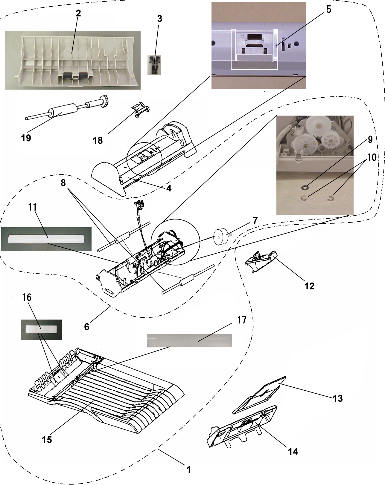
FIGURE 1 ADF UNIT
