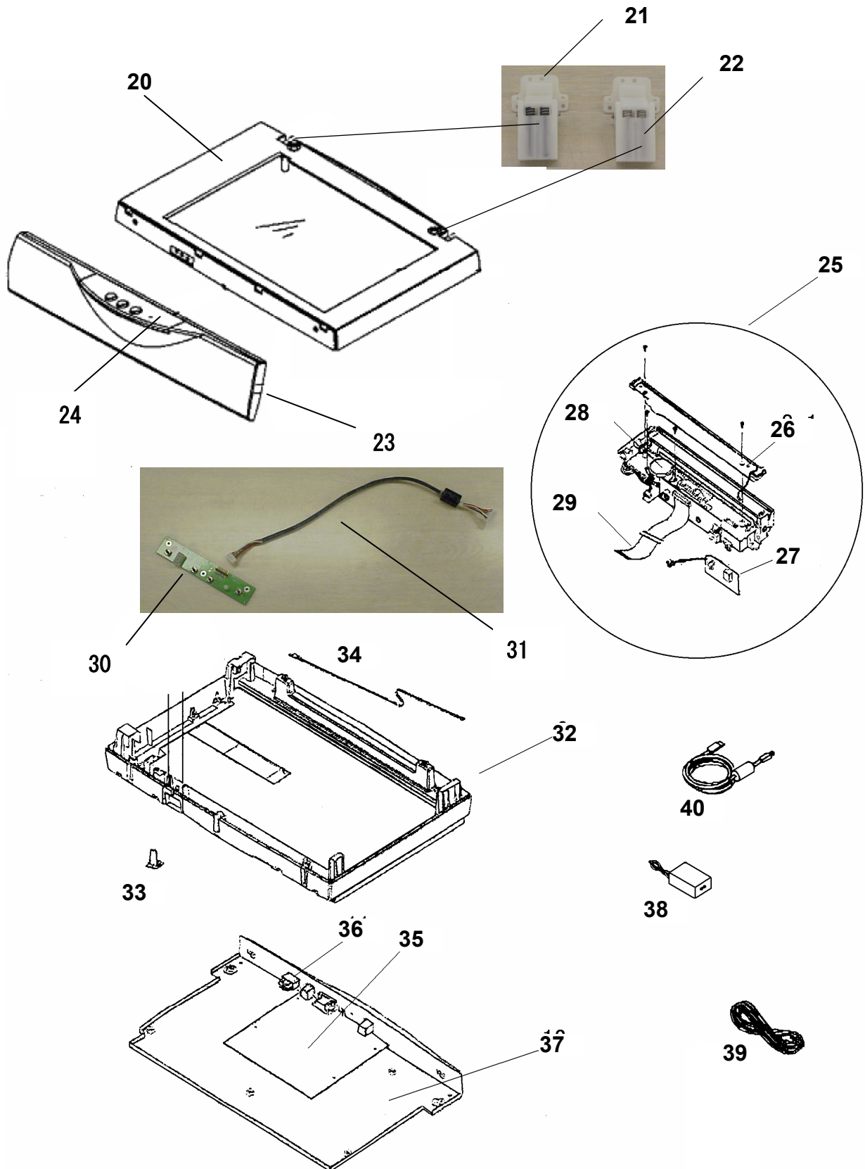
FIGURE 2 FLATBED
