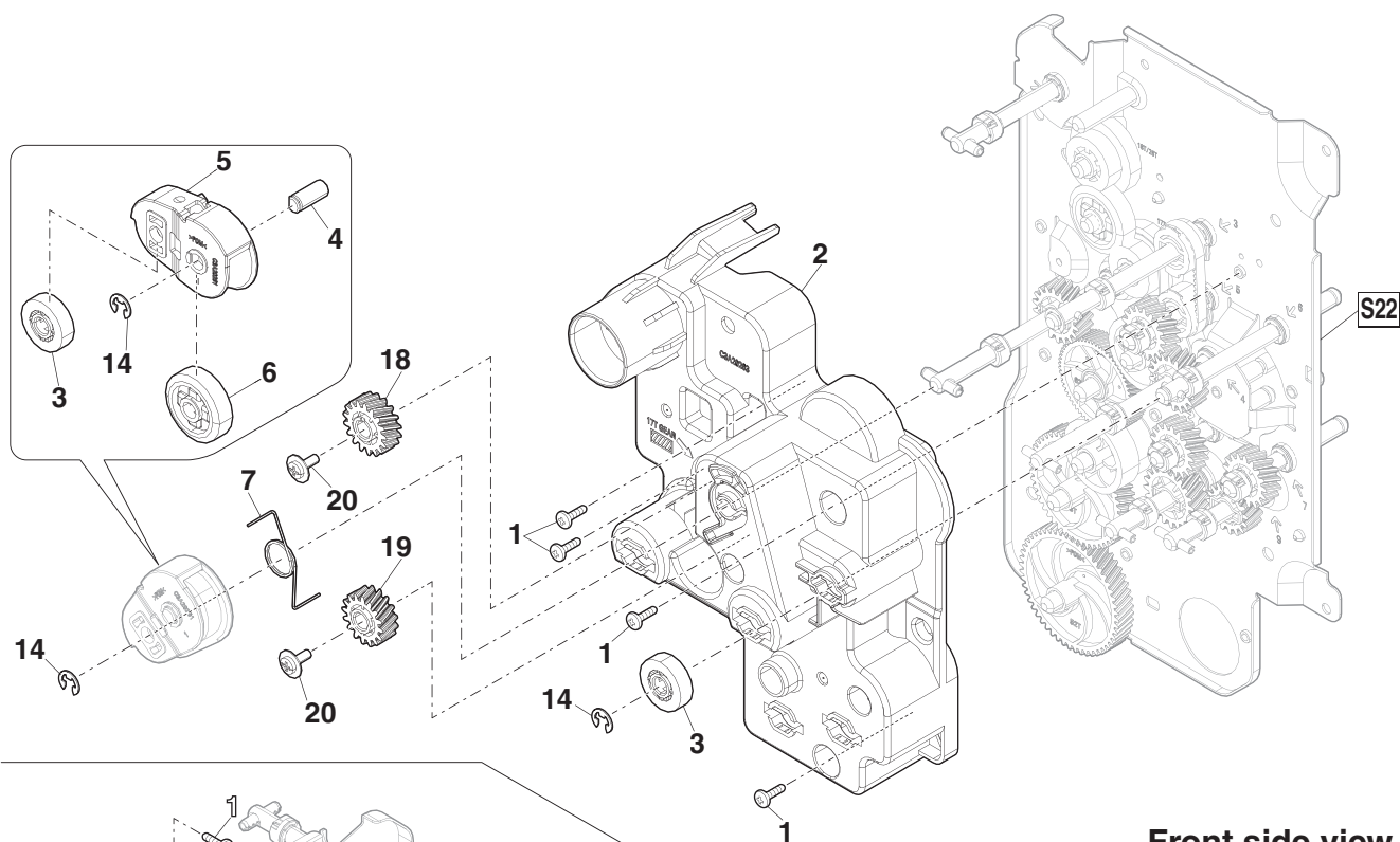
Front side view
