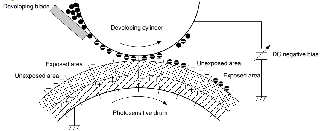
Figure 5-14 Development
