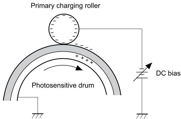
Figure 5-12 Primary charging
