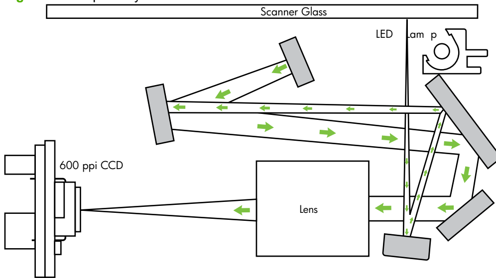
Figure 5-23 Optical system
