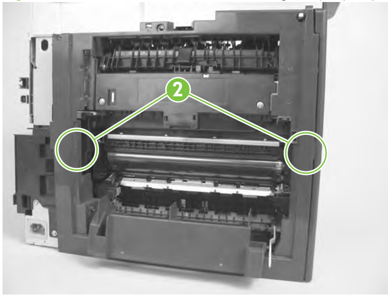
Figure 6-70 Remove the rear cover and feed guide (simplex product) (3 of 6)
