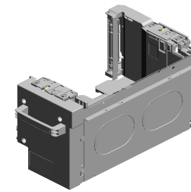
280.D2617599 (NA):TANDEM LCT:RIGHT:ASS'Y
