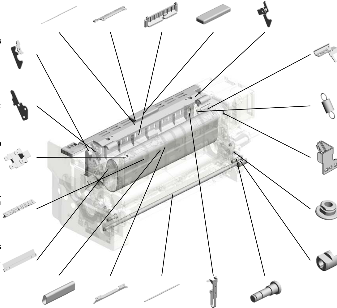
128.D1794197 FLAT BELT-FUSING G:DIA80:SEAL
