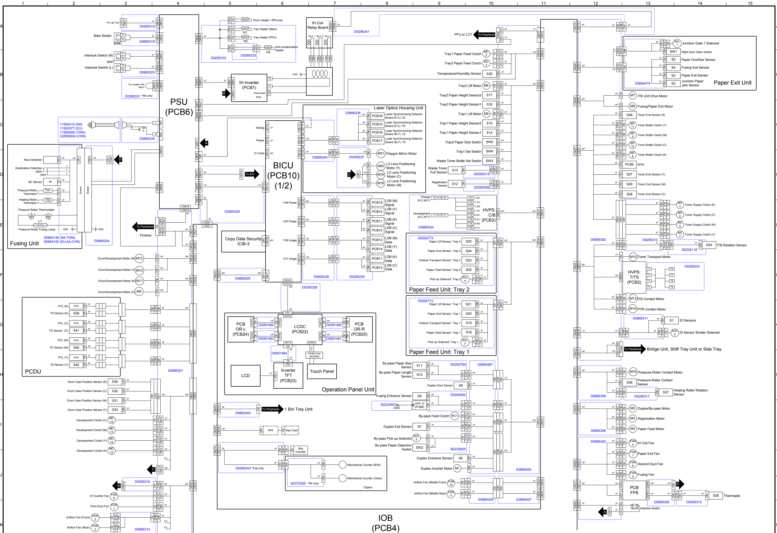
D088/D089 POINT TO POINT DIAGRAM (1/3)
