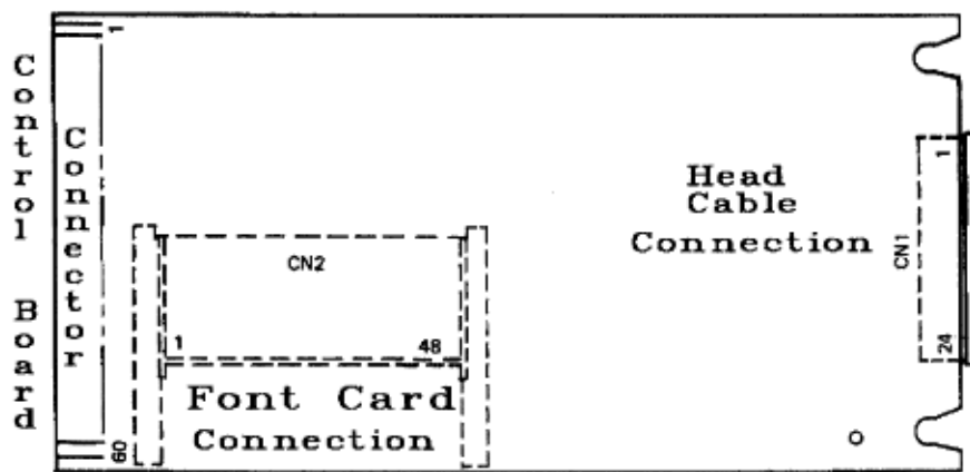
SRBS-PCB (connection board)
