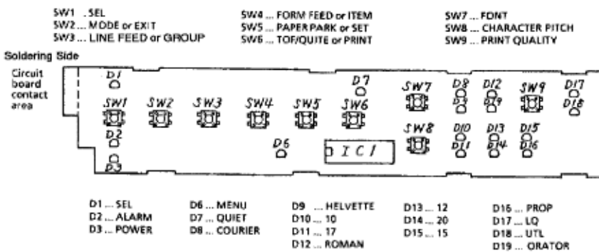
LXSP printed circuit board
