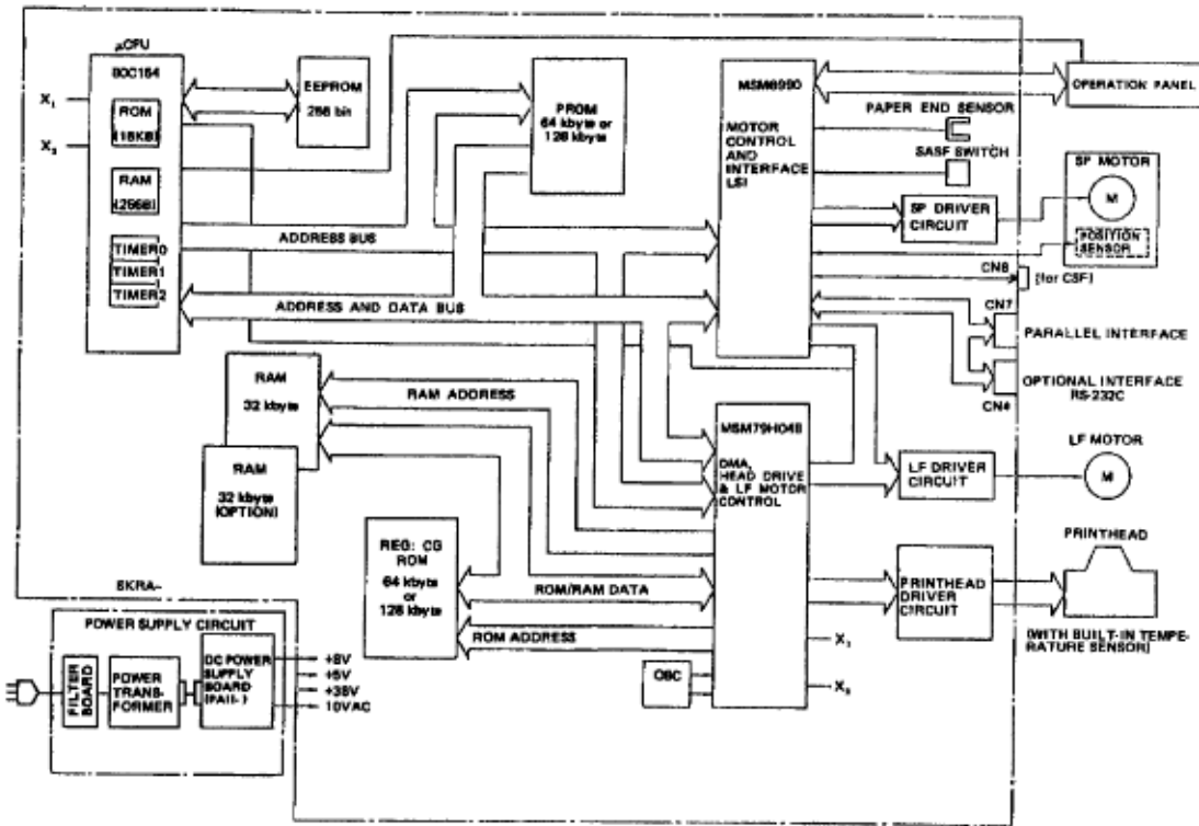
Block Diagram (Microline 390/391)
