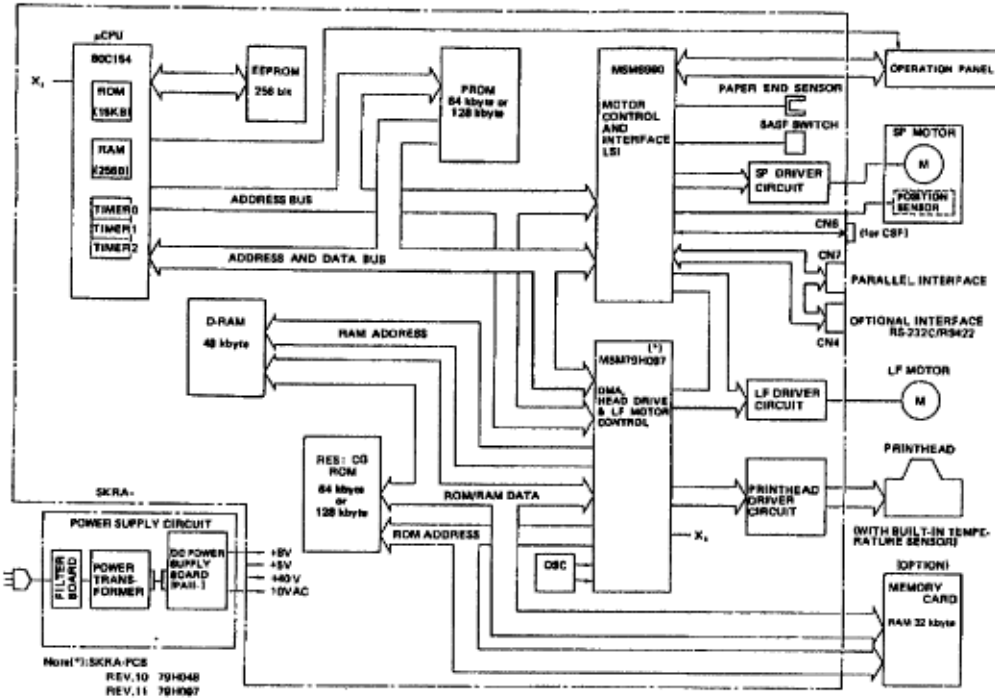
Block Diagram (Microline 390/391-Plus)
