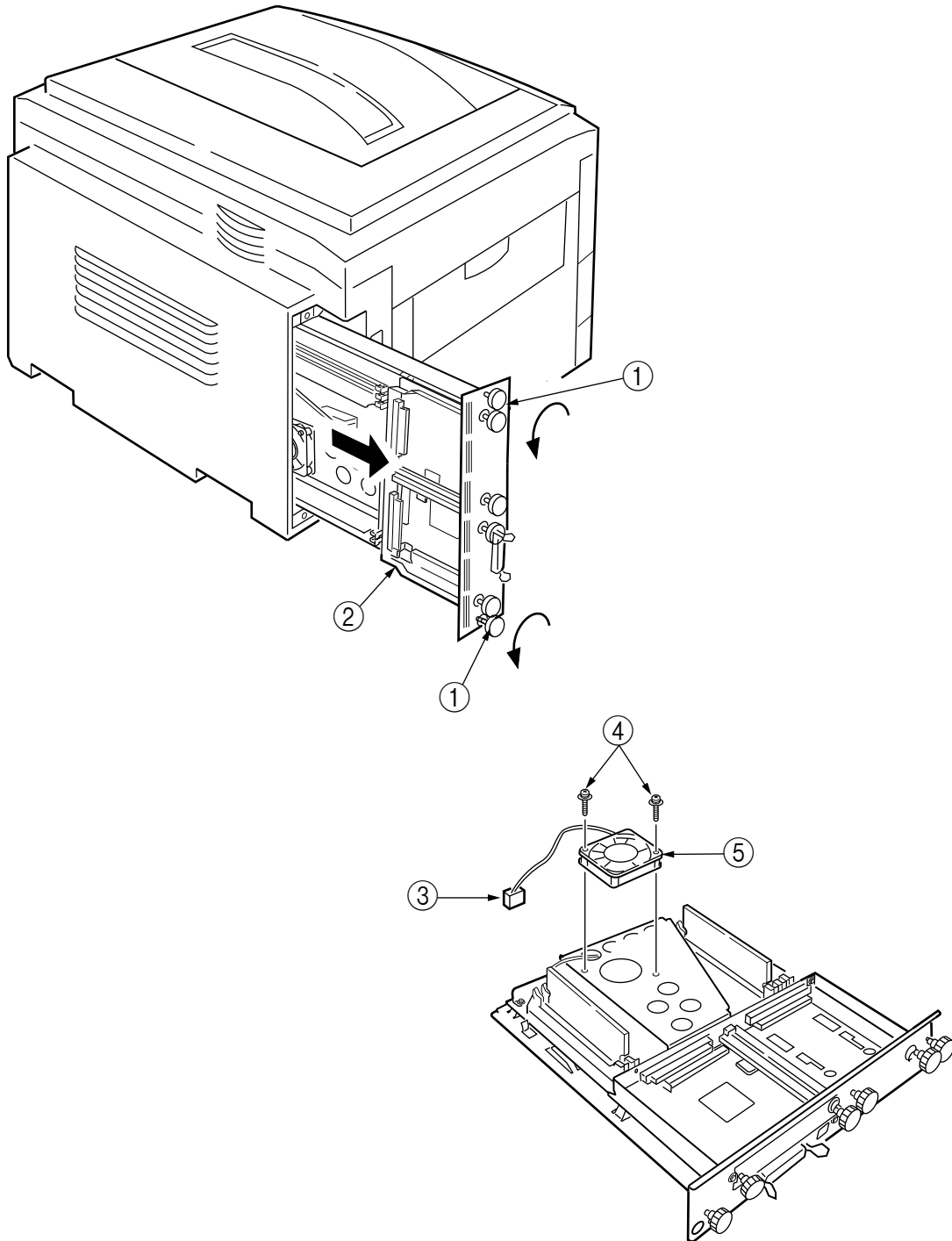
Figure 2-3-41 CU Assy (1/2)
