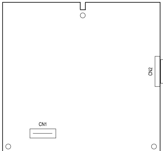
(12) Hight-Voltage PWB
