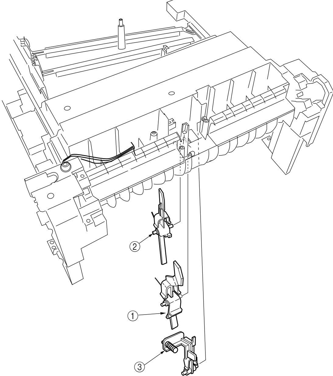
Figure 3-3-28 Entrance MT Sensor Actuator / Entrance Belt Sensor Actuator / Entrance Waste Chassis Sensor Actuator
