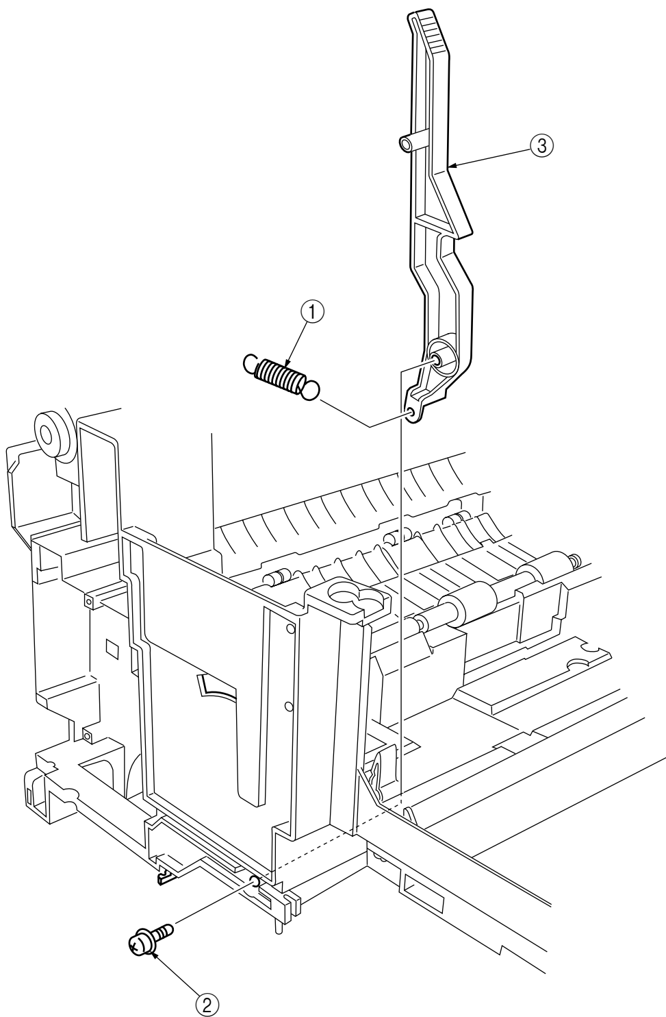
Figure 3-3-31 Fuser Latching Handle (L)
