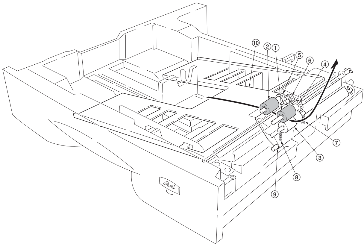
Figure 2-1-6 Paper cassette
