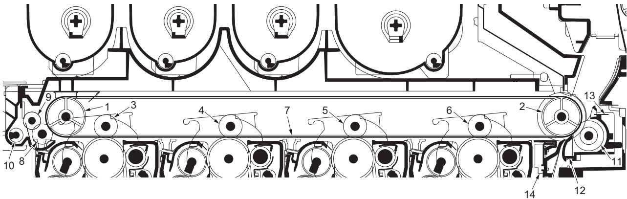
Figure 2-1-15 Transfer/separation section
