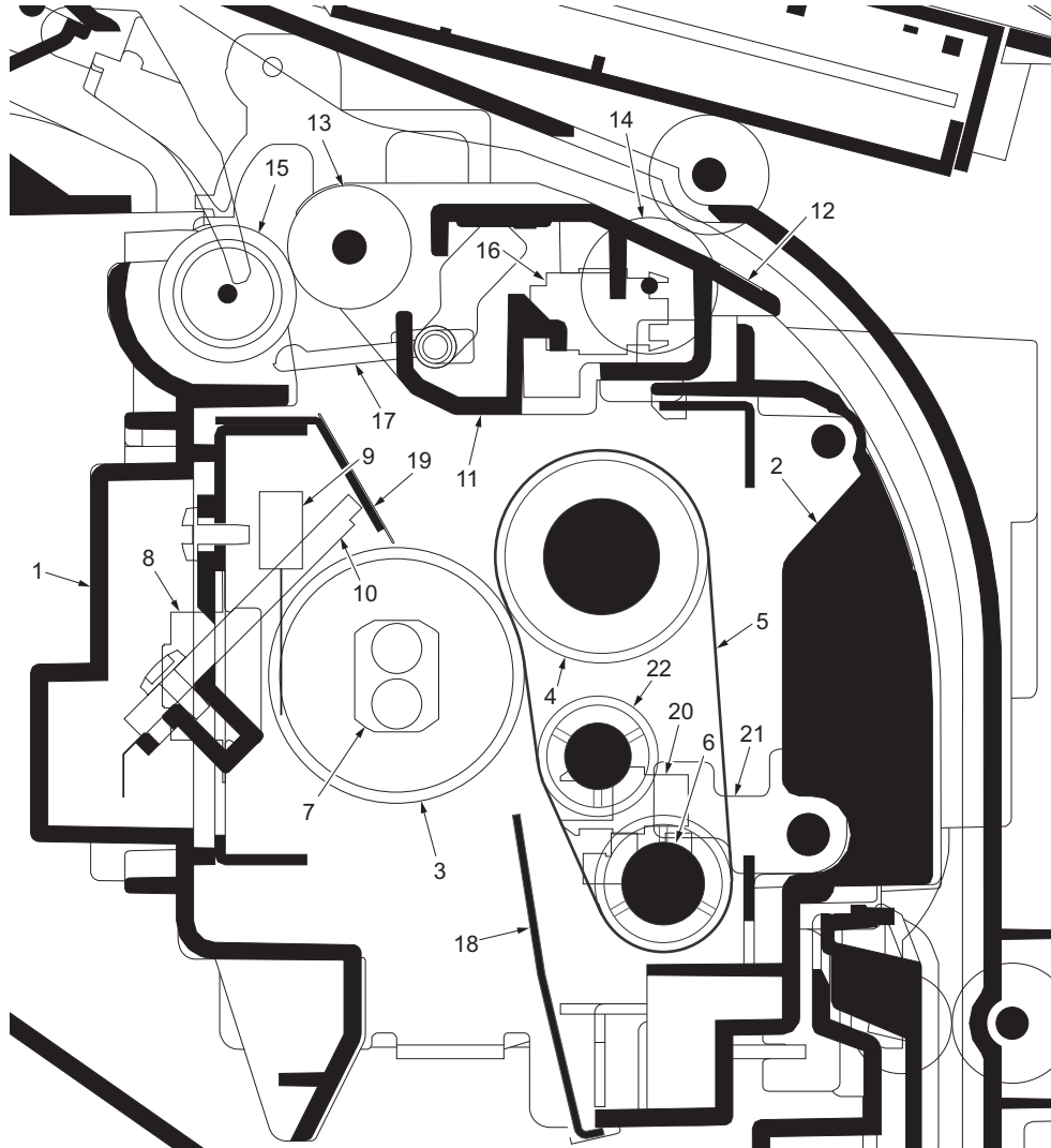
Figure 2-1-17 Fuser section
