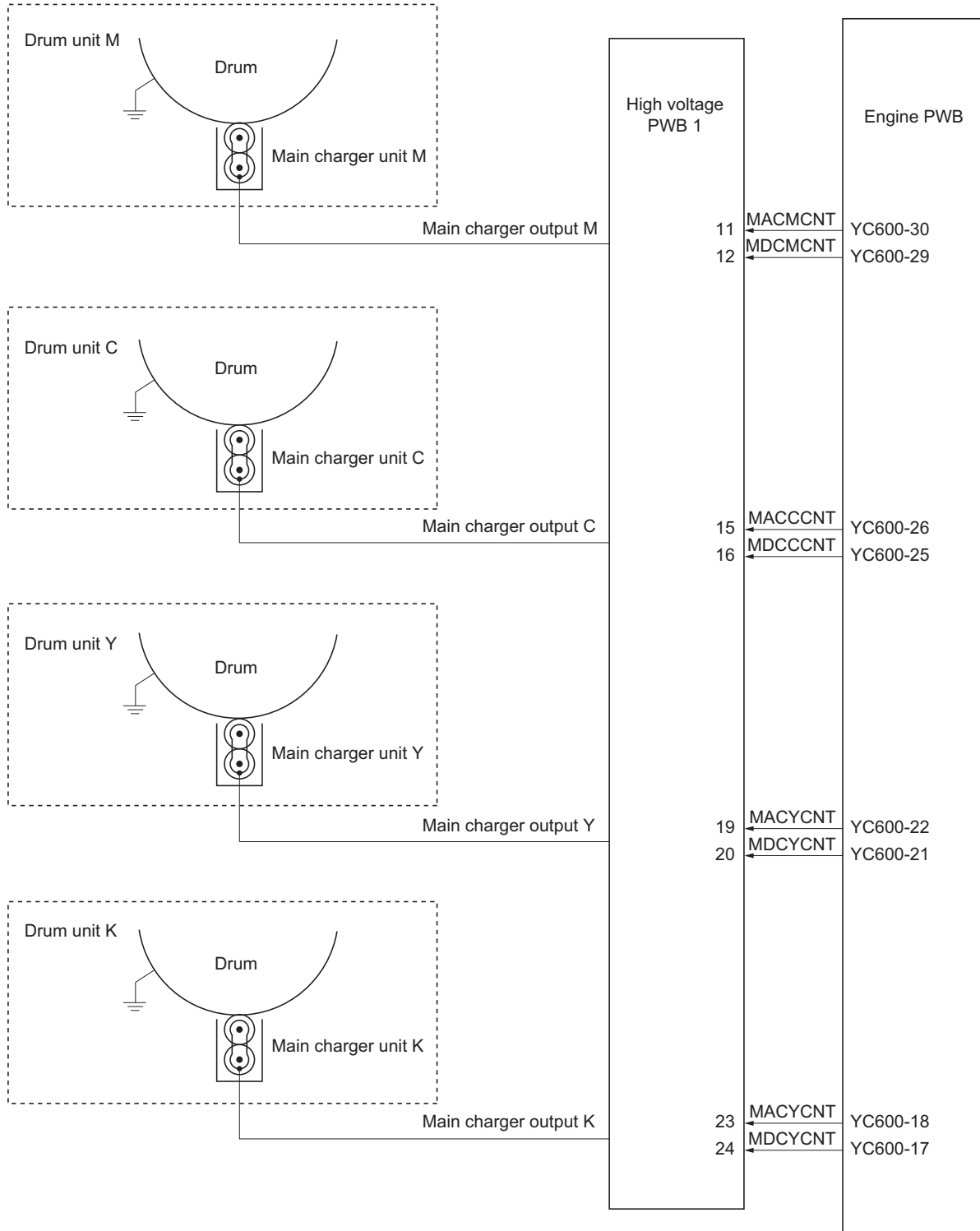
Figure 2-1-10 Main charger section block diagram
