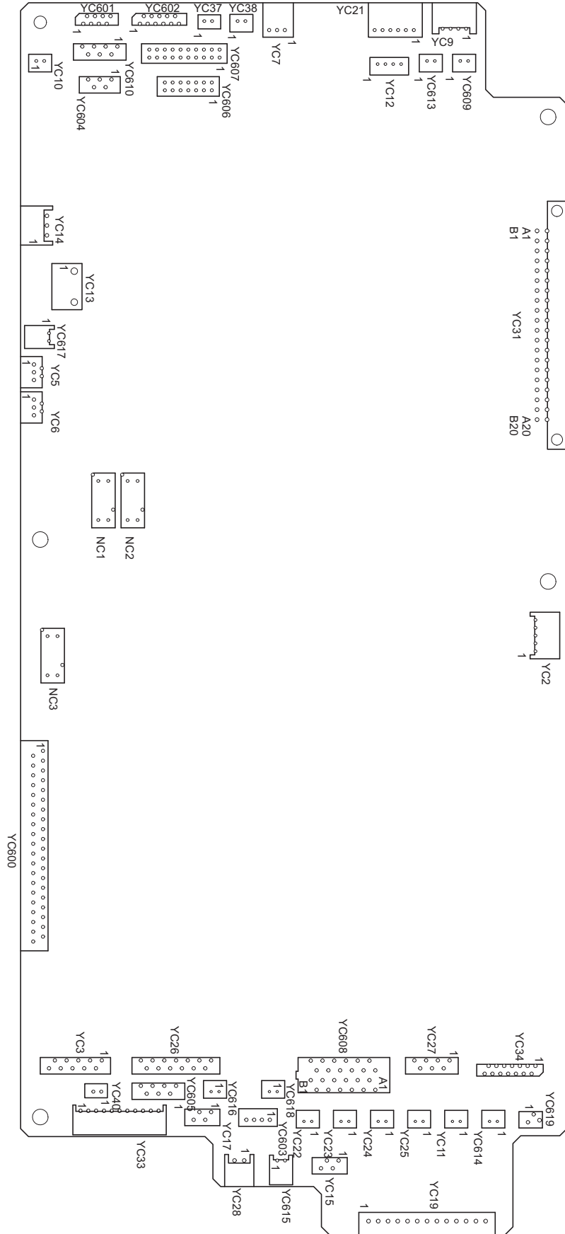
Figure 2-3-2 Engine PWB silk-screen diagram
