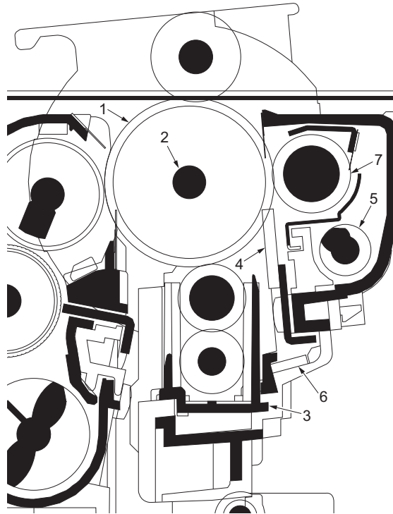
Figure 2-1-7 Drum section
