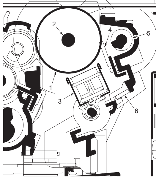
Figure 2-1-7 Drum section
