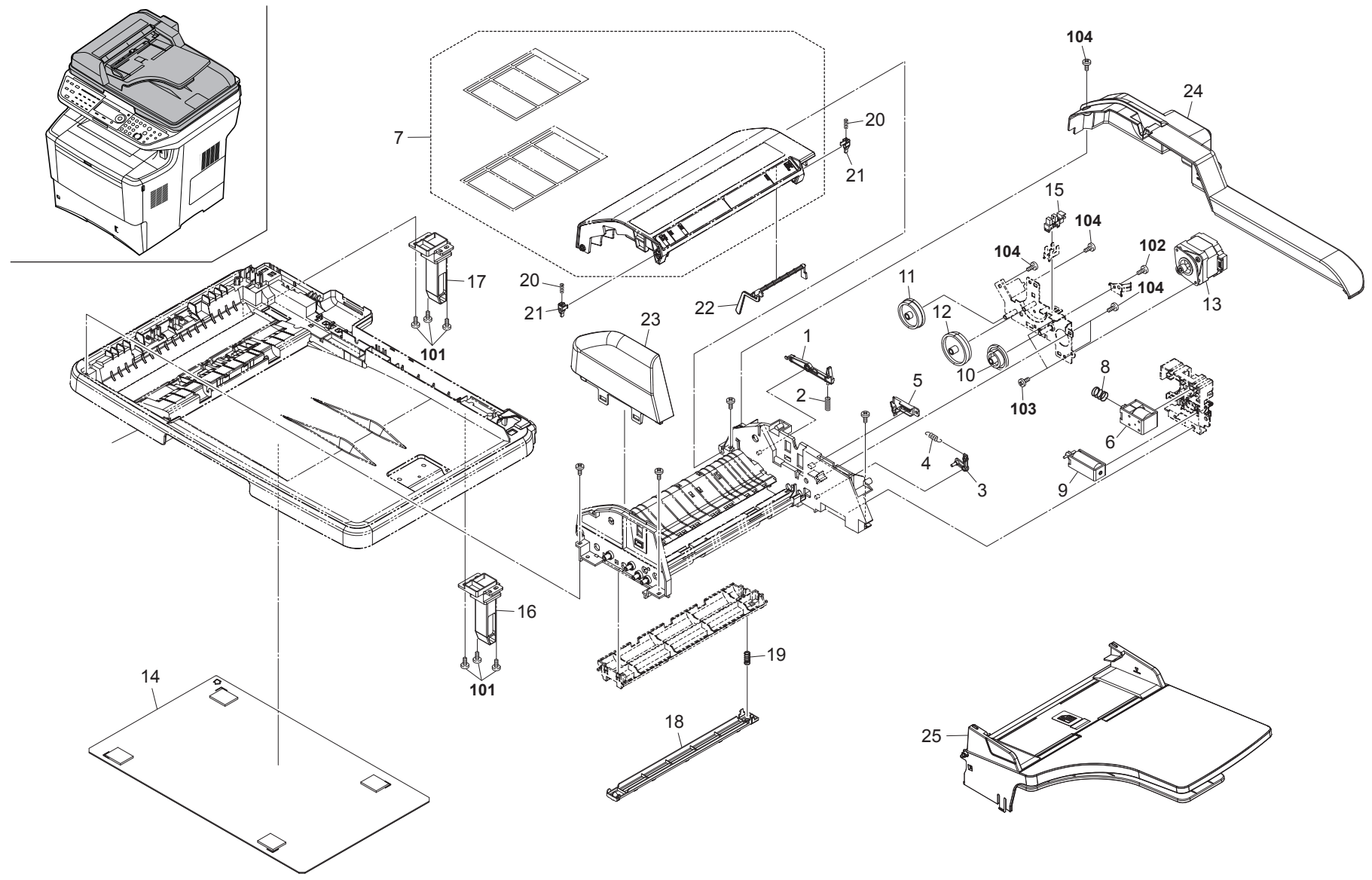
FIG. 19 Document Processor 2
