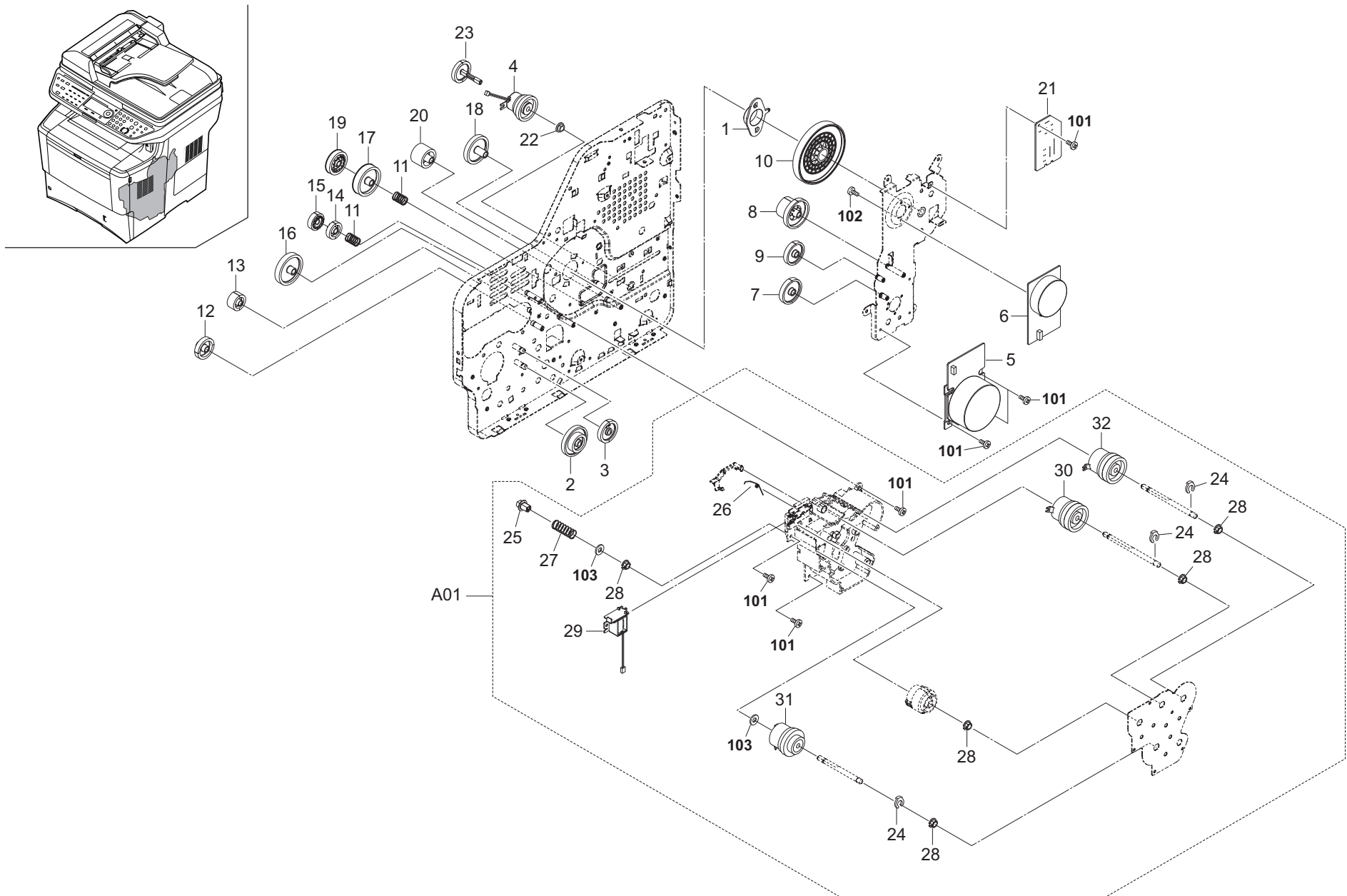
FIG. 14 Drive Section
