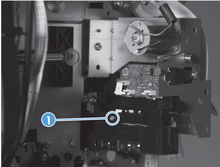
Figure 1-90 Remove the backscatter drop detect assembly (1 of 2)
