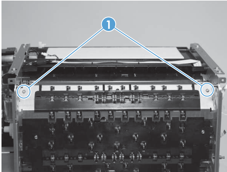
Figure 1-160 Remove the top left paper guide (2 of 3)
