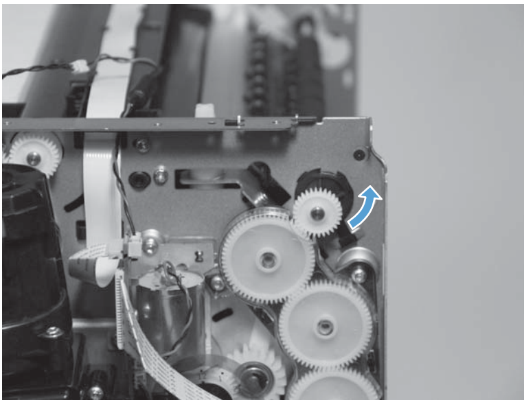
Figure 1-142 Remove the output drive shaft 4 (1 of 2)
