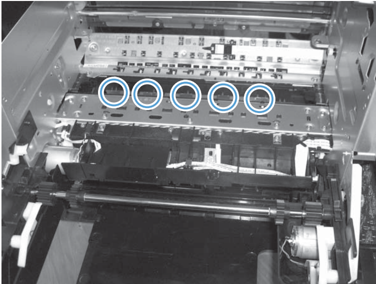
Figure 1-115 Remove the printbar (12 of 12)
