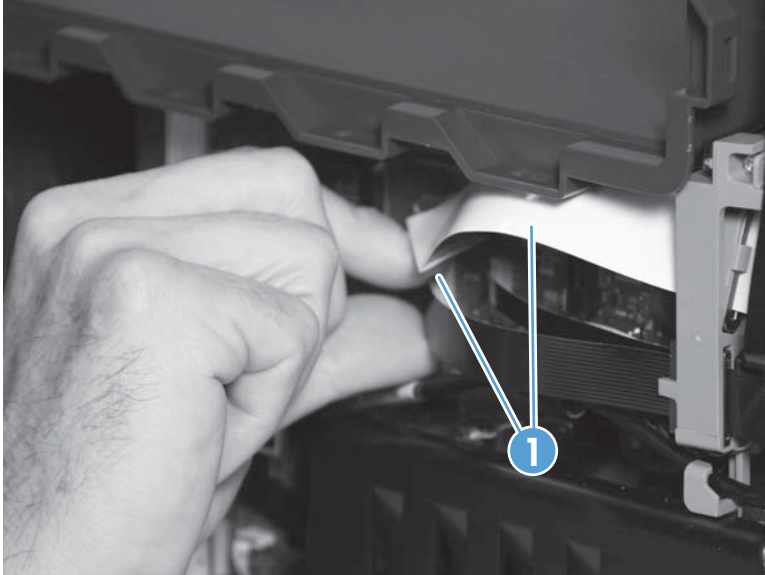
Figure 1-78 Remove the scanner and scanner support bracket (2 of 9)
