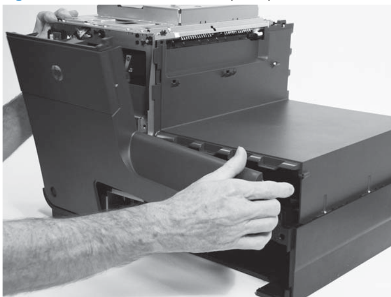
Figure 1-46 Remove the front cover (2 of 2)
