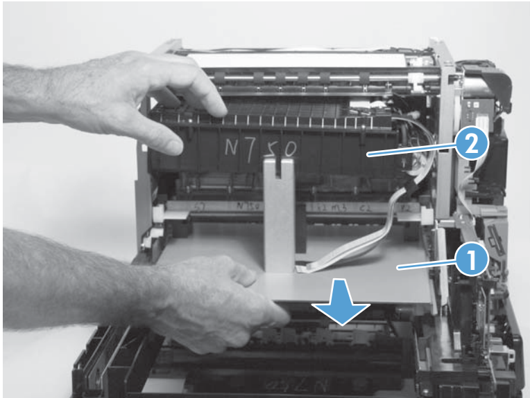
Figure 1-114 Remove the printbar (11 of 12)
