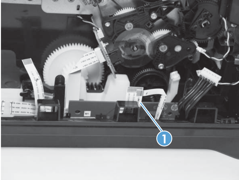
Figure 1-209 Remove the Tray 3 interconnect PCA (1 of 2)
