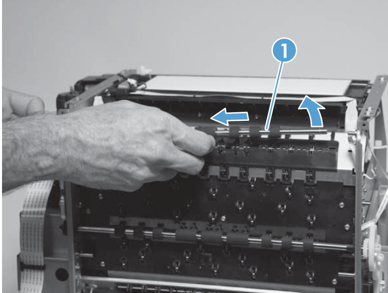
Figure 1-143 Remove the output drive shaft 4 (2 of 2)
