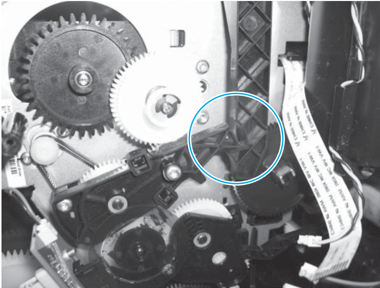
Figure 1-168 Correctly positioned service sled transmission
