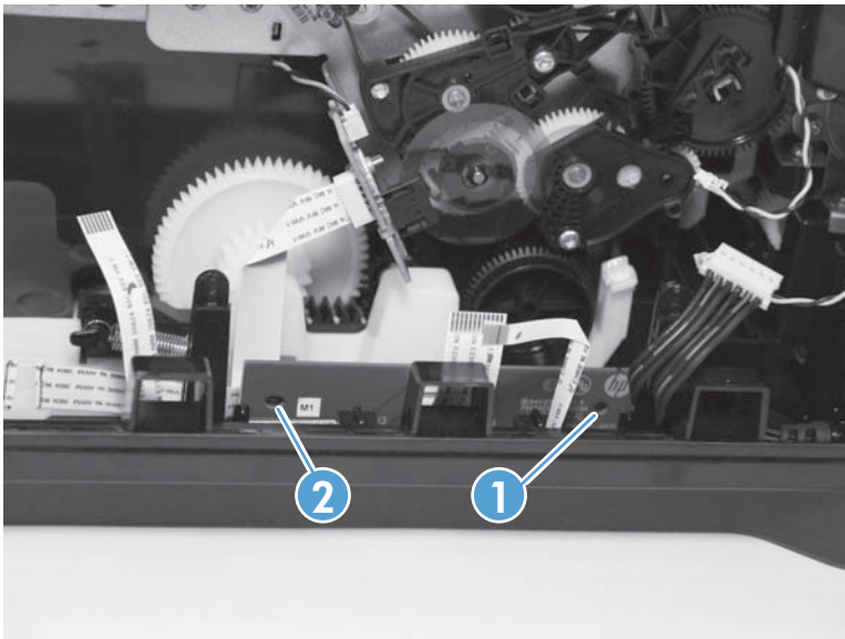
Figure 1-210 Remove the Tray 3 interconnect PCA (2 of 2)
