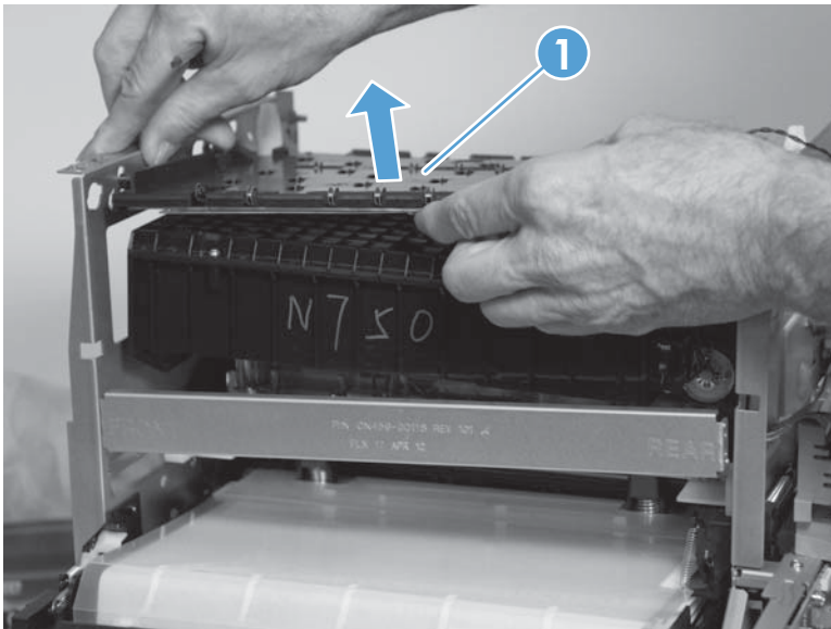
Figure 1-156 Remove the top paper guide (4 of 6)
