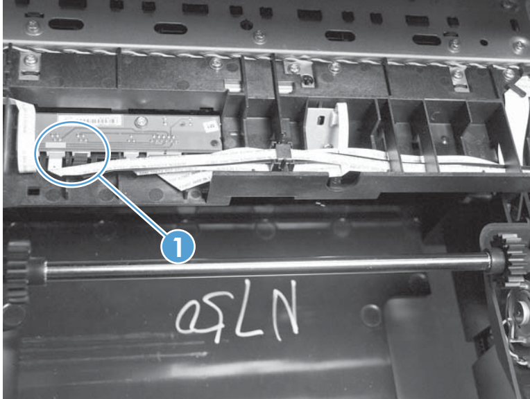
Figure 1-119 Remove the platen (2 of 7)
