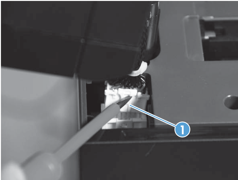
Figure 1-73 Remove the document feeder (4 of 5)
