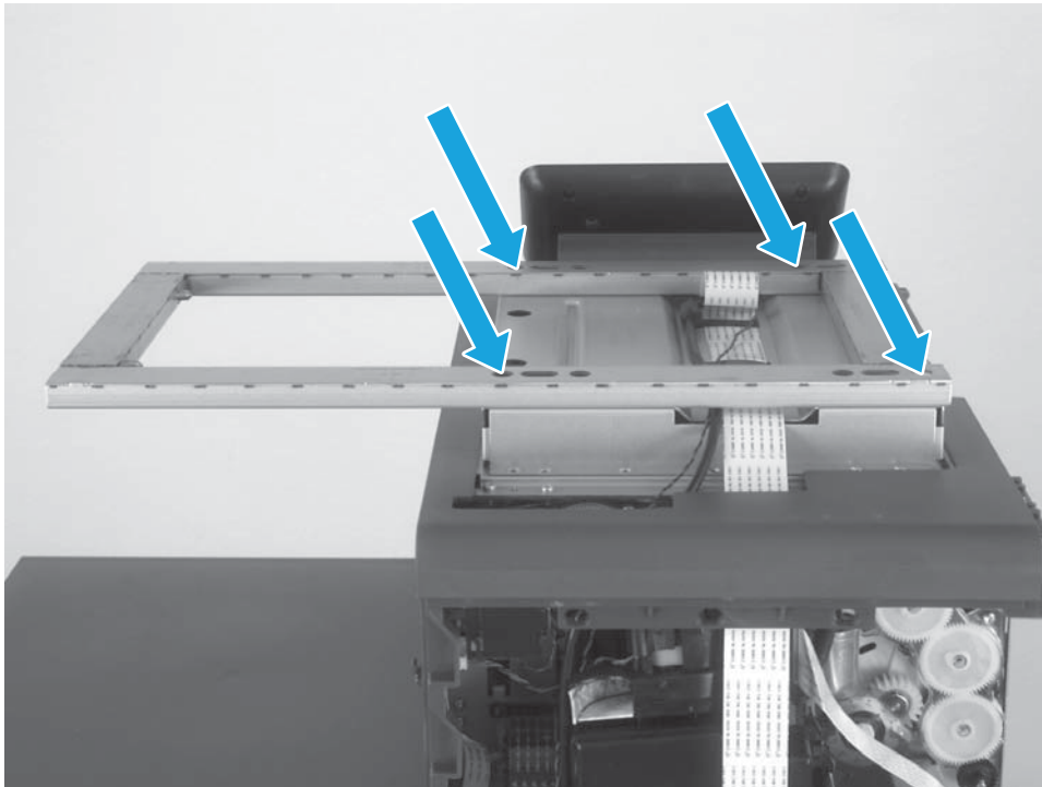
Figure 1-85 Remove the scanner and scanner support bracket (9 of 9)
