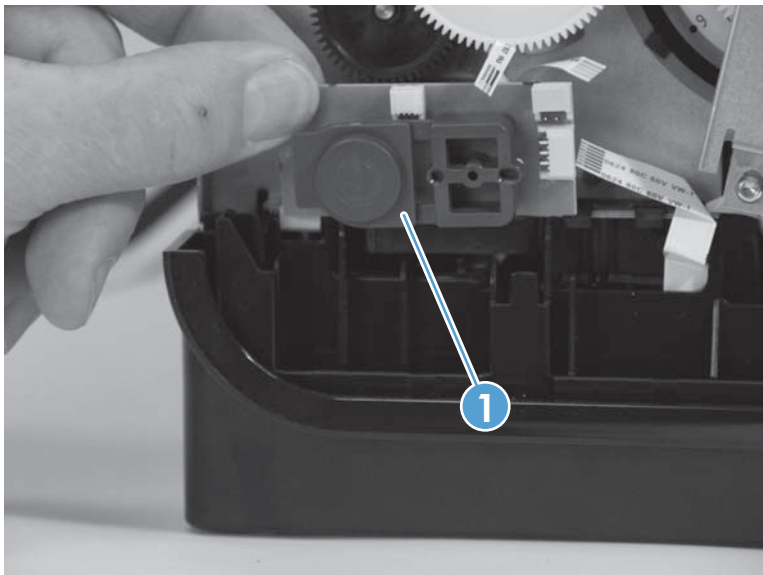
Figure 1-183 Remove the power button PCA (2 of 2)
