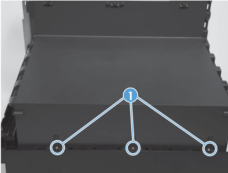
Figure 1-47 Remove the right cover (1 of 2)
