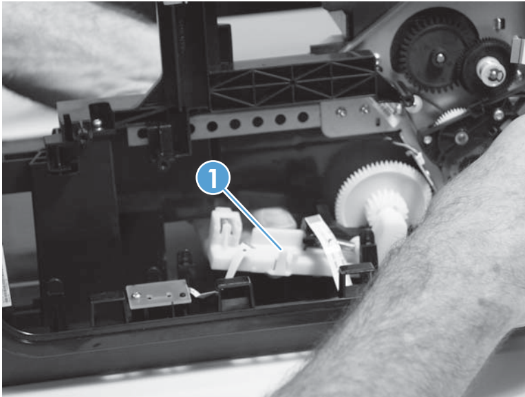
Figure 1-130 Remove the tray lift transmission assembly (2 of 2)
