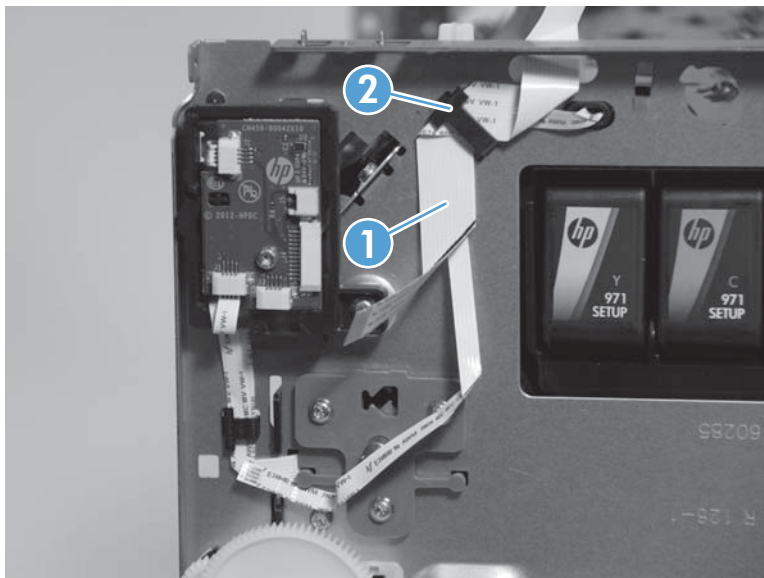
Figure 1-154 Remove the top paper guide (2 of 6)
