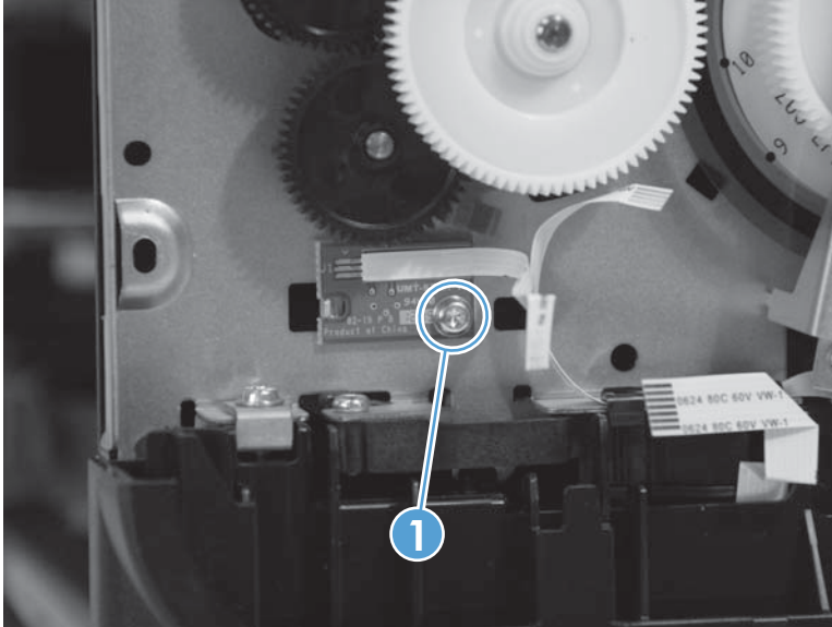
Figure 1-184 Remove the duplex module sensor PCA (1 of 2)
