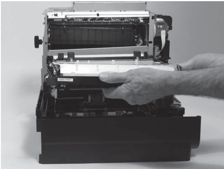
Figure 1-97 Remove the service sled assembly (6 of 6)
