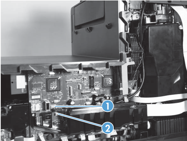
Figure 1-36 Remove the top cover and control panel (2 of 7)
