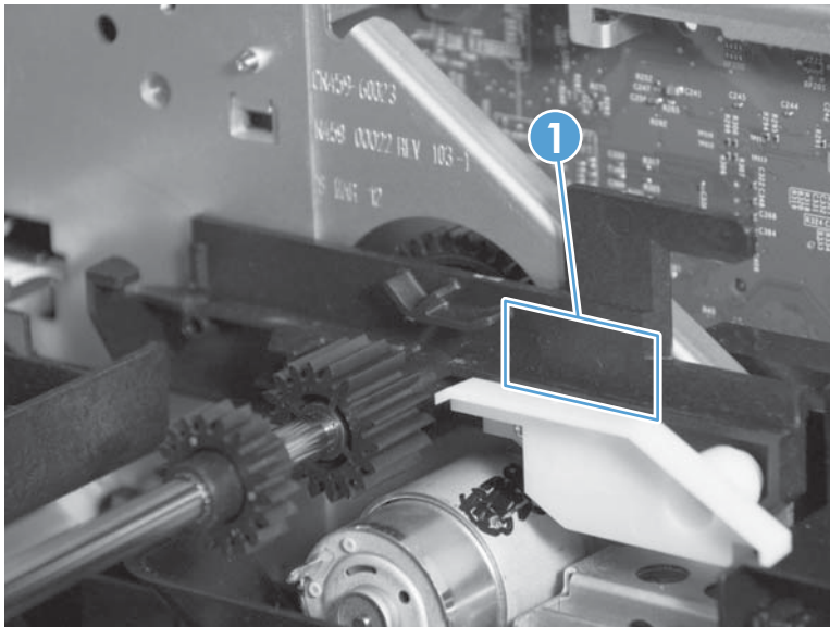
Figure 1-105 Remove the printbar (2 of 12)
