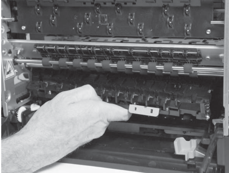
Figure 1-123 Remove the platen (6 of 7)
