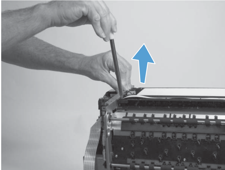
Figure 1-113 Remove the printbar (10 of 12)
