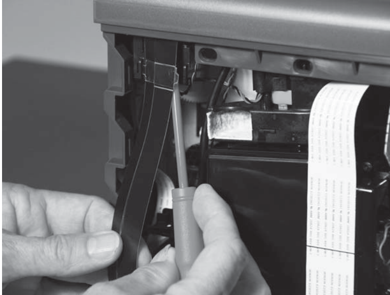
Figure 1-80 Remove the scanner and scanner support bracket (4 of 9)
