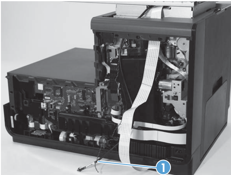
Figure 1-37 Remove the top cover and control panel (3 of 7)
