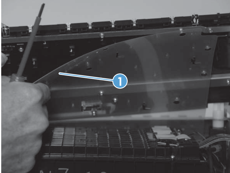
Figure 1-157 Remove the top paper guide (5 of 6)
