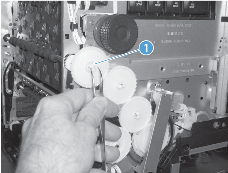
Figure 1-144 Remove drive shaft 3 (1 of 4)
