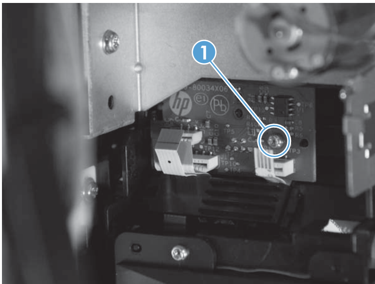
Figure 1-175 Remove the sensor carriage PCA and encoder strip (2 of 8)
