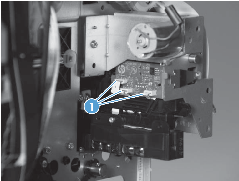
Figure 1-174 Remove the sensor carriage PCA and encoder strip (1 of 8)
