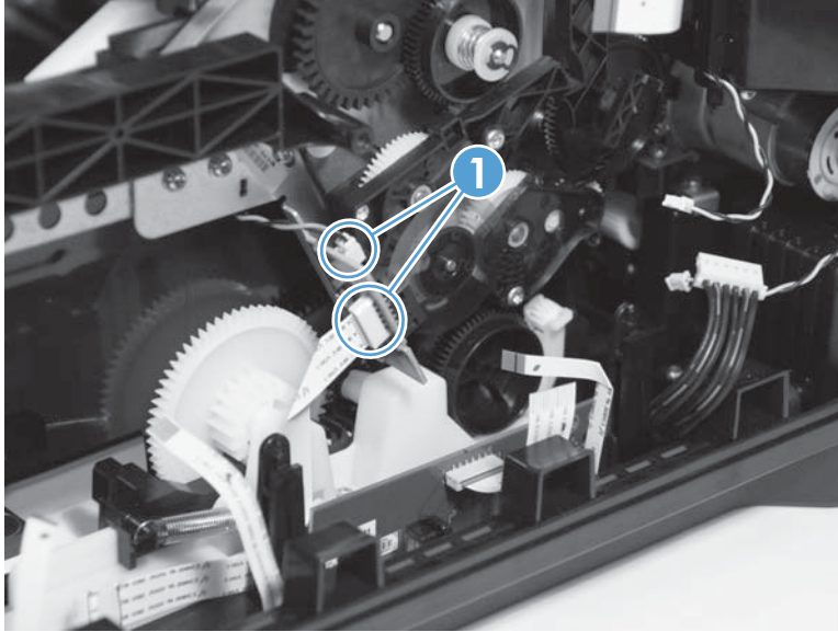
Figure 1-211 Remove the pick encoder distribution PCA (1 of 2)
