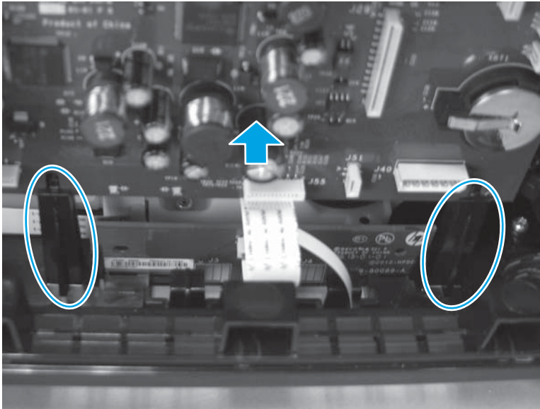
Figure 1-207 Remove the main PCA (7 of 8)
