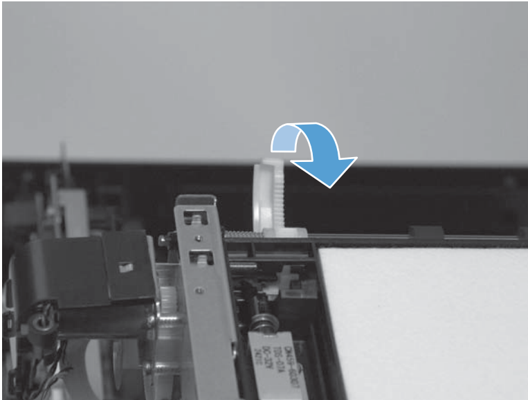
Figure 1-132 Remove the rack-eject lifter flap (1 of 3)
