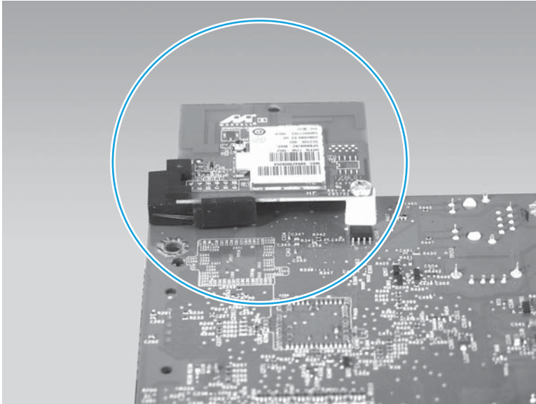
Figure 1-213 Remove the wireless PCA.
