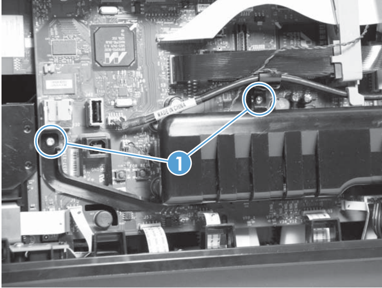
Figure 1-172 Remove the PCA safety shield (1 of 2)
