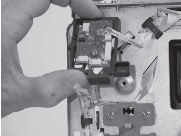
Figure 1-190 Remove the REDI distribution PCA PCA (3 of 3)
