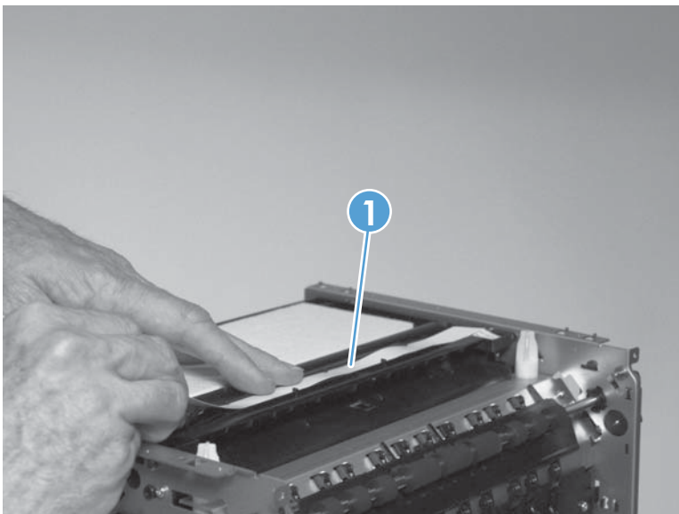
Figure 1-149 Remove the inner top frame (2 of 5)
