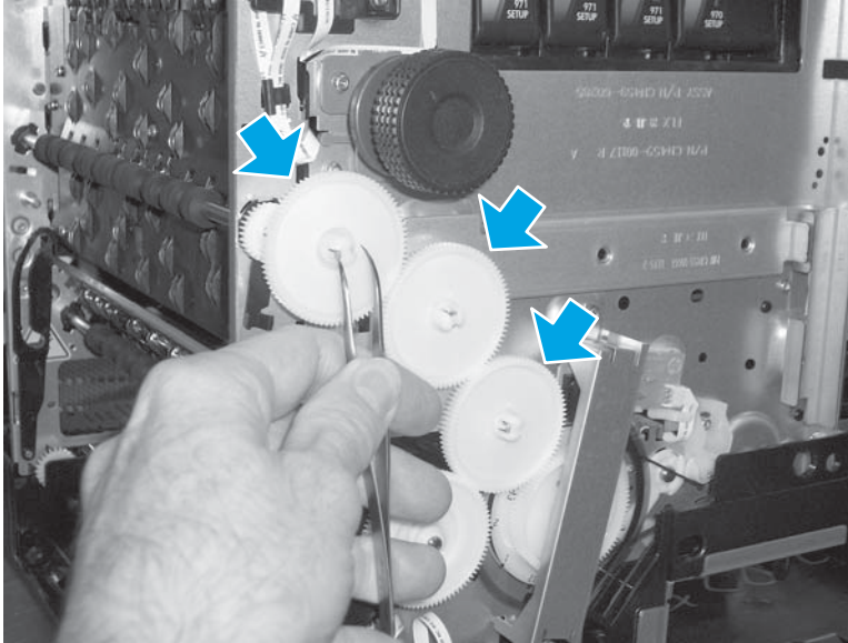
Figure 1-136 Remove the output drive gears
