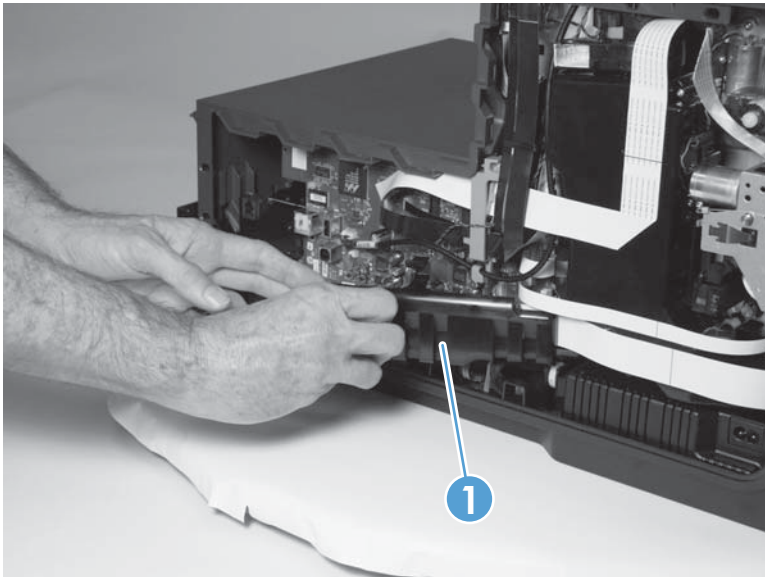
Figure 1-173 Remove the PCA safety shield (2 of 2)
