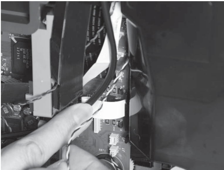
Figure 1-56 Remove the aerosol fan (8 of 12)
