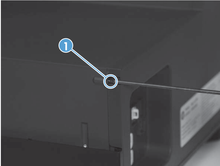
Figure 1-23 Remove the rear cover (1 of 2)
