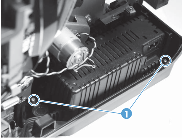
Figure 1-88 Remove the power supply (2 of 3)
