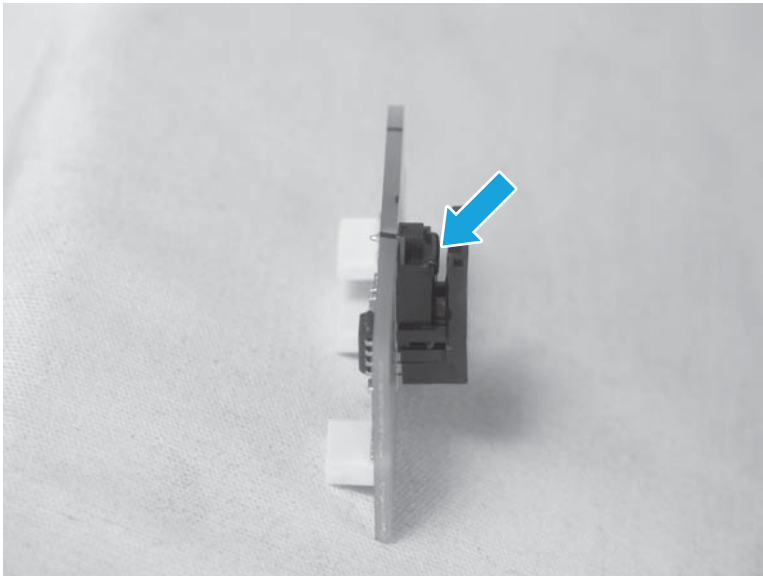
Figure 1-181 Remove the sensor carriage PCA and encoder strip (8 of 8)
