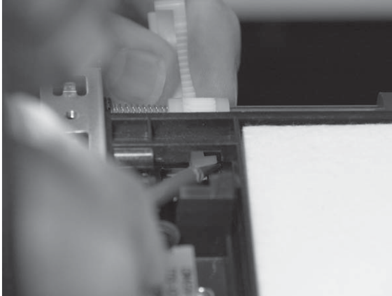
Figure 1-134 Remove the rack-eject lifter flap (3 of 3)
