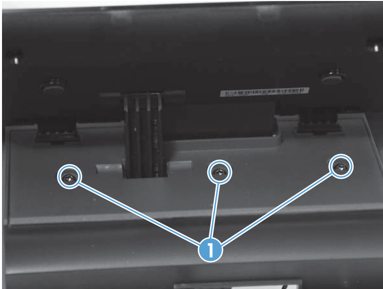
Figure 1-38 Remove the top cover and control panel (4 of 7)
