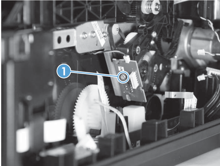
Figure 1-212 Remove the pick encoder distribution PCA (2 of 2)
