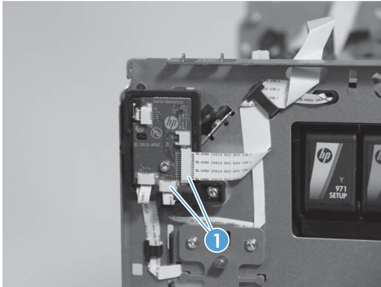
Figure 1-153 Remove the top paper guide (1 of 6)
