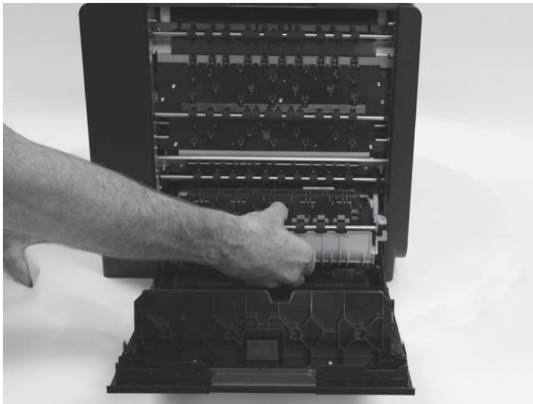
Figure 1-26 Remove the left door (2 of 6)
