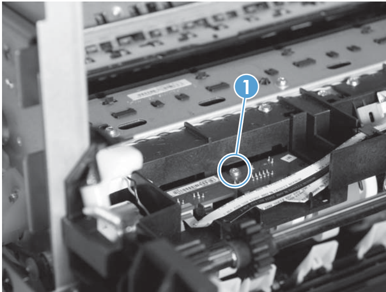
Figure 1-197 Remove the printzone distribution PCA (2 of 3)
