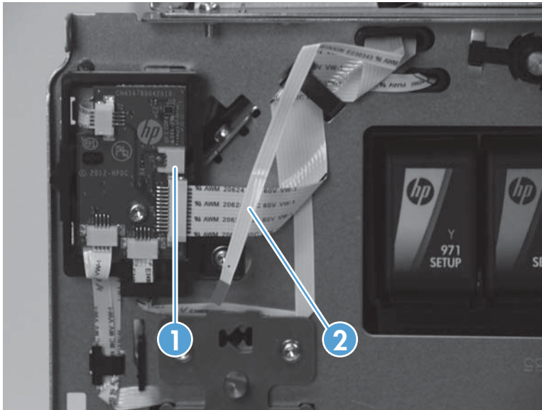
Figure 1-42 Remove the top cap assembly (1 of 3)
