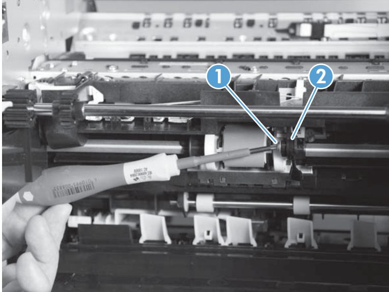
Figure 1-199 Remove the media presence sensor PCA/flag (1 of 2)
