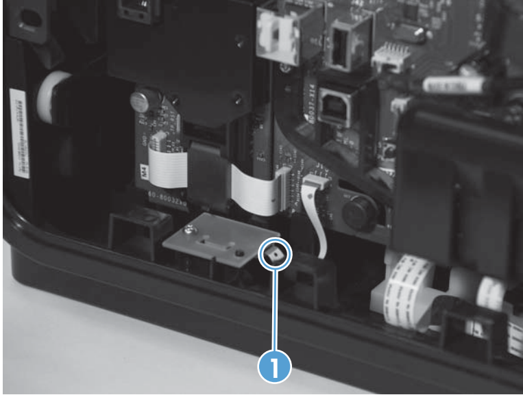
Figure 1-186 Remove the temperature sensor (1 of 2)
