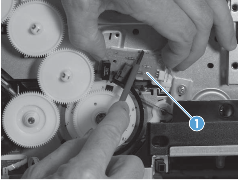
Figure 1-194 Remove the feed motor encoder sensor PCA (4 of 4)
