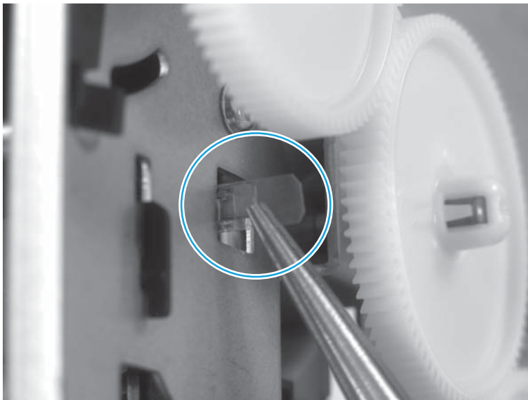
Figure 1-179 Remove the sensor carriage PCA and encoder strip (6 of 8)
