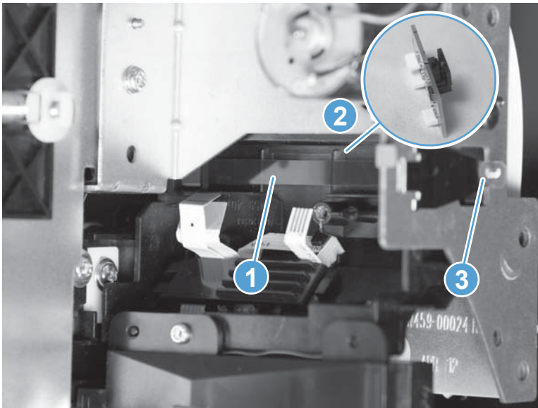
Figure 1-177 Remove the sensor carriage PCA and encoder strip (4 of 8)
