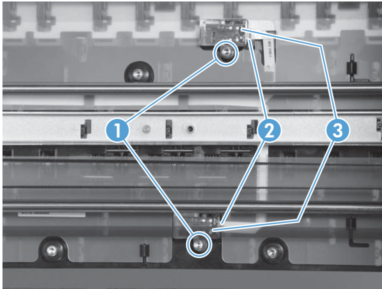
Figure 1-167 Remove the paper REDI sensors
