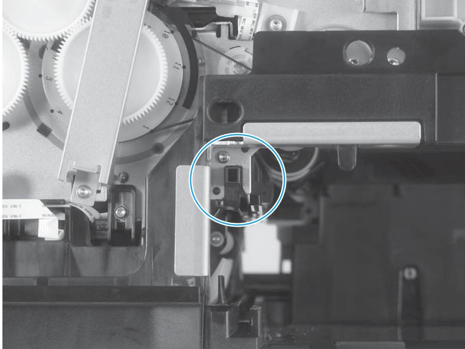
Figure 1-61 Remove the separator/pick assembly (1 of 4)
