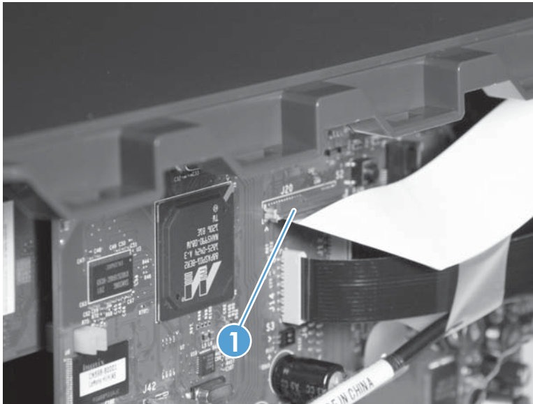
Figure 1-49 Remove the aerosol fan (1 of 12)
