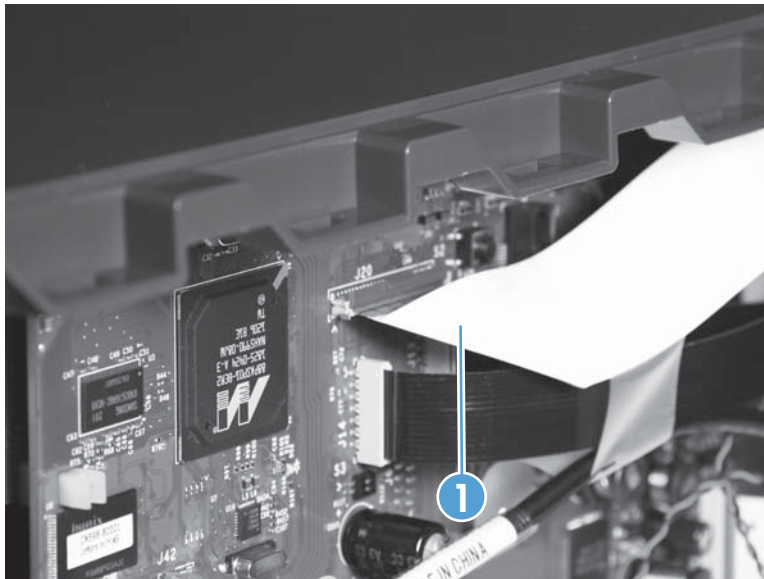
Figure 1-35 Remove the top cover and control panel (1 of 7)
