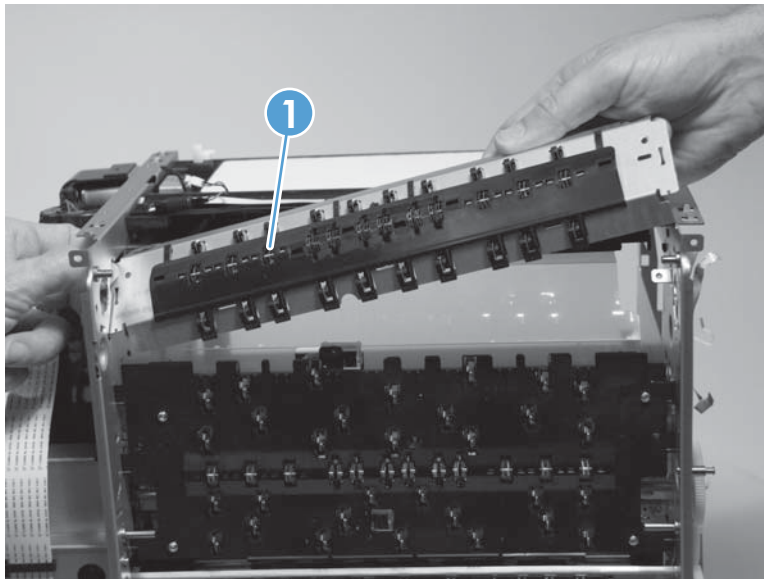
Figure 1-161 Remove the top left paper guide (3 of 3)
