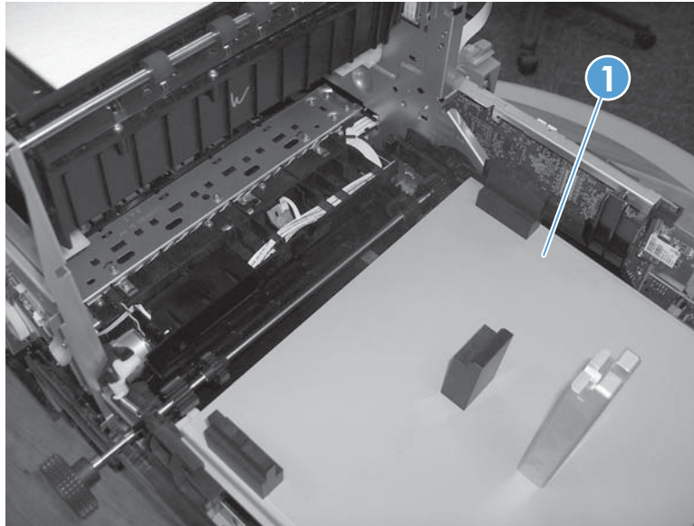
Figure 1-106 Remove the printbar (3 of 12)
