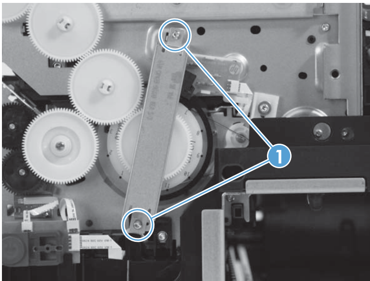
Figure 1-191 Remove the feed motor encoder sensor PCA (1 of 4)
