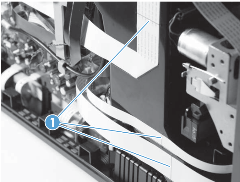
Figure 1-60 Remove the aerosol fan (12 of 12)
