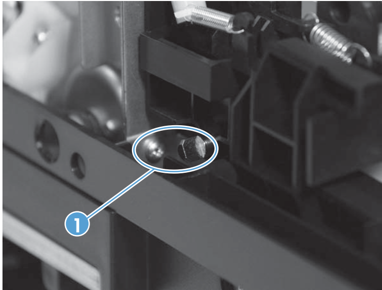
Figure 1-94 Remove the service sled assembly (3 of 6)
