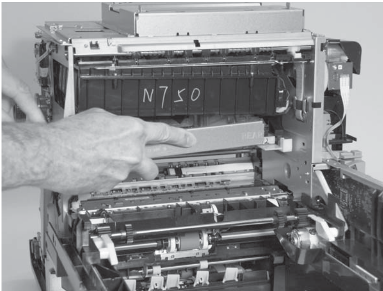
Figure 1-102 Remove the right cross brace (3 of 4)
