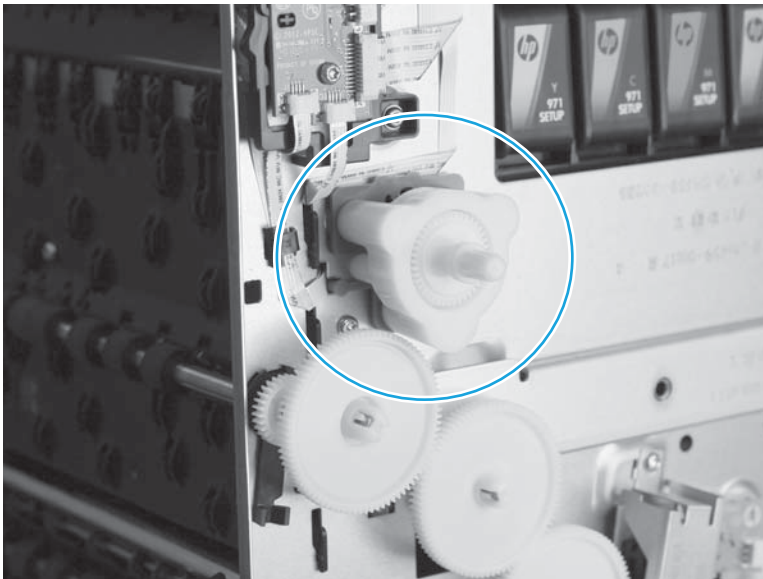
Figure 1-93 Remove the service sled assembly (2 of 6)
