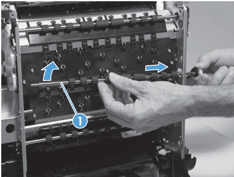
Figure 1-147 Remove drive shaft 3 (4 of 4)
