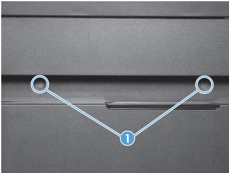
Figure 1-81 Remove the scanner and scanner support bracket (5 of 9)
