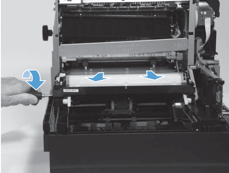
Figure 1-96 Remove the service sled assembly (5 of 6)
