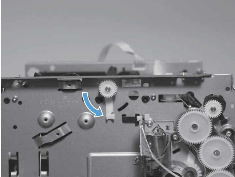
Figure 1-140 Remove the output drive shaft 5 (1 of 2)
