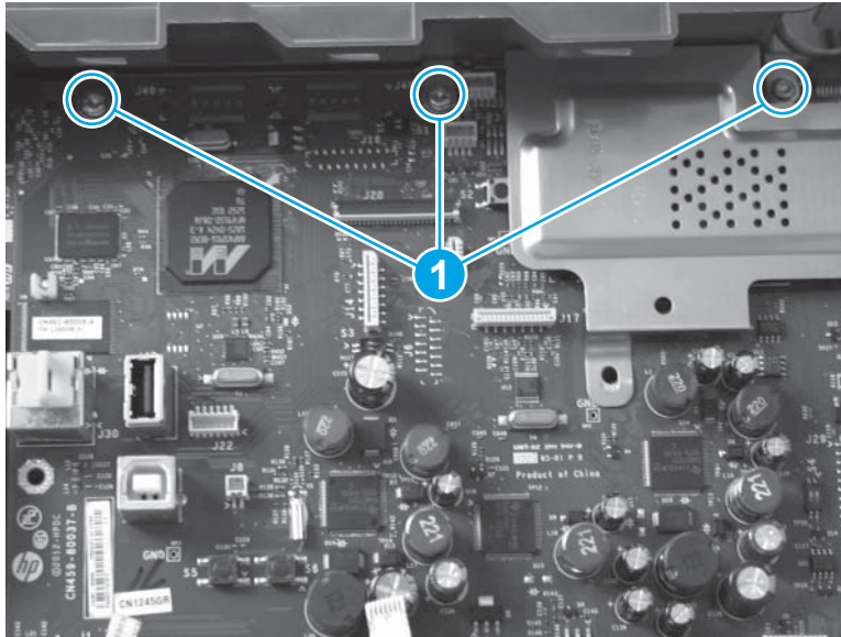
Figure 1-205 Remove the main PCA (5 of 8)
