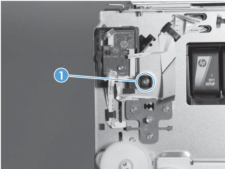
Figure 1-189 Remove the REDI distribution PCA PCA (2 of 3)
