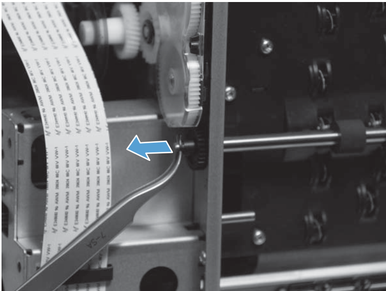
Figure 1-145 Remove drive shaft 3 (2 of 4)
