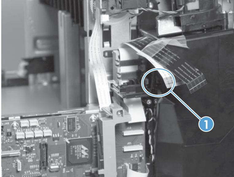
Figure 1-109 Remove the printbar (6 of 12)
