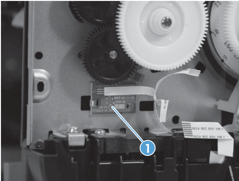
Figure 1-185 Remove the duplex module sensor PCA (2 of 2)
