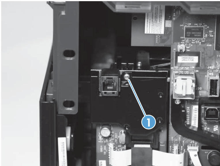
Figure 1-171 Remove the fax PCA (2 of 2)
