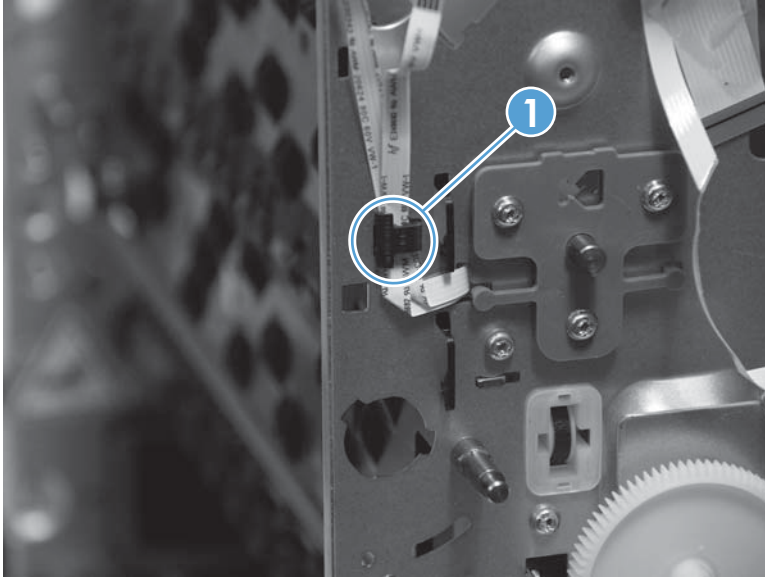
Figure 1-166 Remove the center left paper guide (4 of 4)
