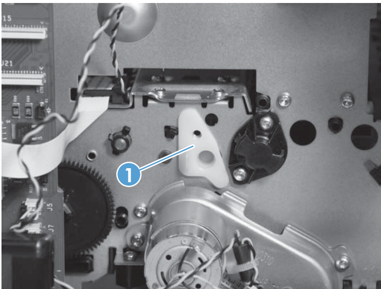
Figure 1-122 Remove the platen (5 of 7)
