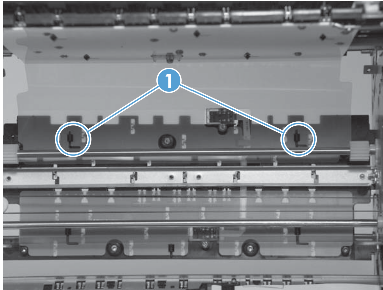
Figure 1-164 Remove the center left paper guide (2 of 4)
