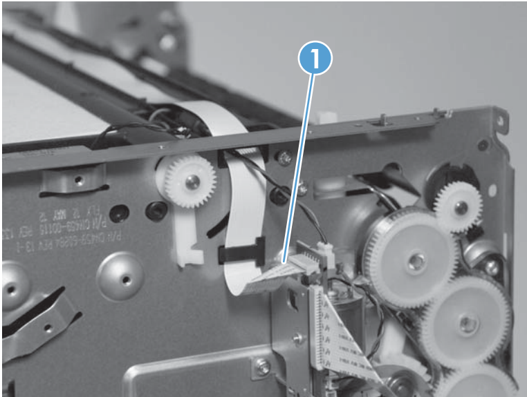
Figure 1-148 Remove the inner top frame (1 of 5)
