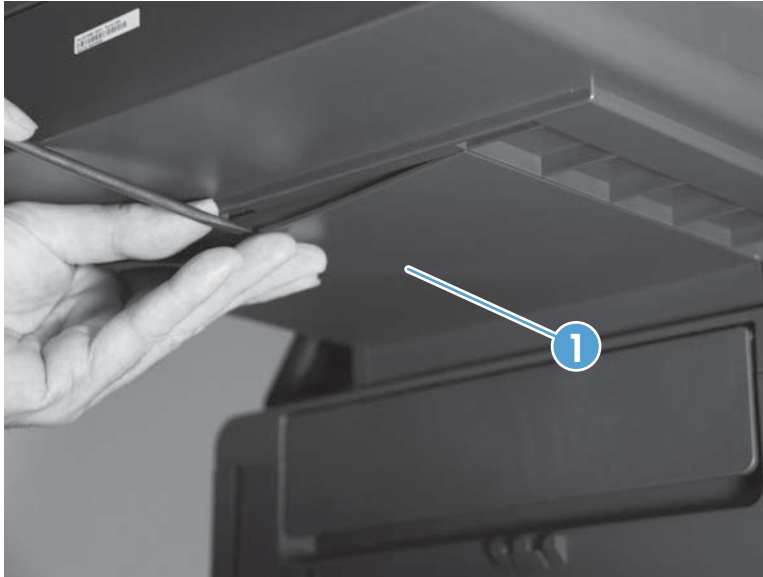
Figure 1-77 Remove the scanner and scanner support bracket (1 of 9)
