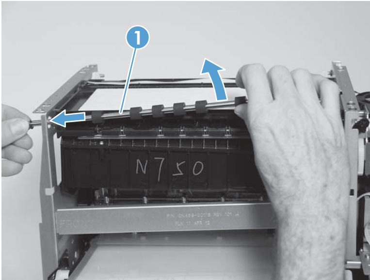
Figure 1-139 Remove the output drive shaft 6 (3 of 3)
