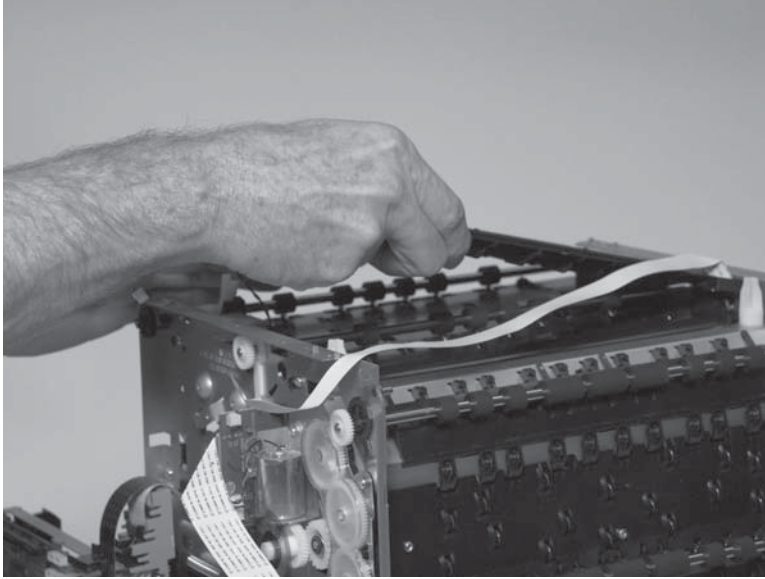
Figure 1-152 Remove the inner top frame (5 of 5)
