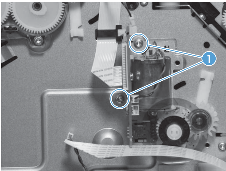
Figure 1-127 Remove the printbar lift motor (2 of 3)
