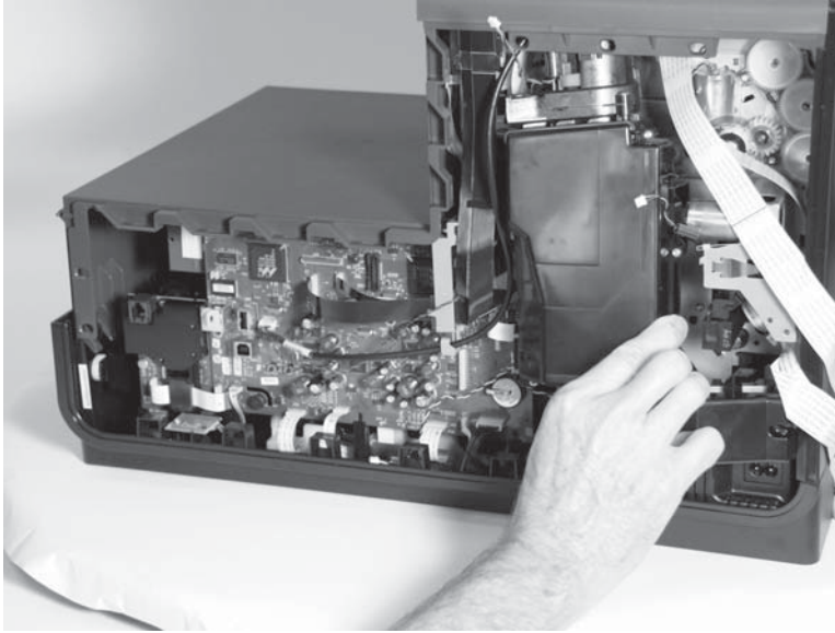
Figure 1-59 Remove the aerosol fan (11 of 12)
