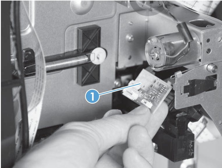
Figure 1-176 Remove the sensor carriage PCA and encoder strip (3 of 8)
