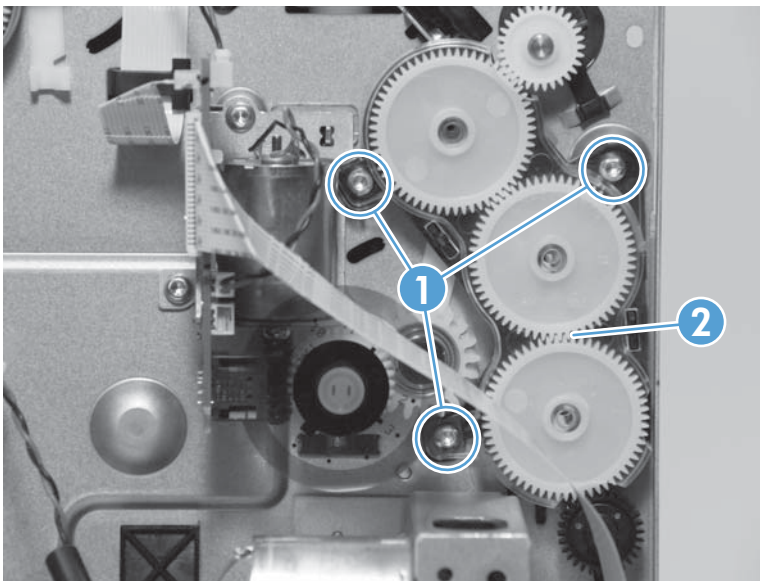
Figure 1-125 Remove the drying path gear assembly
