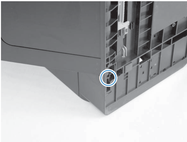
Figure 1-29 Remove the left door (5 of 6)
