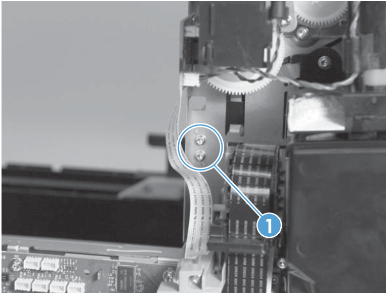
Figure 1-101 Remove the right cross brace (2 of 4)
