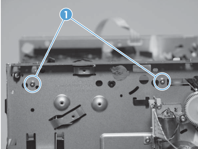
Figure 1-155 Remove the top paper guide (3 of 6)
