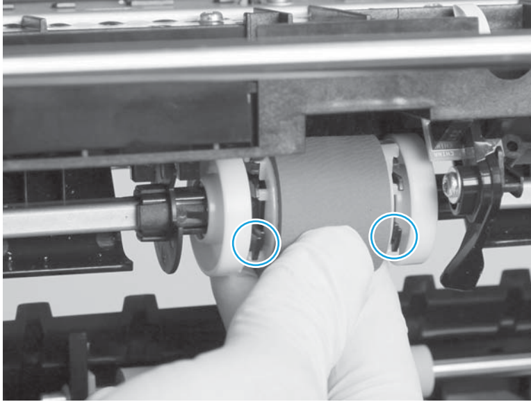
Figure 1-67 Reinstall the separator/pick assembly (3 of 5)
