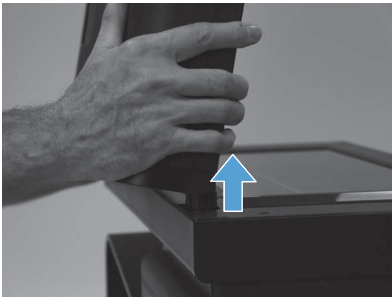
Figure 1-71 Remove the document feeder (2 of 5)
