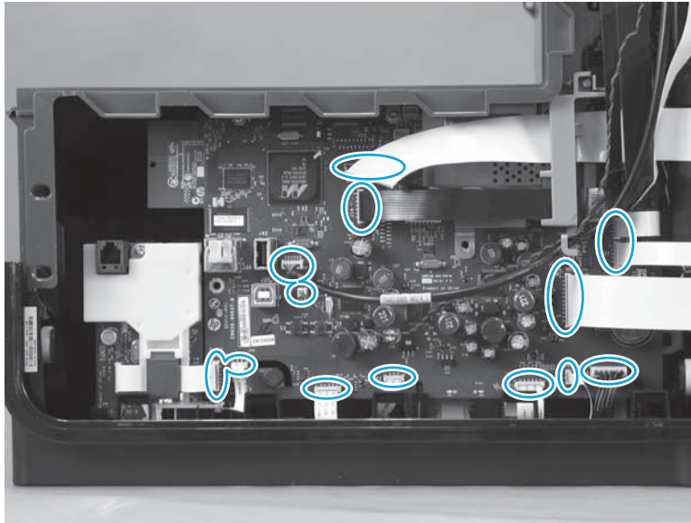
Figure 1-201 Remove the main PCA (1 of 8)
