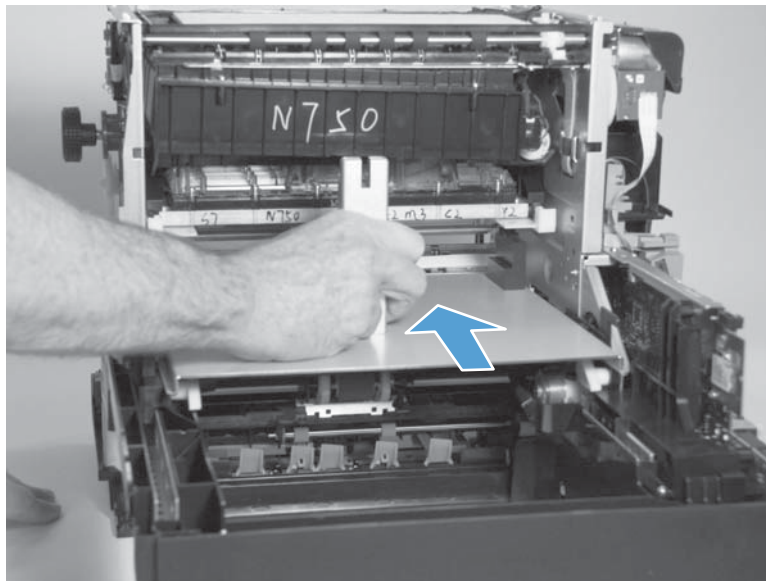
Figure 1-107 Remove the printbar (4 of 12)
