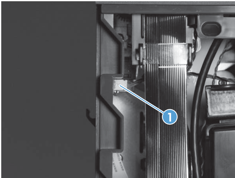
Figure 1-54 Remove the aerosol fan (6 of 12)
