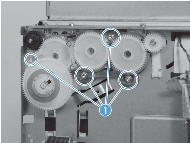
Figure 1-135 Remove the eject drive gear module
