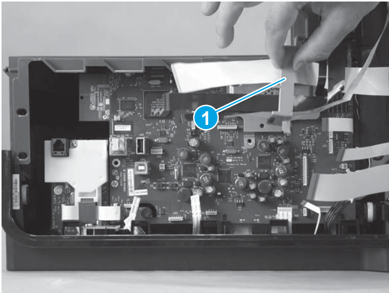
Figure 1-204 Remove the main PCA (4 of 8)
