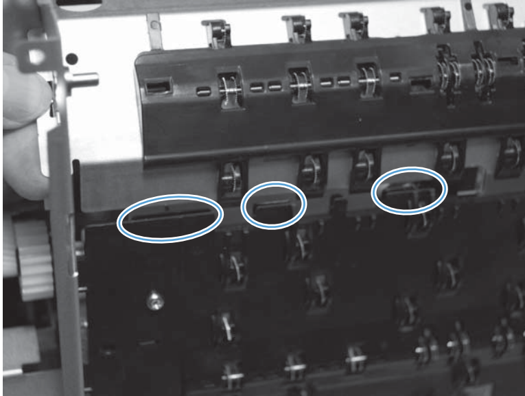
Figure 1-162 Reinstall the top left paper guide
