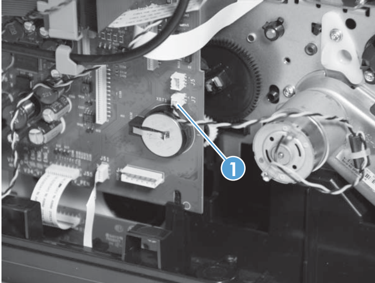
Figure 1-75 Remove the duplex drive module (1 of 2)
