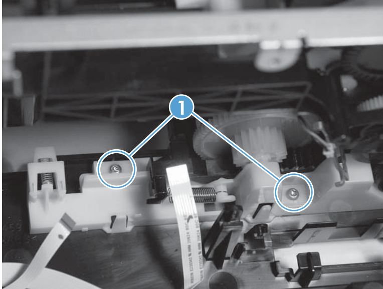
Figure 1-129 Remove the tray lift transmission assembly (1 of 2)
