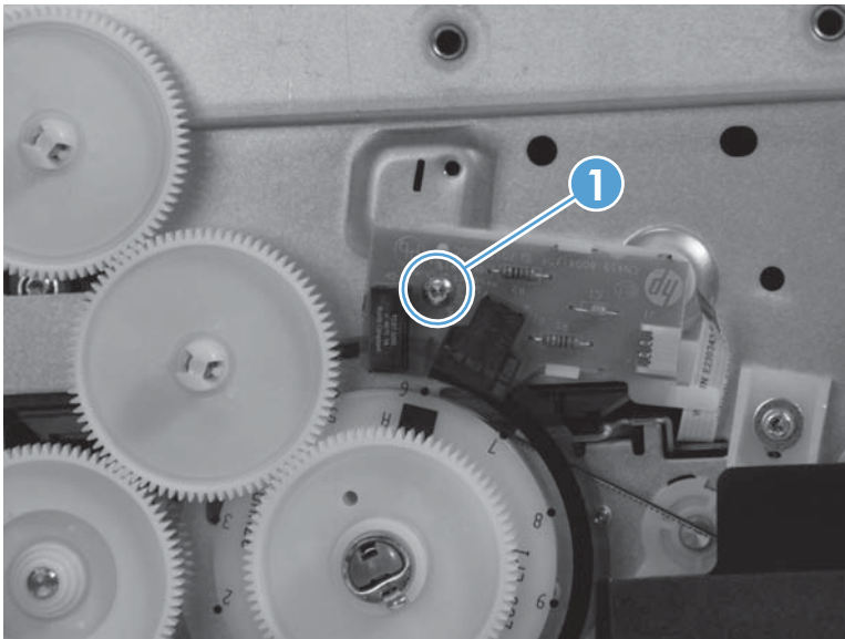
Figure 1-193 Remove the feed motor encoder sensor PCA (3 of 4)
