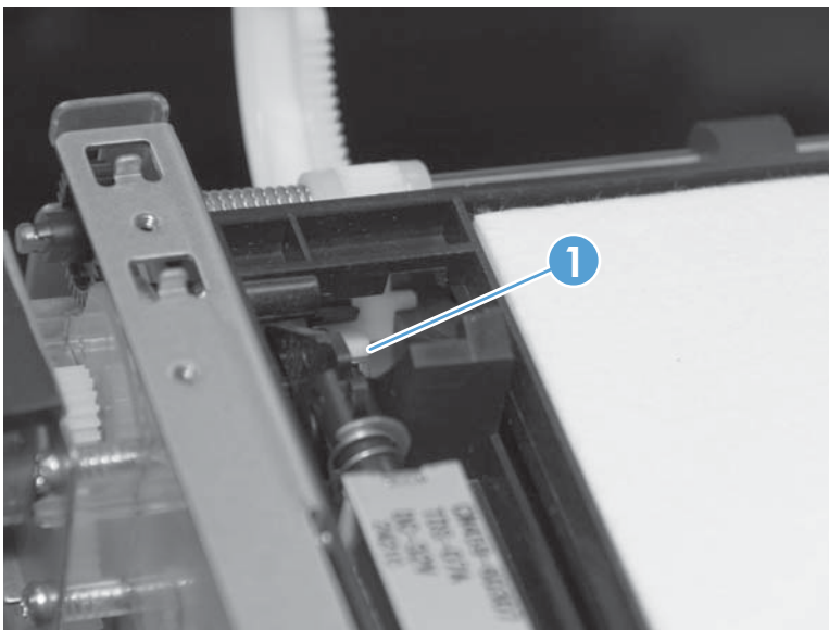
Figure 1-133 Remove the rack-eject lifter flap (2 of 3)
