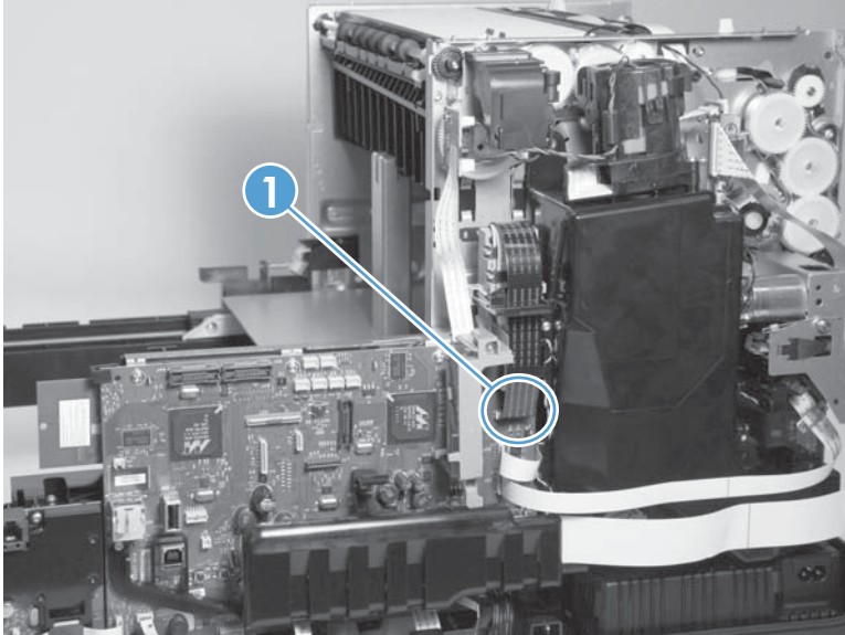
Figure 1-108 Remove the printbar (5 of 12)
