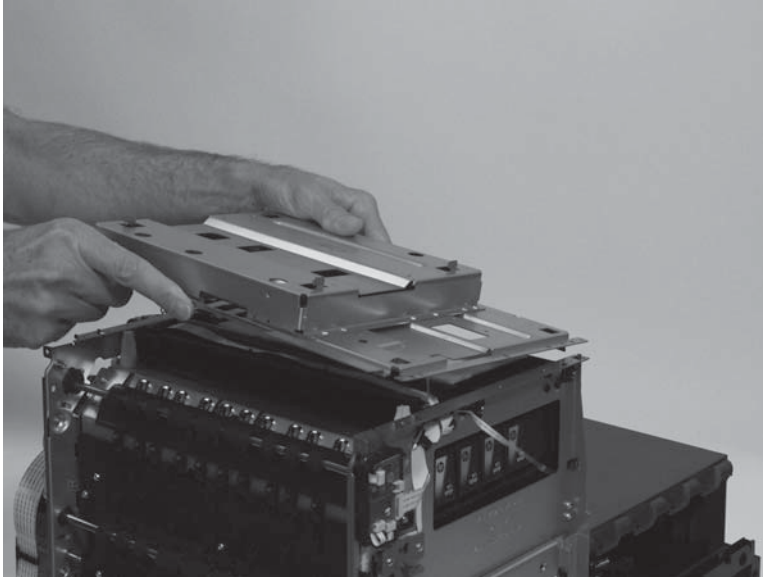
Figure 1-44 Remove the top cap (3 of 3)
