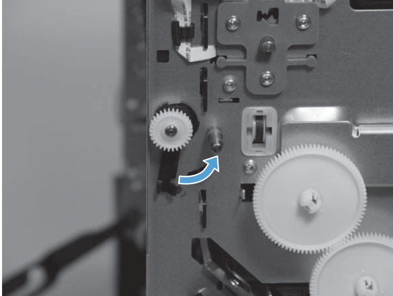
Figure 1-146 Remove drive shaft 3 (3 of 4)
