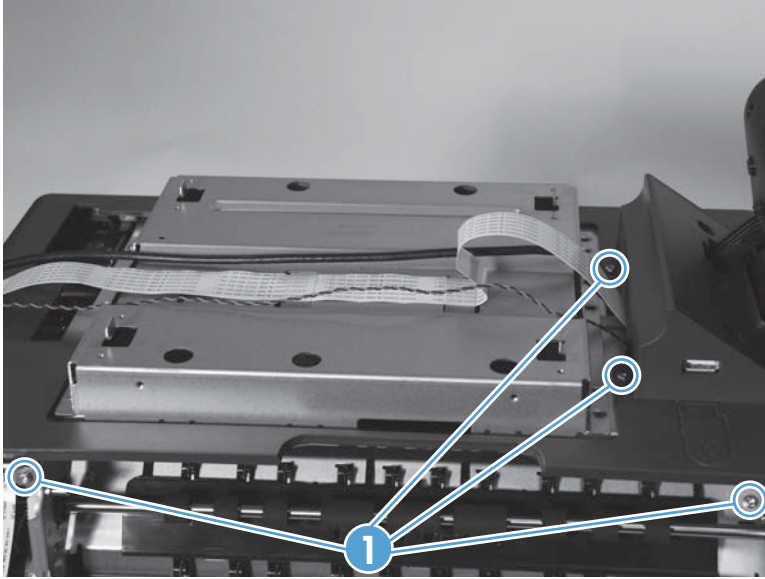
Figure 1-40 Remove the top cover and control panel (6 of 7)
