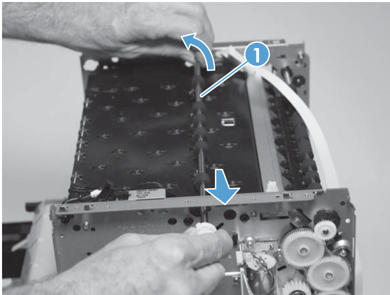
Figure 1-141 Remove the output drive shaft 5 (2 of 2)
