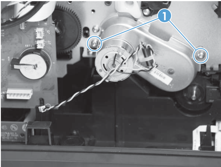
Figure 1-76 Remove the duplex drive module (2 of 2)
