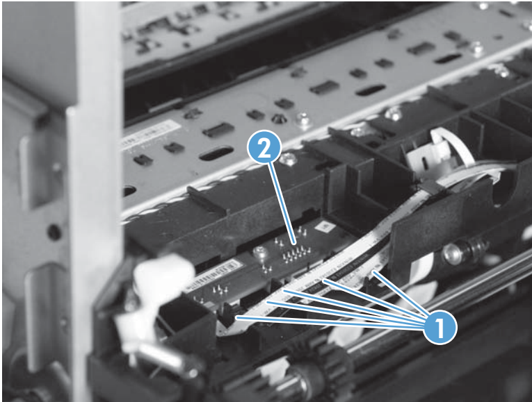
Figure 1-198 Remove the printzone distribution PCA (3 of 3)
