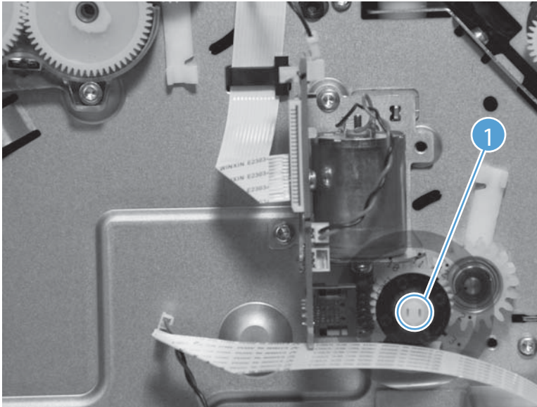
Figure 1-128 Remove the printbar lift motor (3 of 3)
