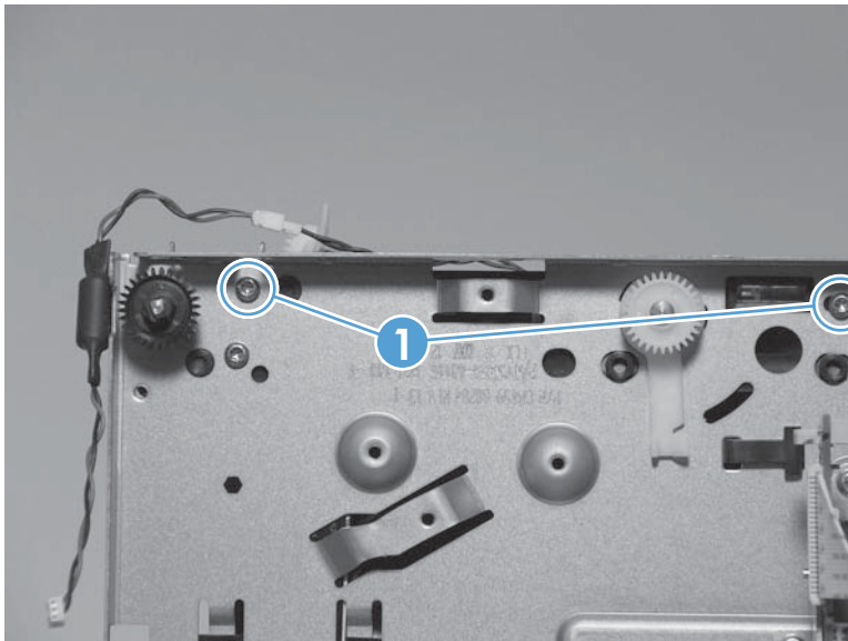
Figure 1-151 Remove the inner top frame (4 of 5)
