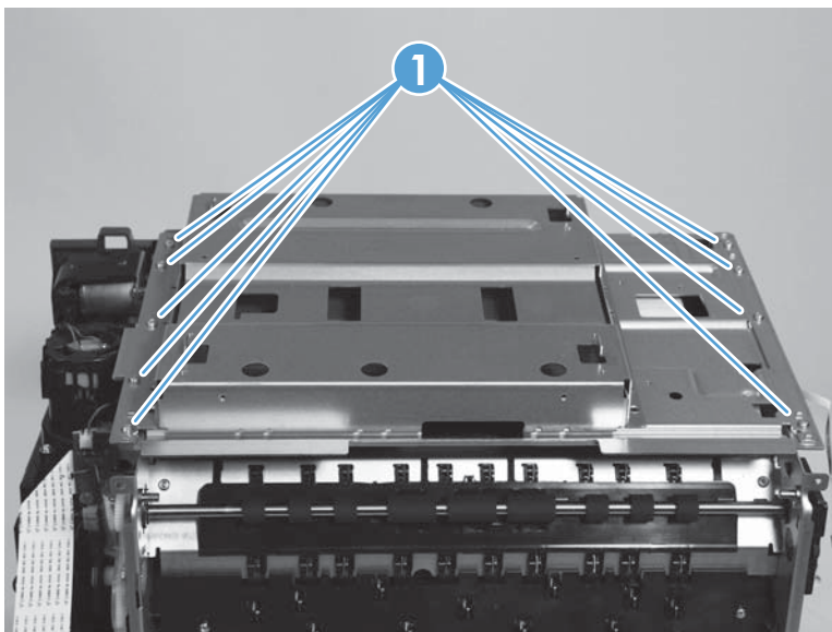
Figure 1-43 Remove the top cap (2 of 3)
