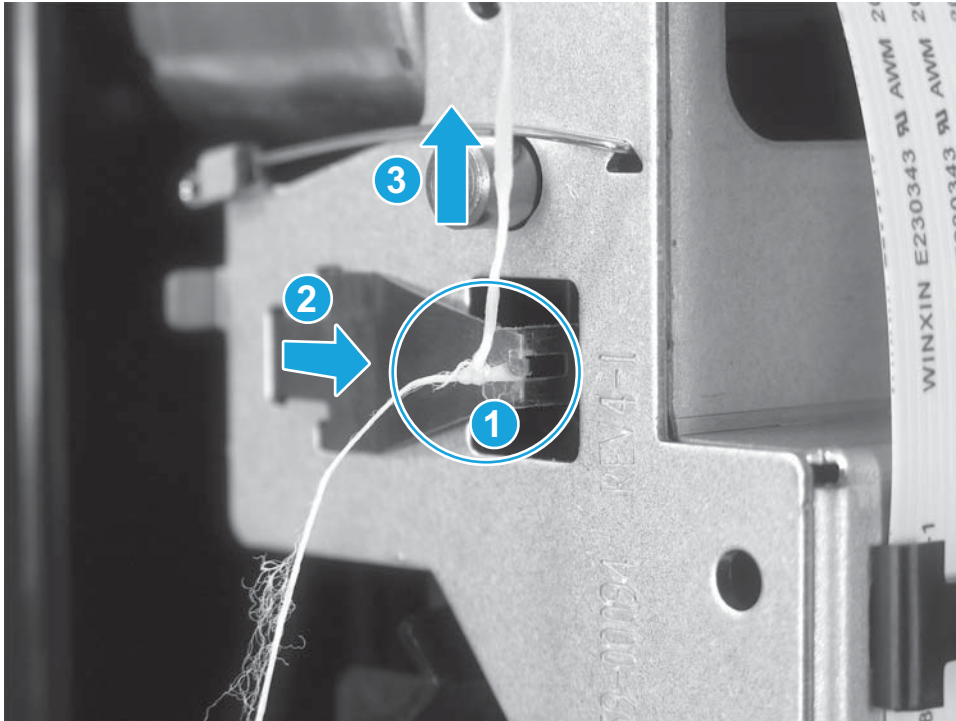
Figure 1-178 Remove the sensor carriage PCA and encoder strip (5 of 8)
