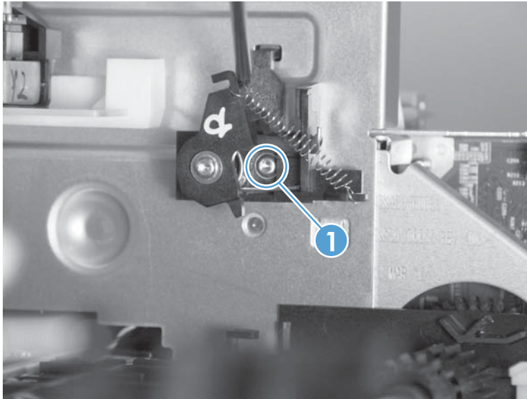
Figure 1-98 Remove the web advance rack assembly (1 of 2)
