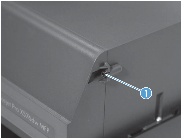
Figure 1-45 Remove the front cover (1 of 2)
