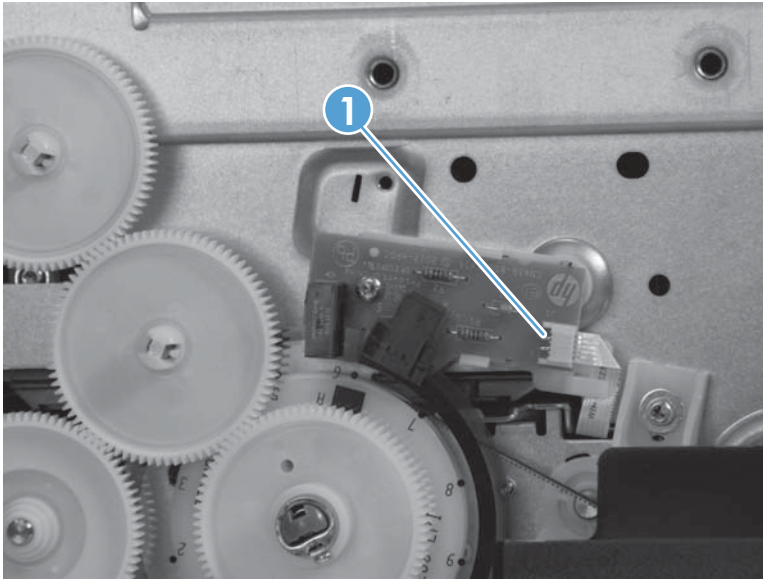
Figure 1-192 Remove the feed motor encoder sensor PCA (2 of 4)
