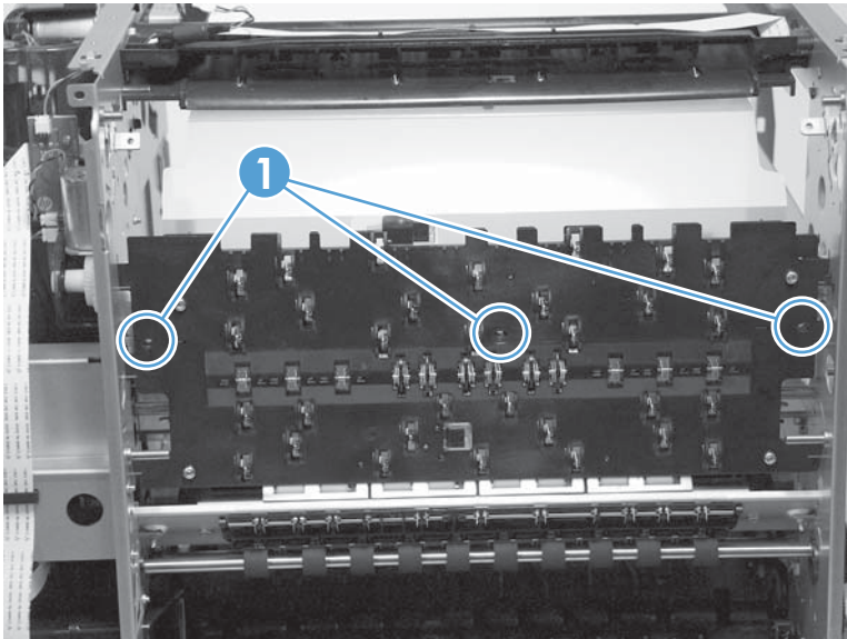
Figure 1-163 Remove the center left paper guide (1 of 4)
