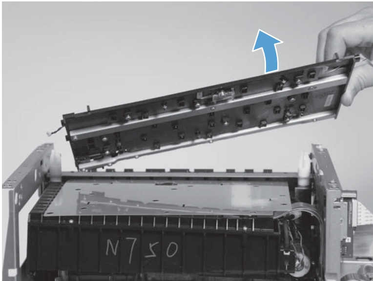
Figure 1-158 Remove the top paper guide (6 of 6)
