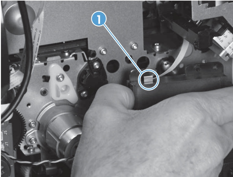
Figure 1-91 Remove the backscatter drop detect assembly (2 of 2)
