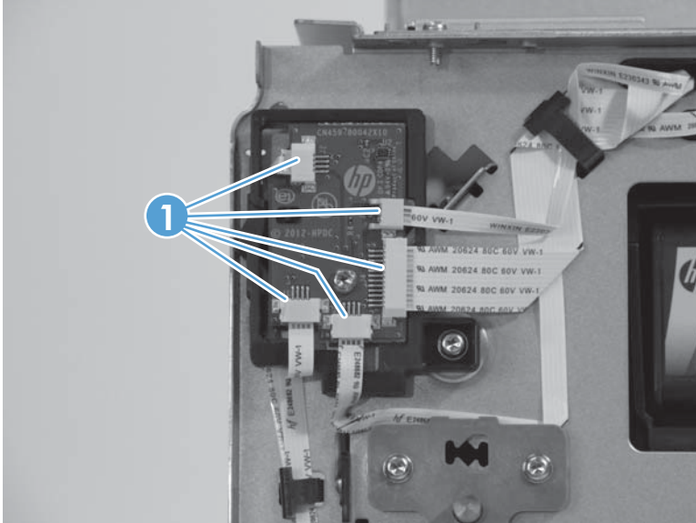
Figure 1-188 Remove the REDI distribution PCA PCA (1 of 3)
