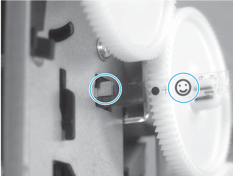
Figure 1-180 Remove the sensor carriage PCA and encoder strip (7 of 8)
