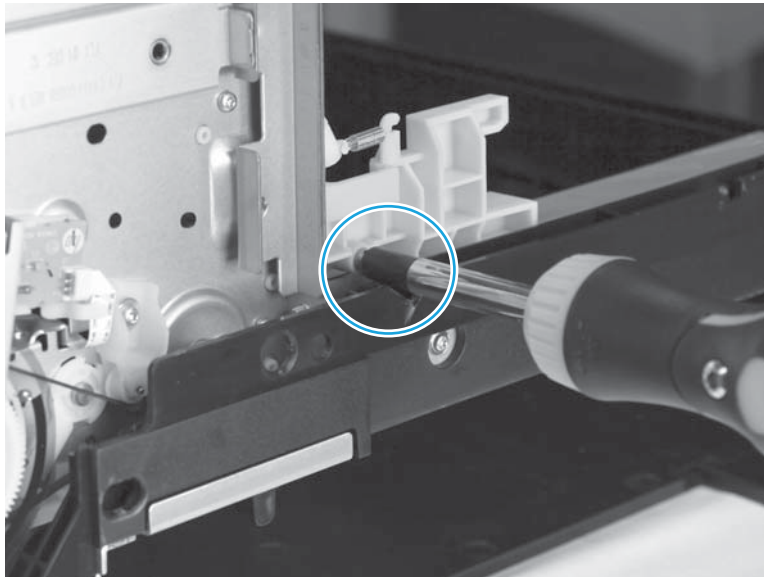
Figure 1-95 Remove the service sled assembly (4 of 6)
