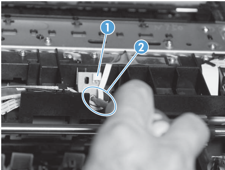
Figure 1-200 Remove the media presence sensor PCA/flag (2 of 2)
