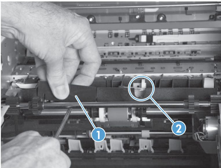
Figure 1-118 Remove the platen (1 of 7)
