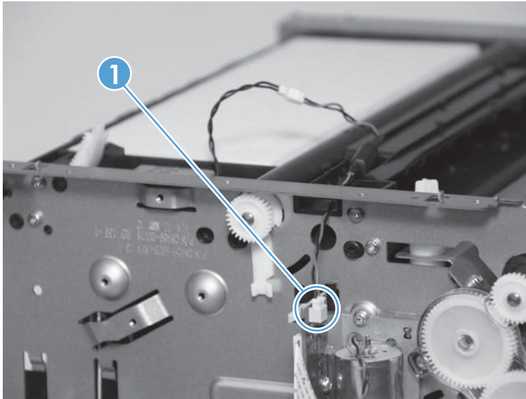
Figure 1-150 Remove the inner top frame (3 of 5)
