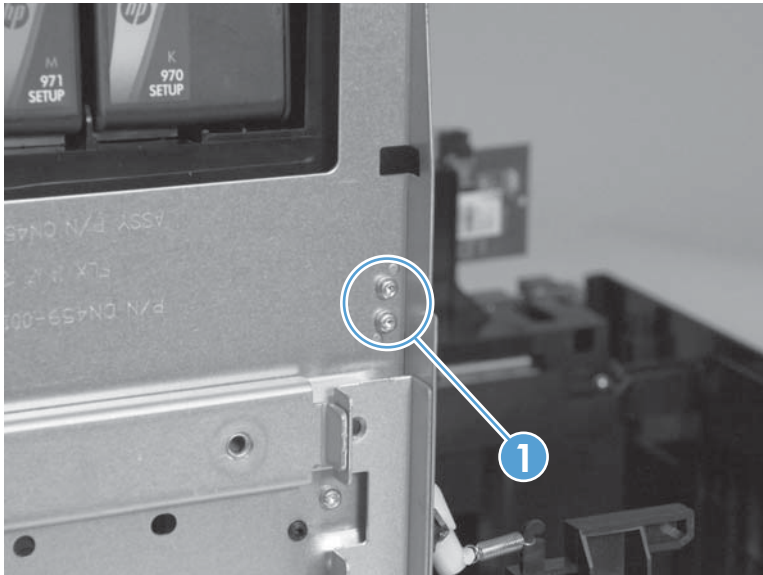
Figure 1-100 Remove the right cross brace (1 of 4)
