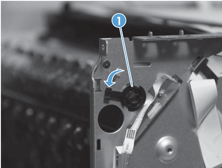
Figure 1-159 Remove the top left paper guide (1 of 3)
