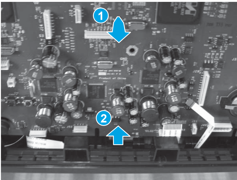
Figure 1-208 Remove the main PCA (8 of 8)
