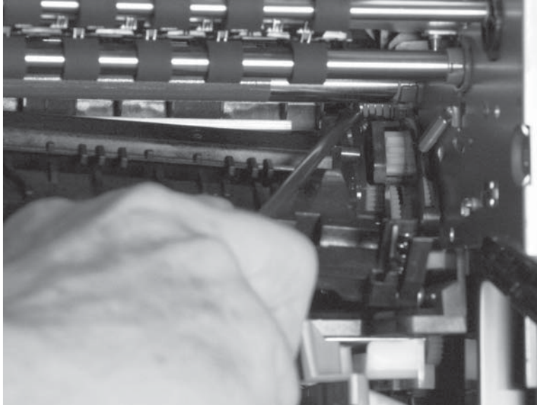
Figure 1-124 Remove the platen (7 of 7)
