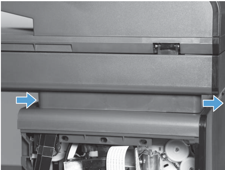
Figure 1-83 Remove the scanner and scanner support bracket (7 of 9)
