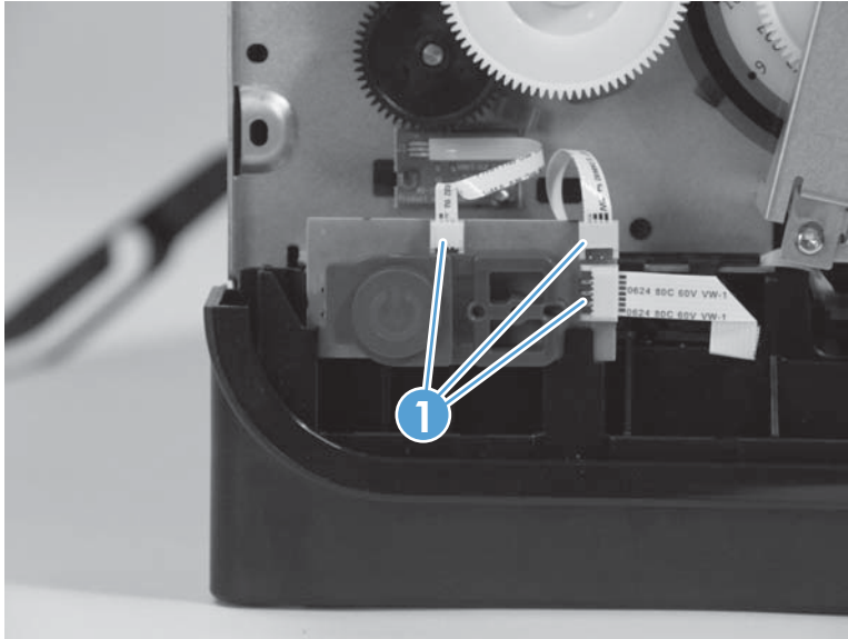
Figure 1-182 Remove the power button PCA (1 of 2)
