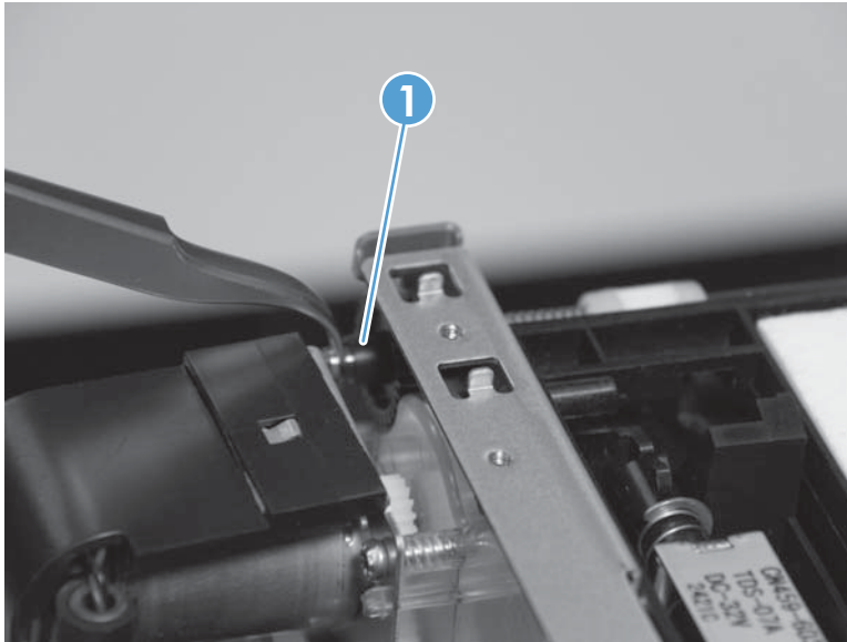
Figure 1-137 Remove the output drive shaft 6 (1 of 3)
