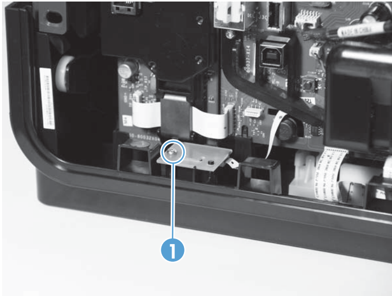
Figure 1-187 Remove the temperature sensor (2 of 2)
