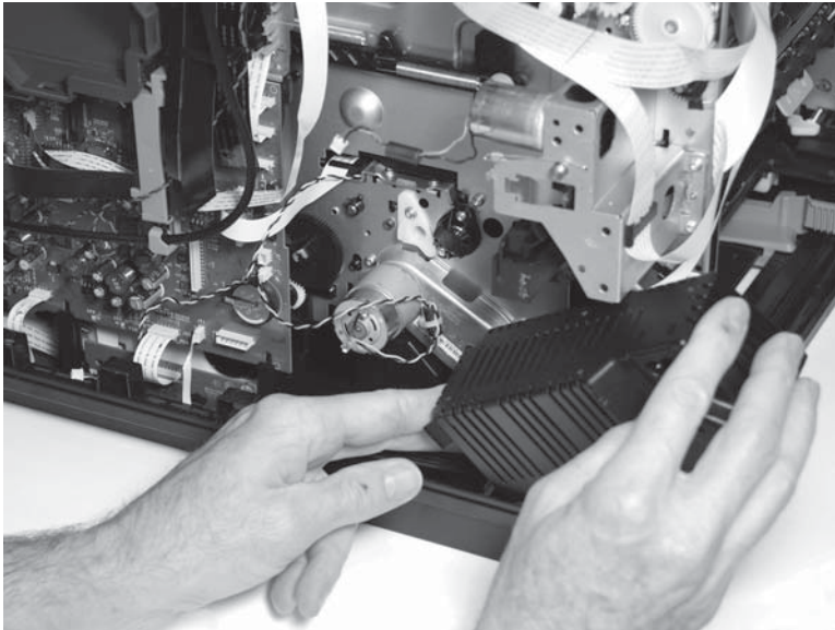
Figure 1-89 Remove the power supply (3 of 3)
