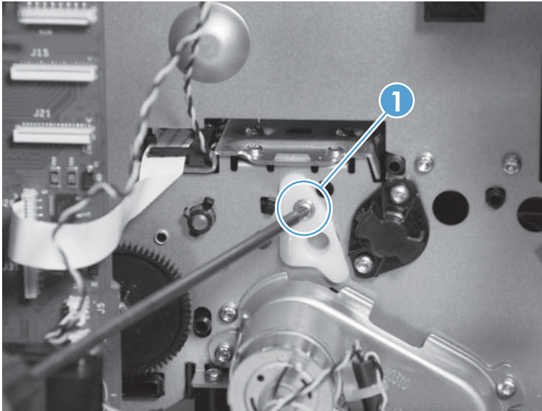
Figure 1-121 Remove the platen (4 of 7)
