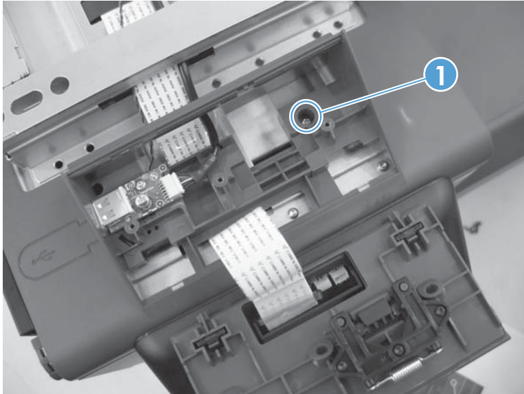
Figure 1-39 Remove the top cover and control panel (5 of 7)
