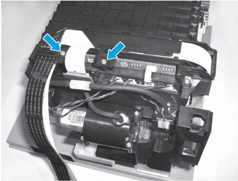
Figure 1-116 Replace the printbar control FFCs (1 of 2)
