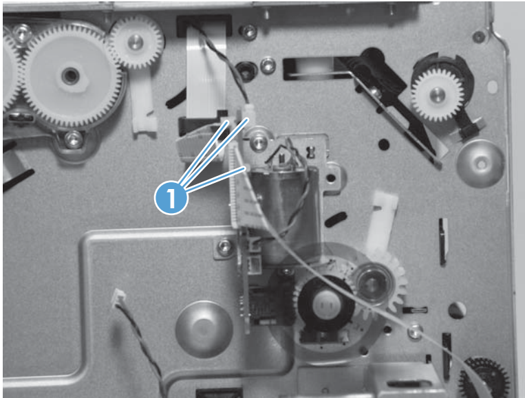
Figure 1-126 Remove the printbar lift motor (1 of 3)
