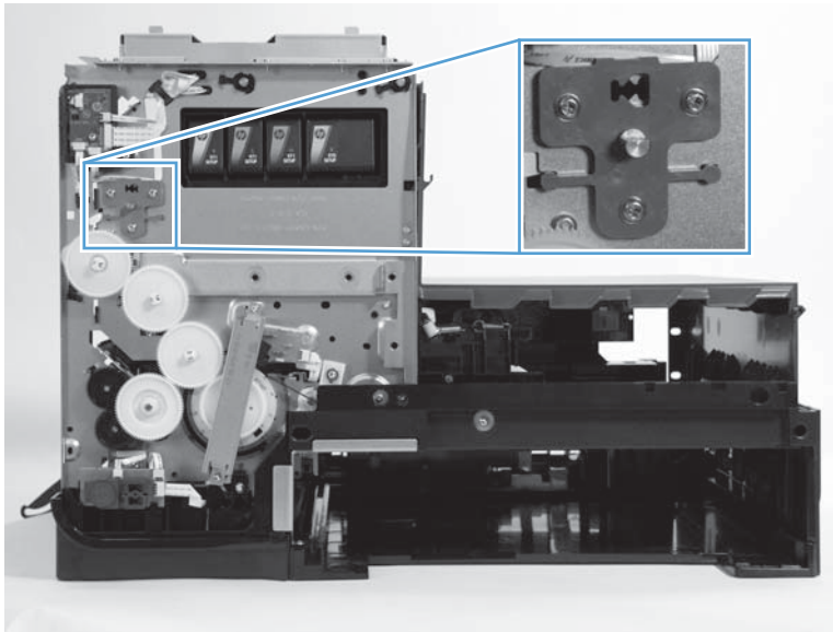
Figure 1-92 Remove the service sled assembly (1 of 6)
