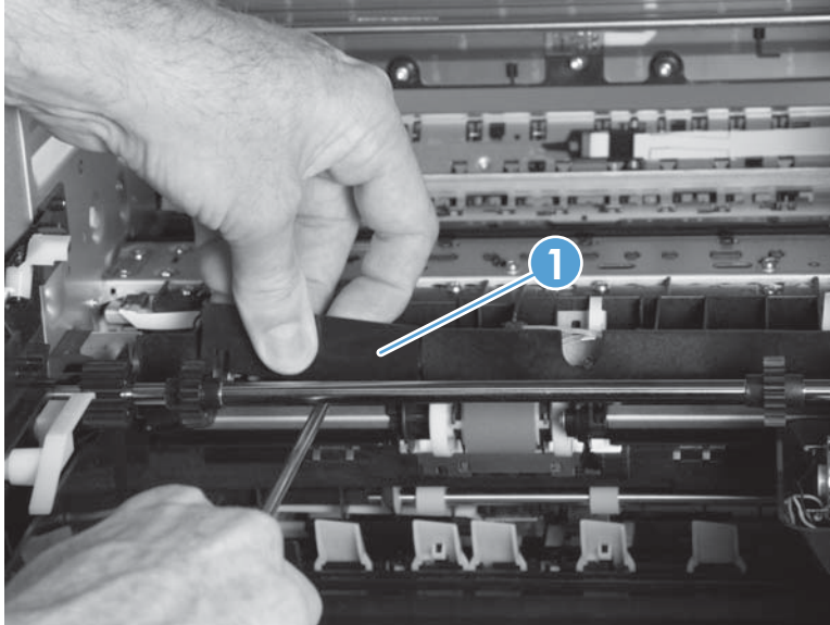
Figure 1-196 Remove the printzone distribution PCA (1 of 3)
