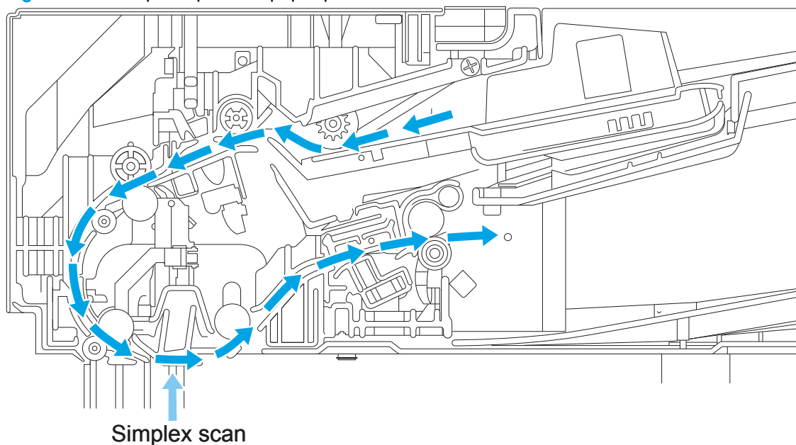
Figure 1-13 Simplex operation paper path
