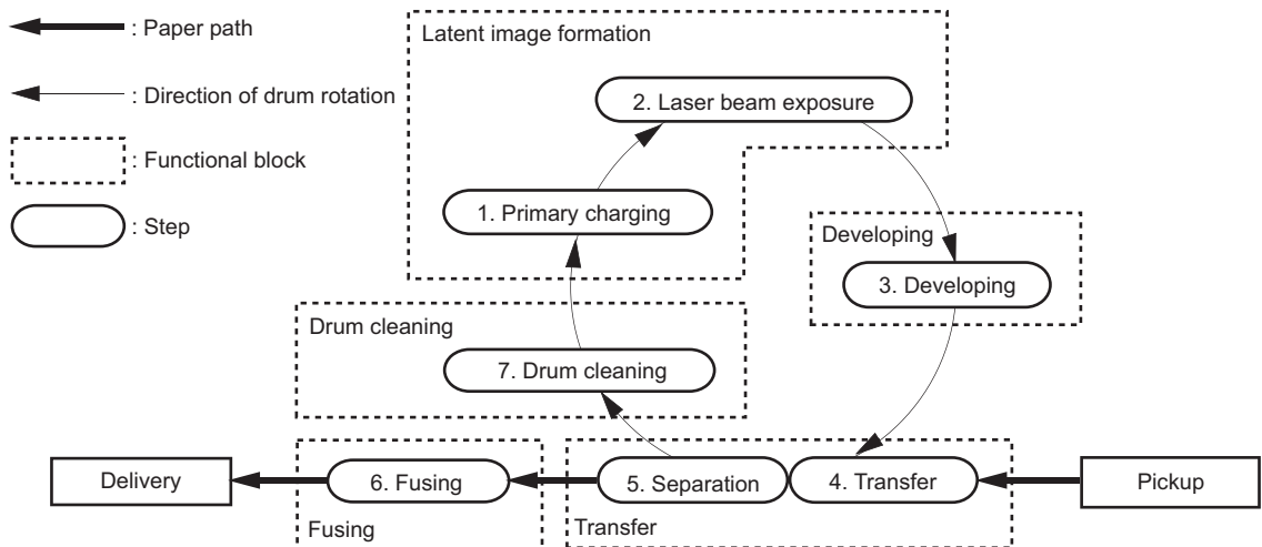
Figure 1-14 Image-formation process
