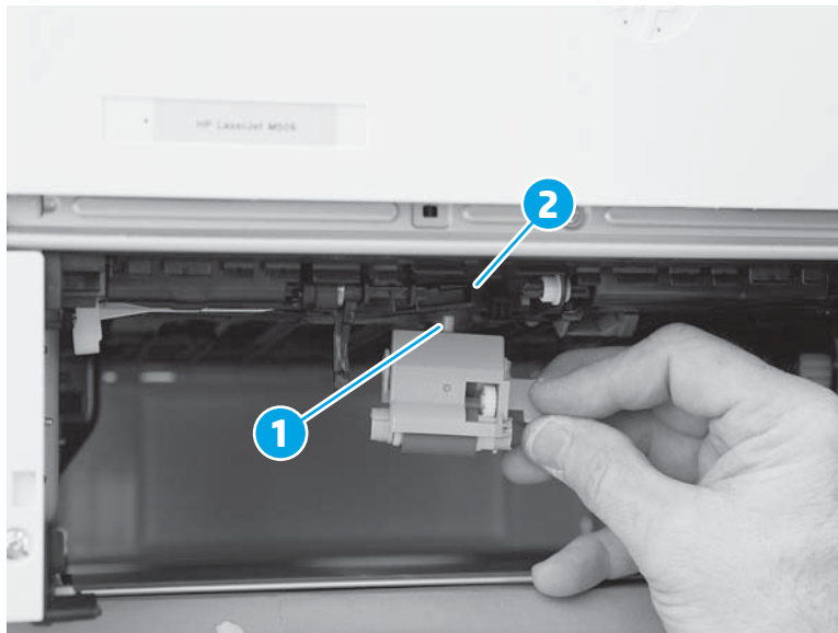
Figure 2-147 Check the pin on the assembly
