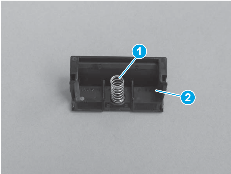
Figure 2-134 Install the spring
