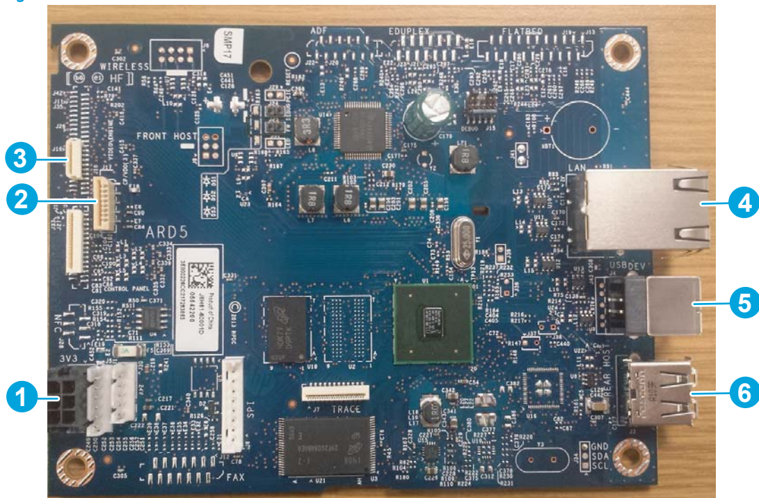
Figure 2-62 Formatter PCA M501
