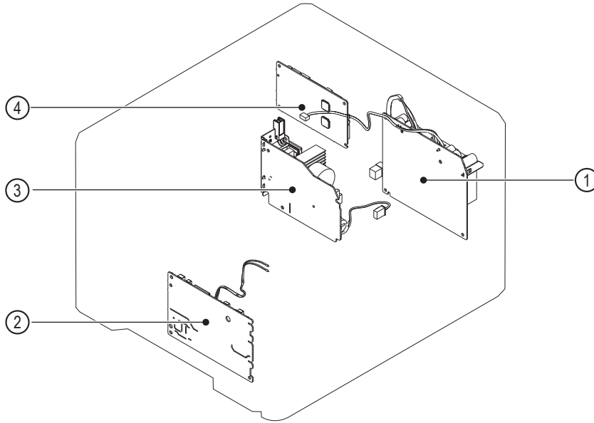
Figure 2-72 PCAs (printer base)
