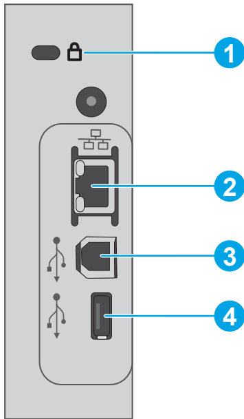
Figure 2-66 External plug and port locations (M501)
