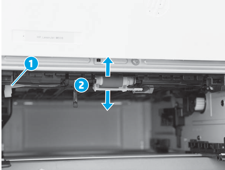
Figure 2-150 Check the installation
