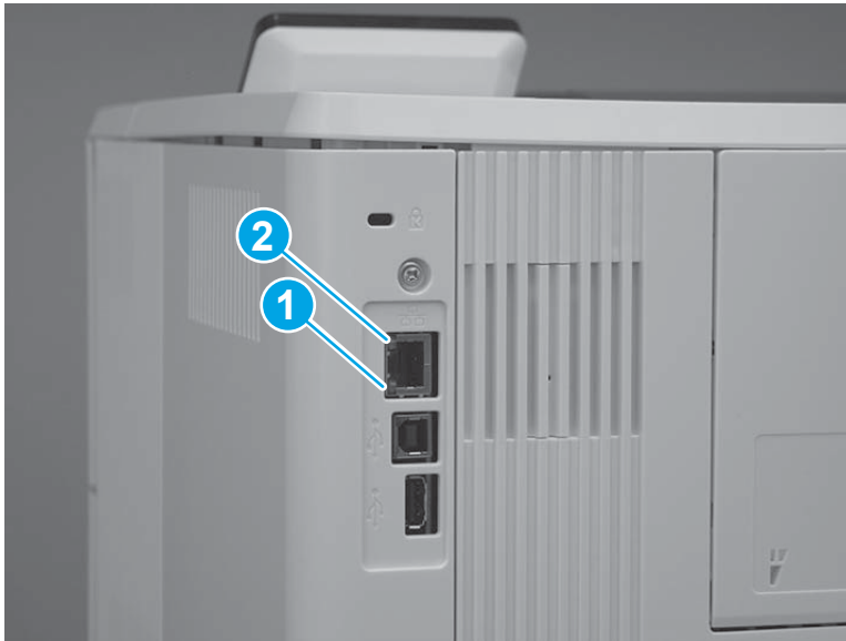
Figure 2-50 Formatter network port LEDs
