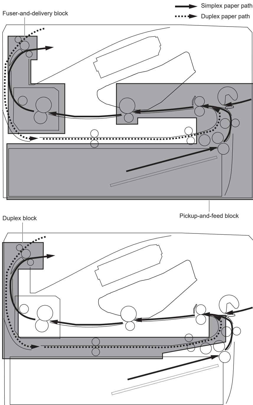
Figure 1-23 Paper handling system
