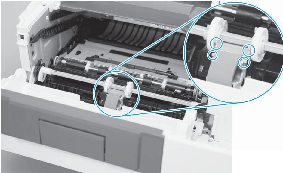
Figure 2-138 Install the roller
