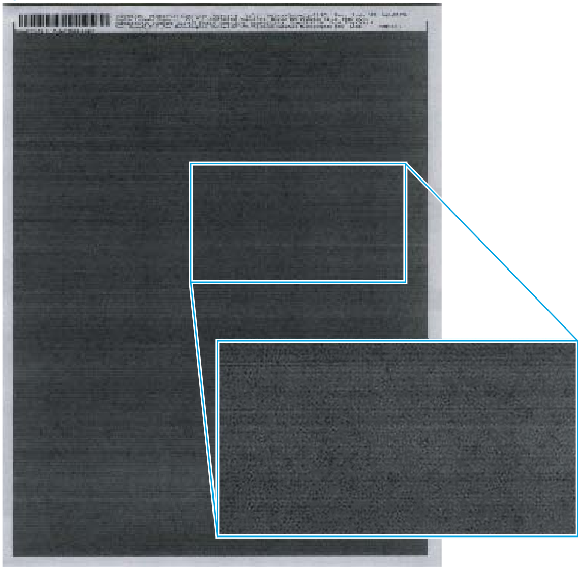
Figure 2-93 Fine-pitch banding
