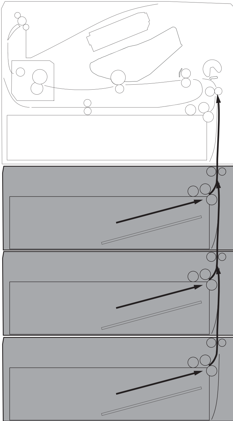
Figure 1-30 550-sheet paper feeder paper path
