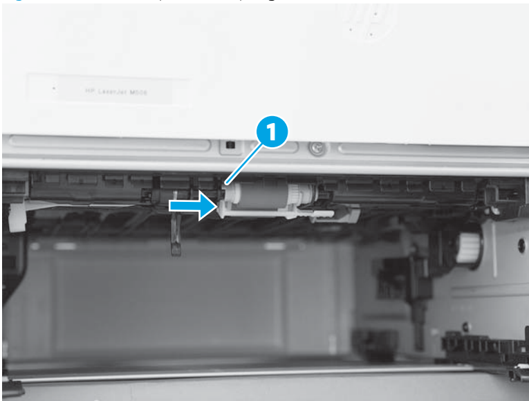
Figure 2-149 Decompress the spring-loaded shaft
