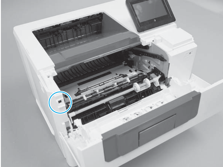
Figure 2-54 Defeat the toner cartridge door interlock
