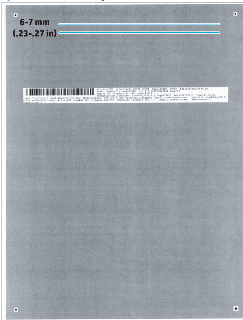
Figure 2-114 Wide-pitch banding
