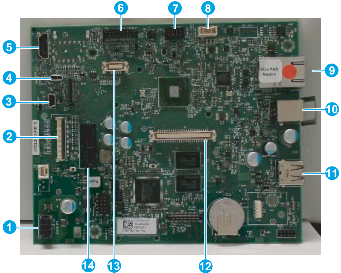
Figure 2-63 Formatter PCA (M506/E50045/M507/E50145)
