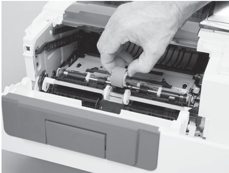
Figure 2-129 Remove the roller
