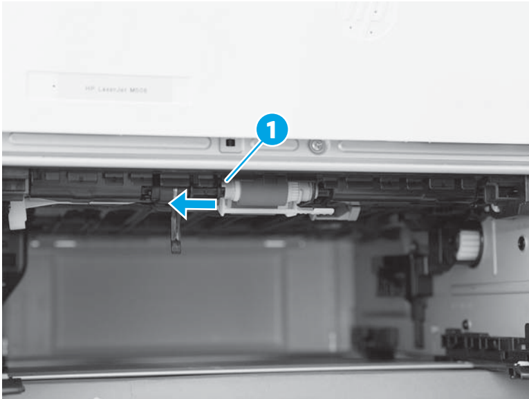
Figure 2-144 Compress the spring-loaded shaft
