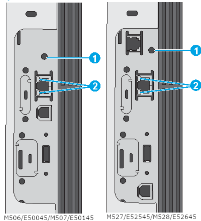
Figure 2-51 Formatter LED lights
