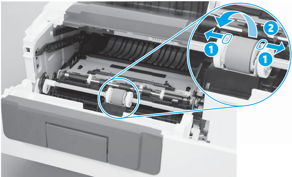
Figure 2-131 Release two tabs
