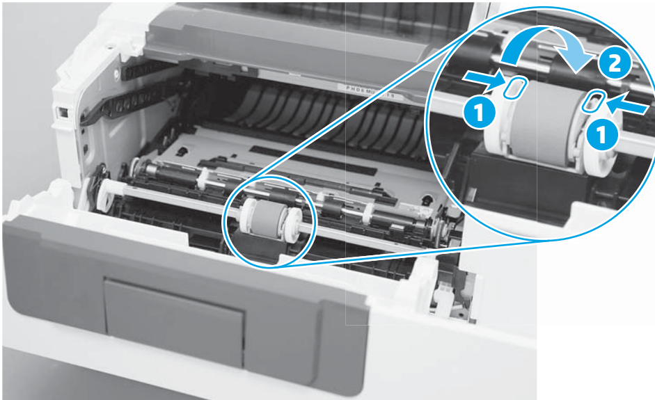
Figure 2-139 Engage two tabs
