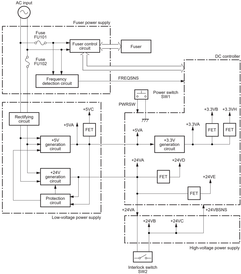
Figure 1-6 Low-voltage power-supply circuit (M506/E50045/M507/E50145, M527/E52545/M528/E52645)
