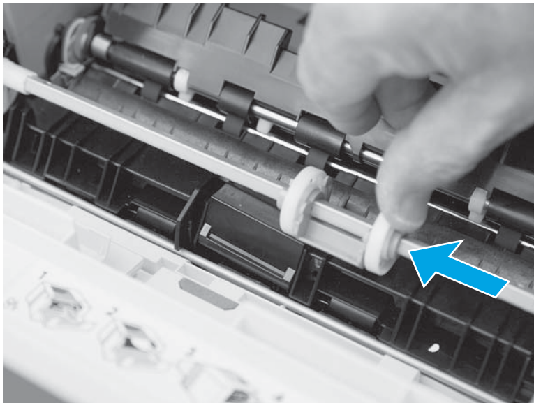
Figure 2-137 Slide the roller carriage to the left
