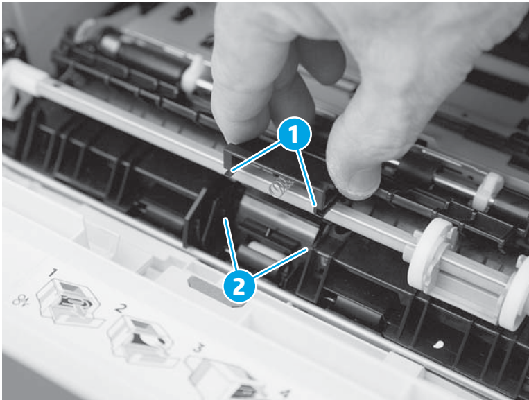
Figure 2-135 Align the assembly with the holder
