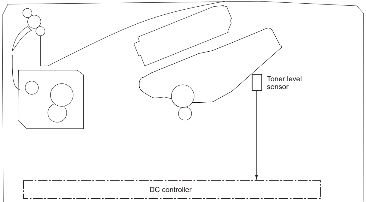
Figure 1-13 Toner-level sensor
