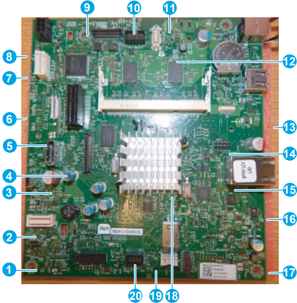
Figure 2-64 Formatter PCA M527/E52545/M528/E52645
