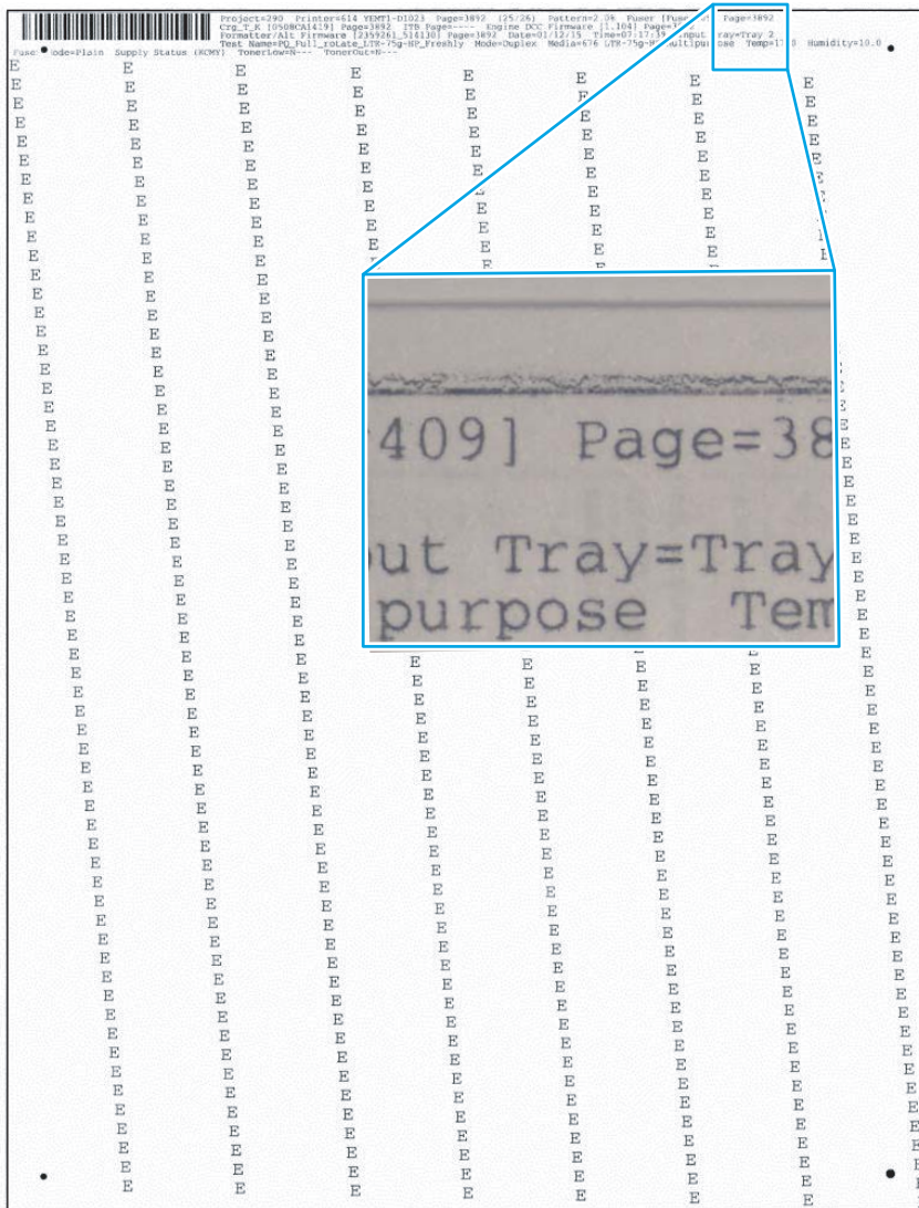
Figure 2-113 Toner in the leading edge margin (fuser slap)
