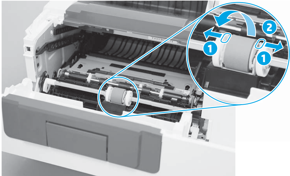
Figure 2-128 Release two tabs
