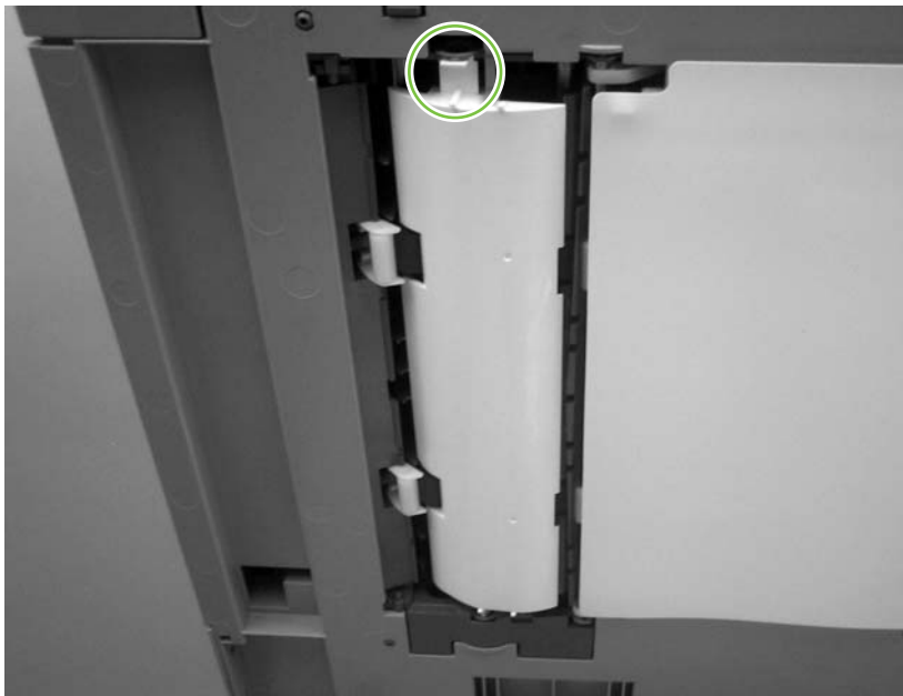
Figure 5-186 Remove the ADF white mylar-backing (3 of 3)
