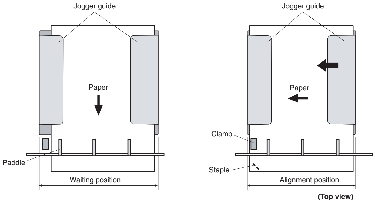
Figure 4-46 Staple-mode feed operation
