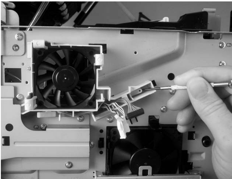
Figure 5-66 Remove the main and reversing-unit fans (8 of 9)
