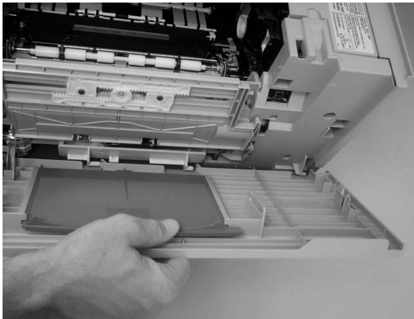
Figure 5-76 Remove the tray 1 assembly (2 of 5)
