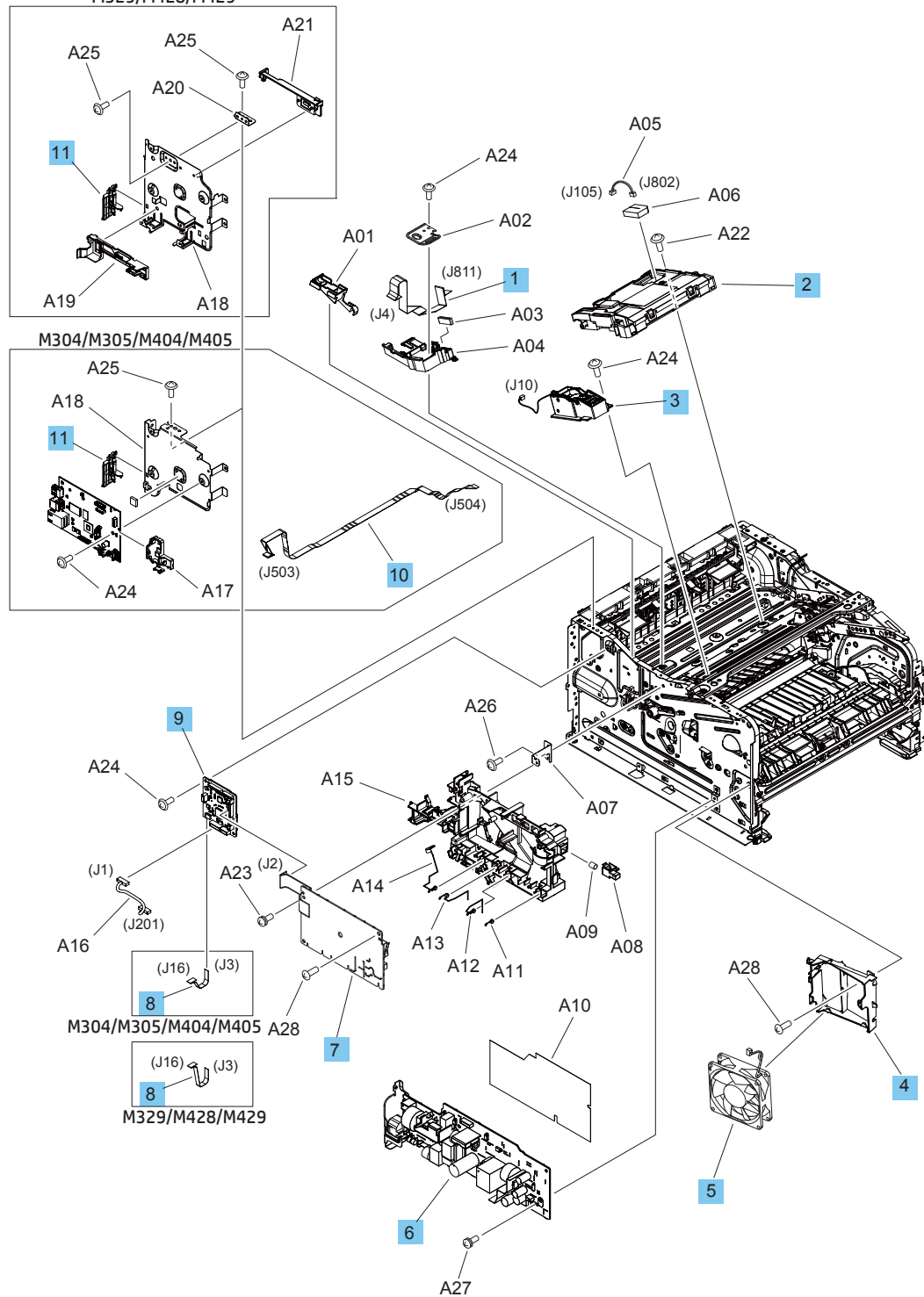
Figure 2-8 Internal components, printer base (1 of 3) M329/M428/M429
