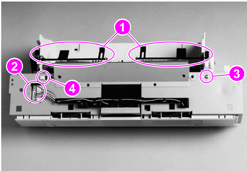
Figure 52. Delivery-fan assembly
