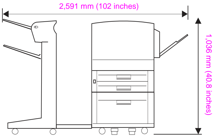
Figure 7. Space requirements with a finishing device (3,000-sheet stapler/stacker shown) and tray 4 installed
