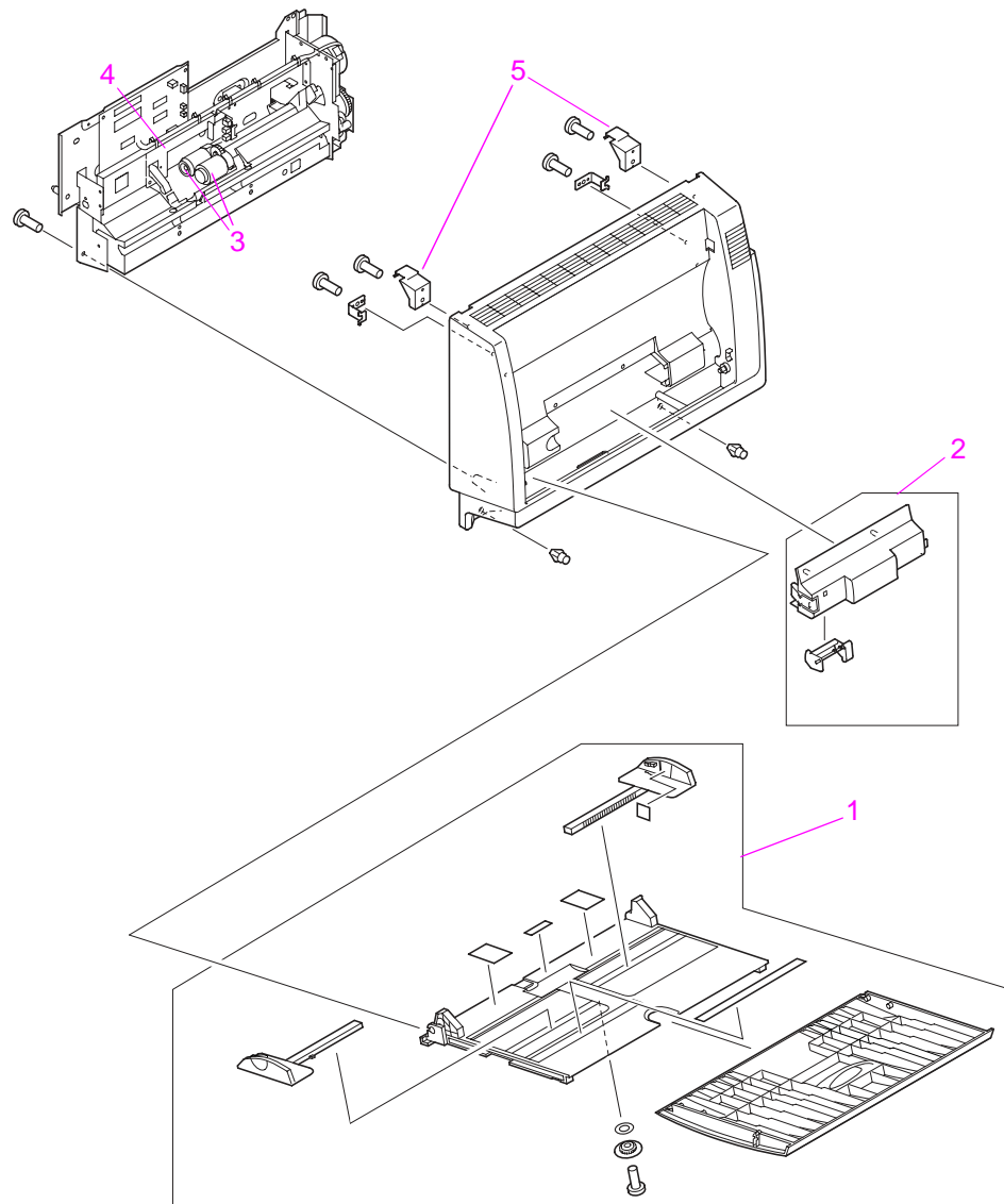
Figure 154. Tray 1 assembly
