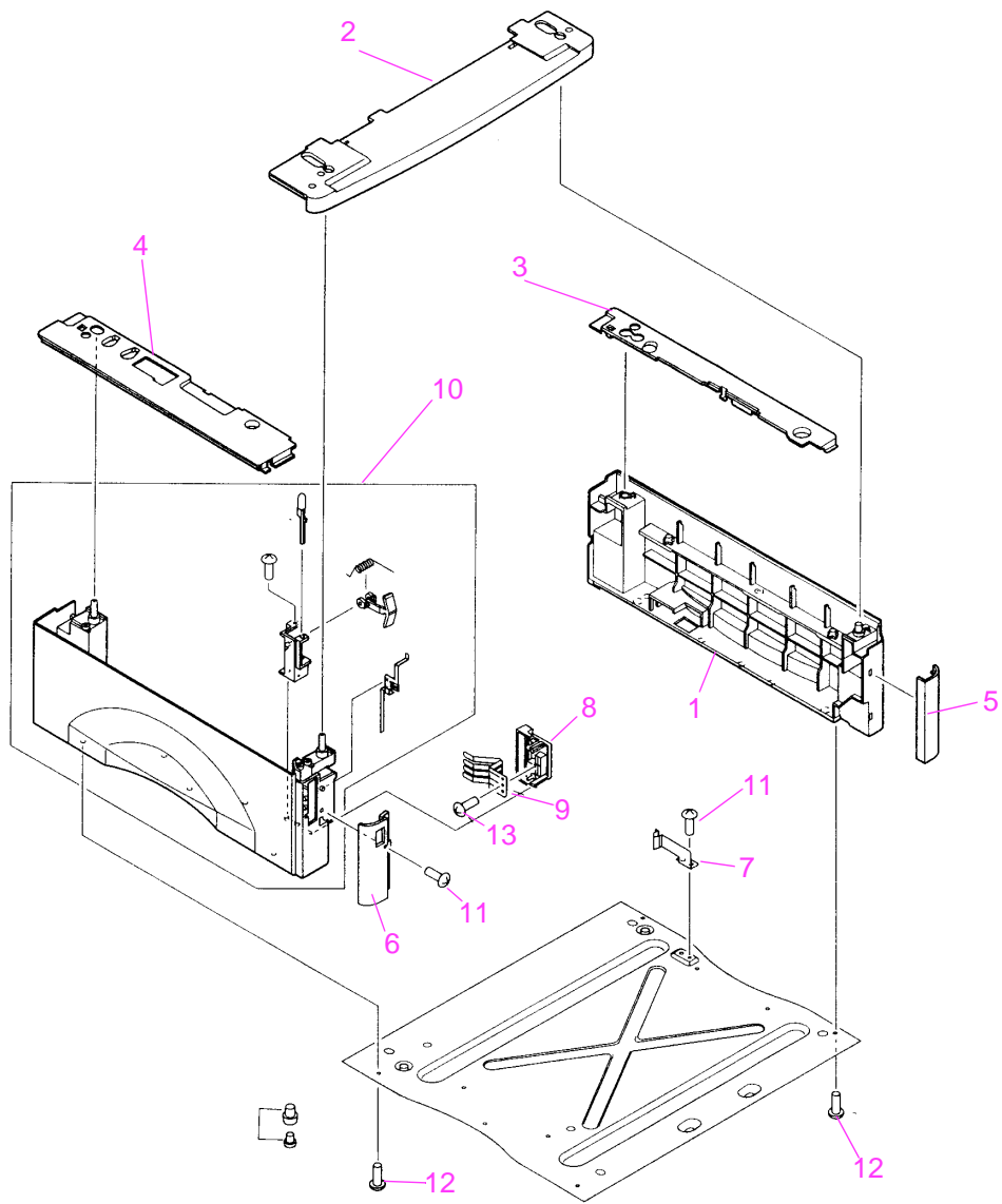
Figure 8-19 500-sheet Feeder
