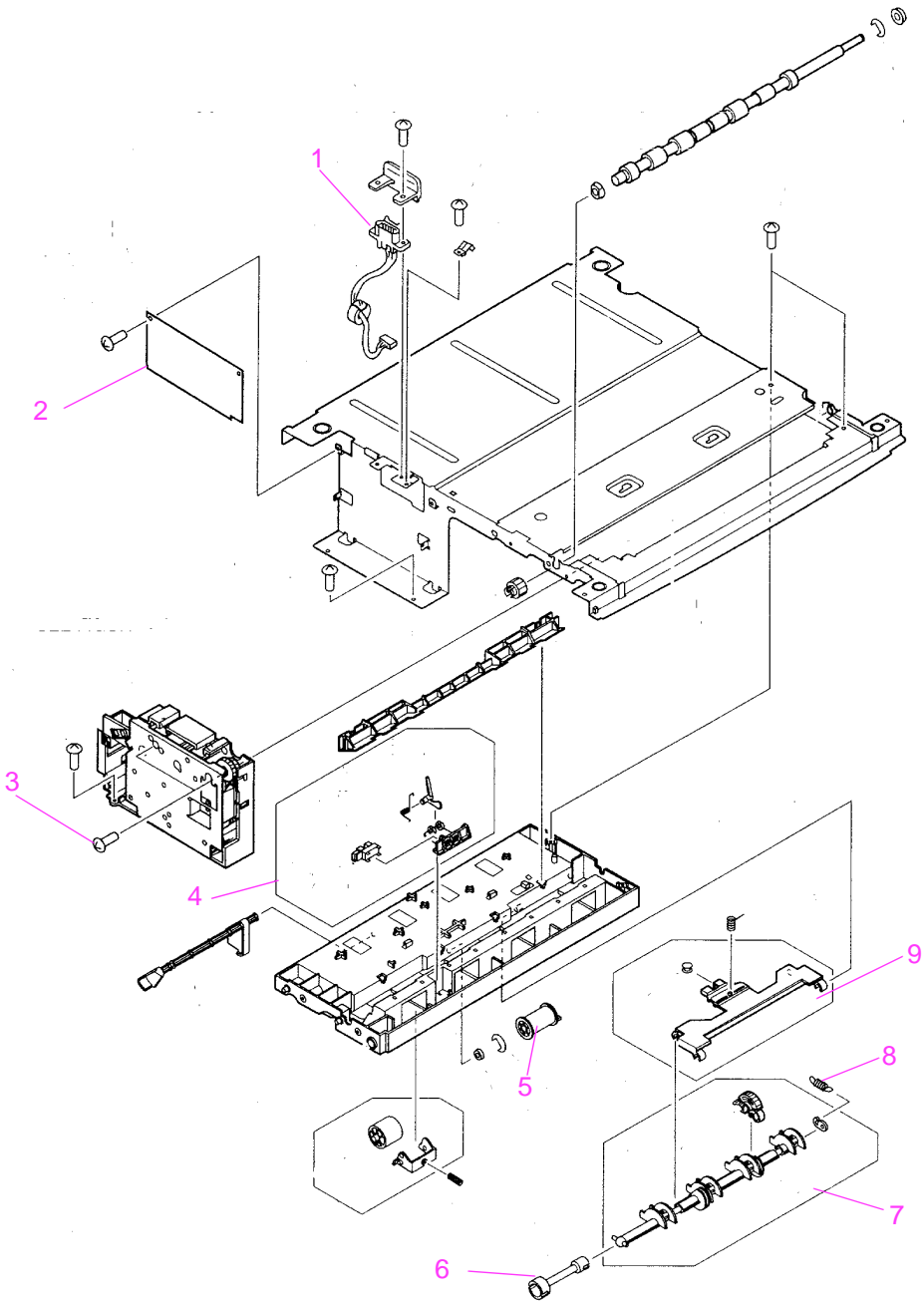
Figure 8-20 500-sheet Feeder
