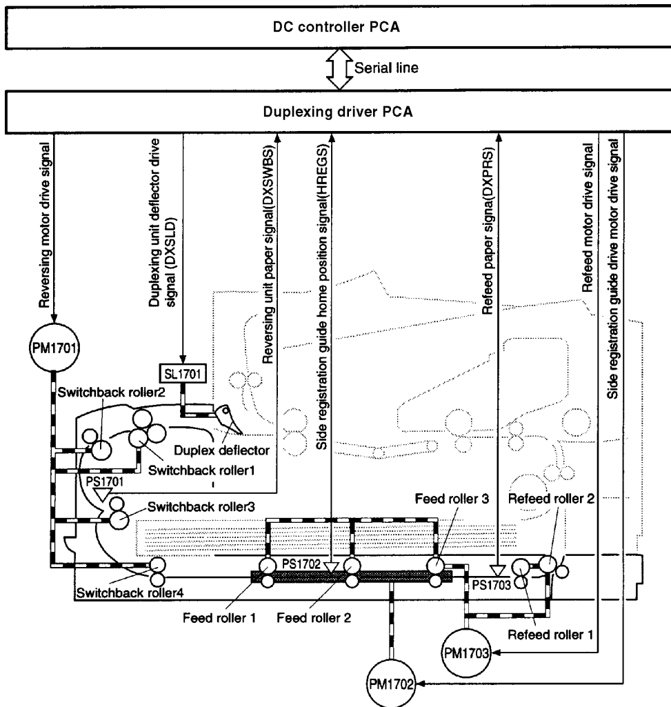
Figure 7-16 Duplexing Unit
