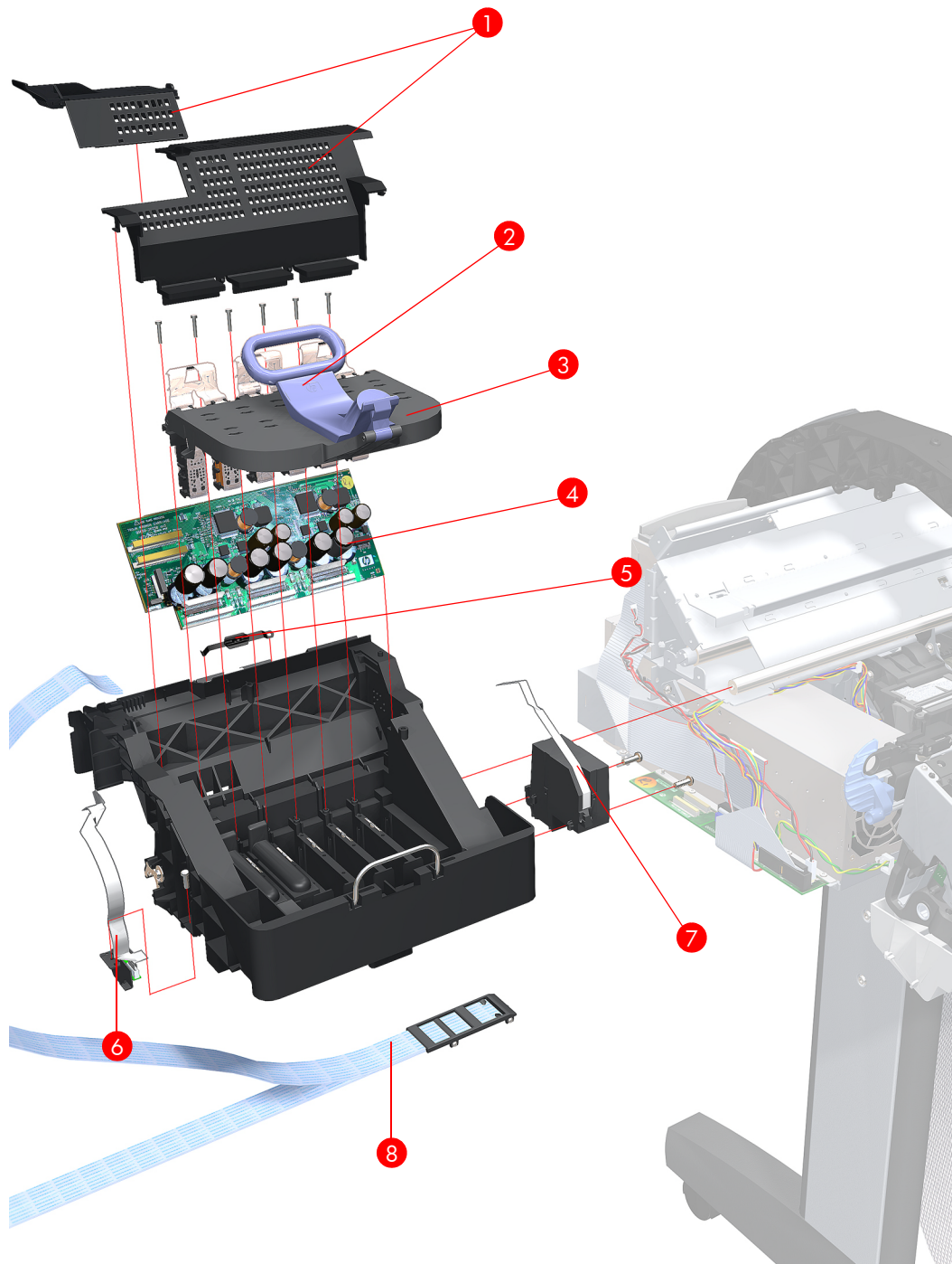
Figure 5-8: Carriage Assembly
