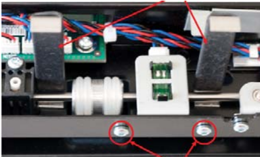
Fixing screws for Roller Sensor
