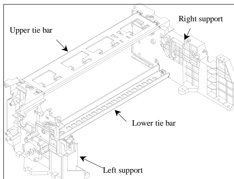
Chassis Structure
