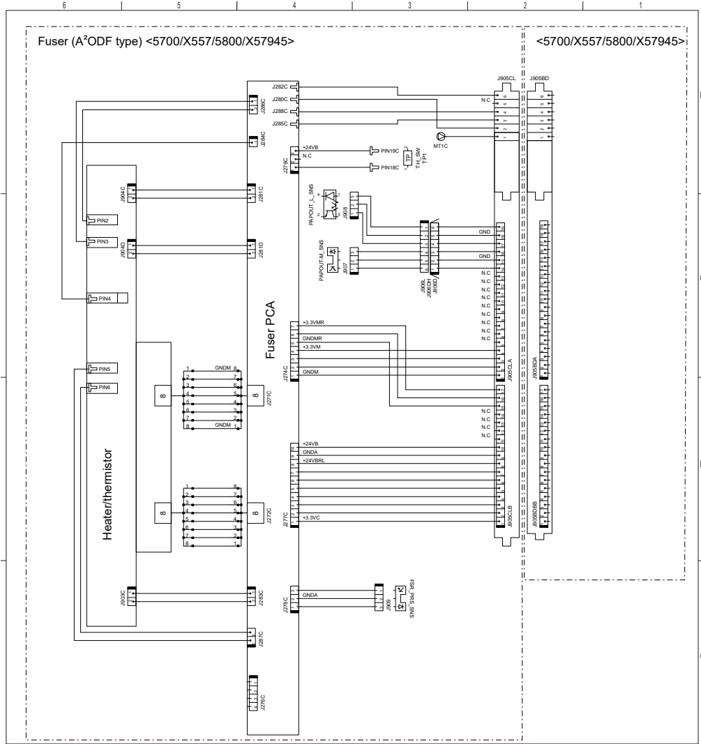
Figure 4-89 General circuit diagram, base printer (4 of 7)
