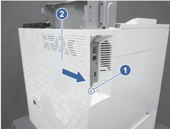
Figure 5-373 Remove the formatter cover
