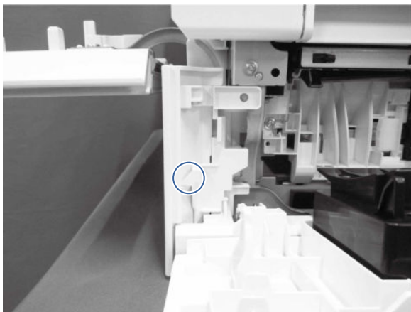
Figure 5-185 Remove the front right cover
