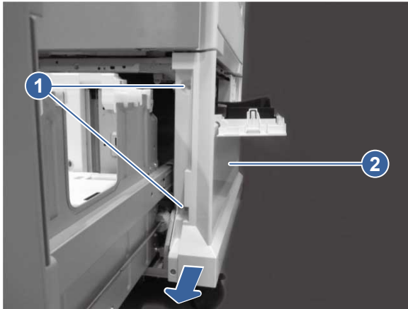
Figure 5-865 Remove the right door (HCI)
