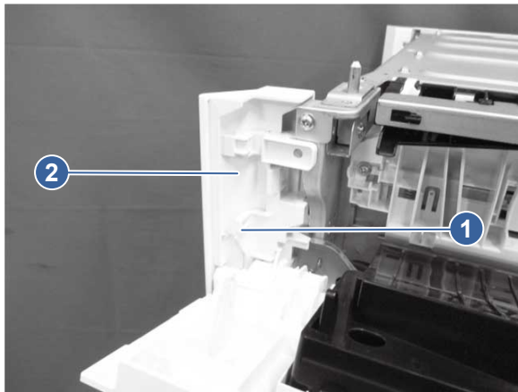
Figure 5-810 Remove the front right cover (550-sheet paper feeder)
