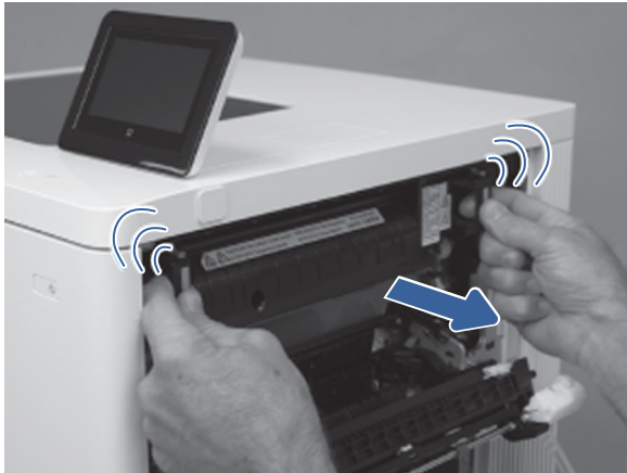
Figure 5-8 Remove the fuser
