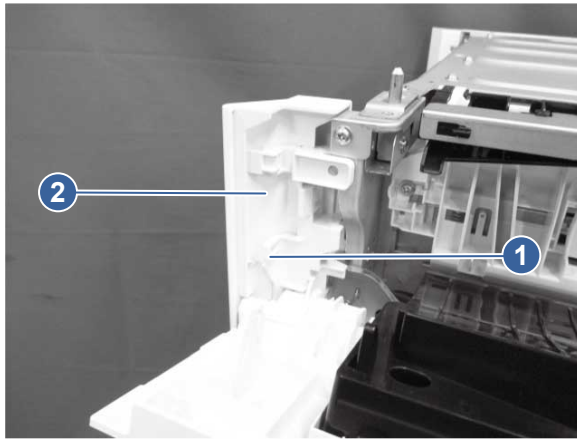
Figure 5-842 Remove the front right cover (550-sheet paper feeder)
