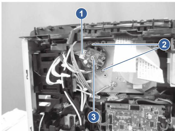
Figure 5-763 Remove the motor
