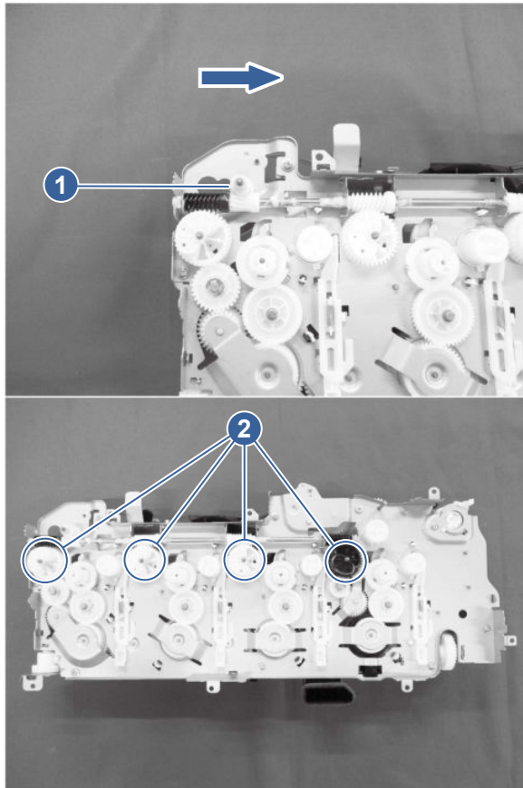
Figure 5-470 Align the gears
