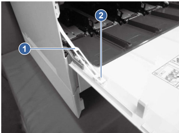
Figure 5-591 Release the left link arm
