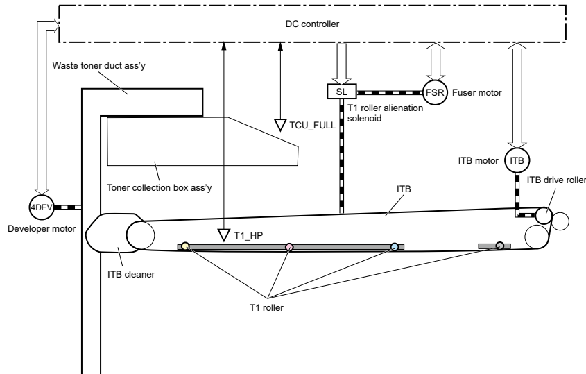
Figure 3-25 ITB unit
