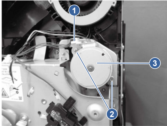
Figure 5-469 Remove the motor
