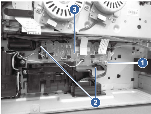
Figure 5-692 Remove the rear PCA
