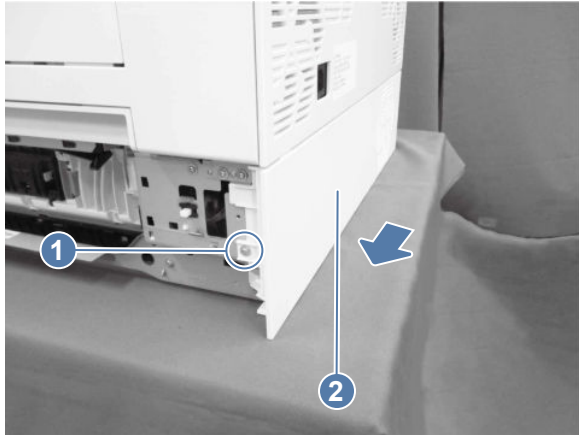
Figure 5-401 Remove the rear lower cover
