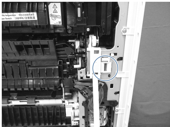
Figure 4-50 Defeat the right door interlock
