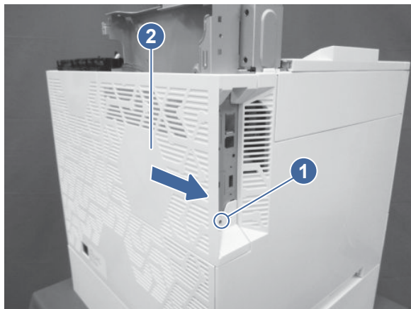
Figure 5-145 Remove the formatter cover
