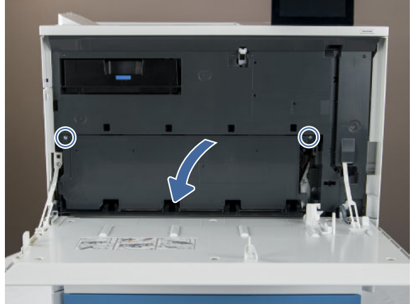
Figure 2-4 Remove two screws, open the cover
