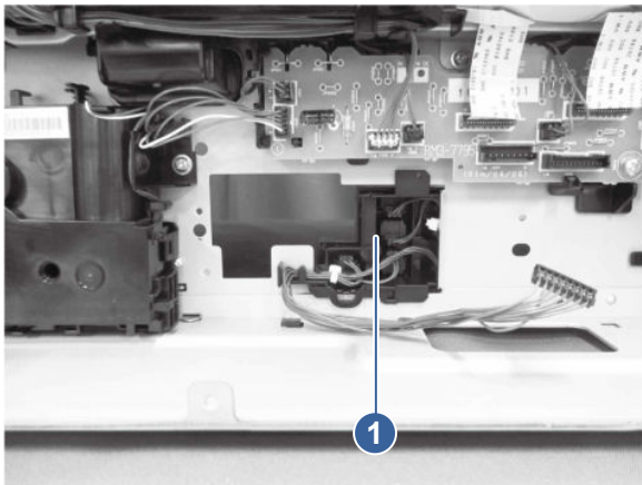
Figure 5-414 Remove the Tray 2 media size detect assembly
