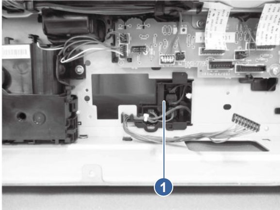
Figure 5-413 Remove the Tray 2 media size detect assembly
