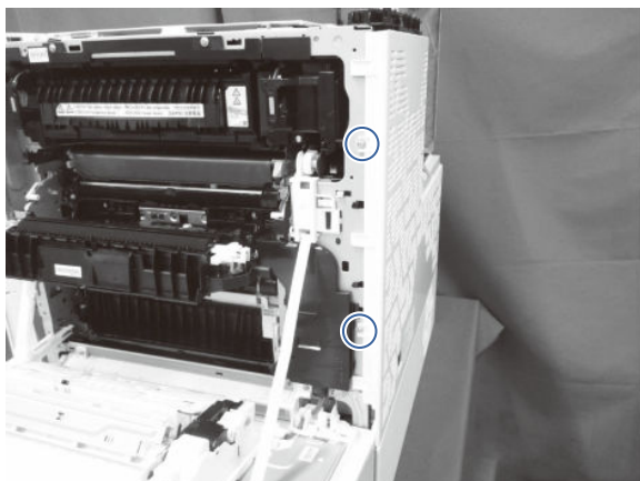
Figure 5-374 Remove two screws
