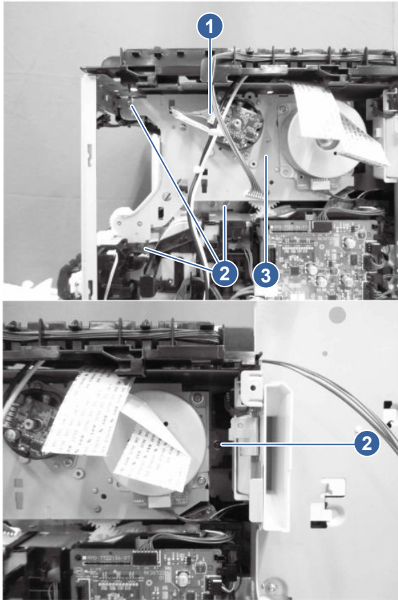
Figure 5-437 Remove the assembly
