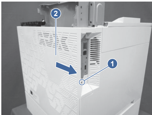
Figure 5-707 Remove the formatter cover
