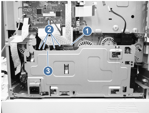
Figure 5-448 Disconnect the LVPS connectors
