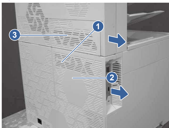
Figure 5-924 Remove the 3-bin stapler-stacker formatter cover
