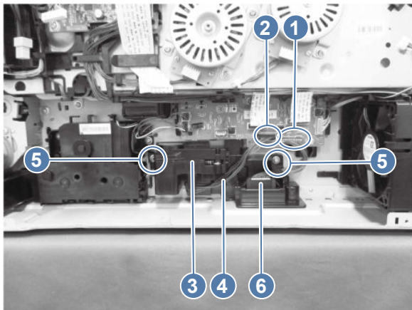
Figure 5-412 Remove the auto close assembly
