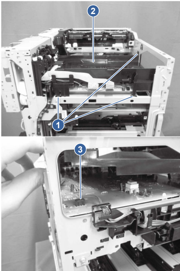
Figure 5-579 Release three tabs
