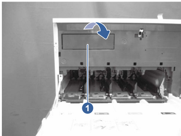
Figure 5-655 Remove the TCU cover
