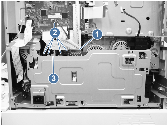
Figure 5-351 Disconnect the LVPS connectors
