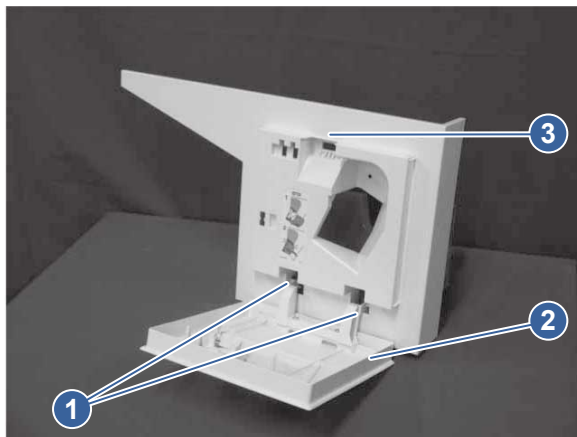
Figure 5-999 Remove the staple door from the staple cover
