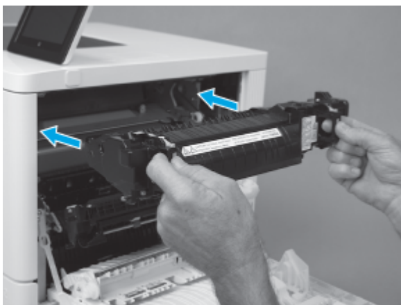
Figure 5-9 Align the fuser with the opening
