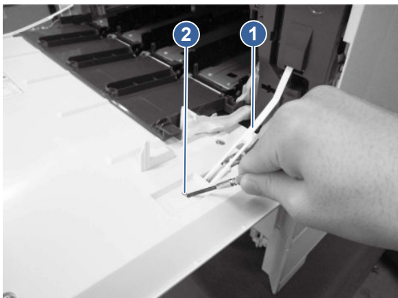
Figure 5-592 Release the right link arm
