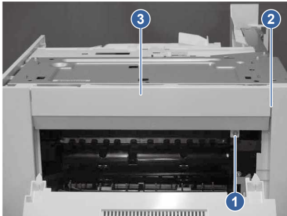
Figure 5-1000 Remove the 3-bin stapler-stacker right upper cover
