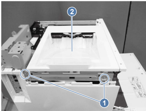
Figure 5-567 Remove the output bin
