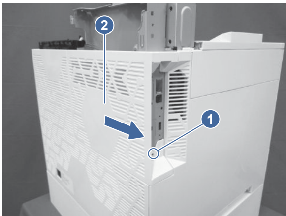
Figure 5-723 Remove the formatter cover
