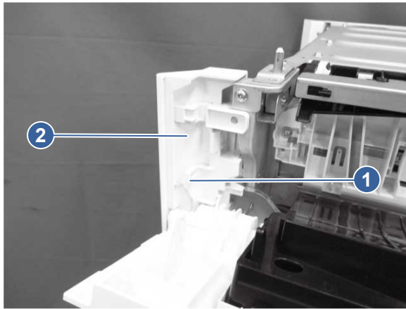
Figure 5-817 Remove the front right cover (550-sheet paper feeder)
