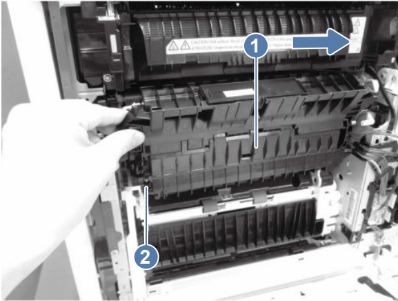
Figure 5-642 Remove the secondary transfer assembly
