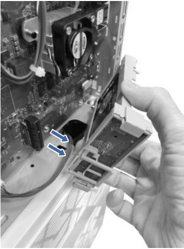
Figure 5-95 Remove the HDD
