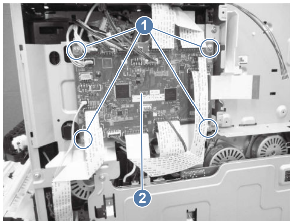
Figure 5-521 Remove the DC controller
