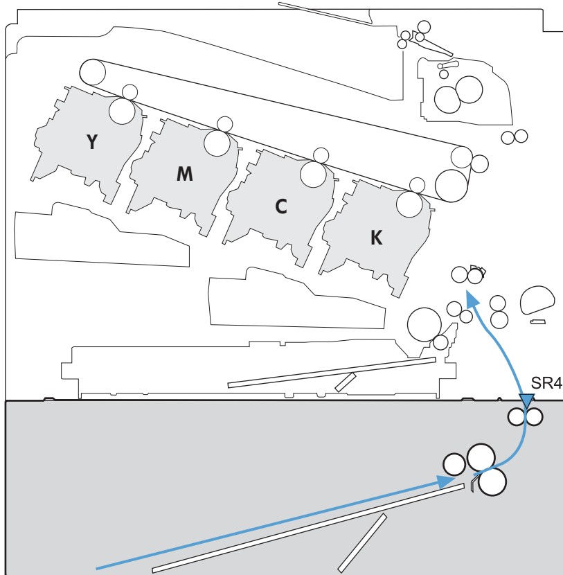
Figure 1-50 Jam detection
