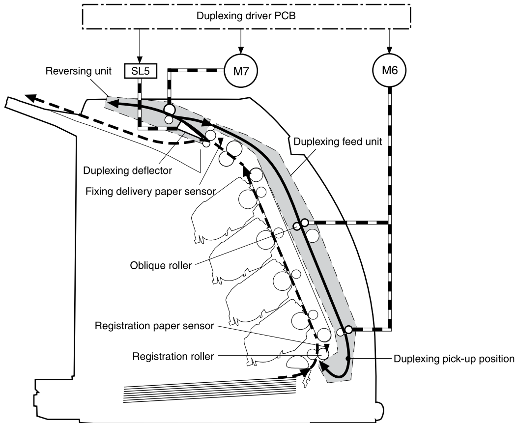
Figure 4-19 Duplexing components
