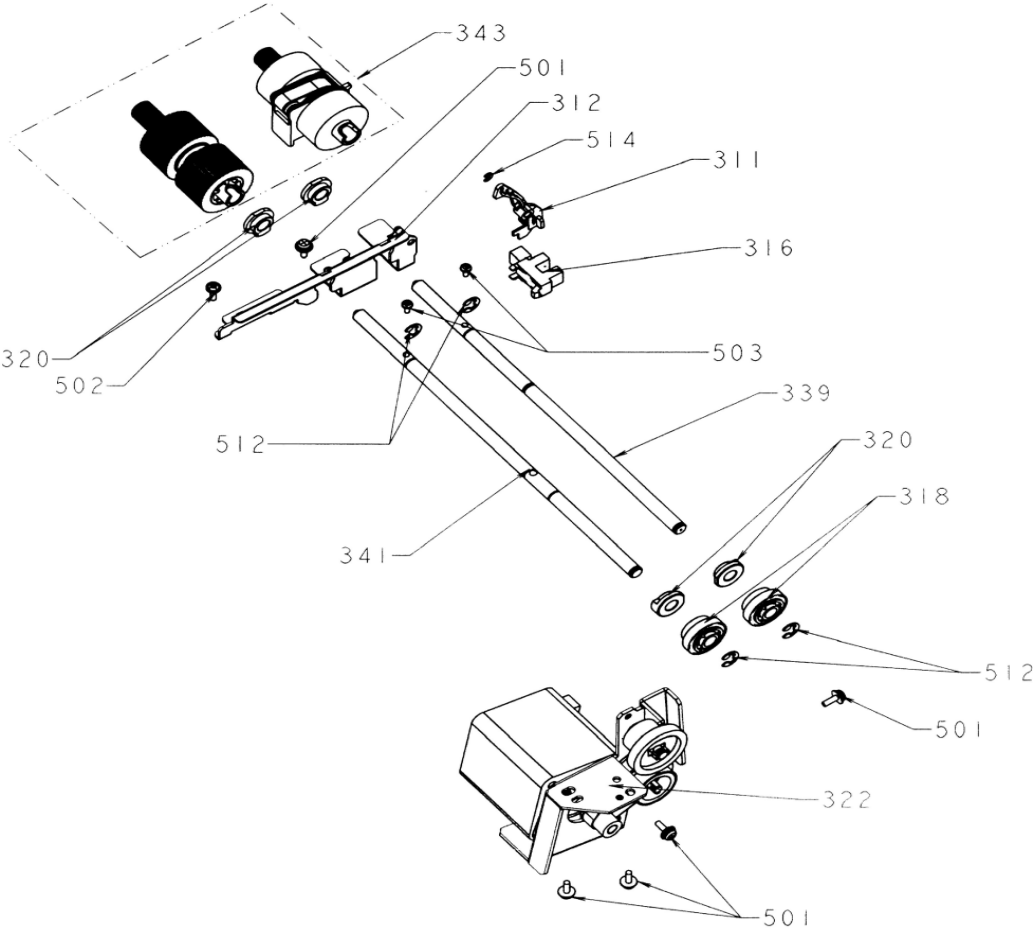
Figure 17 ADF UNIT LOWER PART (3/3)
