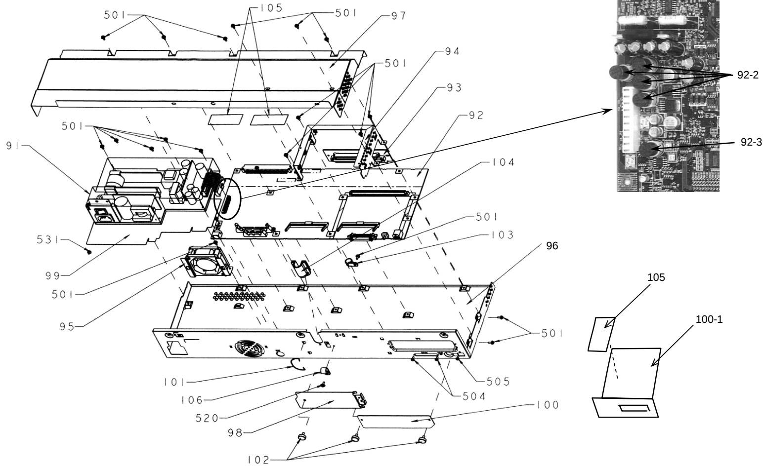
Figure 6 PCA UNIT
