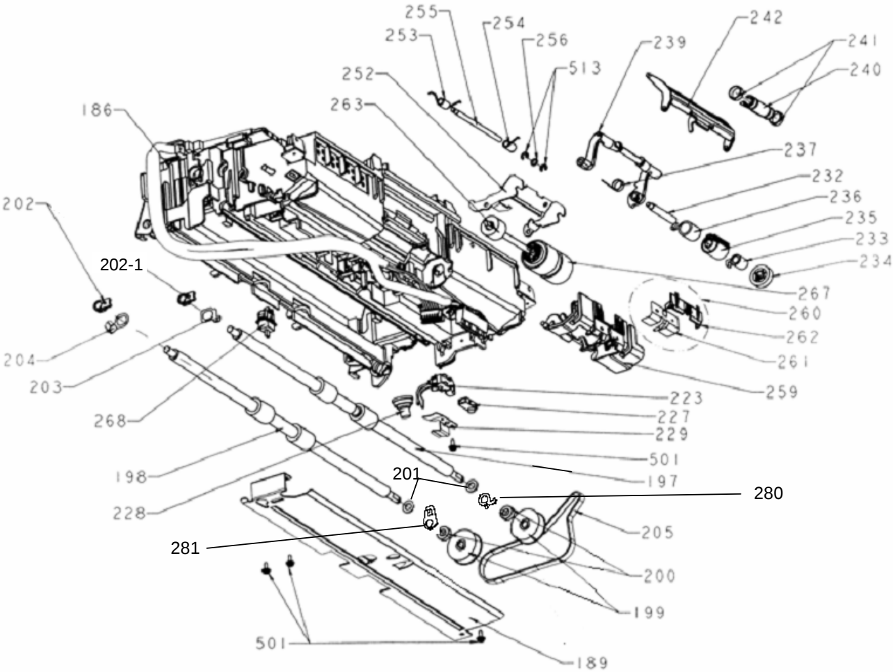
Figure 14 ADF UNIT UPPER PART (2/2)
