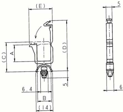
Fig. 10 CABLE CLAMP (1/5)
