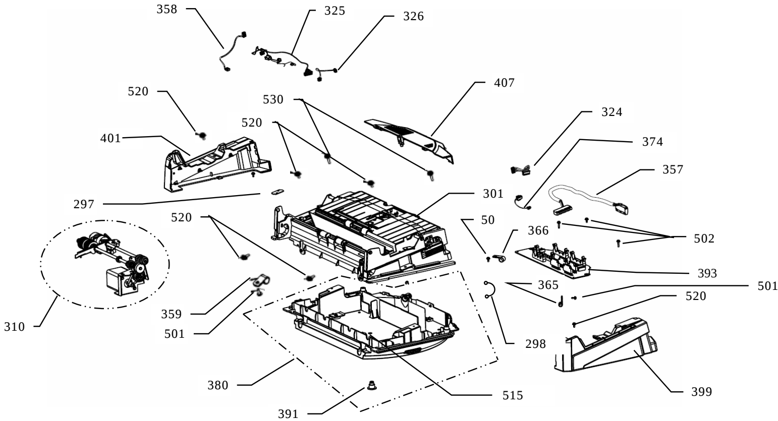
Figure 15 ADF UNIT LOWER PART (1/3)
