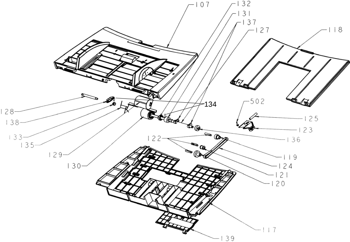
Figure 9 CHUTE ASSEMBLY (1/2)
