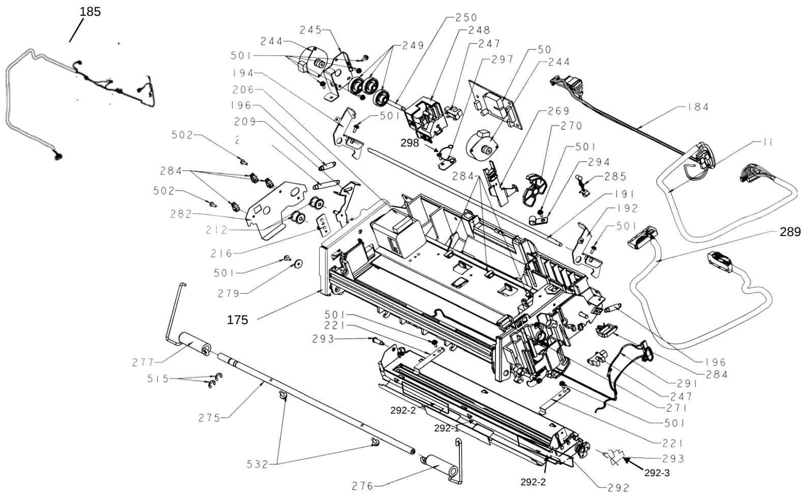
Figure 13 ADF UNIT UPPER PART (1/2)
