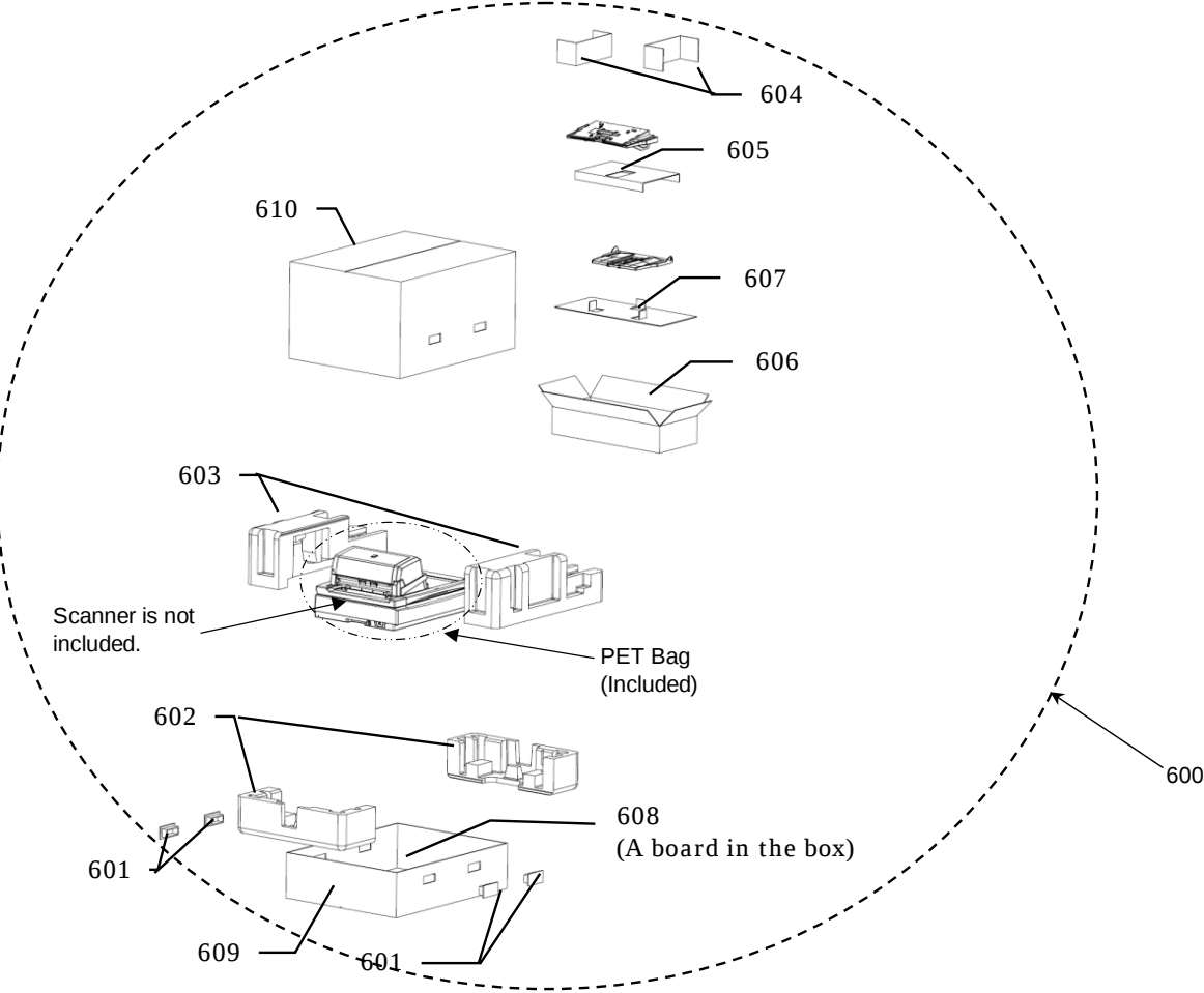
Figure 18 PACKAGING BOX
