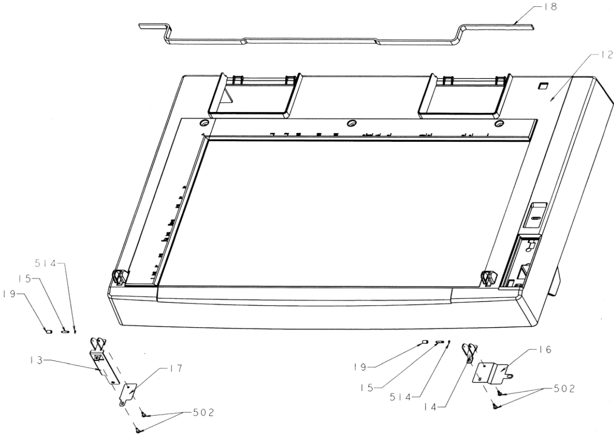
Figure 3 FB COVER
