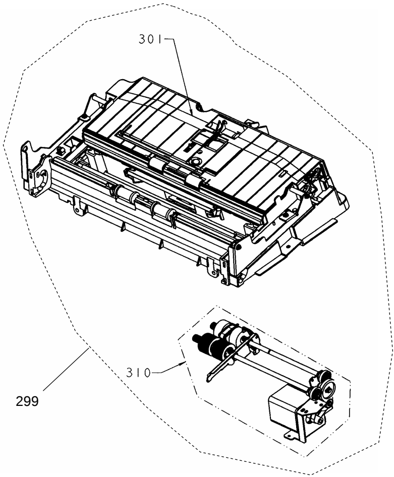
Figure 14 ADF UNIT LOWER PART (1/3)
