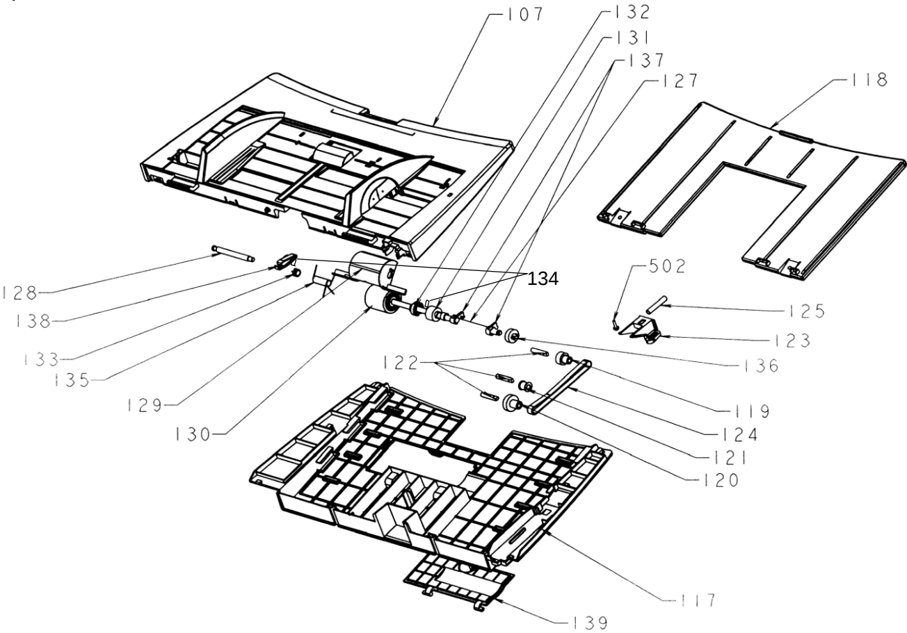
Figure 8 CHUTE ASSEMBLY (1/2)
