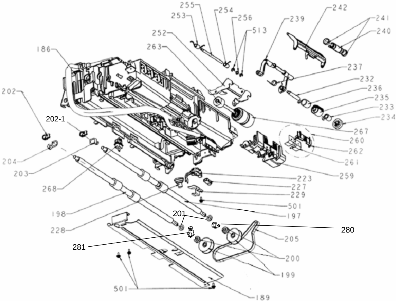
Figure 13 ADF UNIT UPPER PART (2/2)
