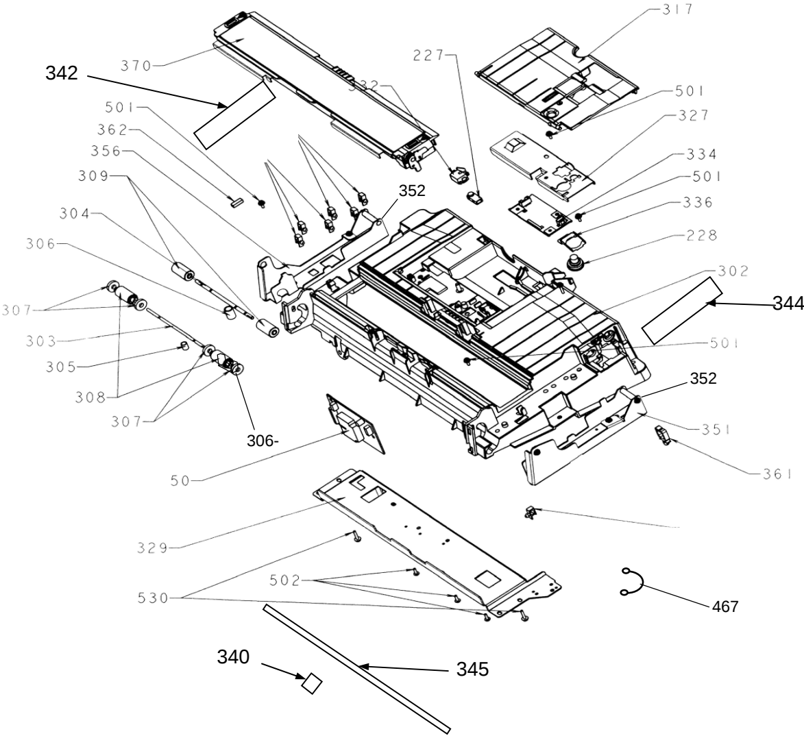
Figure 15 ADF UNIT LOWER PART (2/3)
