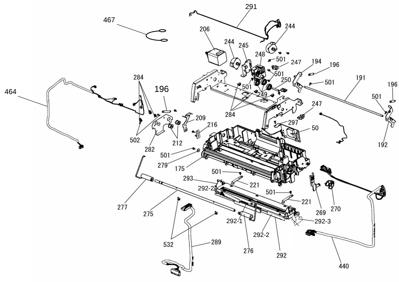
Figure 12 ADF UNIT UPPER PART (1/2)
