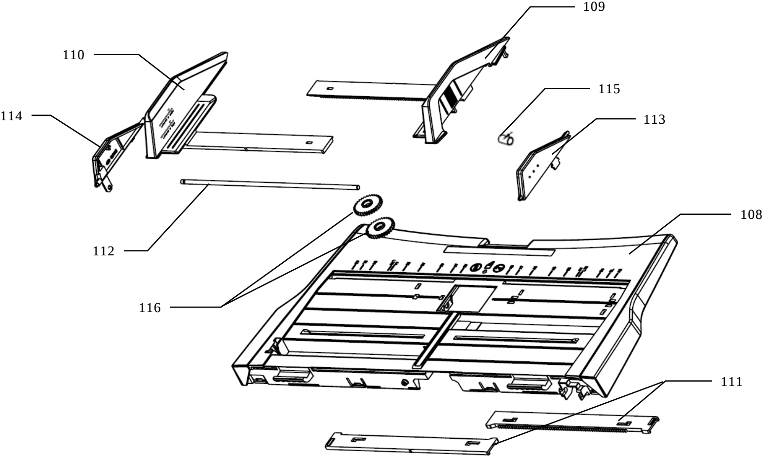
Figure 9 CHUTE ASSEMBLY (2/2)
