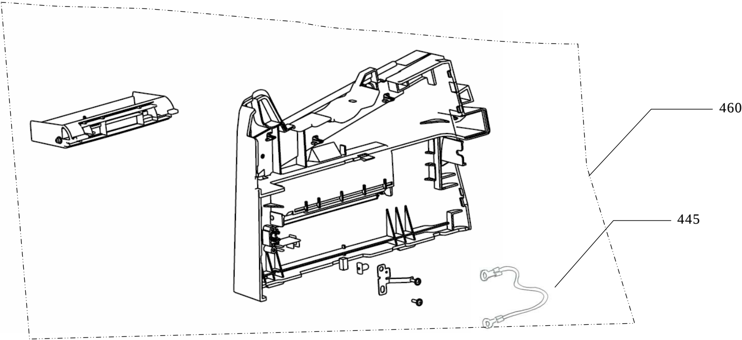
Figure 6 REAR COVER
