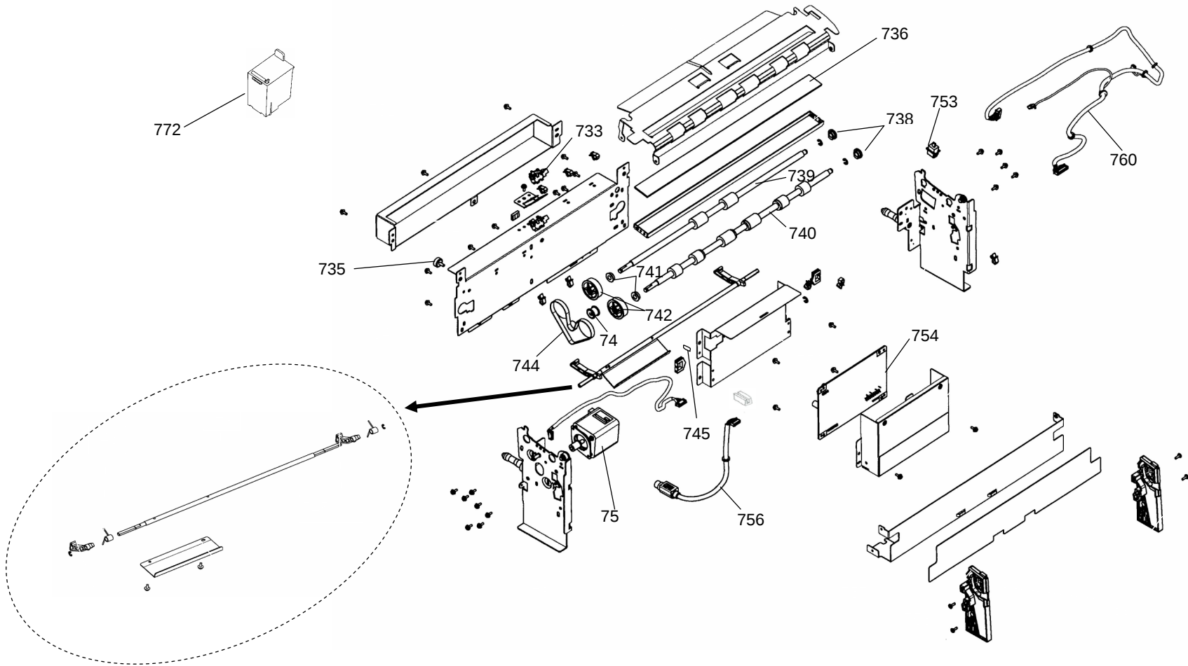
Figure 20 IMPRINTER (2/2)
