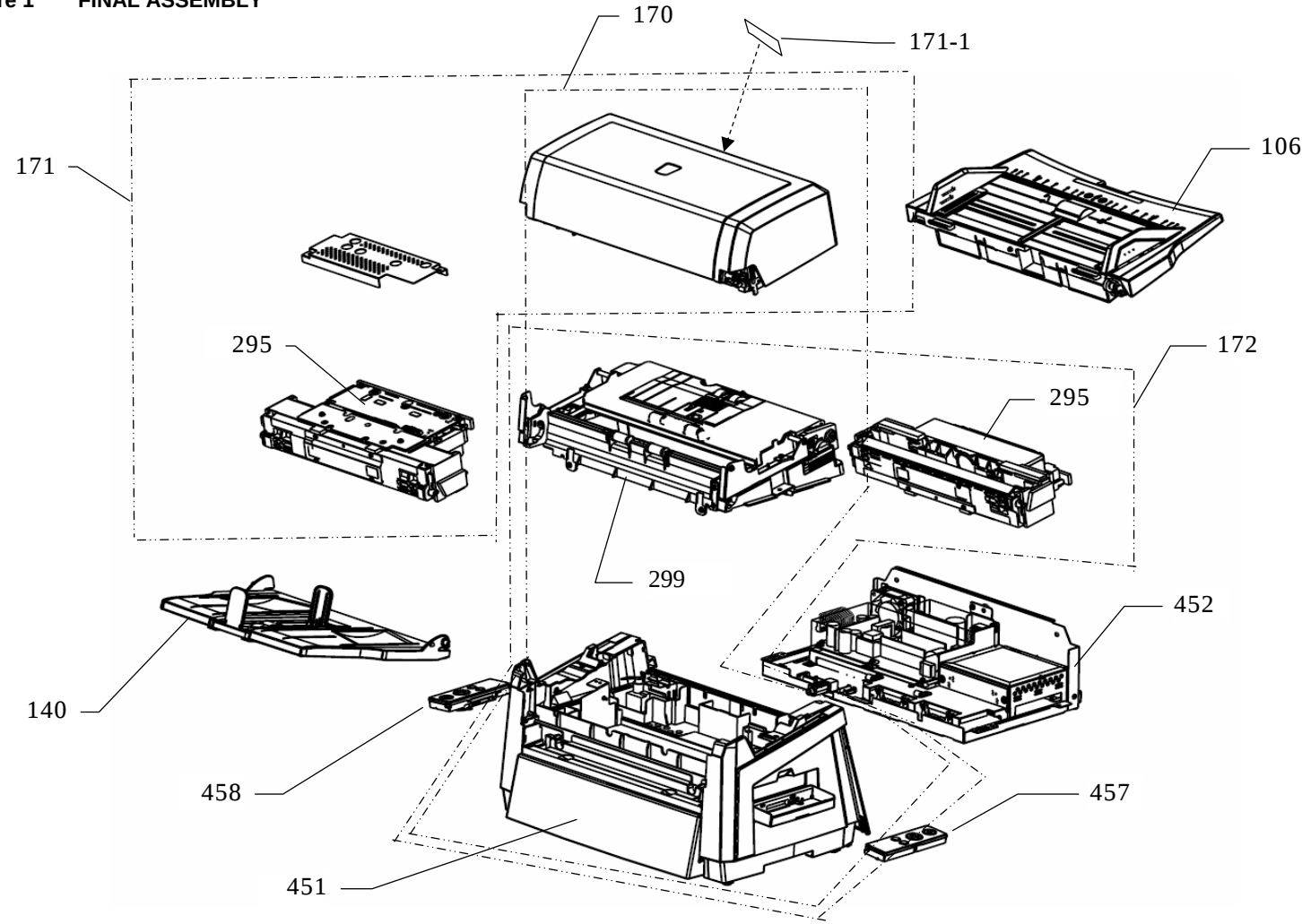
Figure 1 FINAL ASSEMBLY
