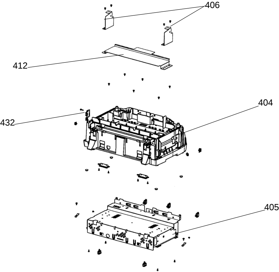
Figure 4 BASE UNIT
