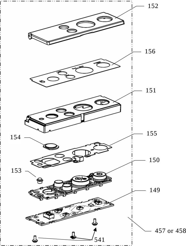
Figure 7 PANEL UNIT
