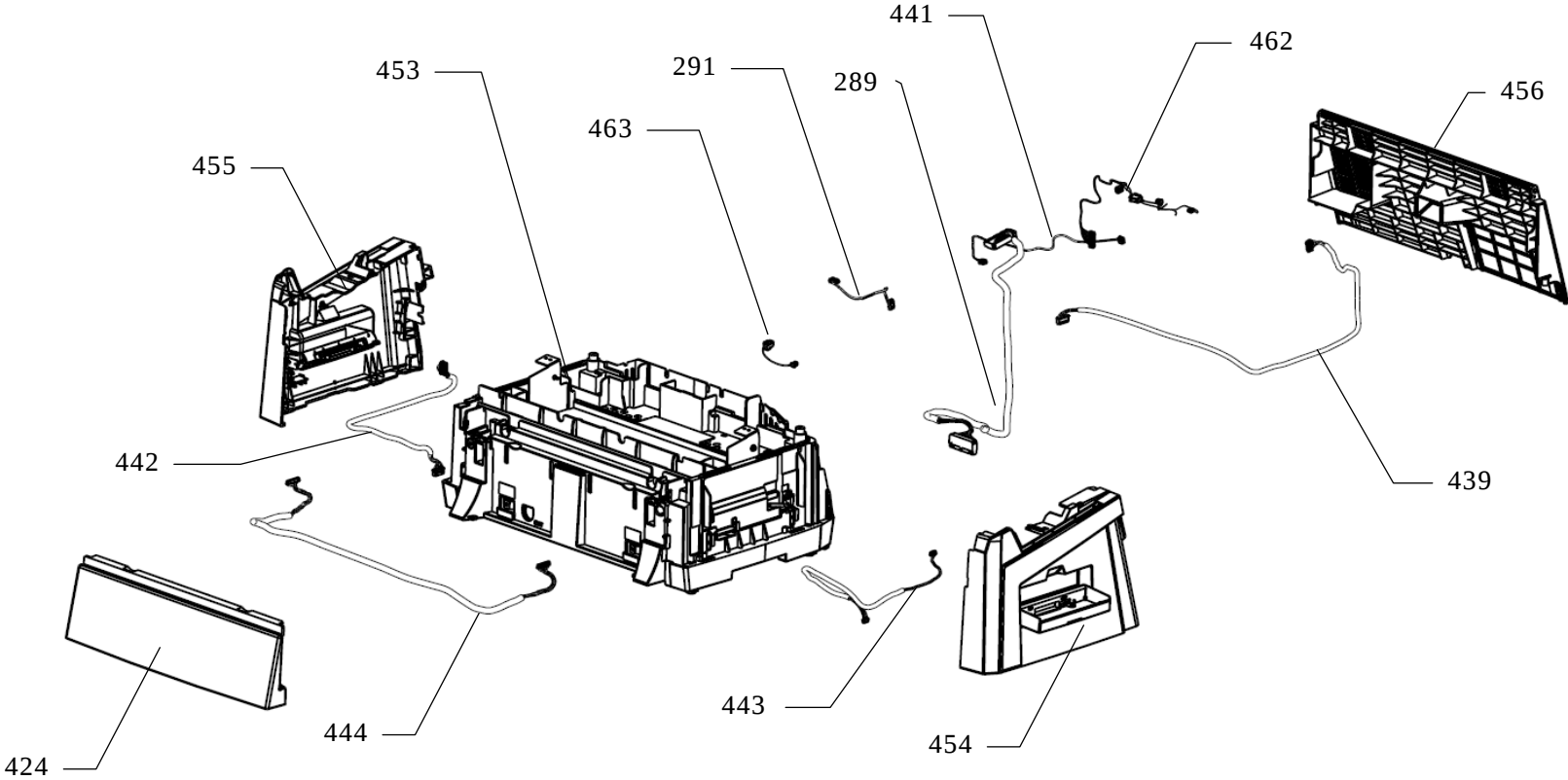
Figure 2 BASE SECTION
