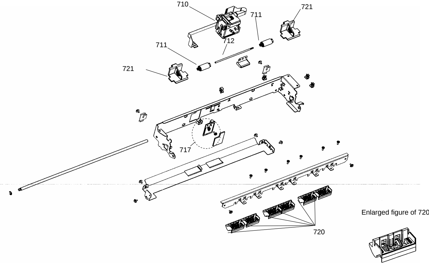
Figure 19 IMPRINTER (1/2)
