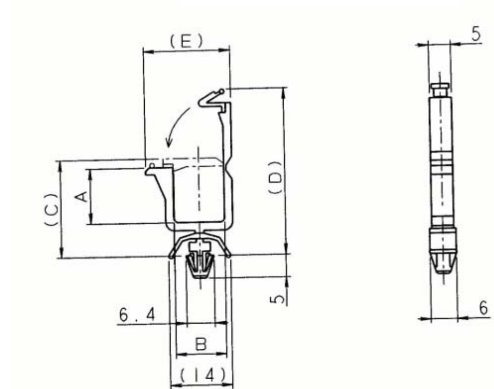
Fig. 10 CABLE CLAMP (1/5)
