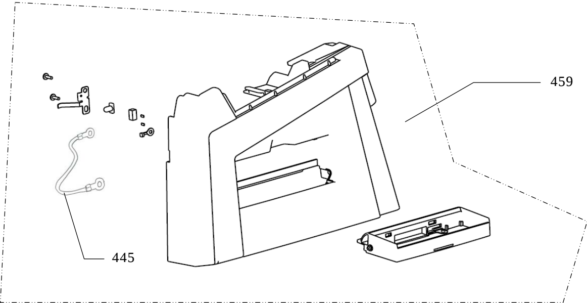
Figure 5 FRONT COVER
