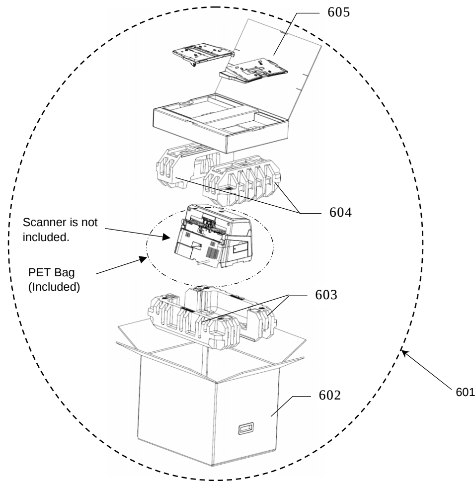
Figure 17 PACKAGING BOX, SCANNER (fi-6670/fi-6670A)
