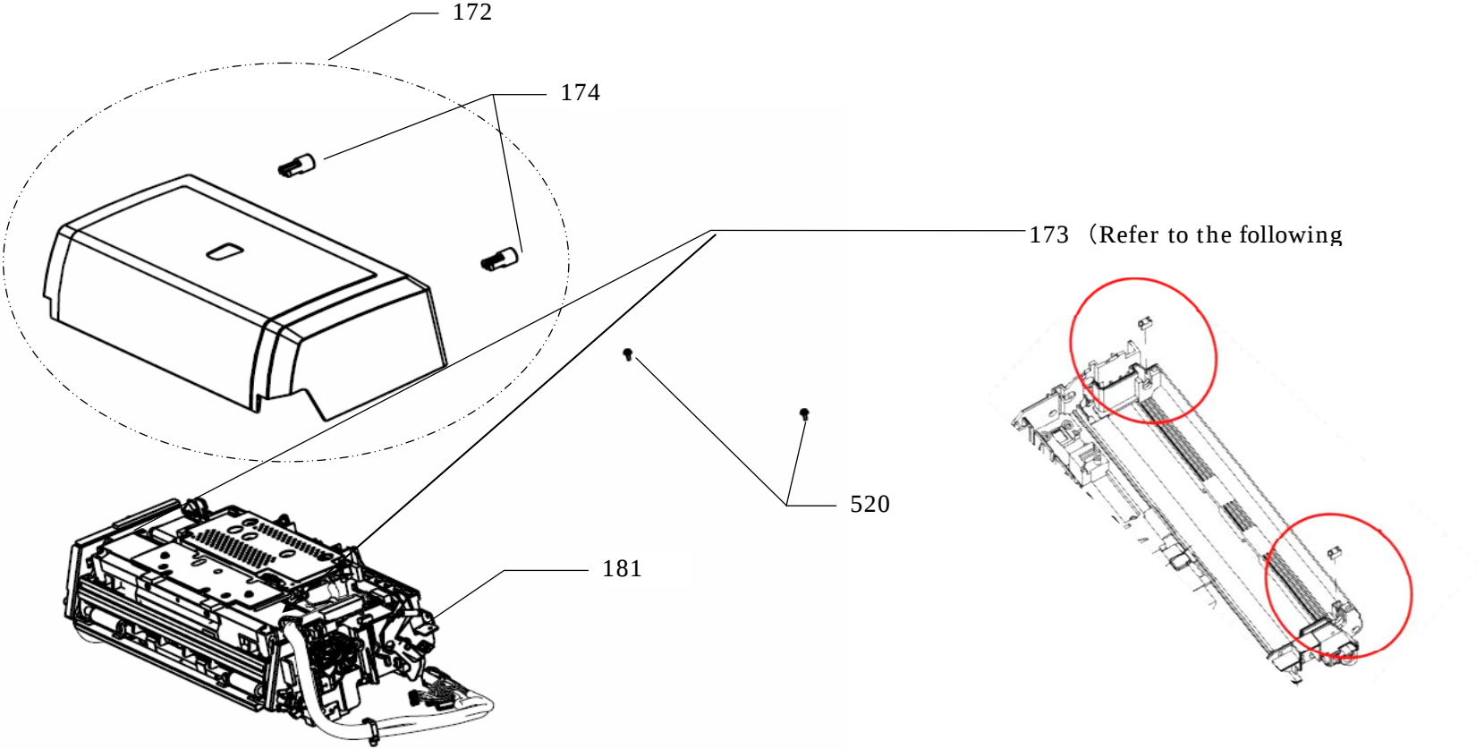
Figure 11 ADF UNIT FINAL ASSEMBLY
