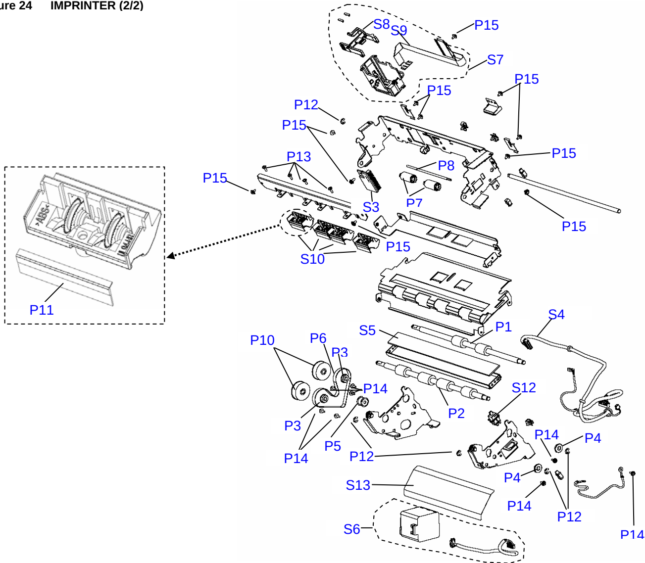
Figure 24 IMPRINTER (2/2)
