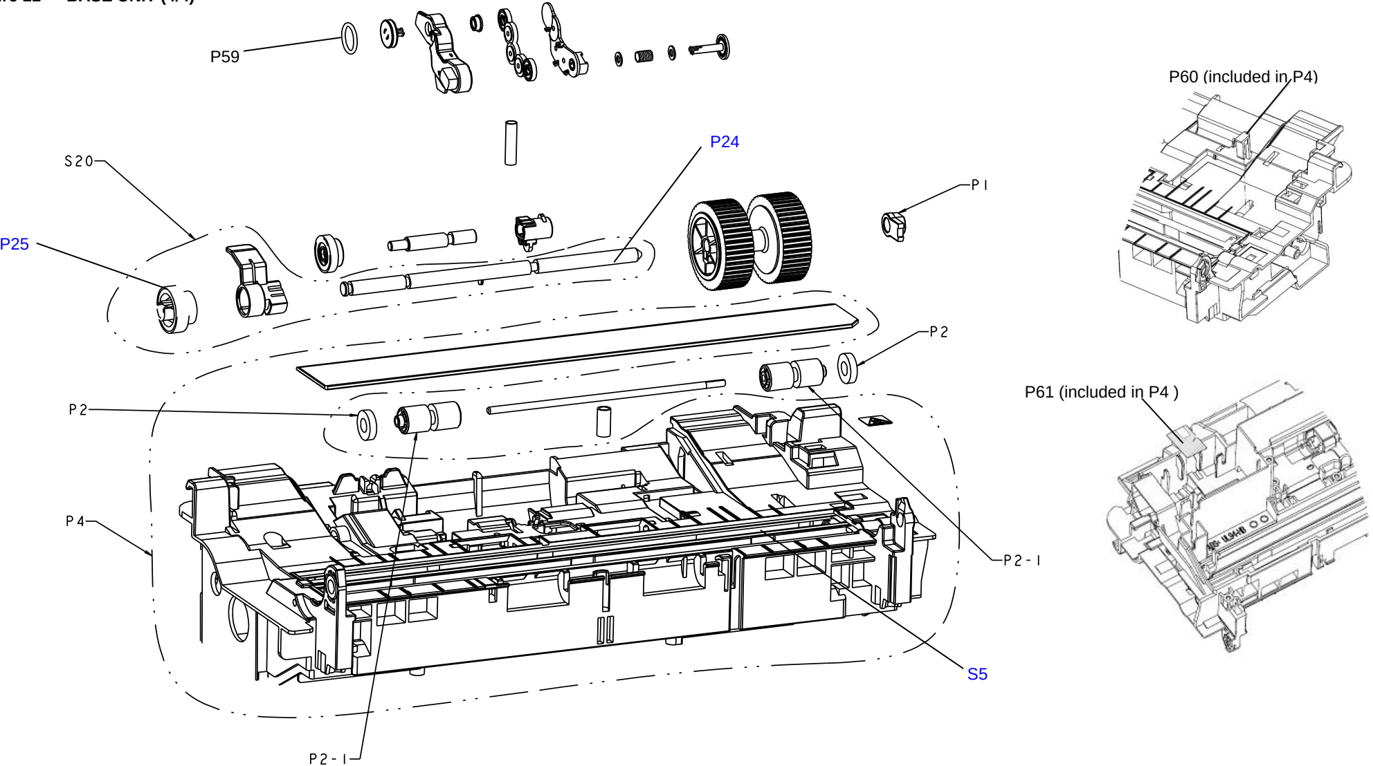
Figure 11 BASE UNIT (4/4)
