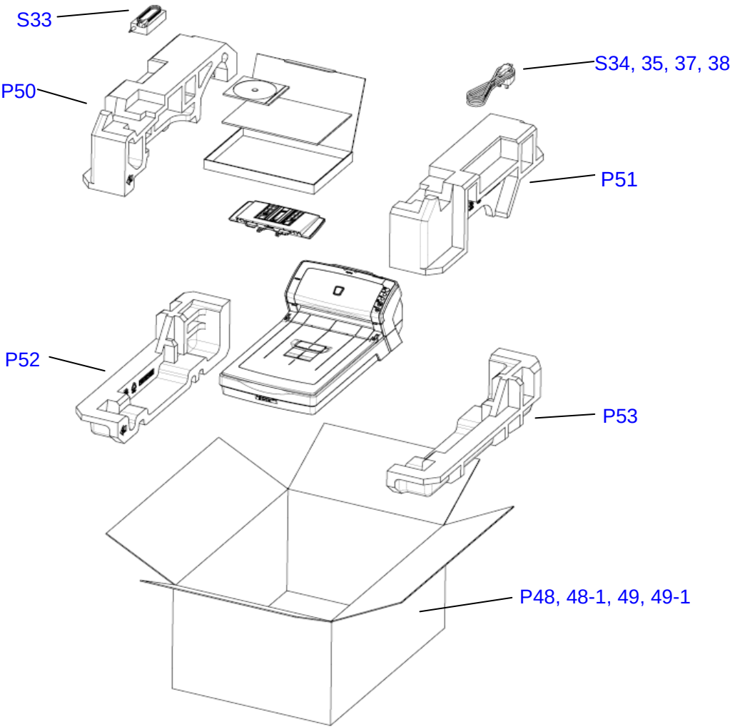
Figure 22 PACKAGE (fi-6240/fi-6230)
