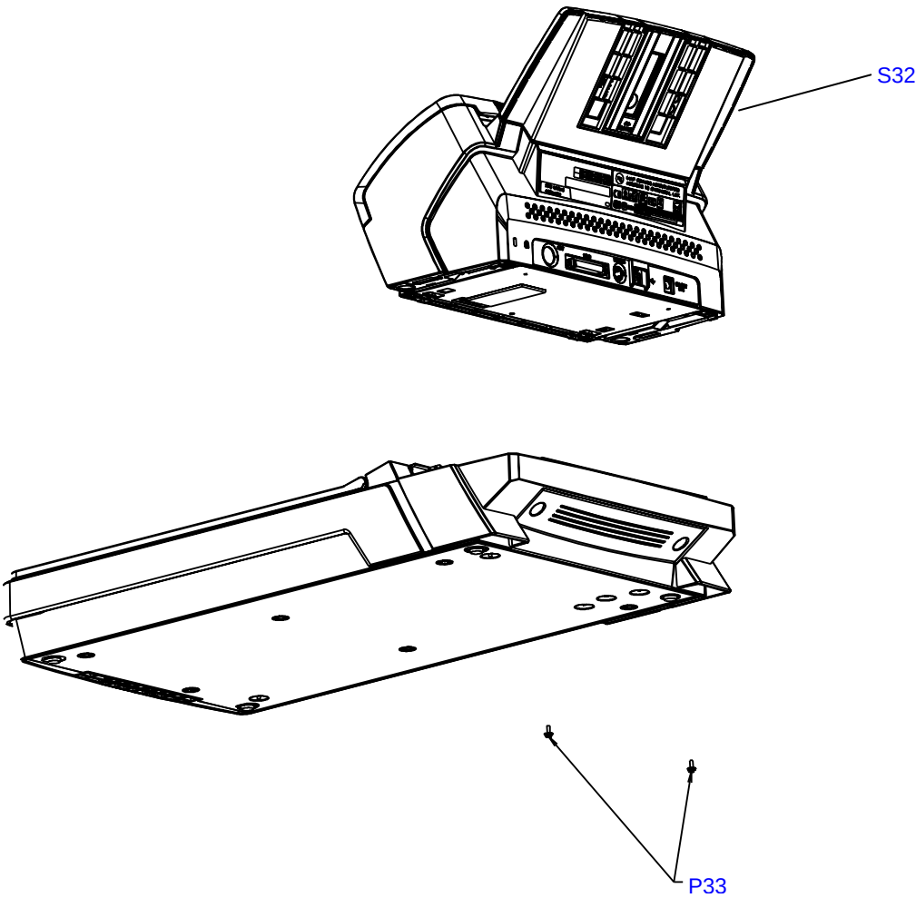
Figure 1 FINAL ASSEMBLY (fi-6240/fi-6230)
