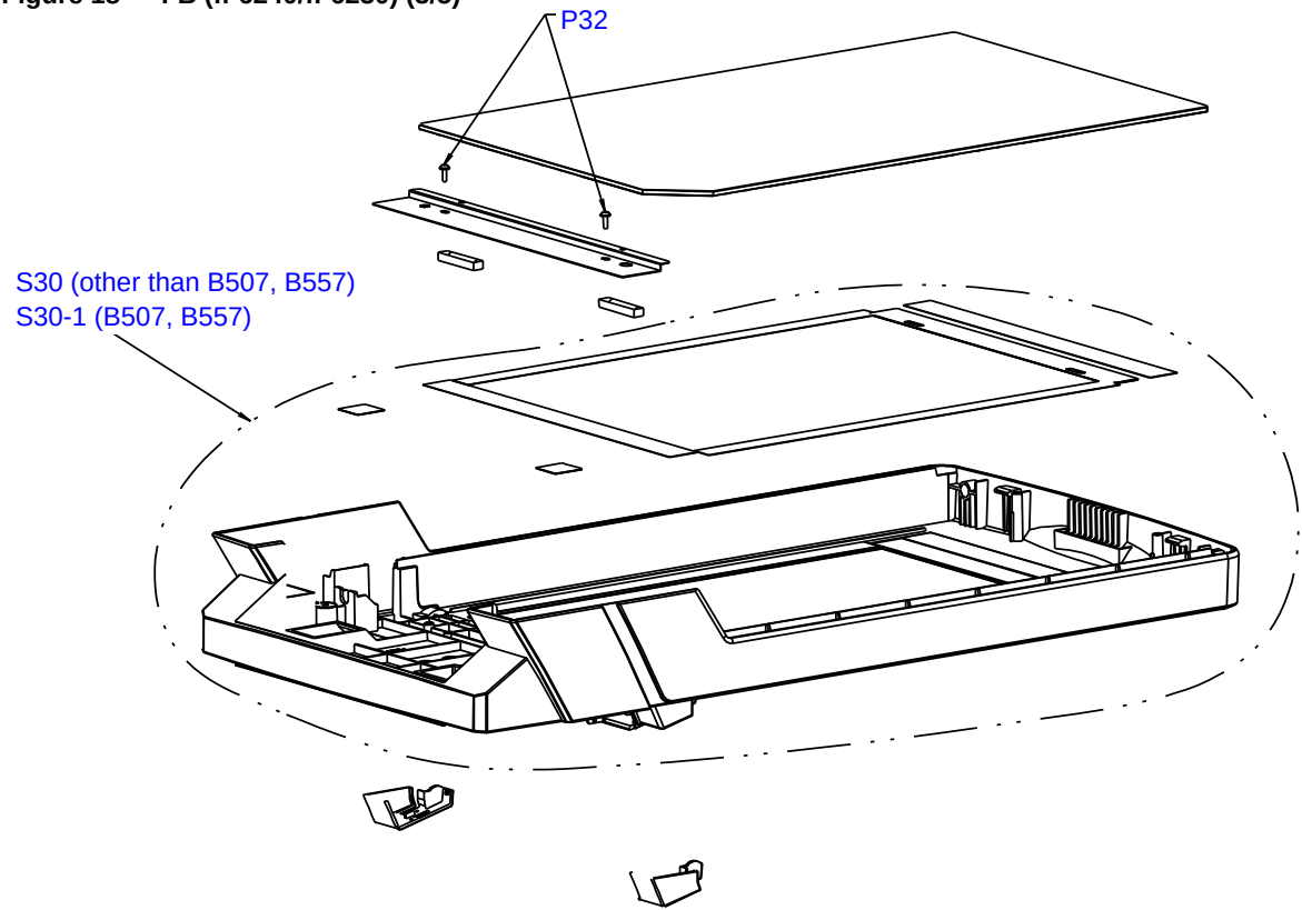
Figure 18 FB (fi-6240/fi-6230) (3/5)
