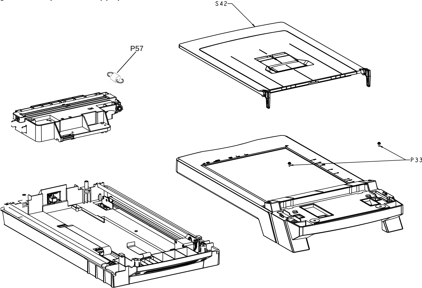
Figure 16 FB (fi-6240/fi-6230) (1/5)
