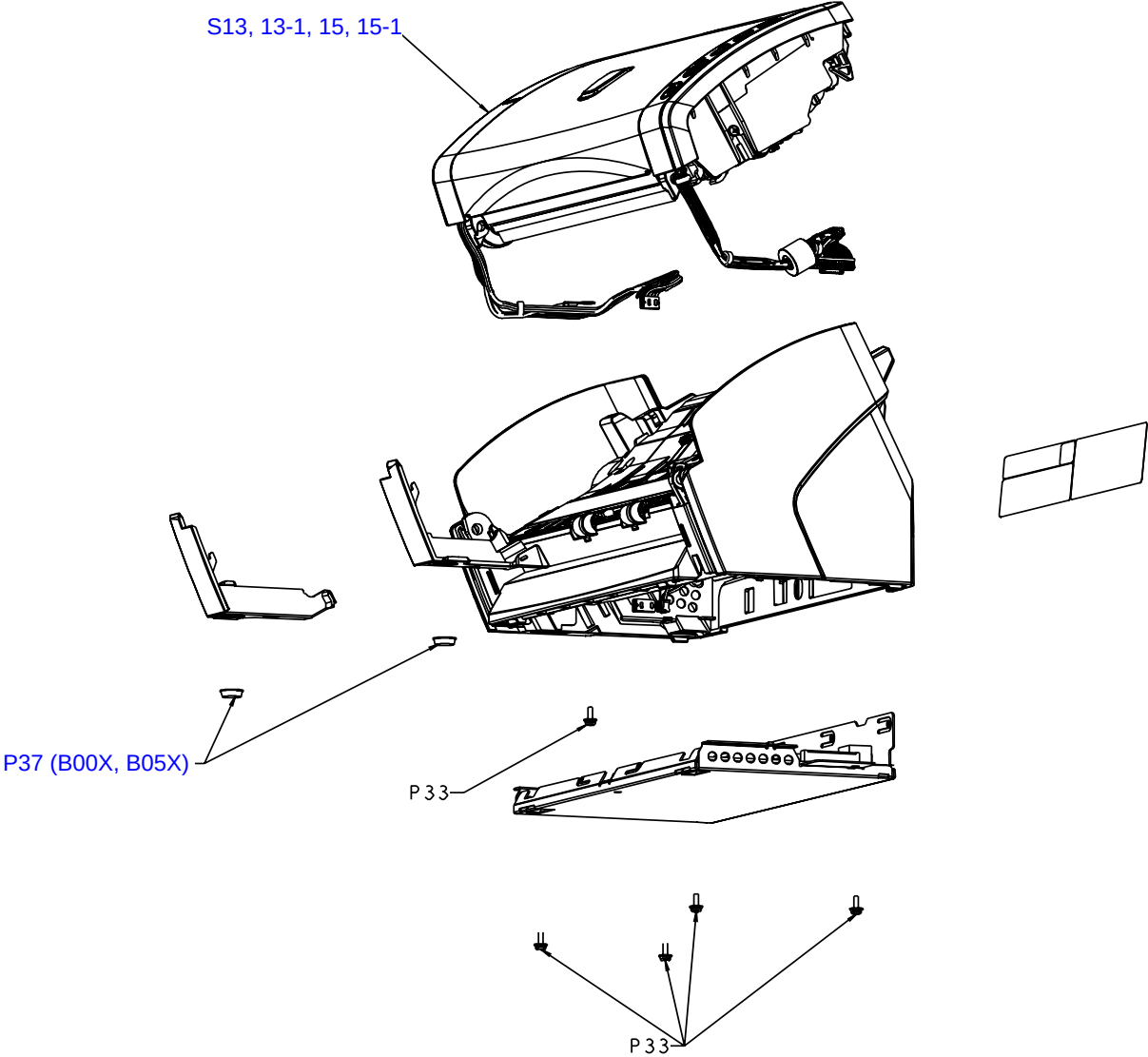
Figure 3 SCAN UNIT
