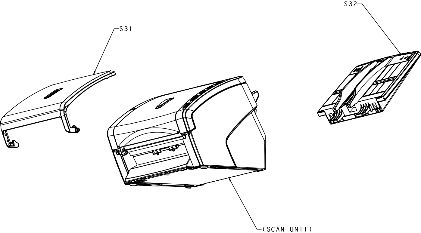
Figure 2 FINAL ASSEMBLY (fi-6140/fi-6130)
