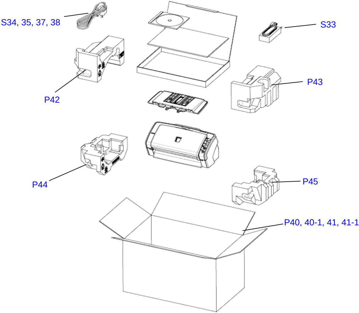
Figure 21 PACKAGE (fi-6140/fi-6130)
