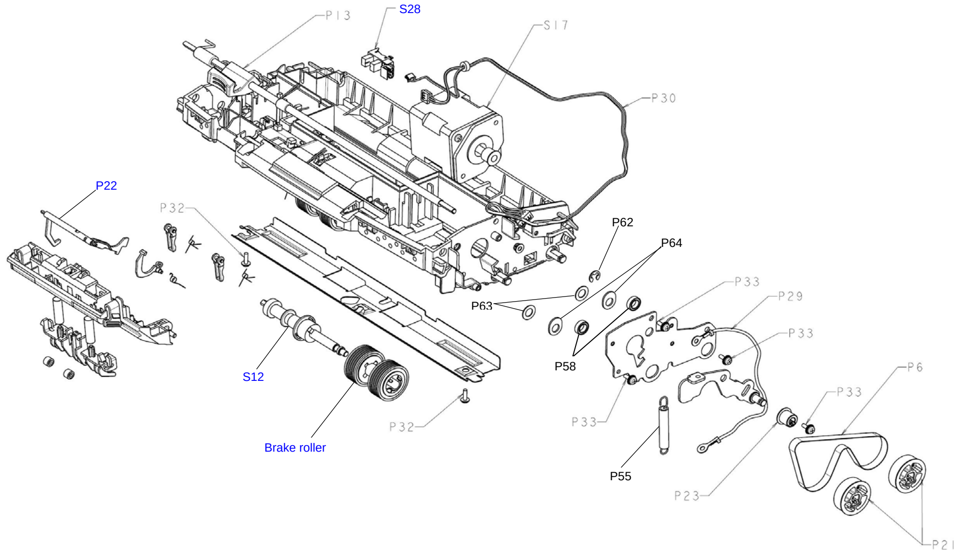
Figure 6 UPPER UNIT (3/4)
