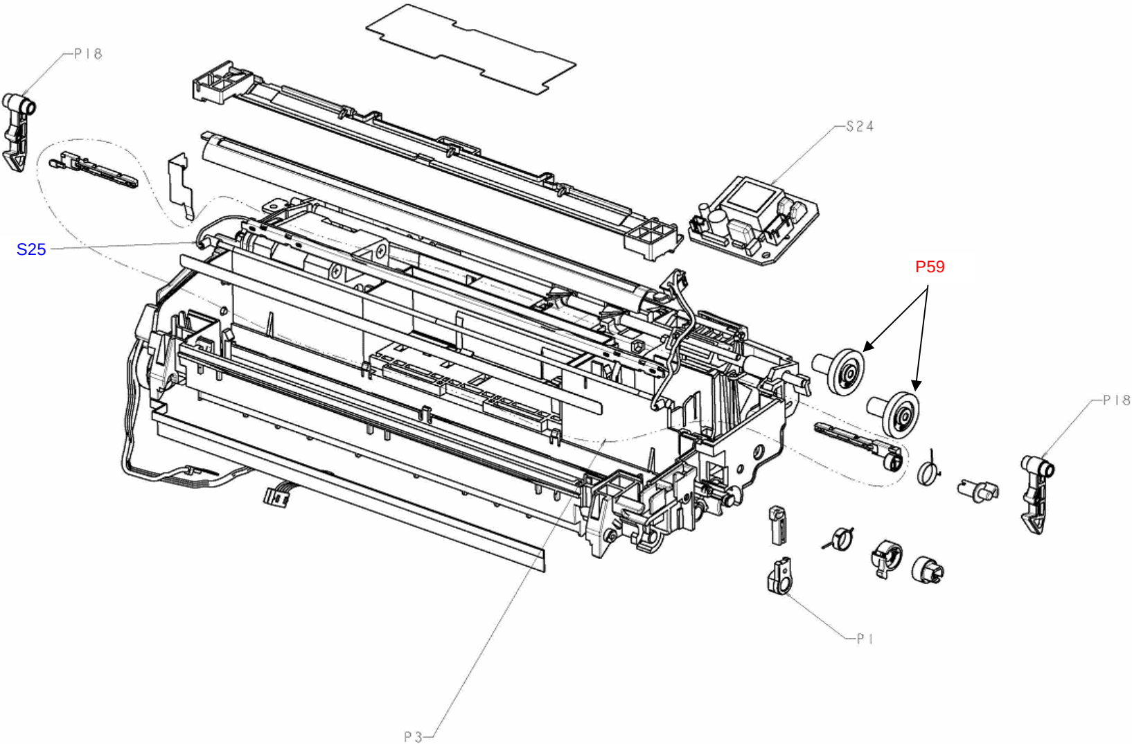
Figure 5 UPPER UNIT (2/4)
