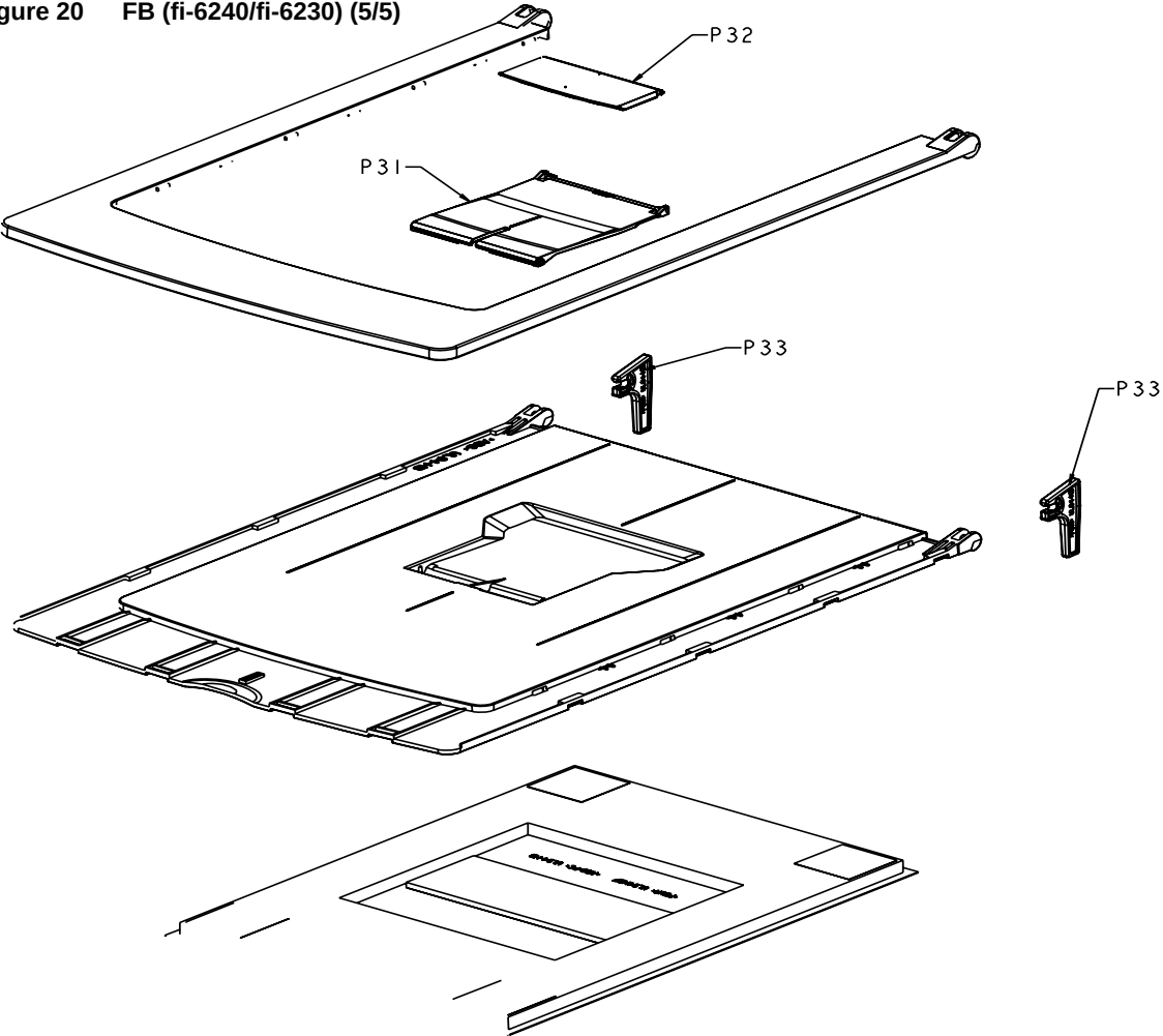
Figure 20 FB (fi-6240/fi-6230) (5/5)
