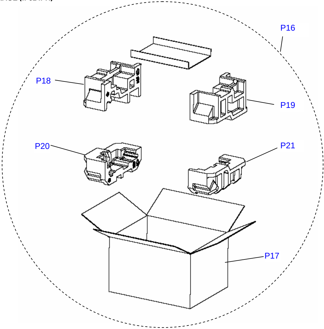
Figure 25 PACKAGE (fi-614PR)
