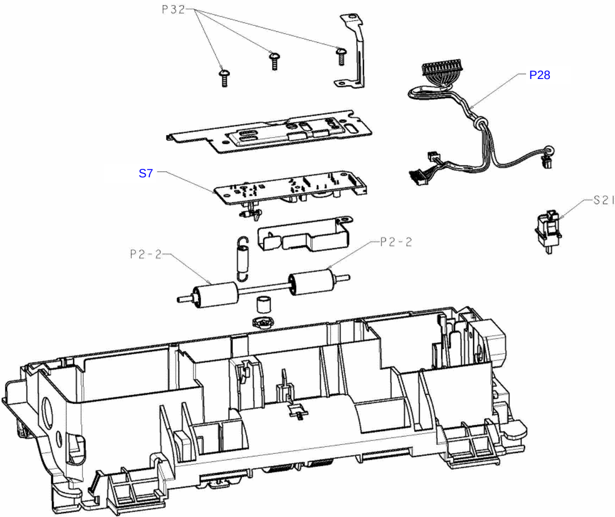
Figure 10 BASE UNIT (3/4)
