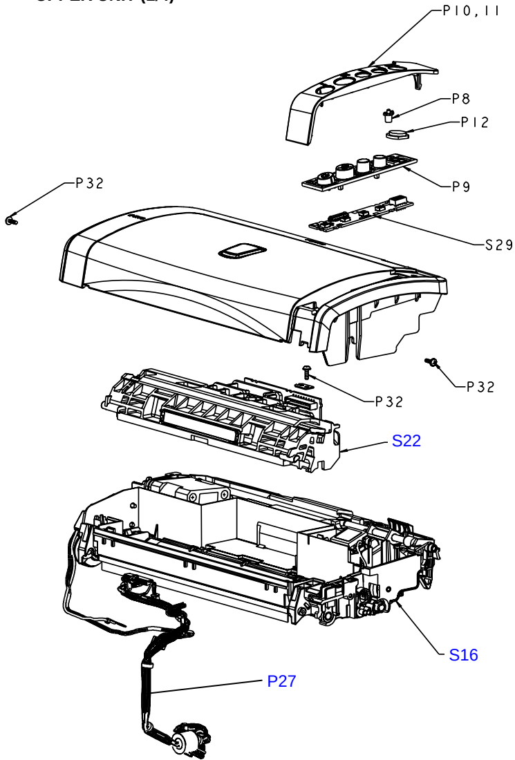
Figure 4 UPPER UNIT (1/4)
