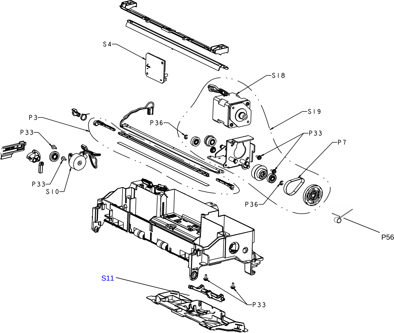
Figure 9 BASE UNIT (2/4)
