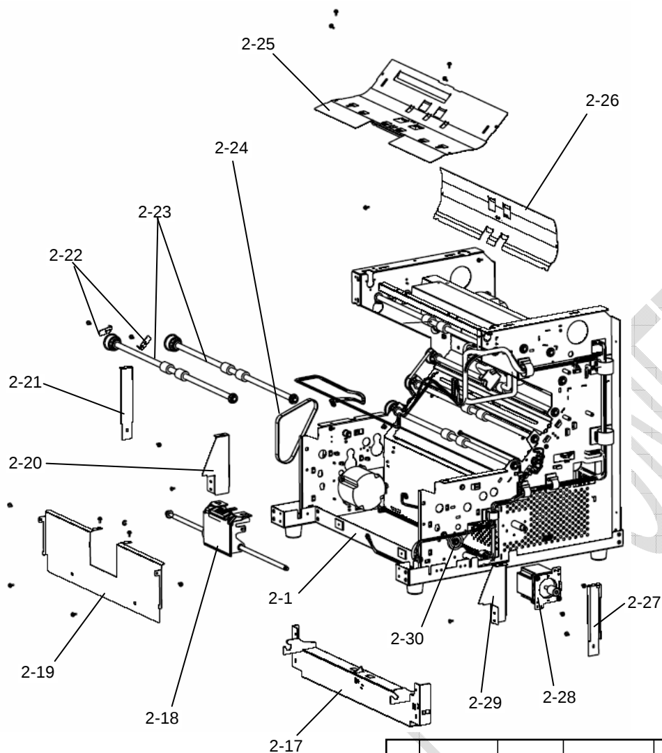
FIGURE 2. BASE UNIT 2/2
