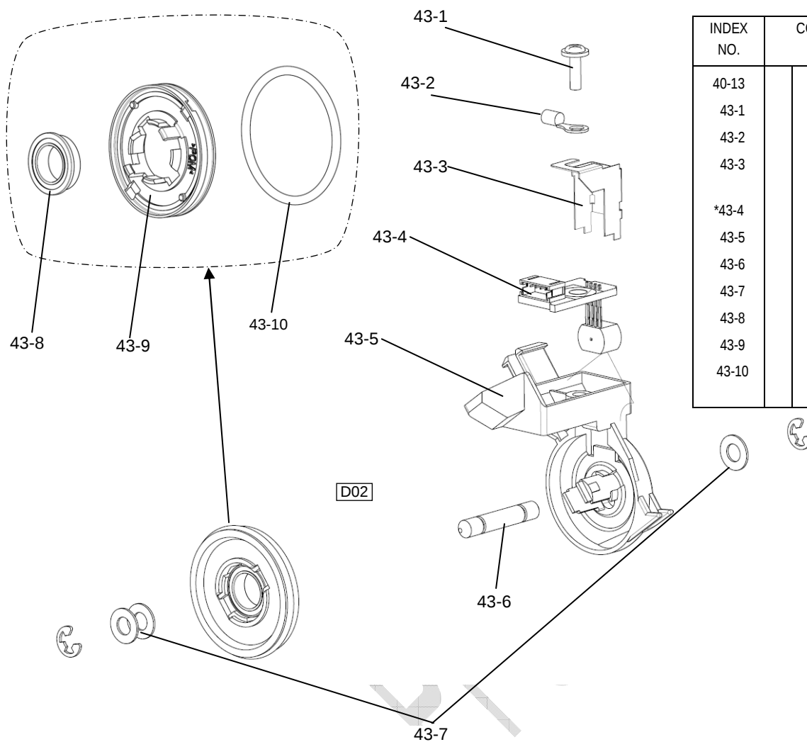
FIGURE 43. ENCODER UNIT
