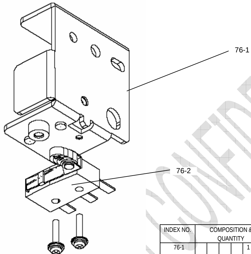
FIGURE 76. INTERLOCK SWITCH ASSY
