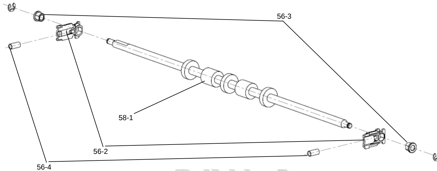
FIGURE 58. PINCH ROLLER ASSY 3
