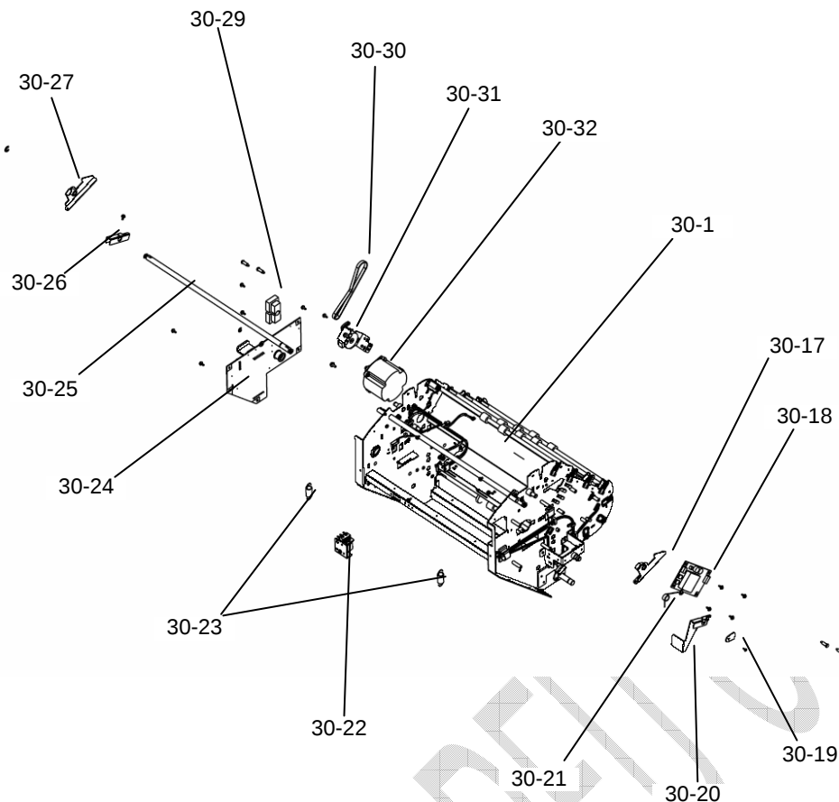
FIGURE 30. UPPER UNIT 2/2
