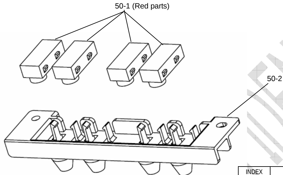
FIGURE 50. SENSOR PTR ASSY
