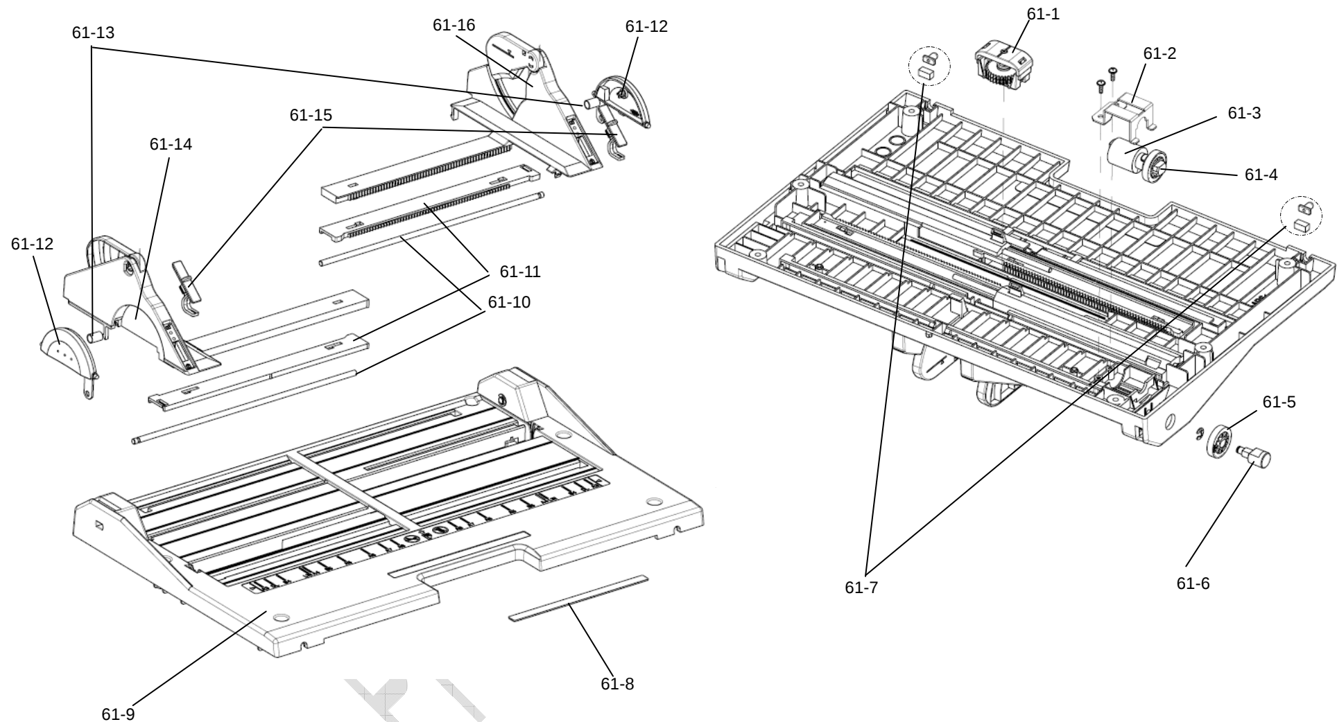
FIGURE 61. HOPPER BASE ASSY
