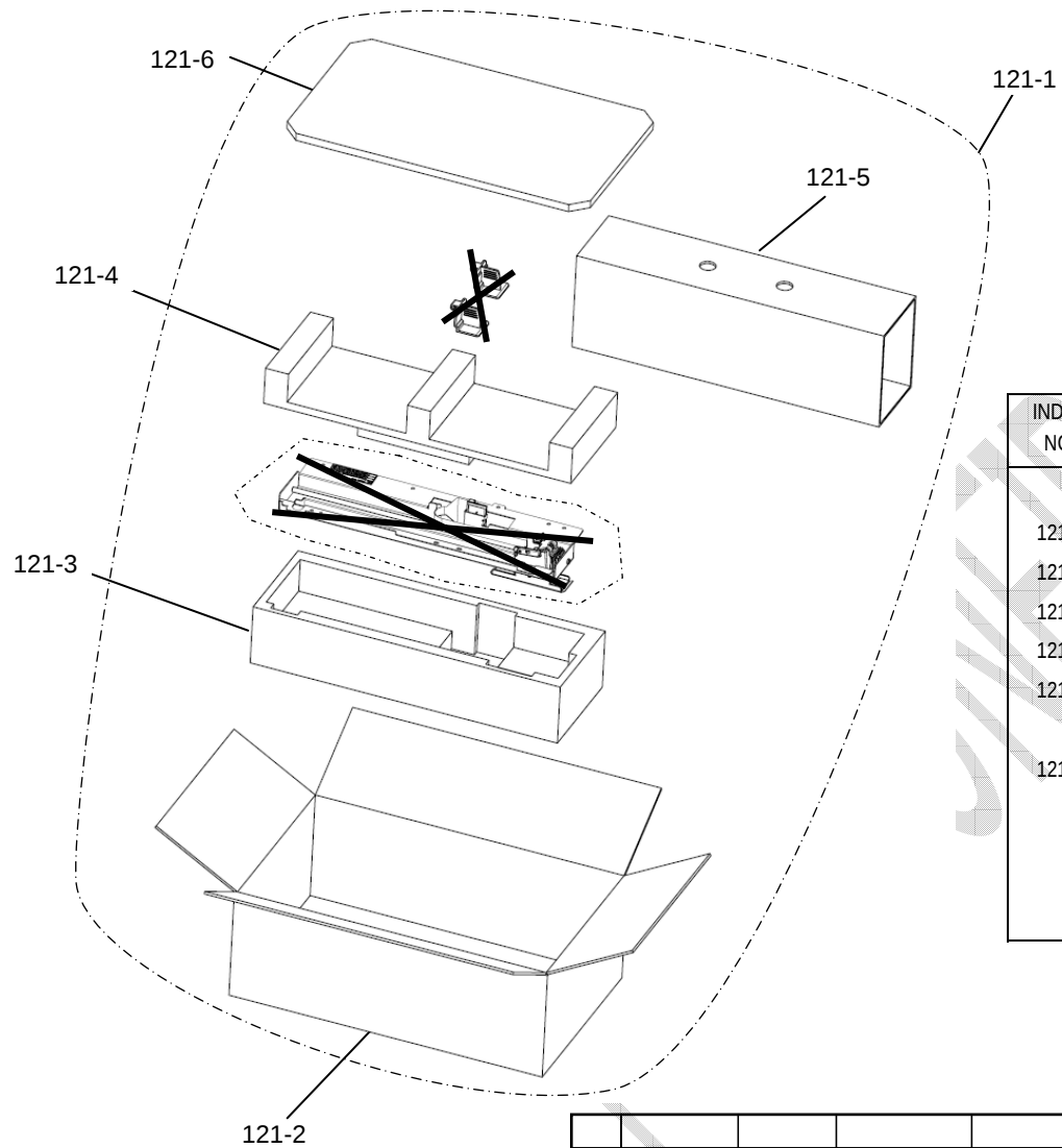
FIGURE 121 PACKAGES, IMPRINTER (Option), fi-590PRB
