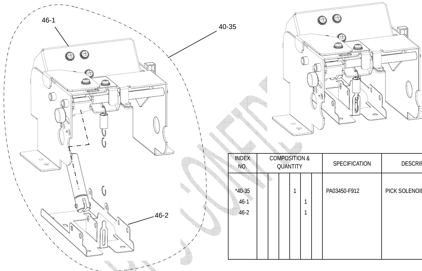
FIGURE 46. PICK SOLENOID
