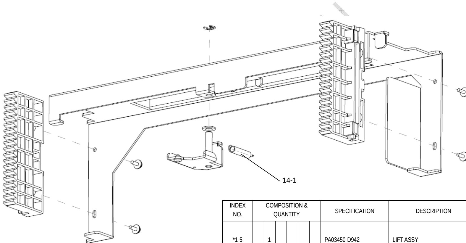
FIGURE 14. STACKER LIFT ASSY
