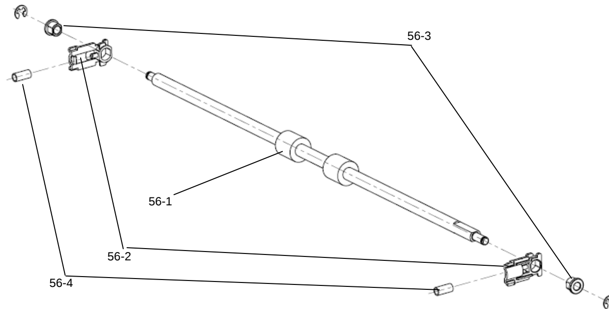
FIGURE 56. PINCH ROLLER ASSY 1
