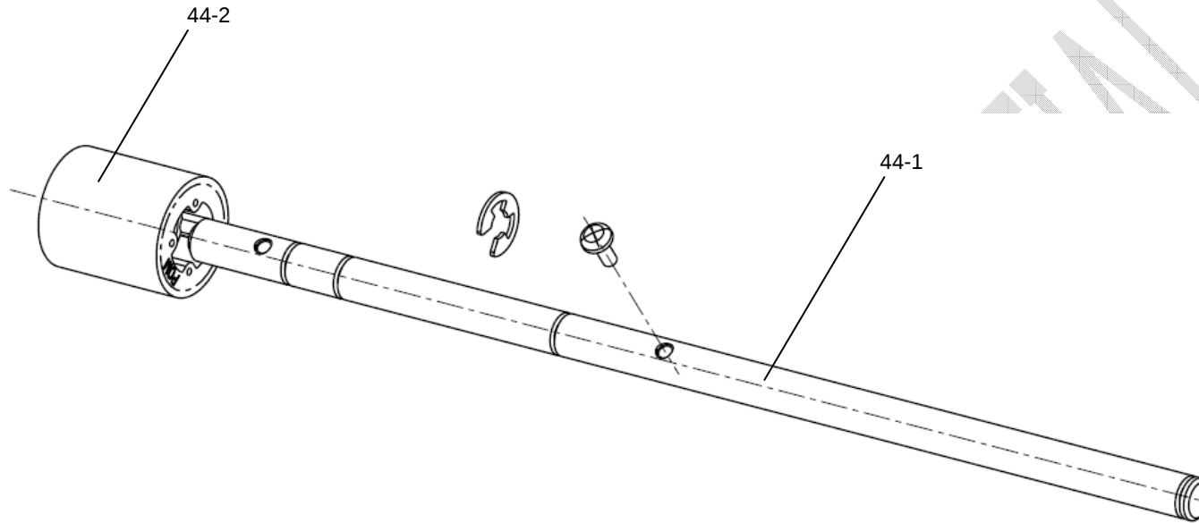
FIGURE 44. SLIDE SHAFT ASSY
