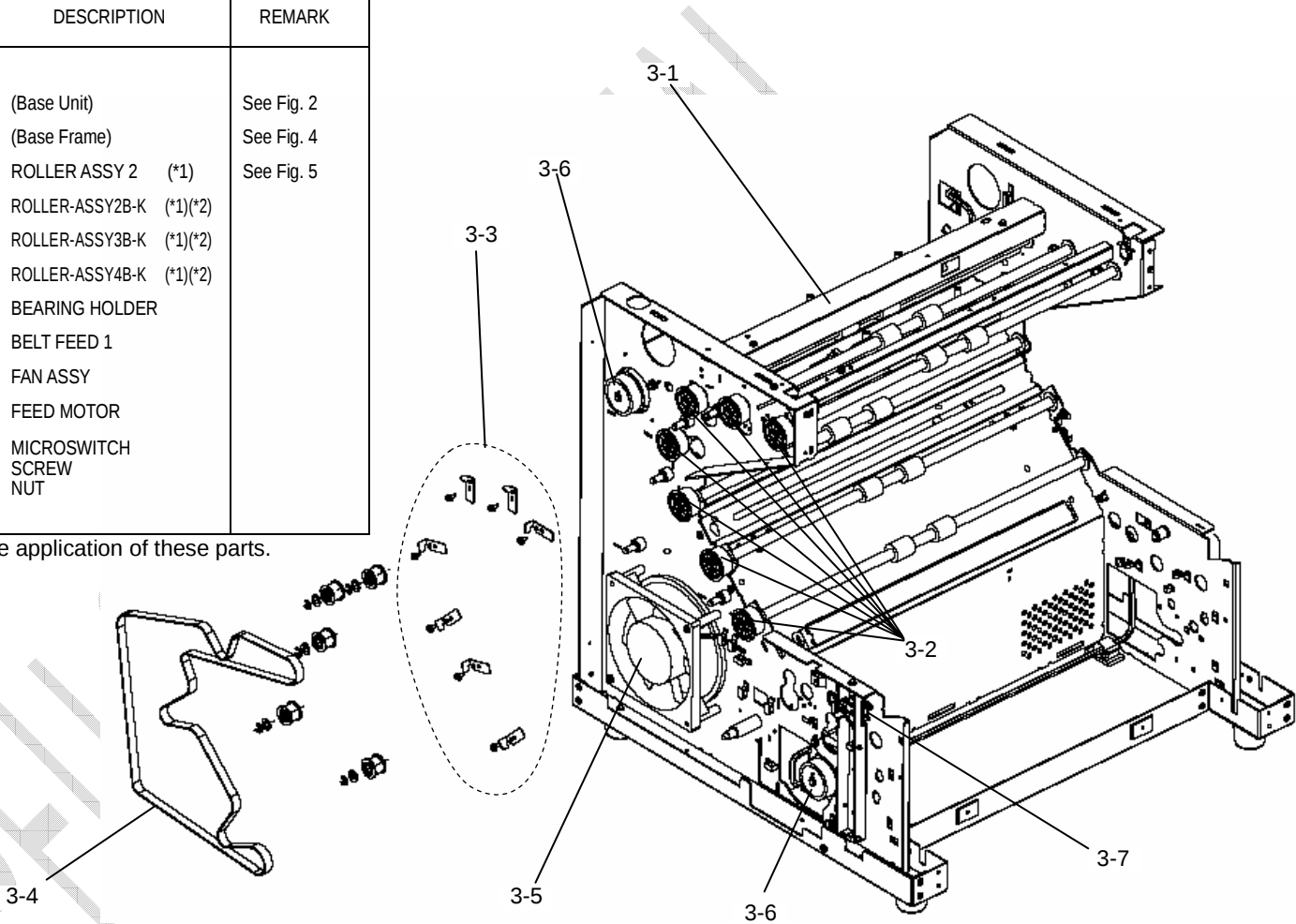
FIGURE 3. BASE FRAME ASSEMBLY 1/2
