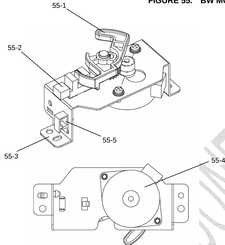
FIGURE 55. BW MOTOR UNIT
