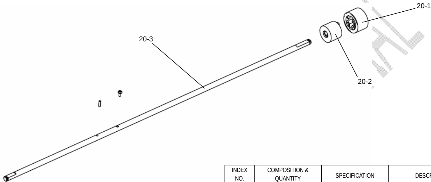
FIGURE 20. HOPPER SHAFT ASSY
