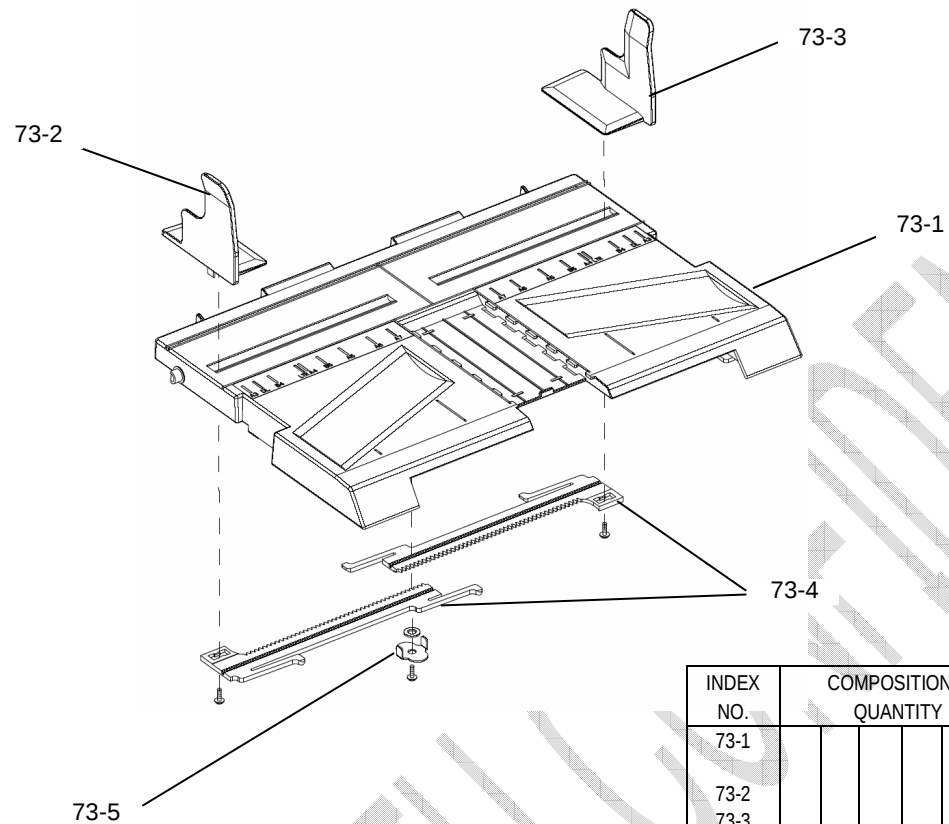
FIGURE 73. STACKER BASE ASSY
