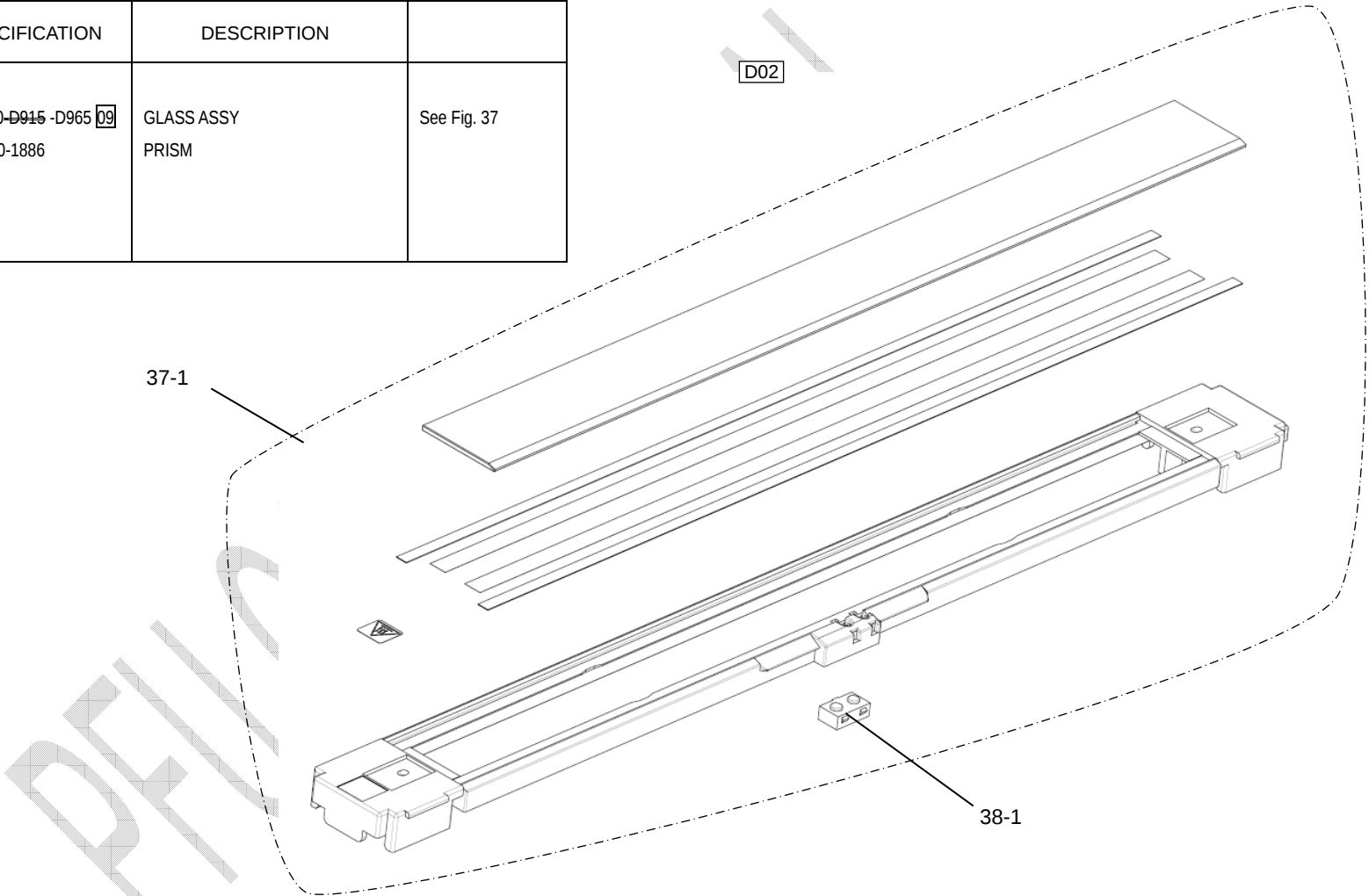
FIGURE 38. LAMP GLASS ASSY
