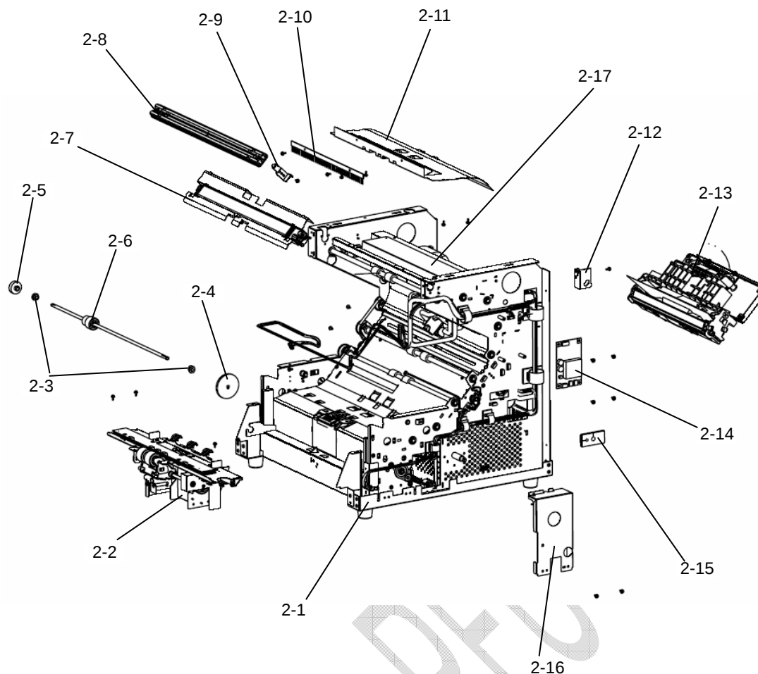
FIGURE 2. BASE UNIT 1/2
