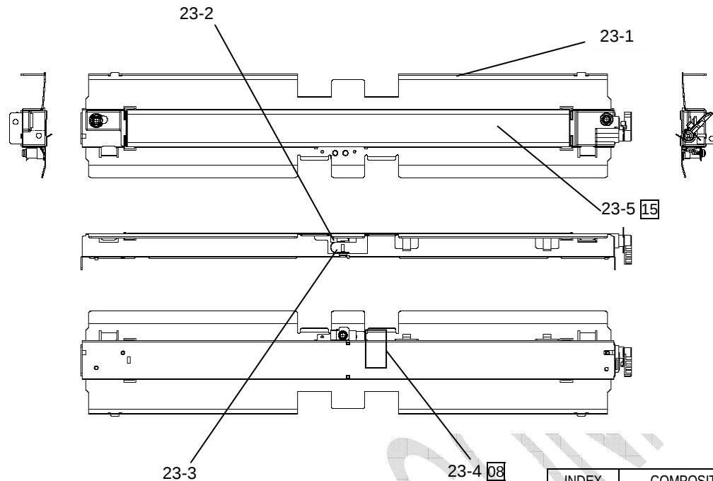
FIGURE 23. BACKGROUND UNIT, LOWER
