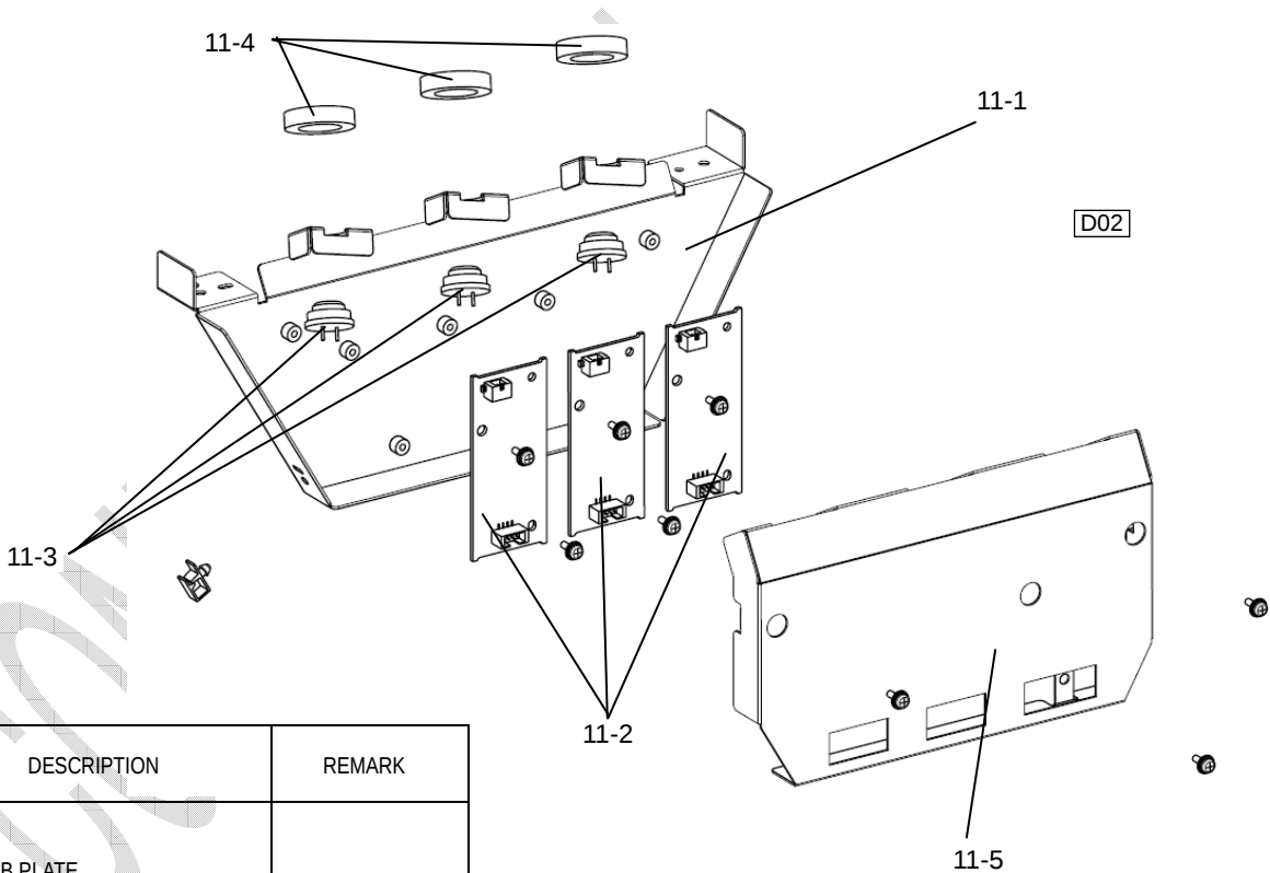
FIGURE 11. US SENSOR ASSEMBLY
