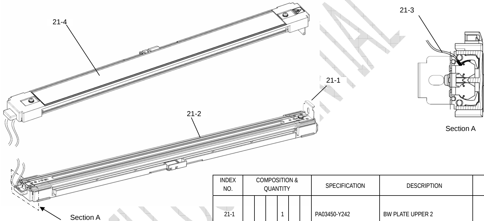
FIGURE 21. LAMP UNIT LOWER
