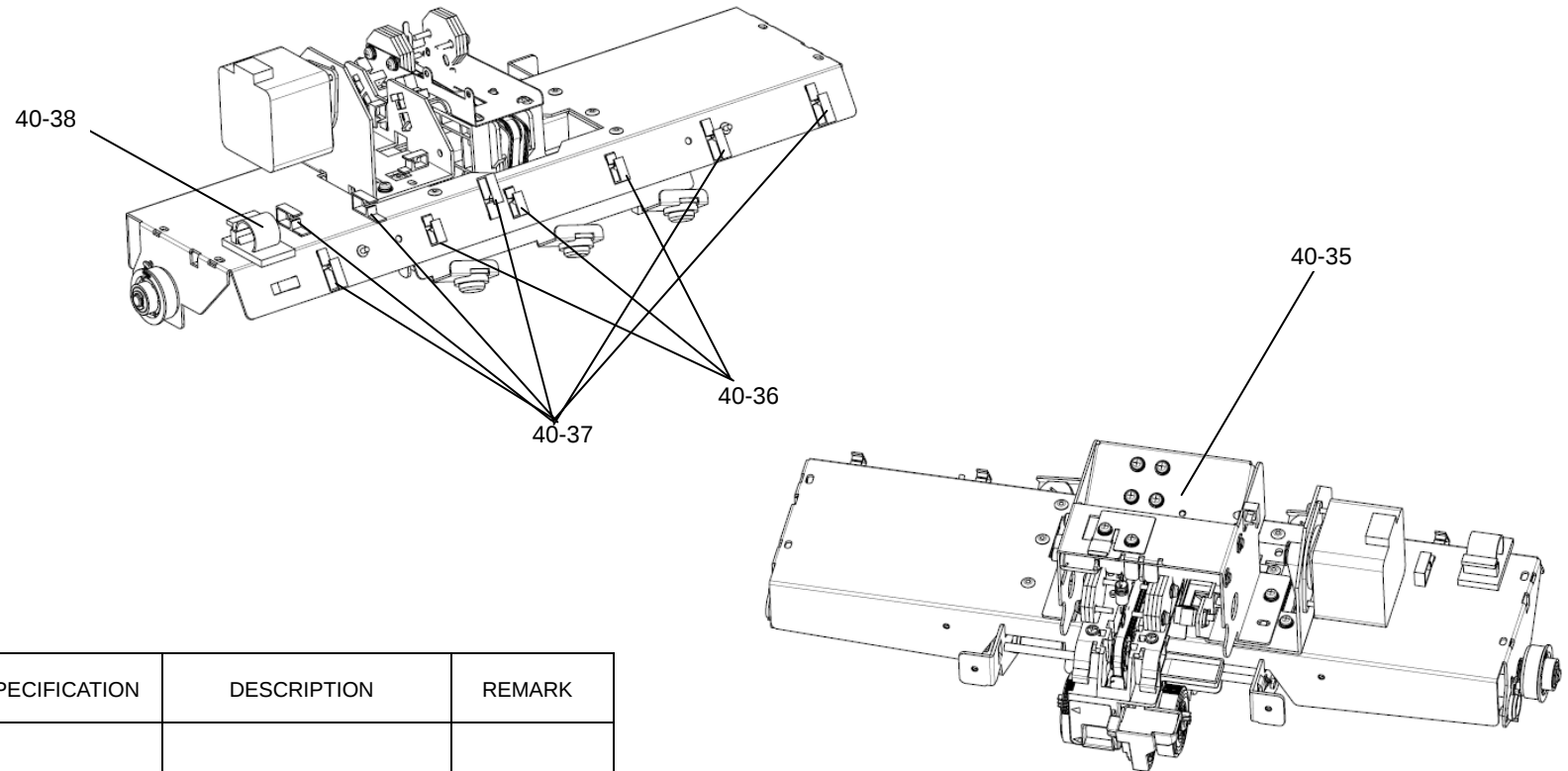
FIGURE 40. SEPARATOR UNIT 5/5
