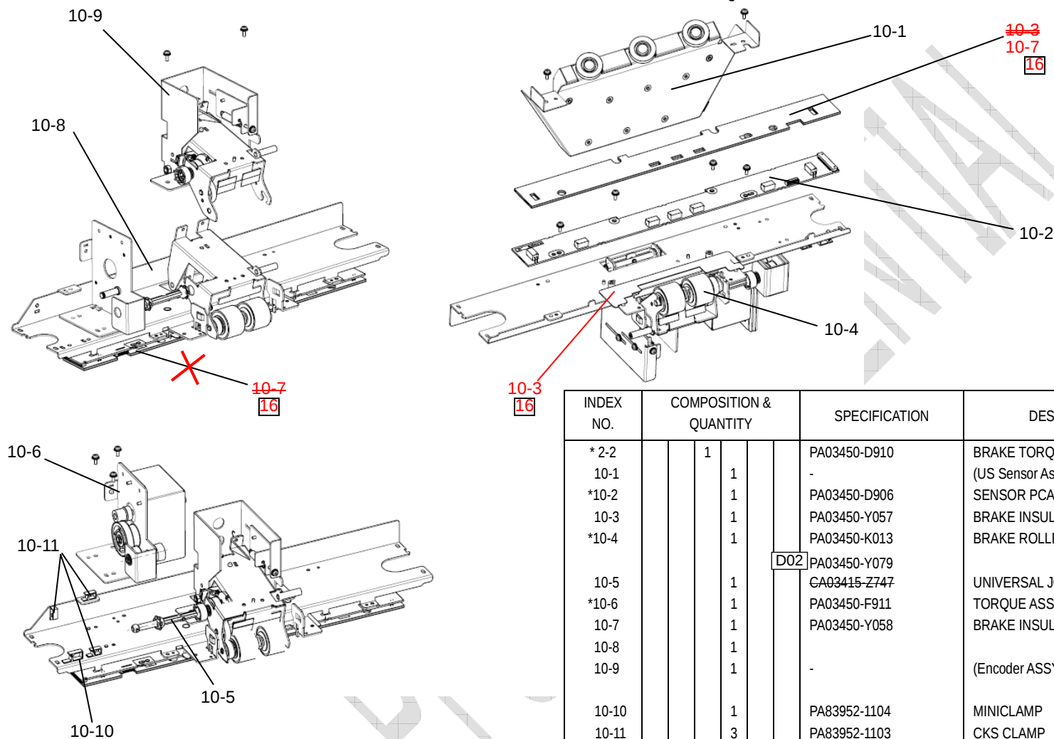
FIGURE 10. BRAKE TORQUE UNIT
