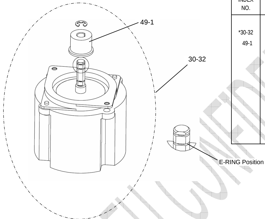
FIGURE 49. SEPARATION MOTOR
