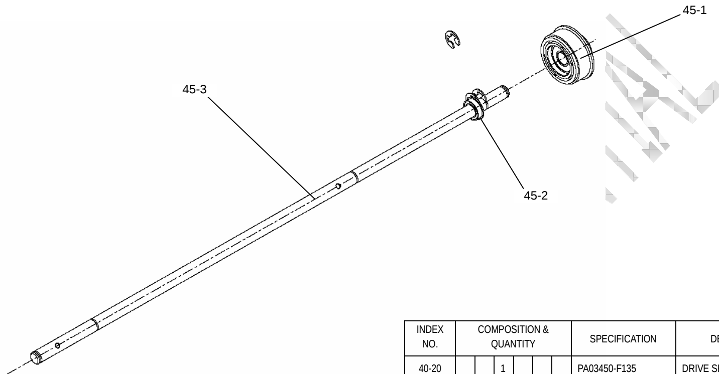
FIGURE 45. DRIVE SHAFT ASSY
