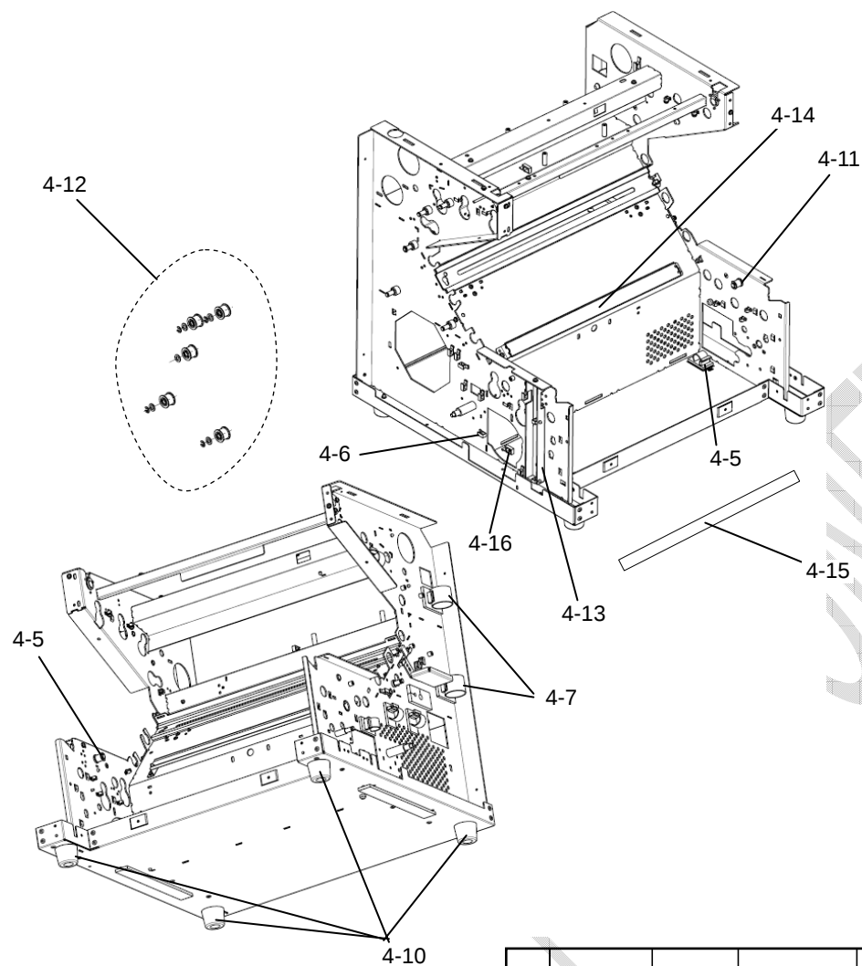
FIGURE 4. BASE FRAME (2/2)
