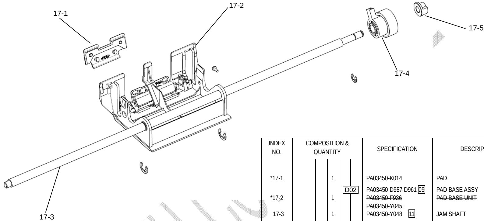
FIGURE 17. PAD UNIT
