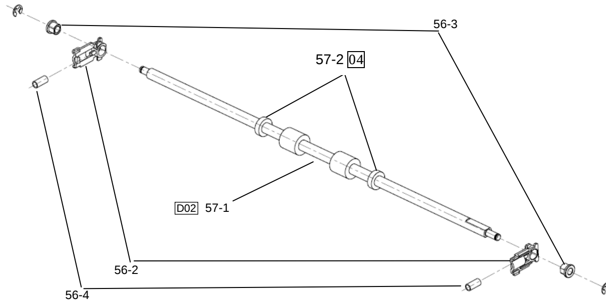
FIGURE 57. PINCH ROLLER ASSY 2
