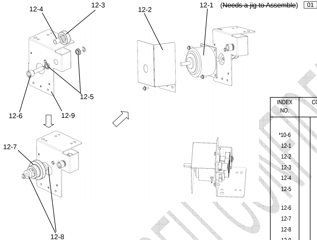
FIGURE 12. TORQUE ASSY
