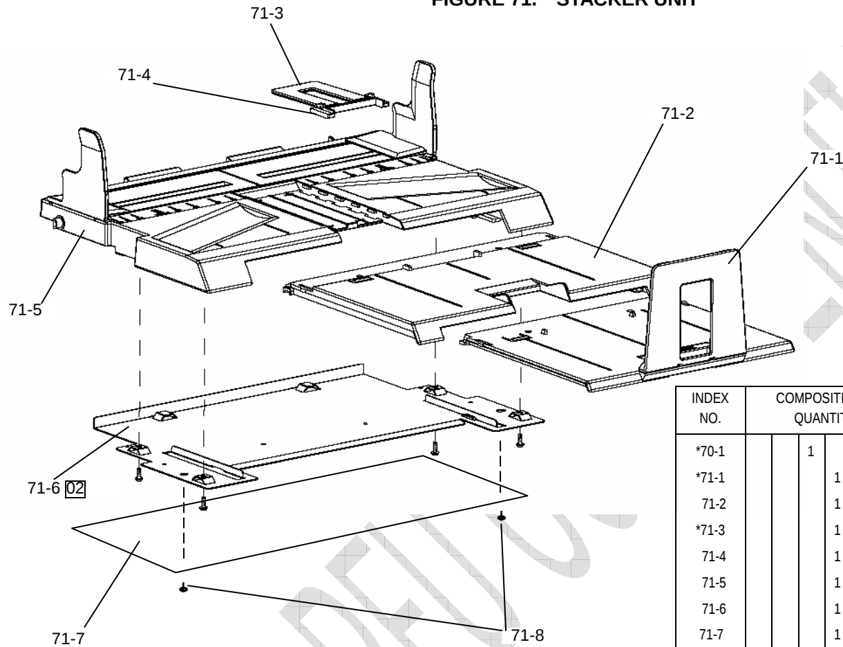
FIGURE 71. STACKER UNIT
