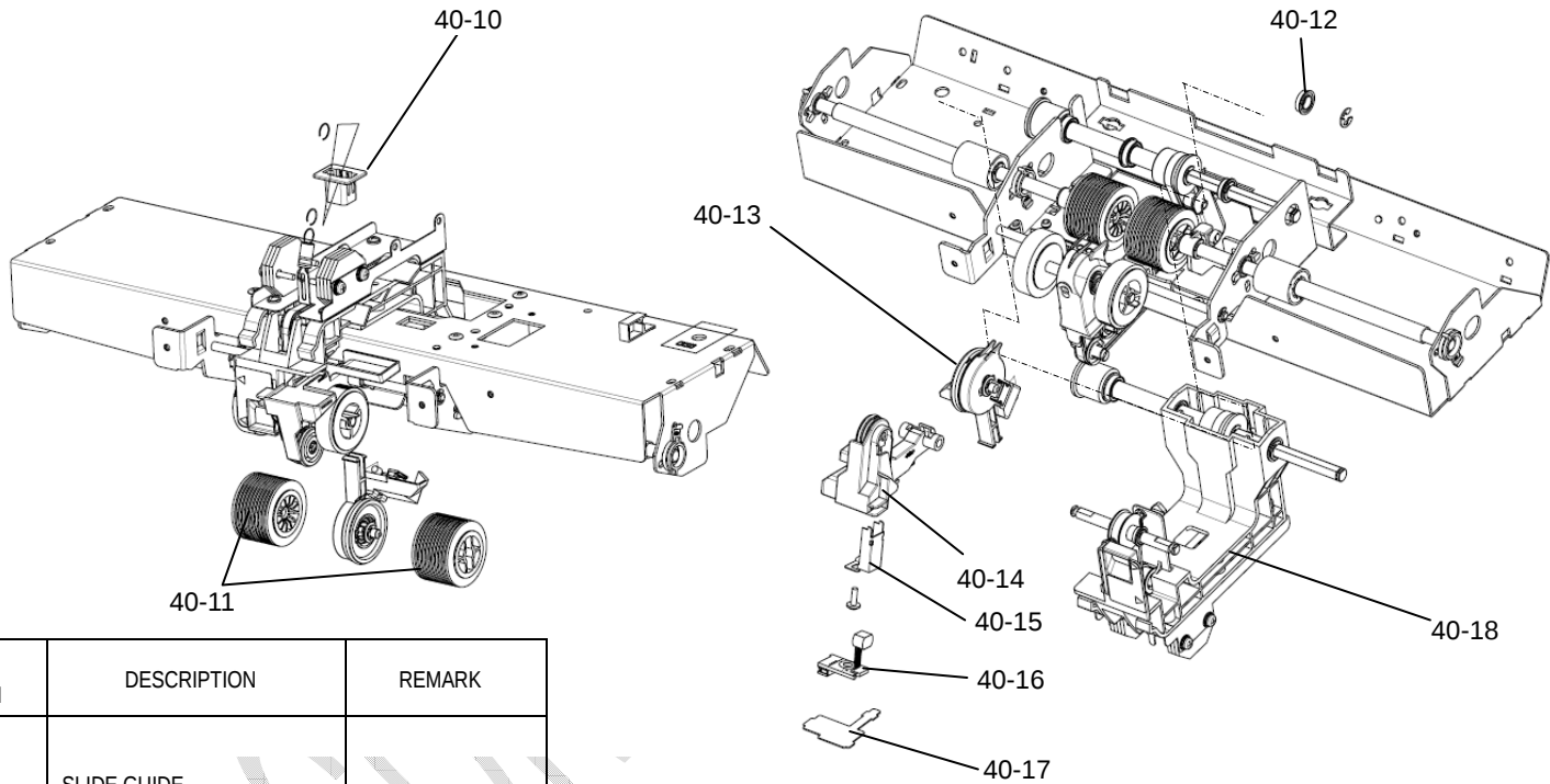
FIGURE 40. SEPARATOR UNIT 2/5
