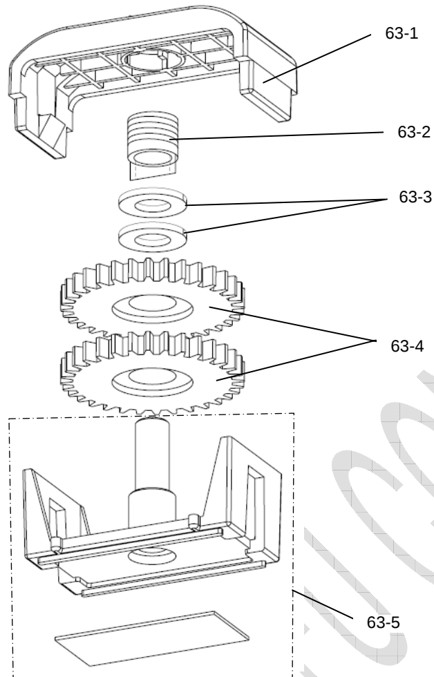
FIGURE 63. HOPPER SLIDE ASSY
