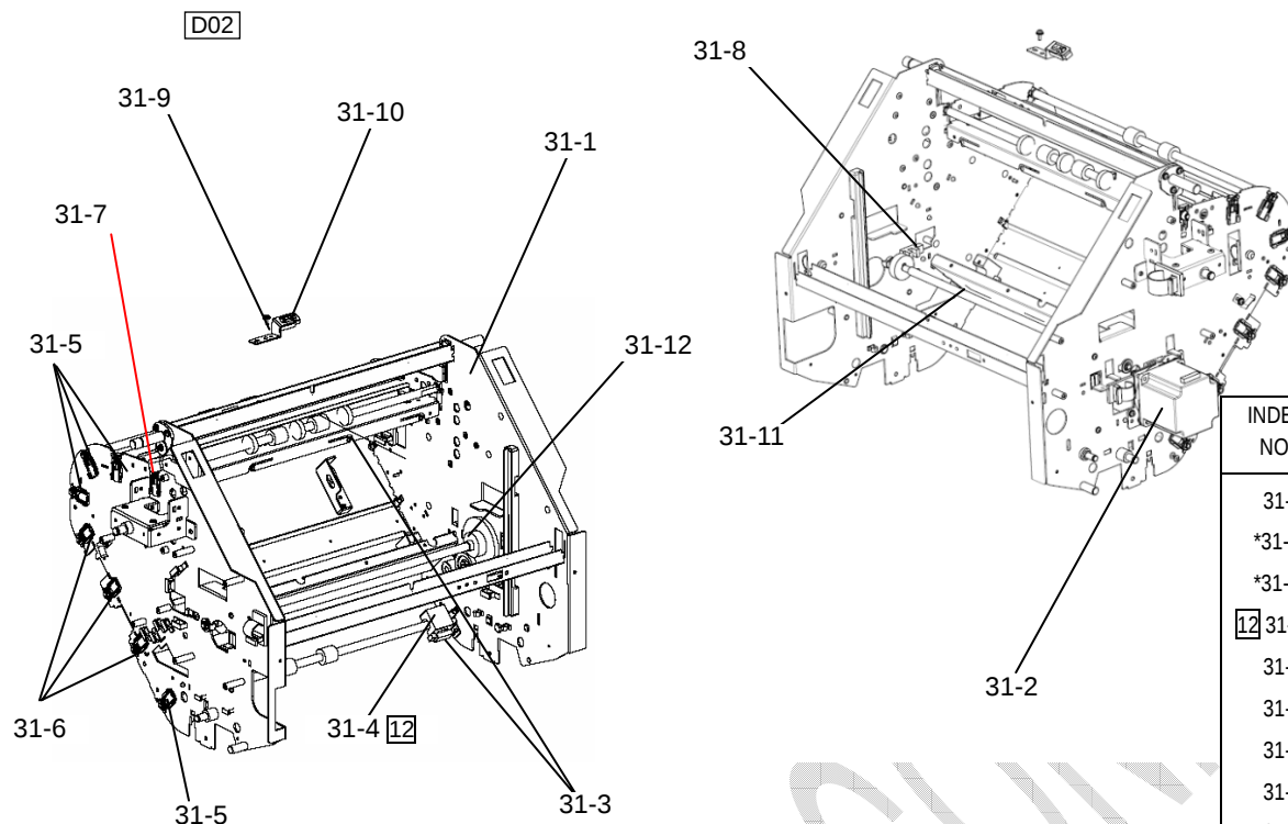
FIGURE 31. UPPER ROLLER ASSY
