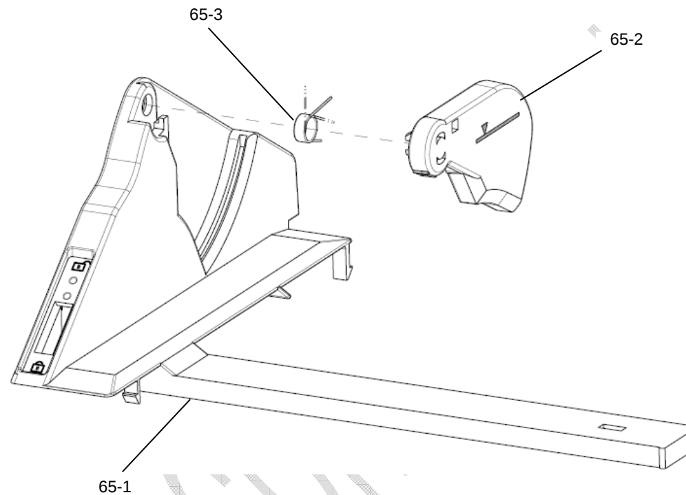
FIGURE 65. HOPPER GUIDE L ASSY
