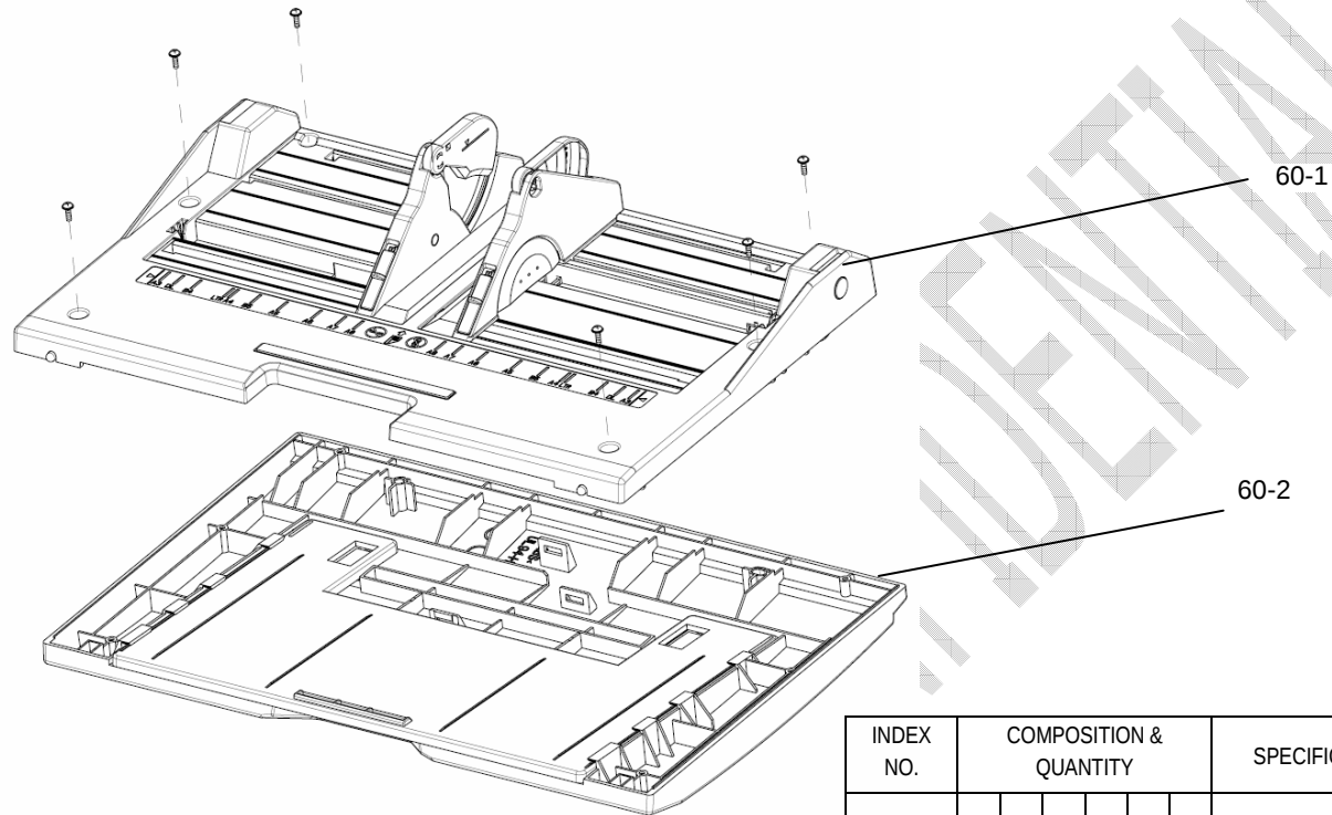
FIGURE 60. HOPPER UNIT
