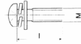
FIGURE B1 SCREW WITH WASHER
