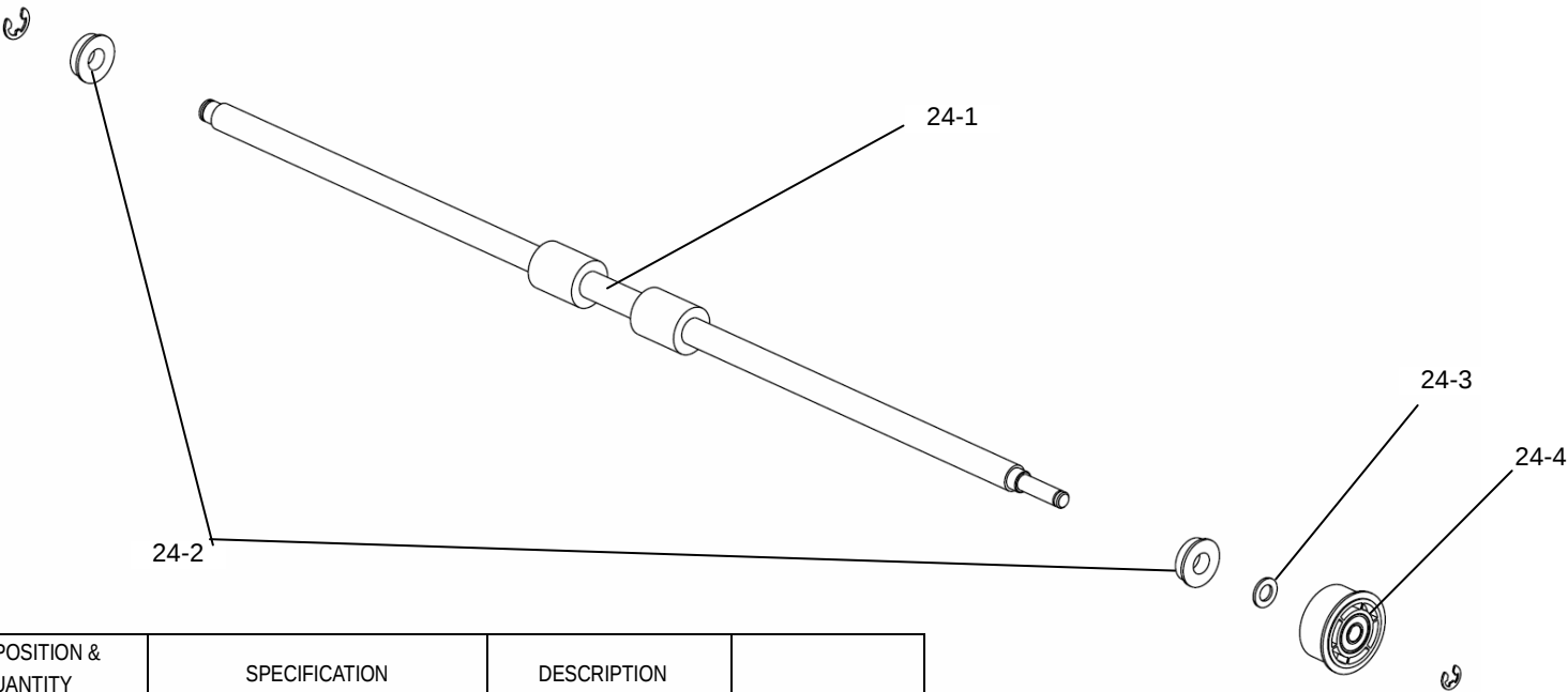
FIGURE 24. ROLLER ASSY 1
