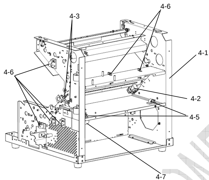
FIGURE 4. BASE FRAME (1/2)
