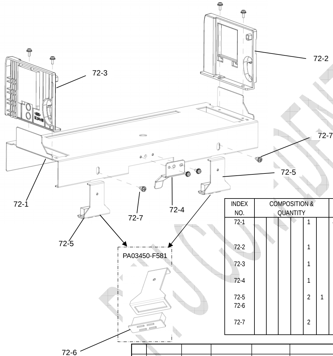
FIGURE 72. STACKER HOLDER ASSY
