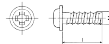
FIGURE B4 PT SCREW
