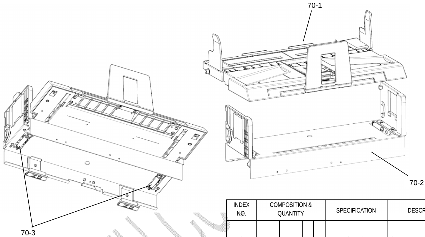
FIGURE 70. STACKER
