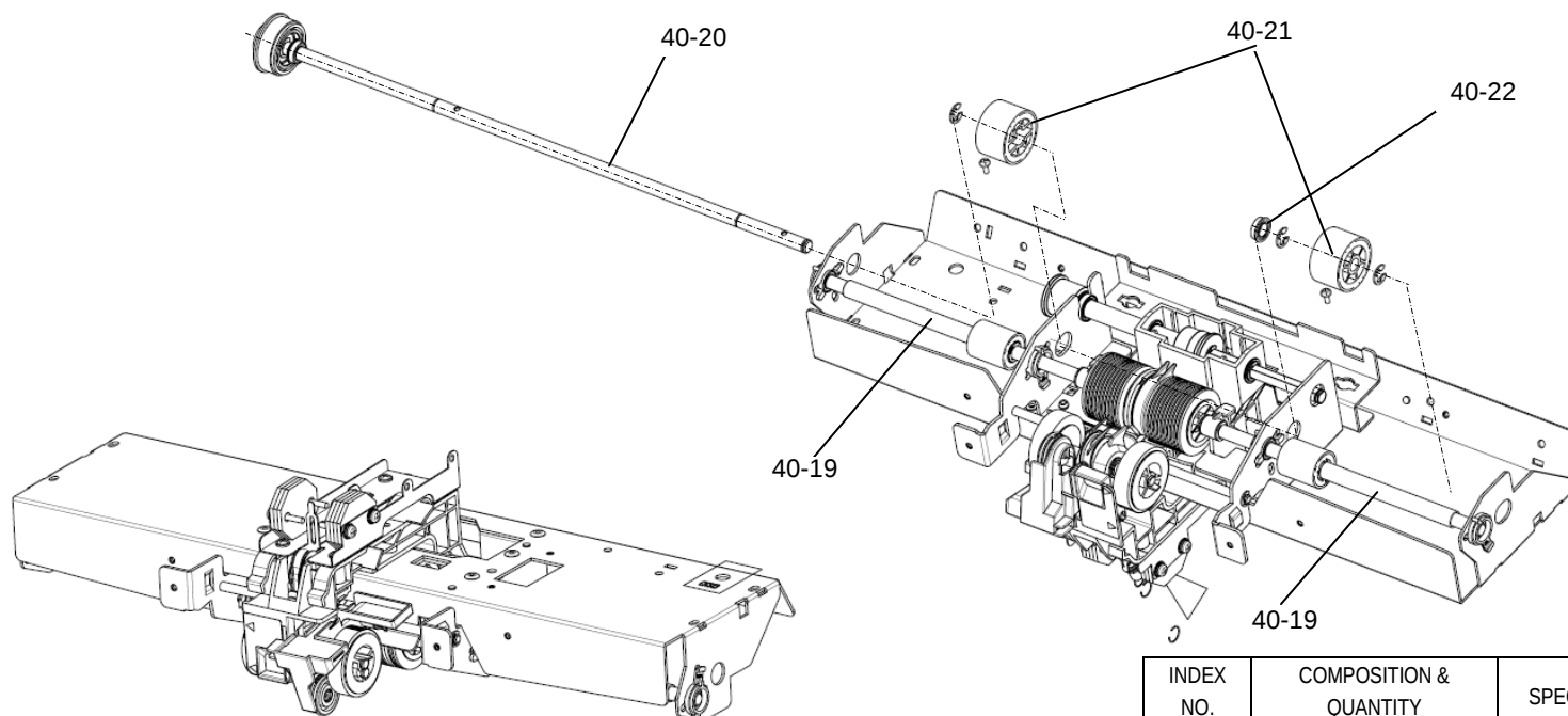
FIGURE 40. SEPARATOR UNIT 3/5
