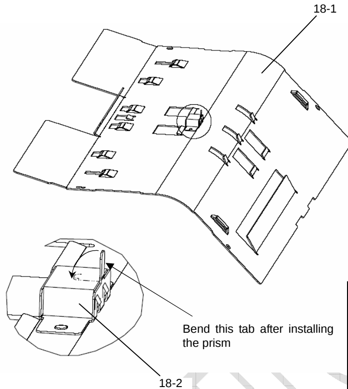
FIGURE 18. BASE GUIDE 1
