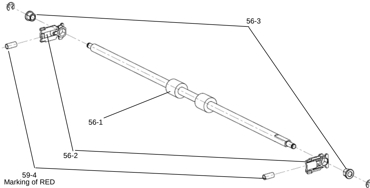
FIGURE 59. PINCH ROLLER ASSY 4
