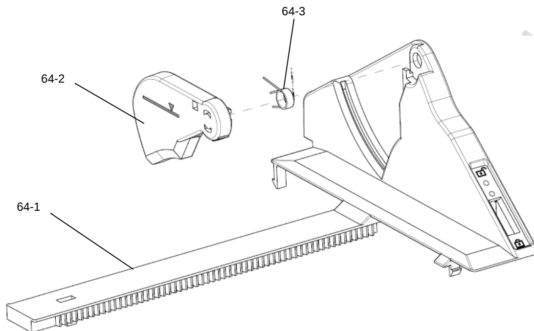
FIGURE 64. HOPPER GUIDE R ASSY
