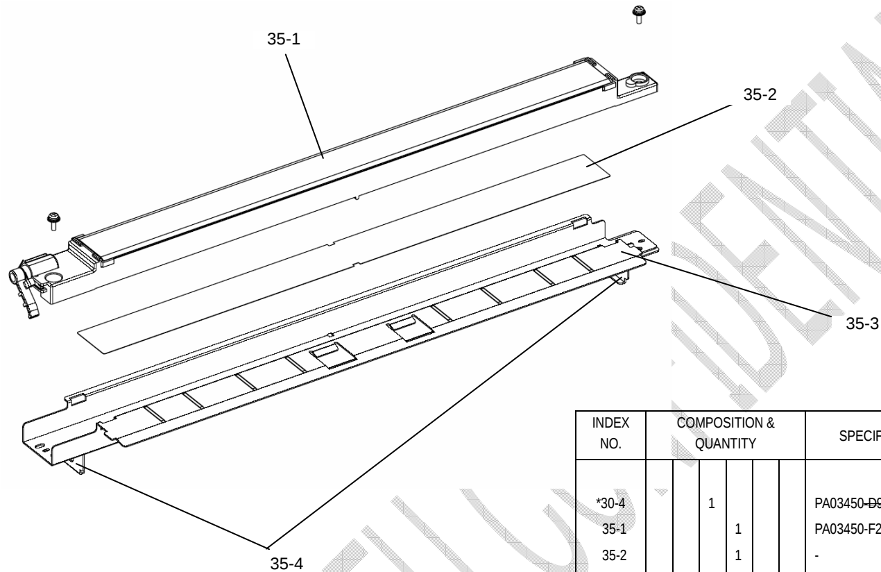
FIGURE 35. BACKGROUND UNIT, UPPER
