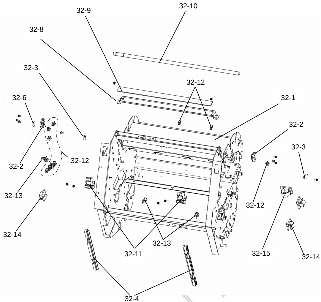
FIGURE 32. UPPER ASSY
