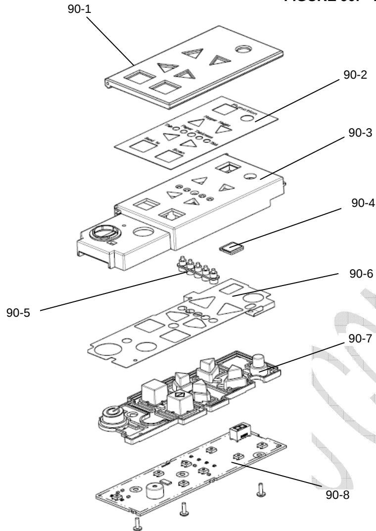
FIGURE 90. PANEL UNIT
