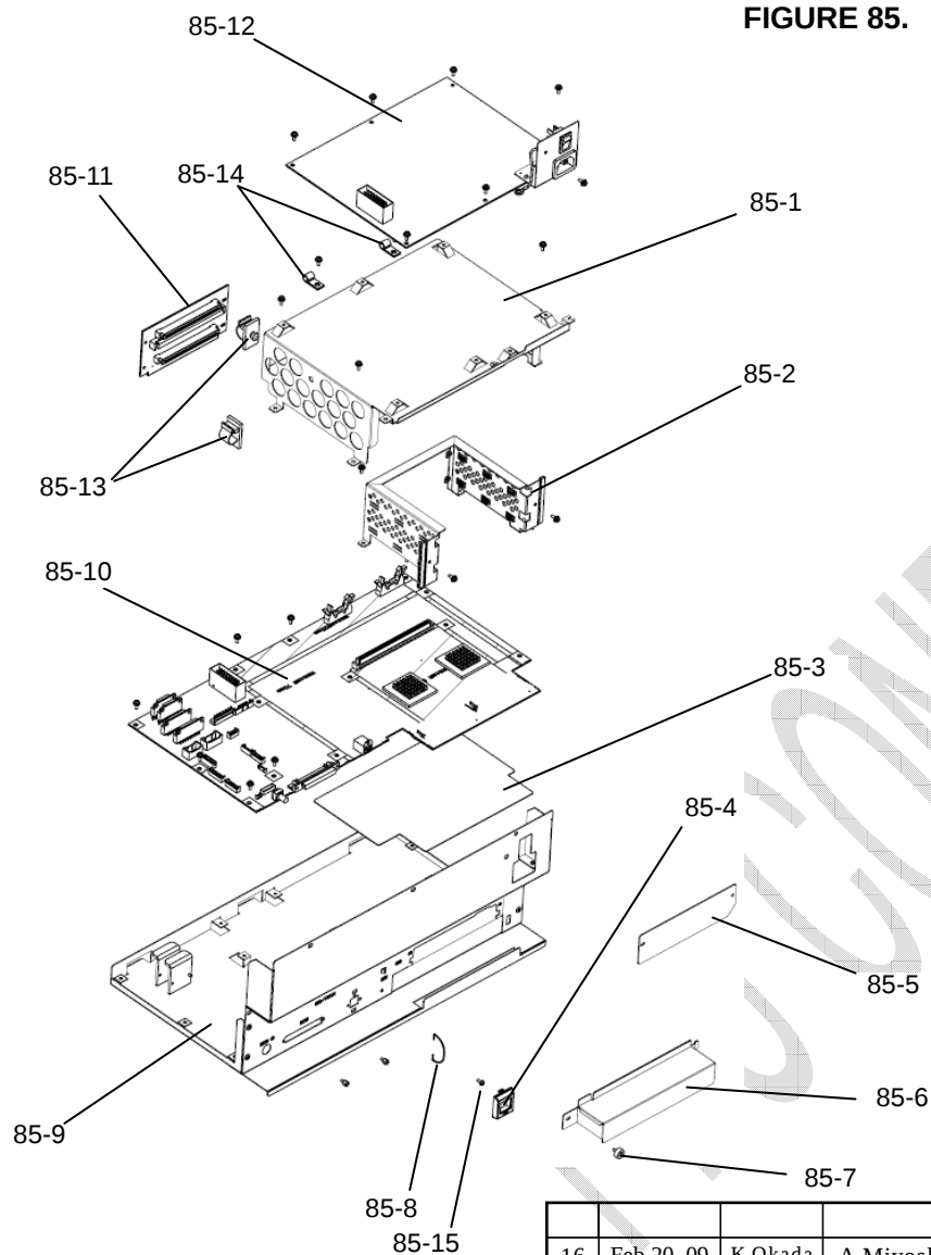
FIGURE 85. PCB UNIT
