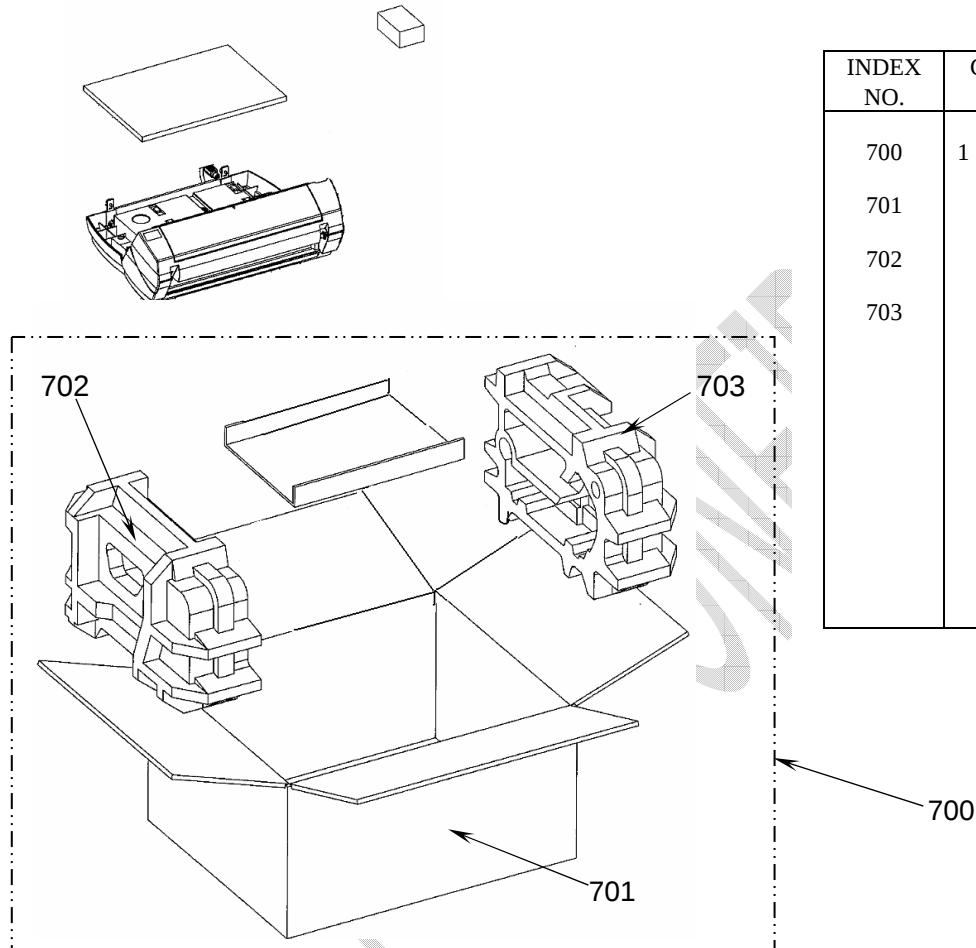
FIGURE 7. PACKAGING BOX for Imprinter (fi-553PR, option)
