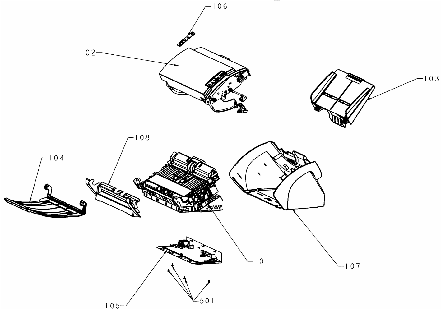
FIGURE 1. FINAL ASSEMBLY
