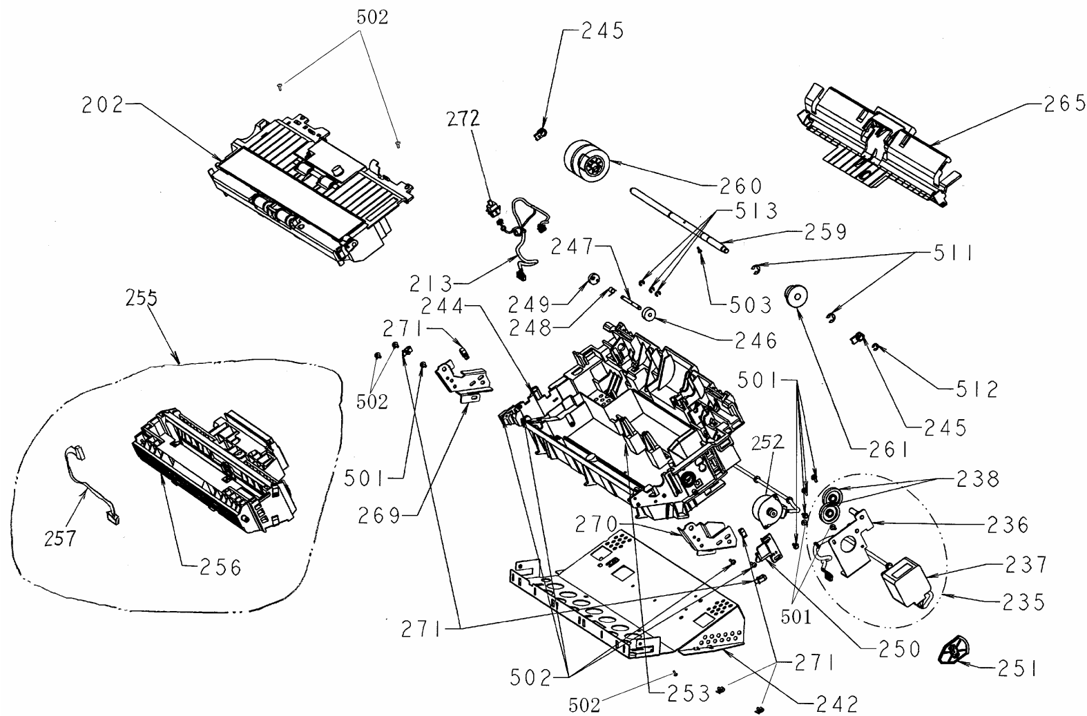
FIGURE 2-1. BASE UNIT
