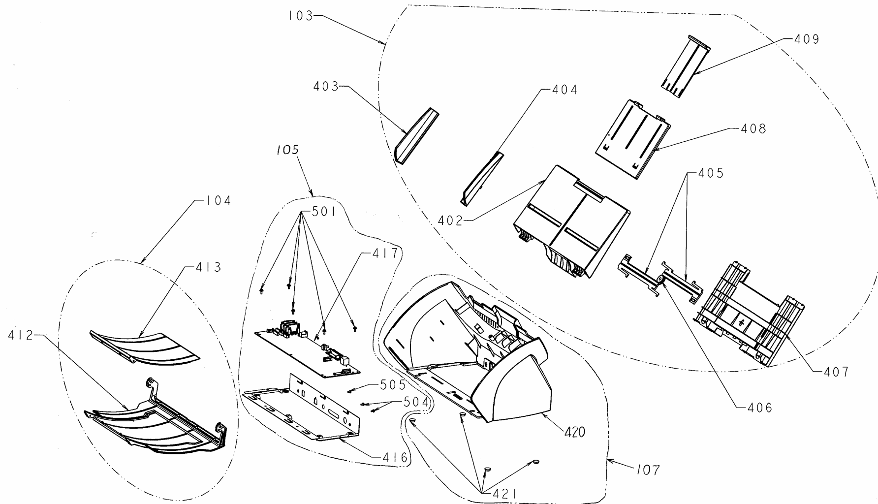
FIGURE 4. PCA, COVER, CHUTE AND STACKER
