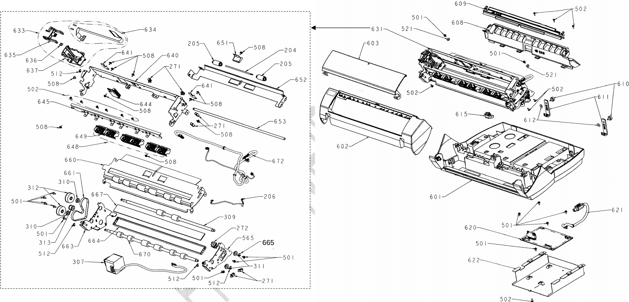
FIGURE 6. fi-553PR Imprinter (Option)
