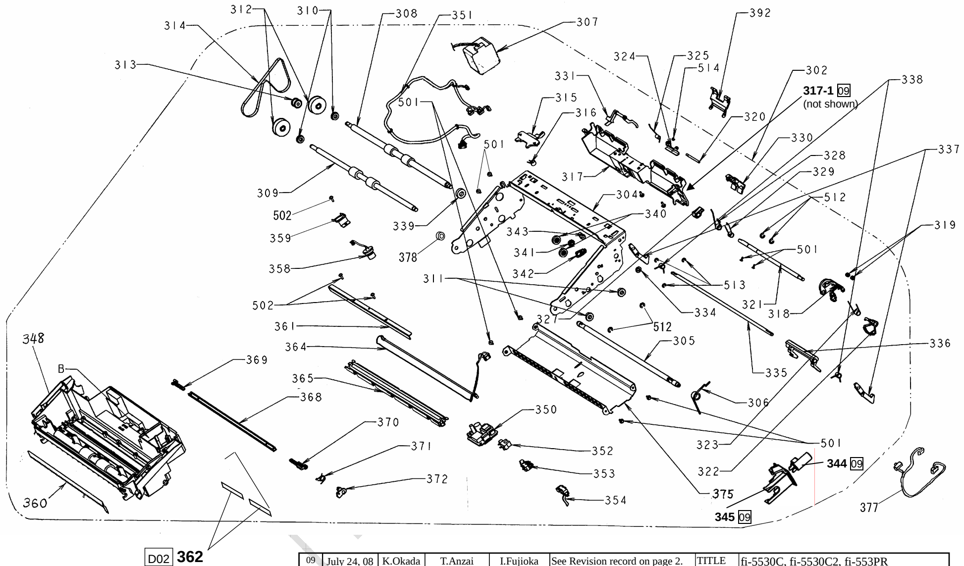
FIGURE 3-1. UPPER UNIT(1/2)
