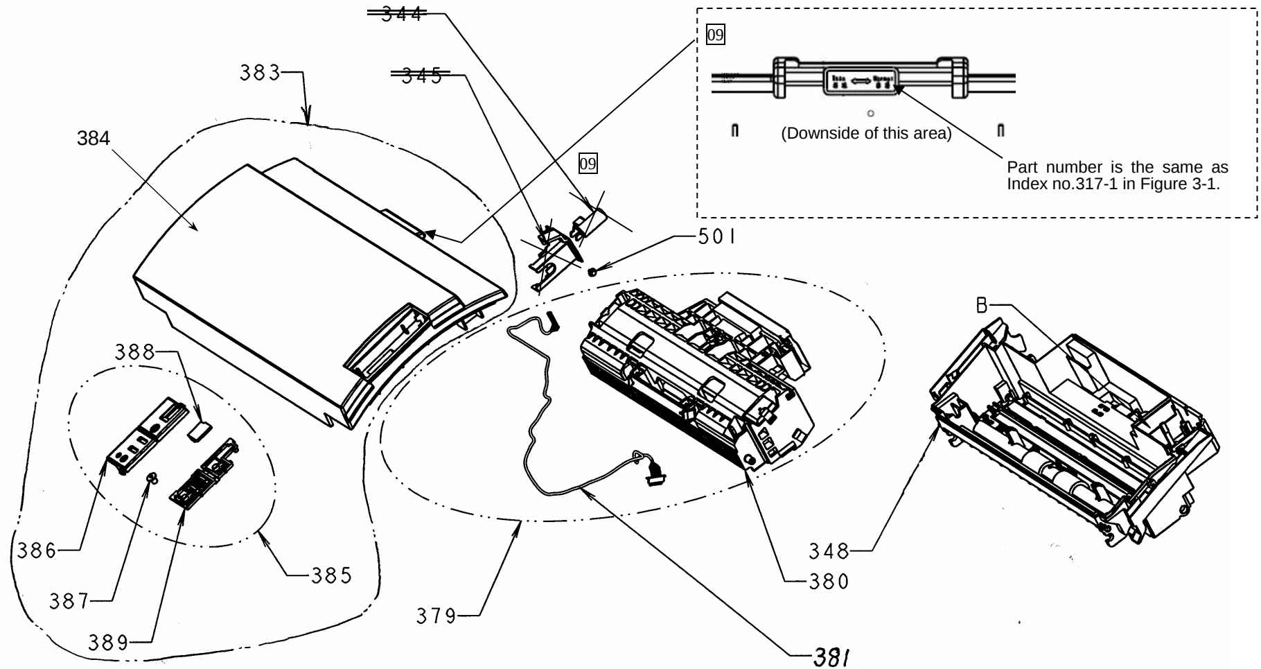
FIGURE 3-2. UPPER UNIT(2/2)
