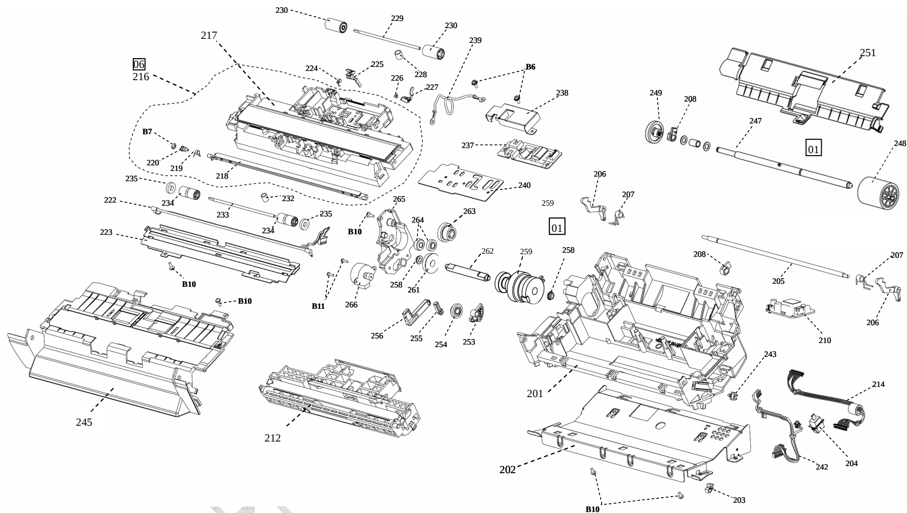
FIGURE 2 BASE UNIT
