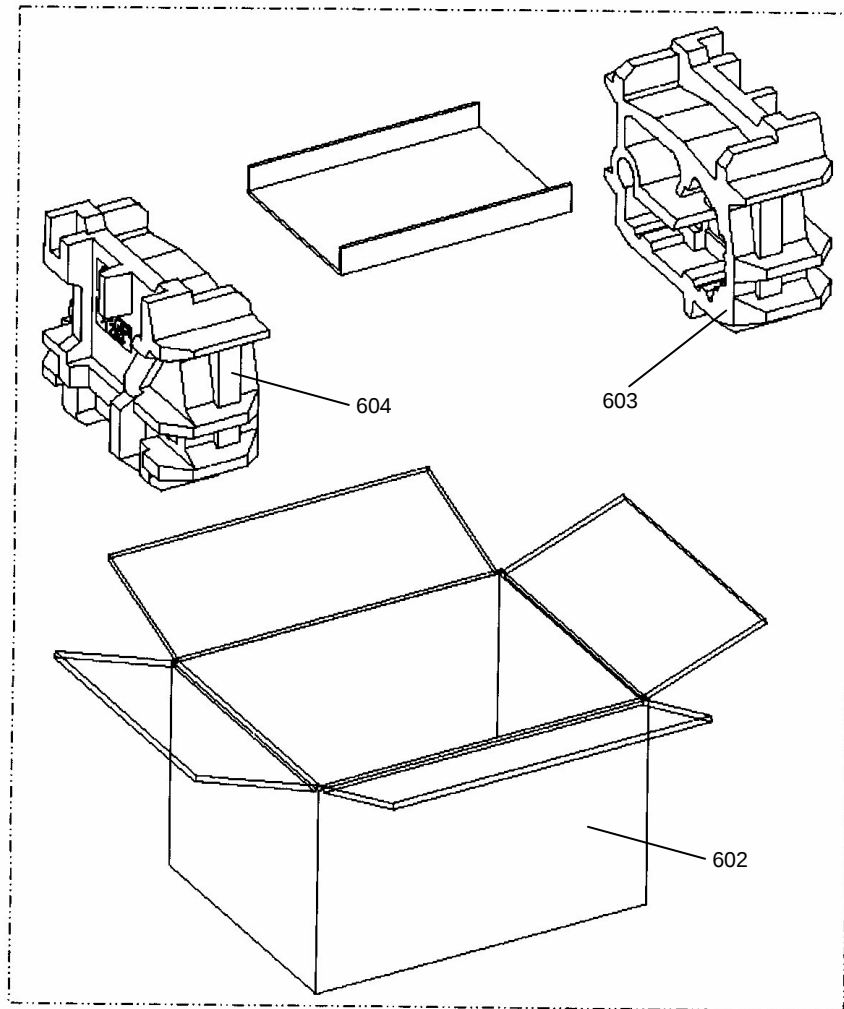
FIGURE 8 PACKAGE, IMPRINTER
