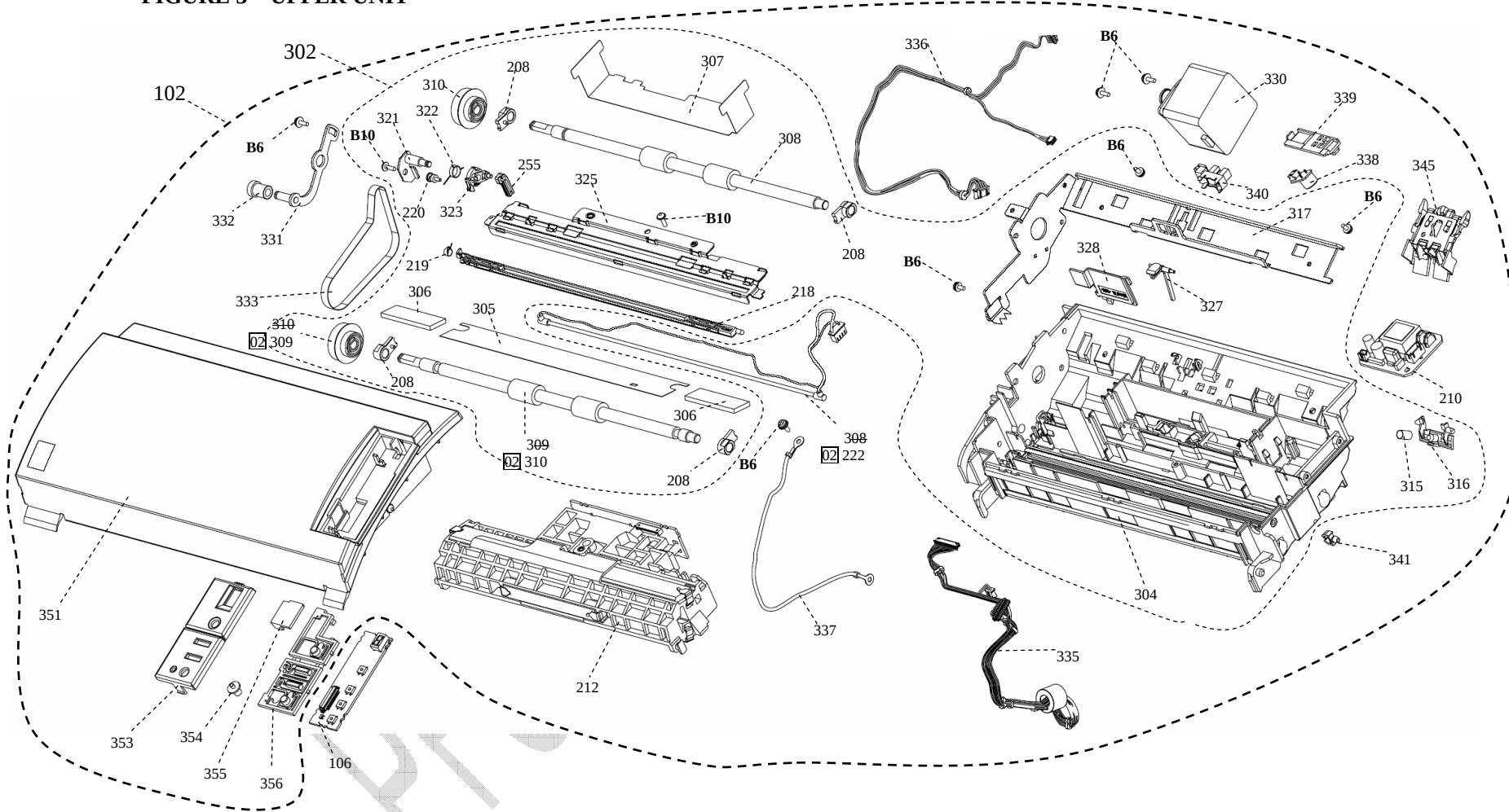
FIGURE 3 UPPER UNIT
