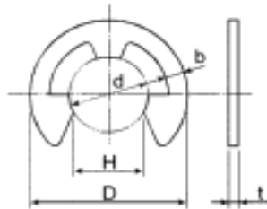
FIGURE B 3 RETAINING RING (E-RING)
