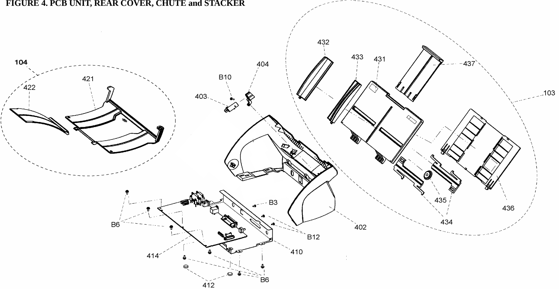
FIGURE 4. PCB UNIT, REAR COVER, CHUTE and STACKER
