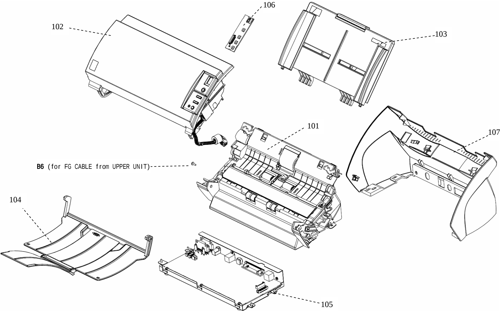
FIGURE 1 FINAL ASSEMBLY
