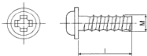
FIGURE B.4 PT SCREW
