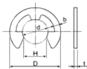
FIGURE B.3 E-RING
