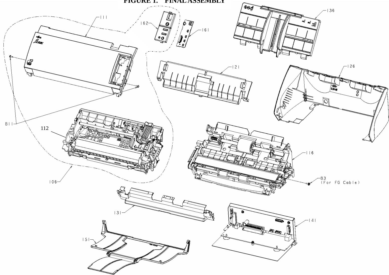
FIGURE 1. FINAL ASSEMBLY
