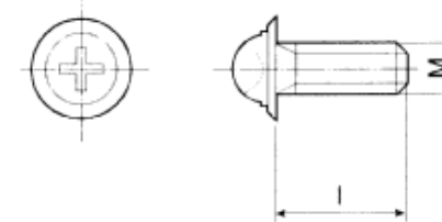
FIGURE B.1 SCREW
