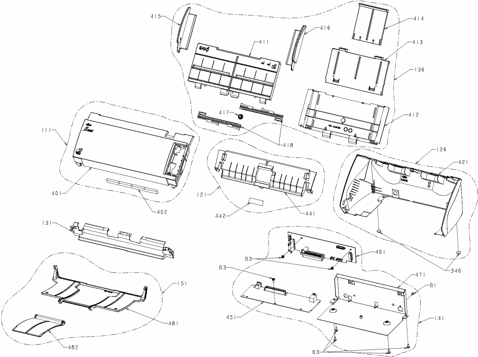
FIGURE 4. PCA, COVER, CHUTER AND STACKER
