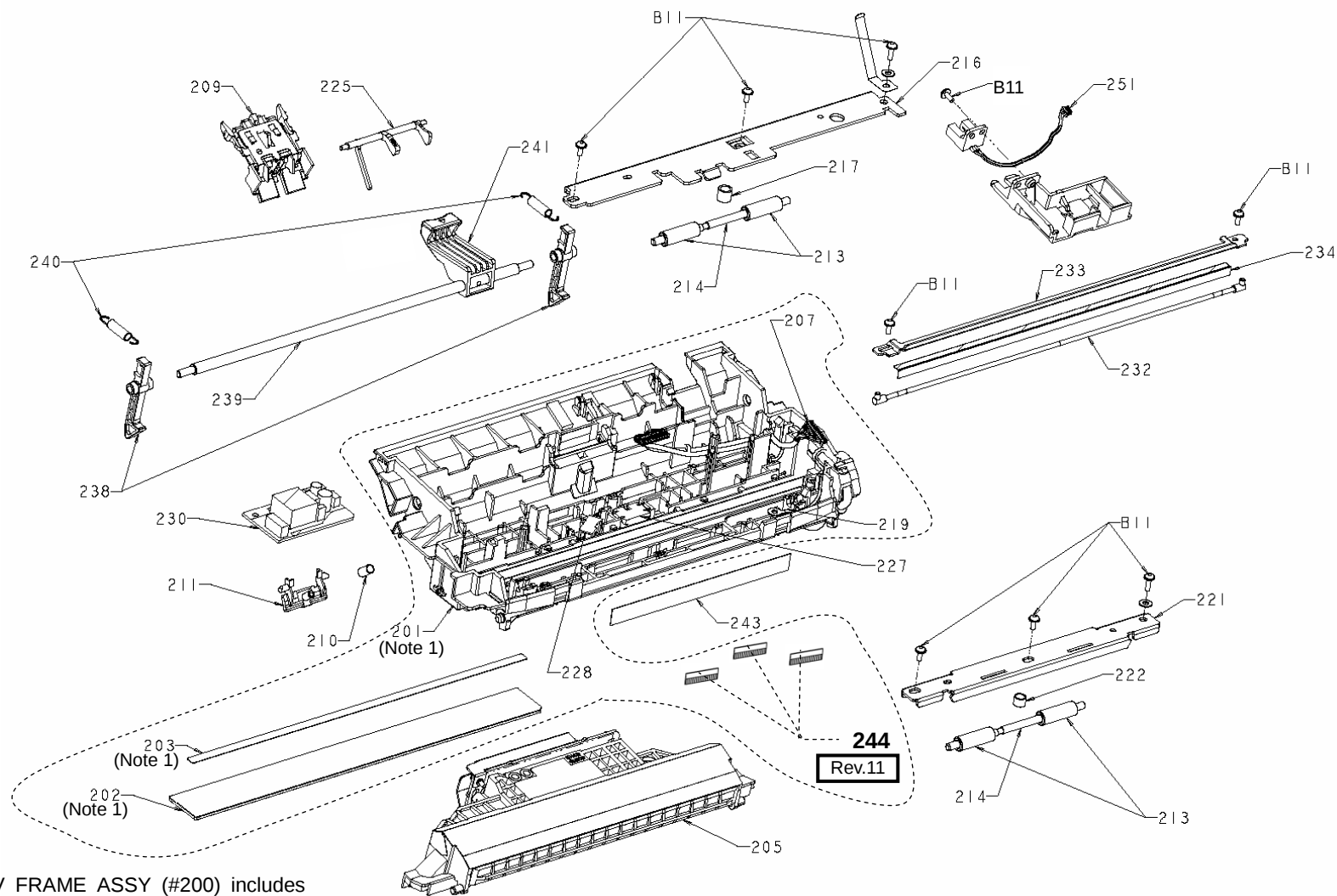
FIGURE 2. REVOLVE UNIT
