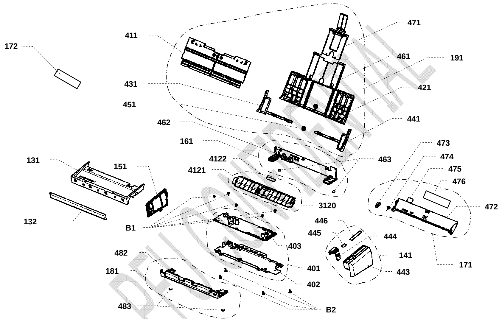
FIGURE 4. S1300i PCA, COVER, CHUTER
