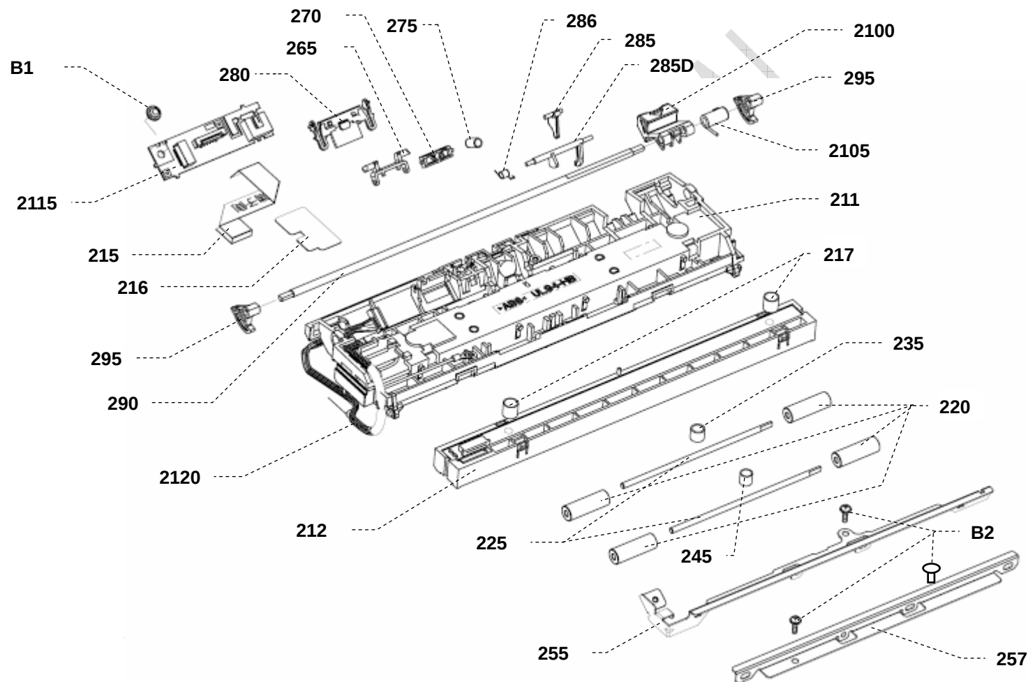
FIGURE 2. S1300i REVOLVE UNIT
