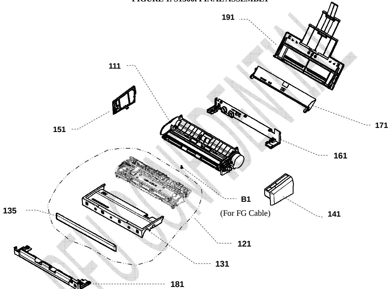
FIGURE 1. S1300i FINAL ASSEMBLY
