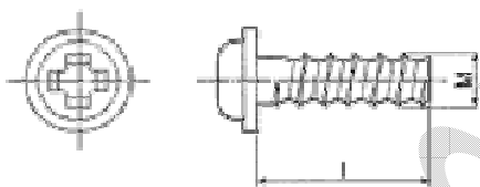
FIGURE B.2 SELF-TAPPING SCREW
