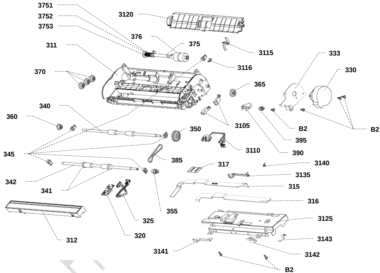
FIGURE 3. S1300i FIXED UNIT
