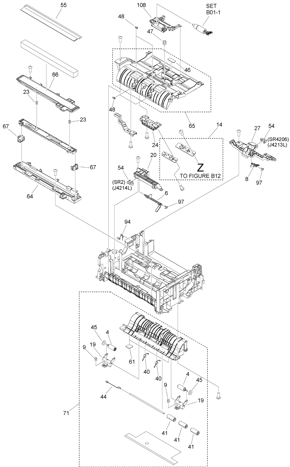
Figure B11 (3/3) AUTO DOCUMENT FEEDER ASS'Y SET
