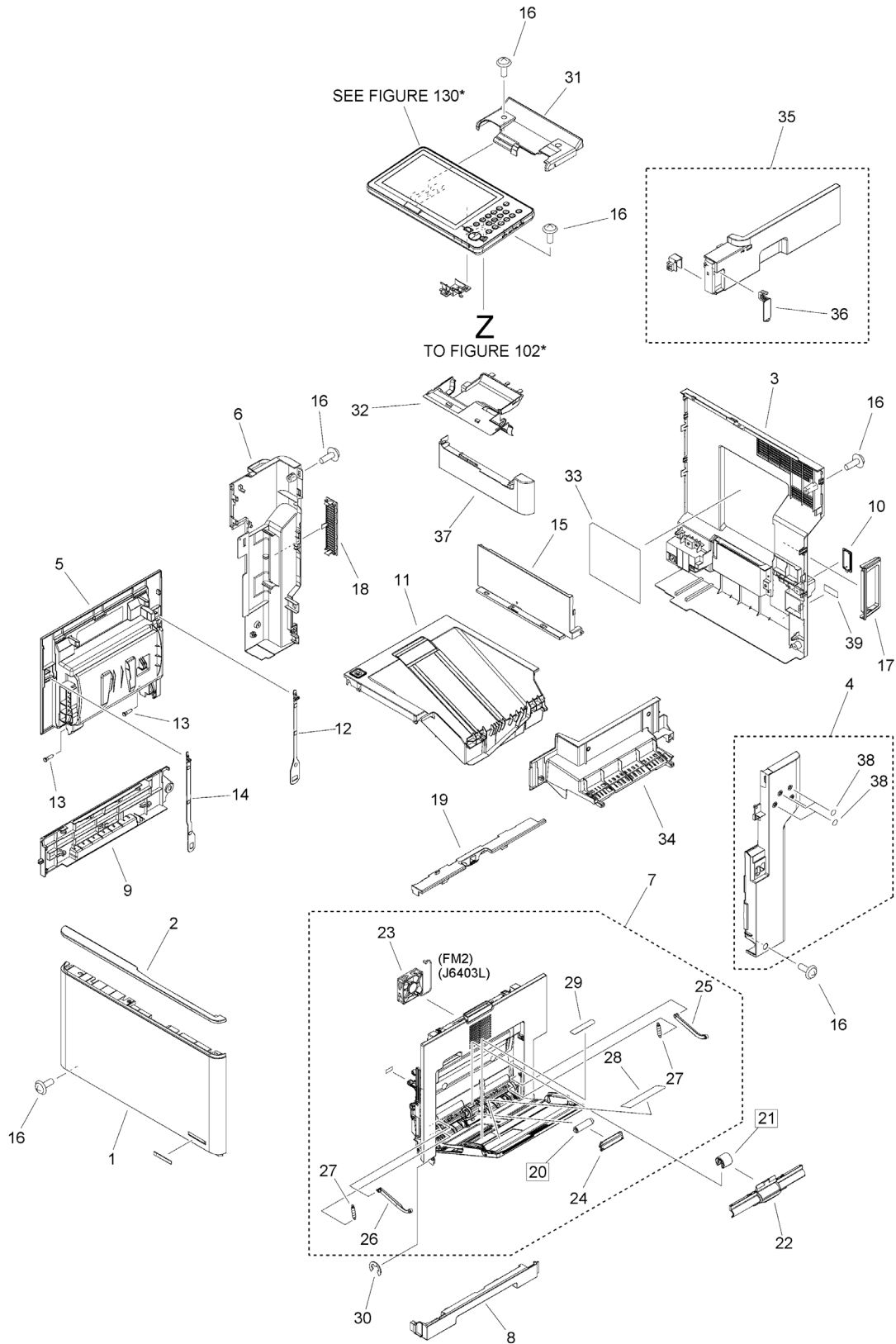
Figure 100L EXTERNAL COVERS, PANELS, ETC. (615i)
