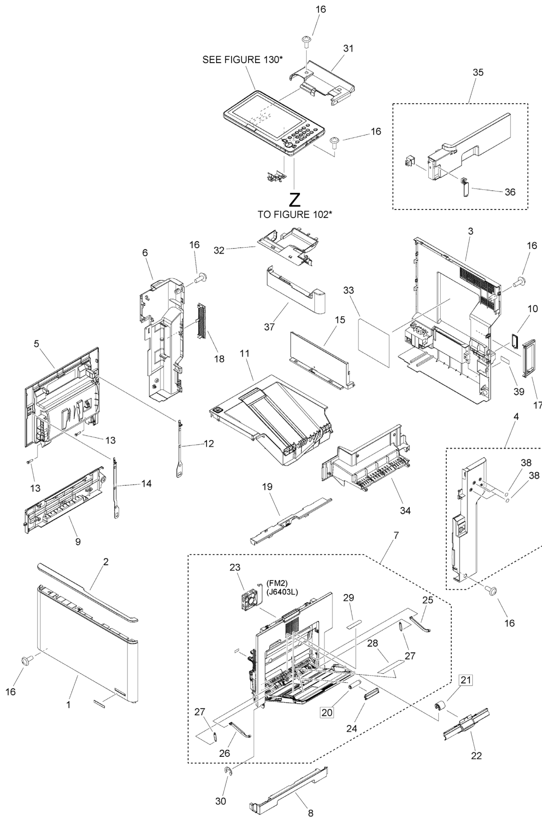
Figure 100M EXTERNAL COVERS, PANELS, ETC. (525i)
