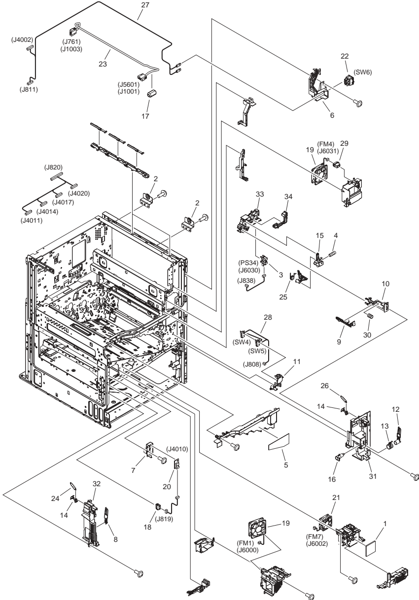
FIGURE 102 INTERNAL COMPONENTS 1
