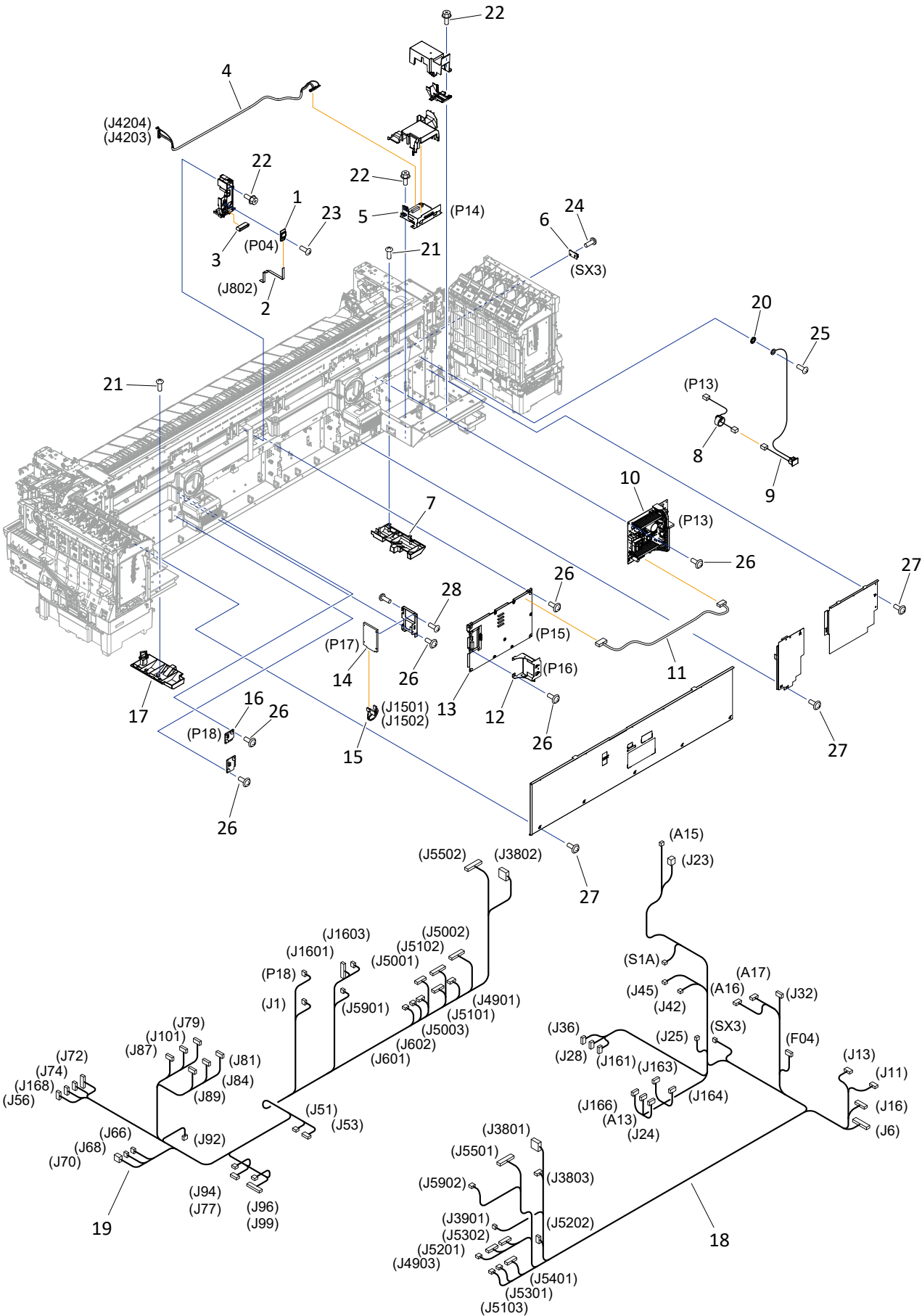
FIGURE 3 Electrical Parts
