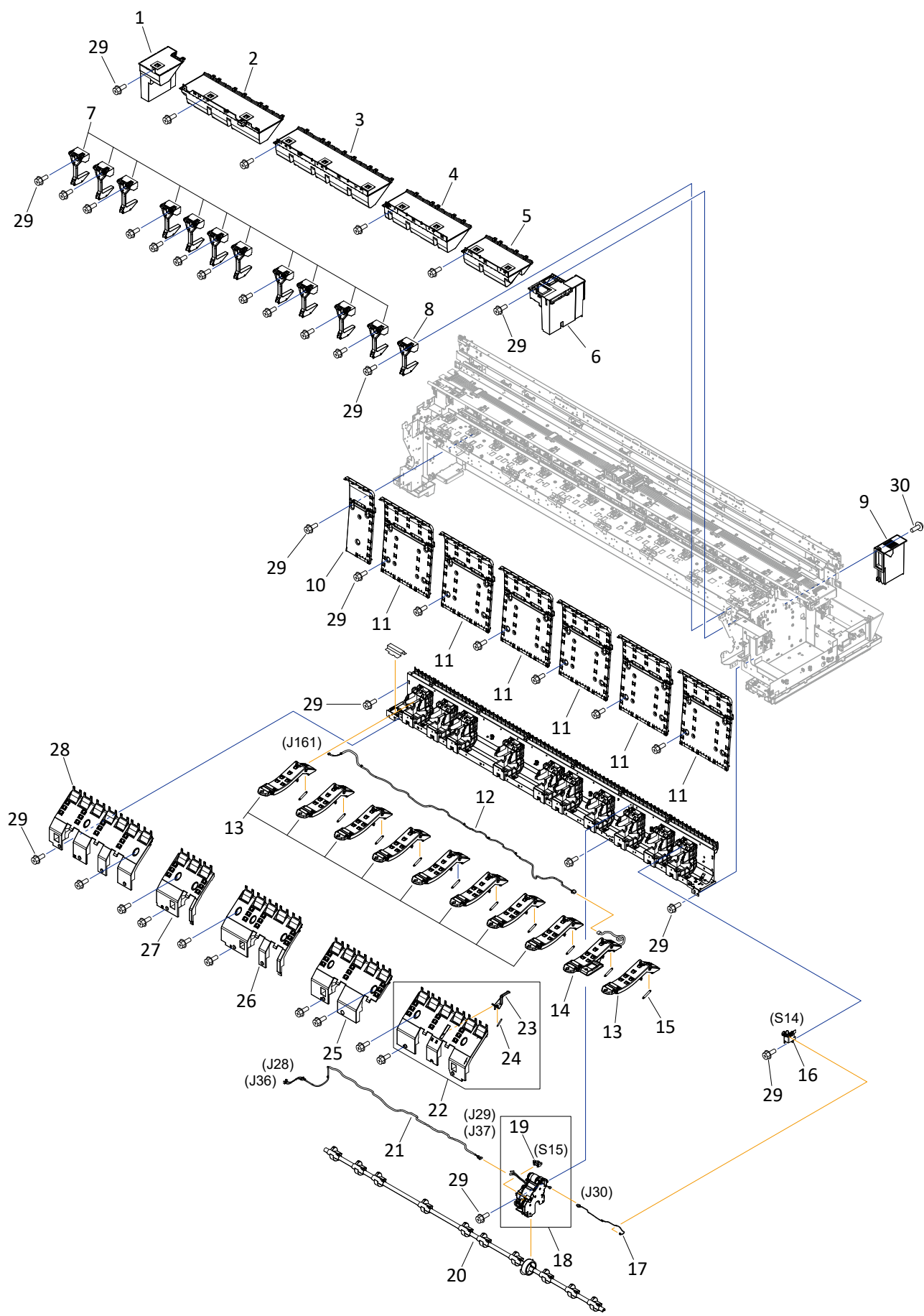
FIGURE 10 Upper Roll Unit, Suction Fan & Waste Ink Unit
