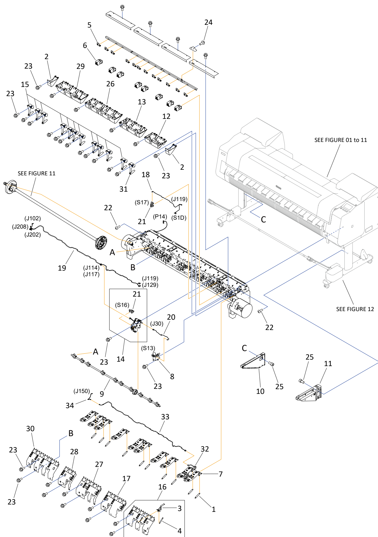
FIGURE R3 Lower Roll Unit RU-63 (Main)
