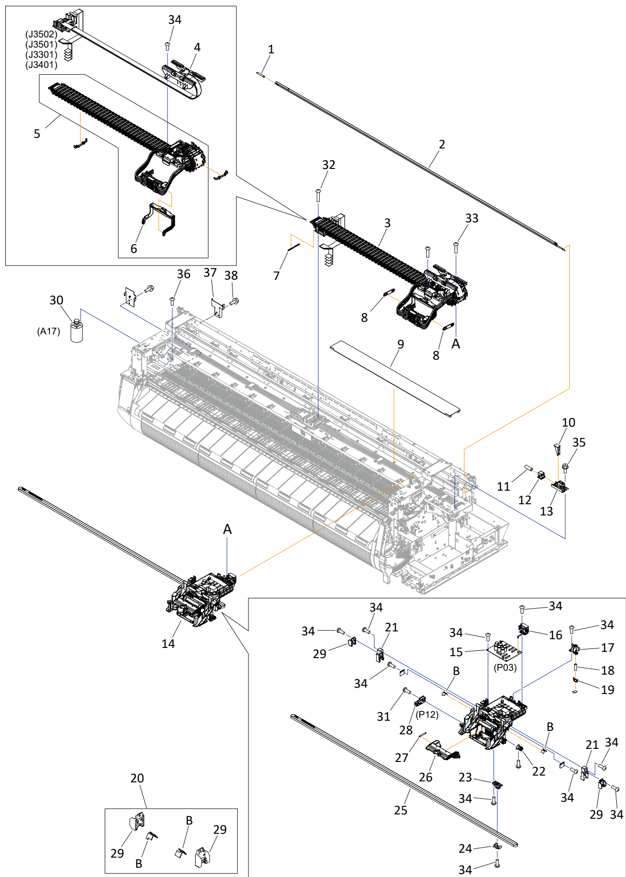
FIGURE 5 Carriage, Tube Unit & Film Strip
