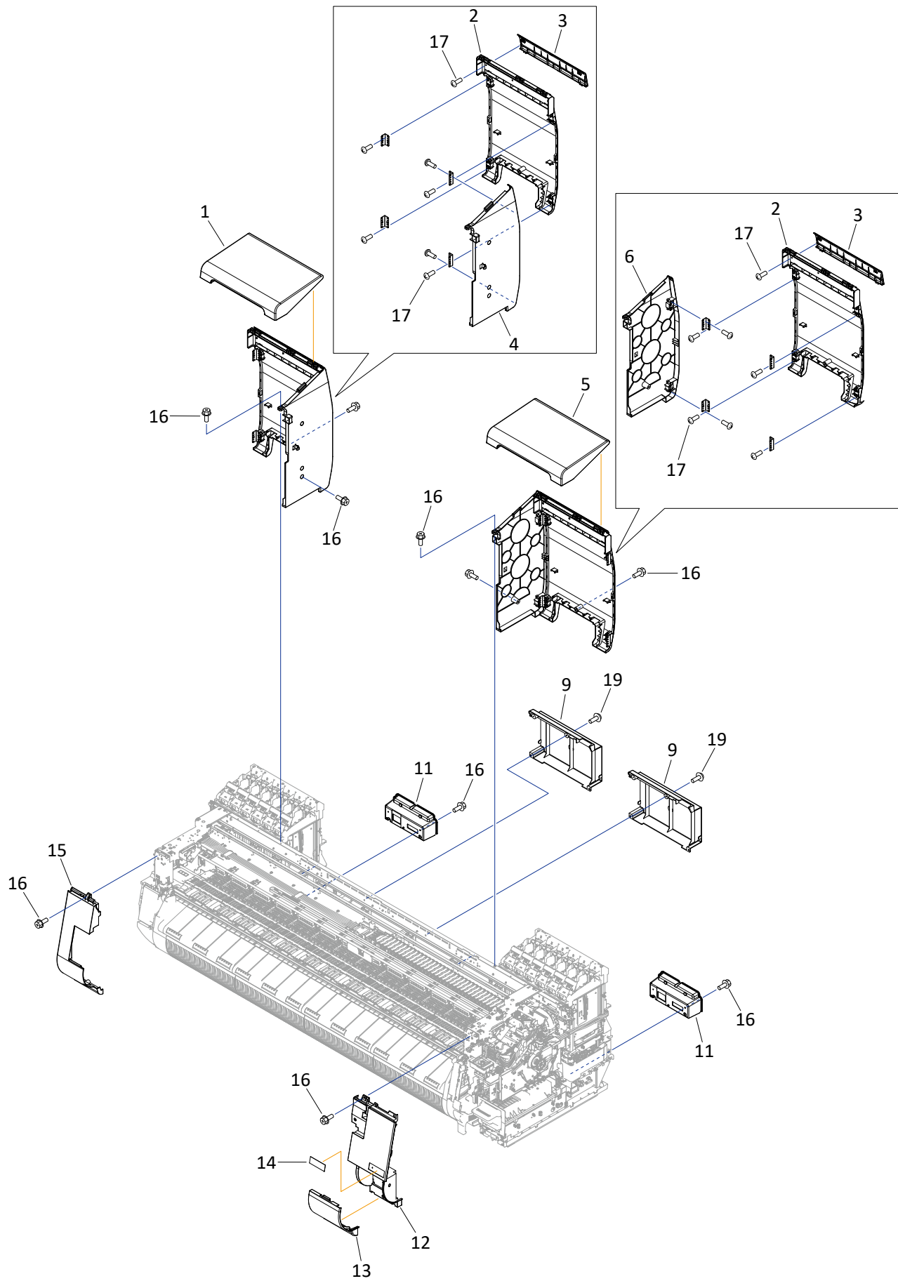
FIGURE 2 Front Covers & Rear Covers
