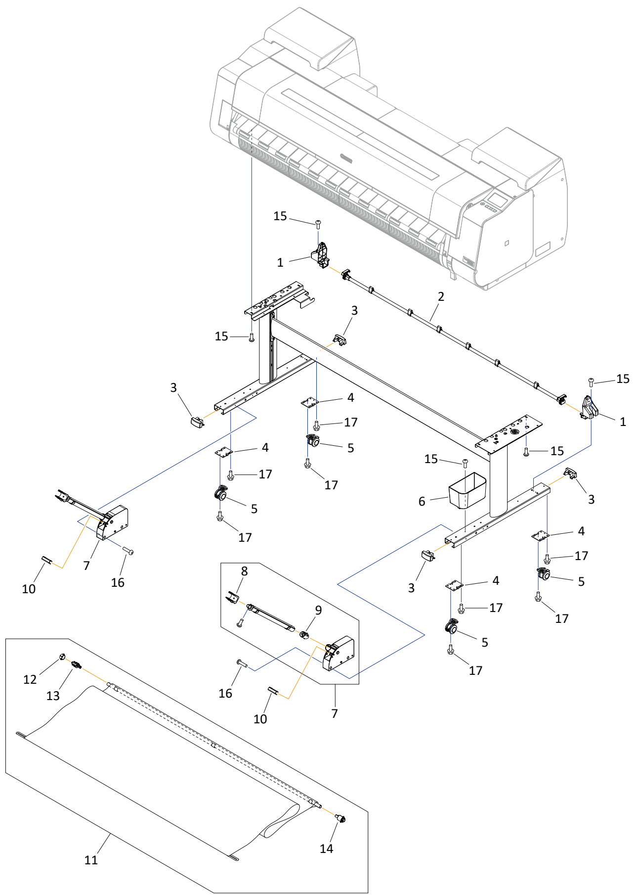
FIGURE 12 Stand Unit
